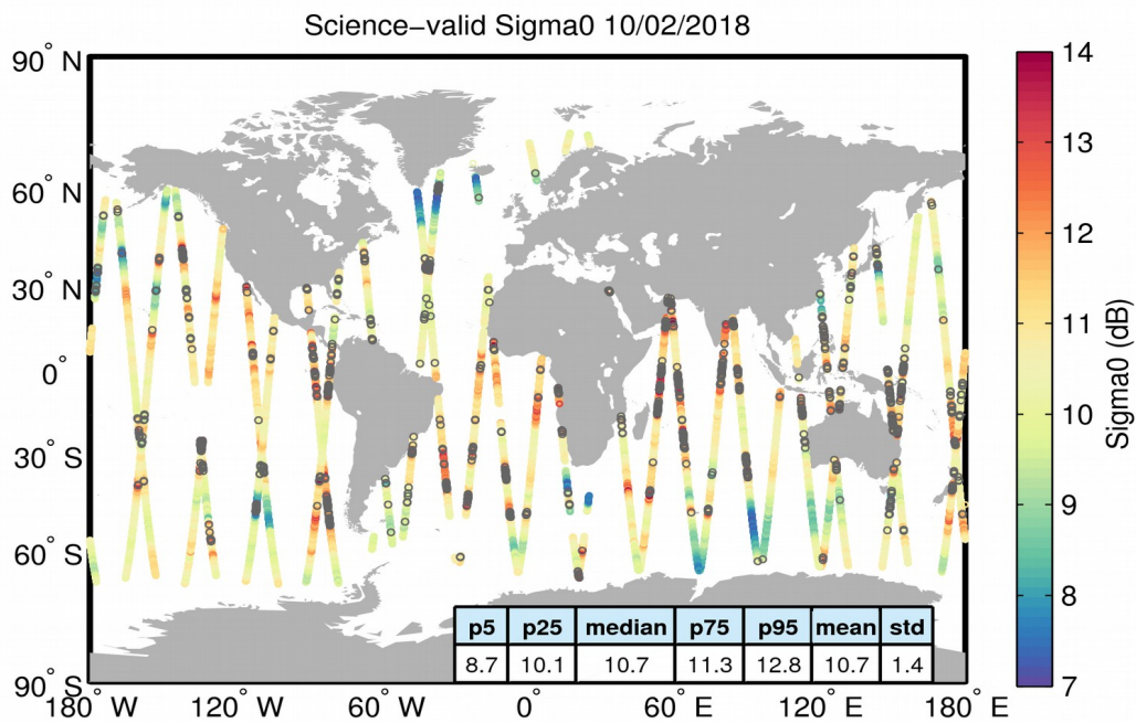
Figure 27. Geographical distribution of science-valid sigma0 data over oceans and lakes for 10/02/2018. The statistical values shown in the table refer to the sigma0 in dB and are calculated over all measurements shown in the figure. Gray circles denote records that have been rejected based on the editing criteria described in Table 4.
