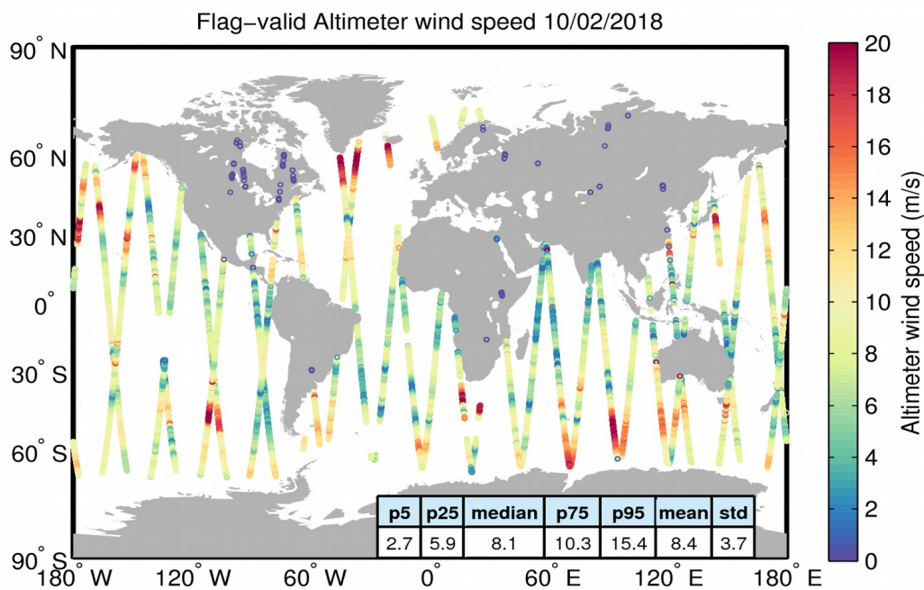
Figure 31. Geographical distribution of flag-valid wind data over oceans and lakes for 10/02/2018. The statistical values shown in the table refer to the wind in m/s and are calculated over all measurements shown in the figure.
