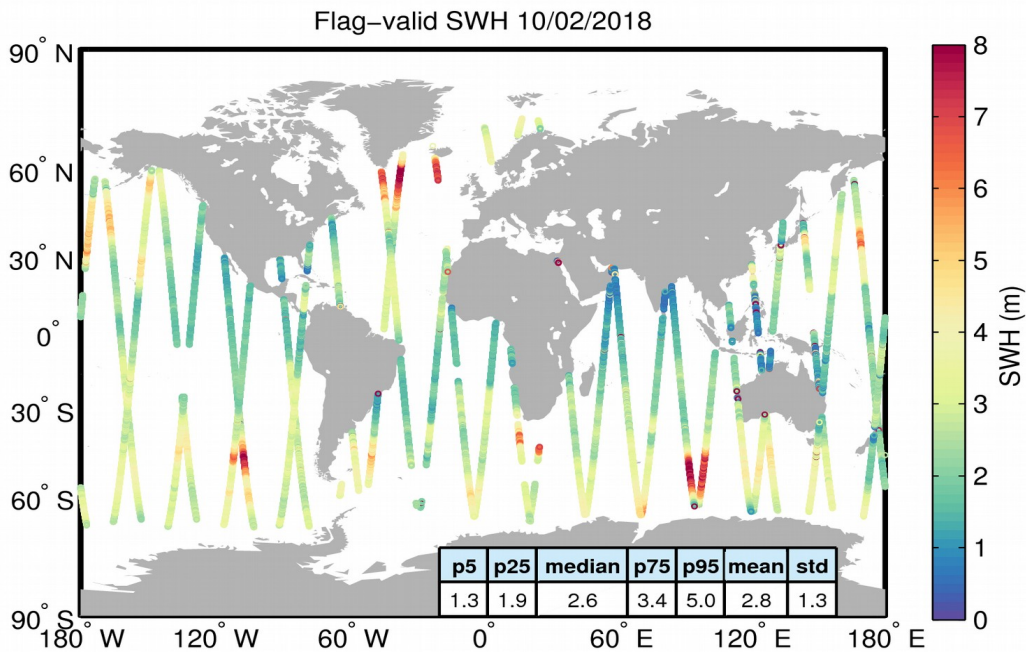
Figure 15. Geographical distribution of flag-valid SWH data over oceans and lakes for 10/02/2018. The statistical values shown in the table refer to the SWH in m and are calculated over all measurements shown in the figure.
