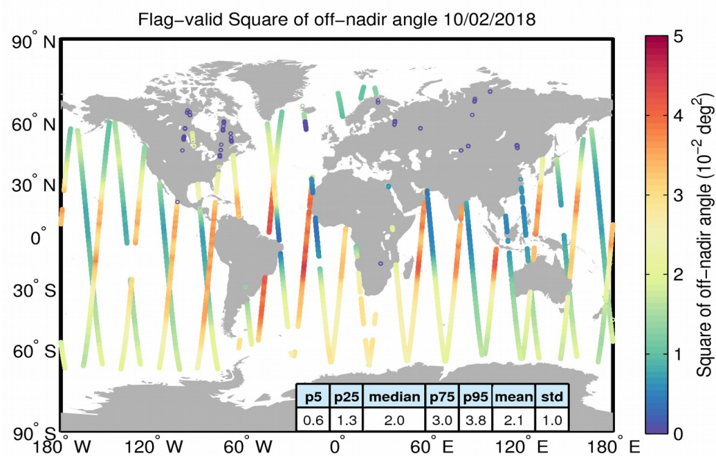
Figure 37. Geographical distribution of flag-valid mispointing data over oceans and lakes for 10/02/2018. The statistical values shown in the table refer to the mispointing in 10^{-2} deg 2 and are calculated over all measurements shown in the figure.
