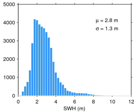
Figure 17. Histogram of flag-valid SWH over oceans and lakes for 10/02/2018. The mean ( \mu ) and standard deviation ( \sigma ) are also shown. Note that values larger than 12 m are excluded from the histogram for the sake of readability but not from the computation of \mu and \sigma .
