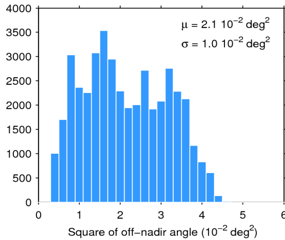
Figure 39. Histogram of flag-valid mispointing over oceans and lakes for 10/02/2018. The mean ( \mu ) and standard deviation ( \sigma ) are also shown. Note that values larger than 6 \cdot 10^{-2} \text{ deg}^2 are excluded from the histogram for the sake of readability but not from the computation of \mu and \sigma .
