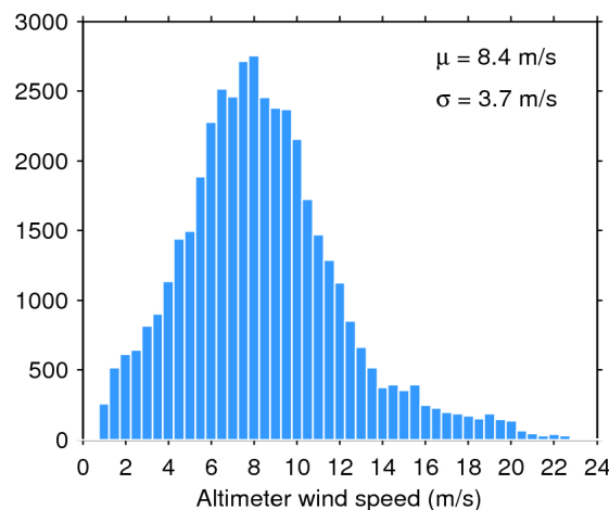
Figure 35. Histogram of science-valid wind over oceans and lakes for 10/02/2018. The mean ( \mu ) and standard deviation ( \sigma ) are also shown. Note that values larger than 24 m/s are excluded from the histogram for the sake of readability but not from the computation of \mu and \sigma .
