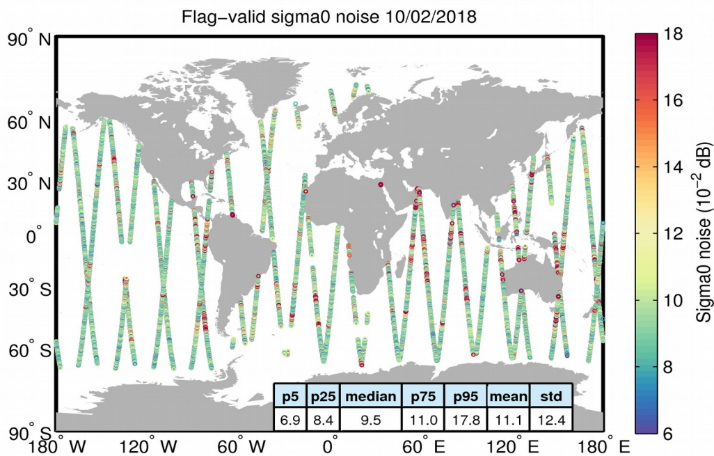
Figure 26. Geographical distribution of flag-valid 20-Hz sigma0 measurement noise over oceans and lakes for 10/02/2018. The statistical values shown in the table refer to the sigma0 noise and are calculated over all measurements shown in the figure.
