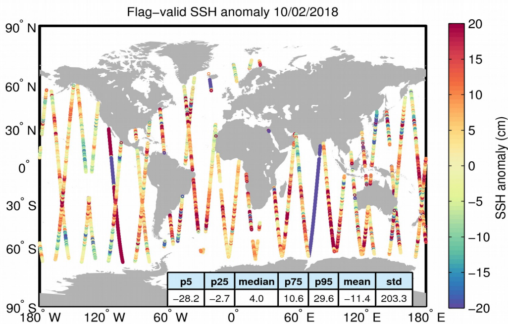
Figure 5. Geographical distribution of flag-valid 1-Hz SSH anomaly data over oceans and lakes for 10/02/2018. The statistical values shown in the table refer to the SSH anomaly in cm and are calculated over all measurements shown in the figure.
