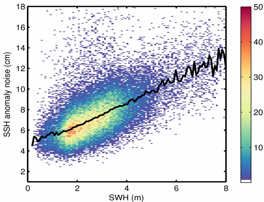
Figure 9. 2D histogram showing flag-valid SSH anomaly noise as a function of SWH for 10/02/2018. The black line denotes the median SSH anomaly noise as a function of SWH.
