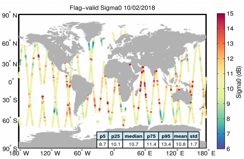
Figure 23. Geographical distribution of flag-valid sigma0 data over oceans and lakes for 10/02/2018. The statistical values shown in the table refer to the sigma0 in dB and are calculated over all measurements shown in the figure.
