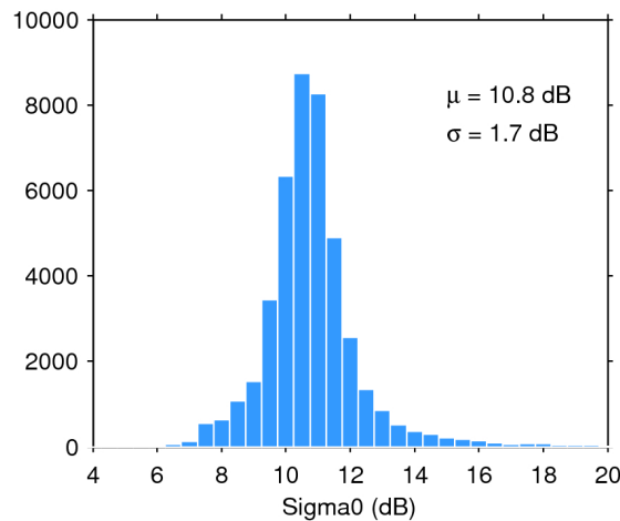
Figure 25. Histogram of flag-valid sigma0 over oceans and lakes for 10/02/2018. The mean ( \mu ) and standard deviation ( \sigma ) are also shown. Note that values outside [4 20] dB are excluded from the histogram for the sake of readability but not from the computation of \mu and \sigma .
