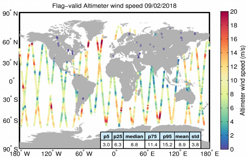
Figure 31. Geographical distribution of flag-valid wind data over oceans and lakes for 09/02/2018. The statistical values shown in the table refer to the wind in m/s and are calculated over all measurements shown in the figure.
