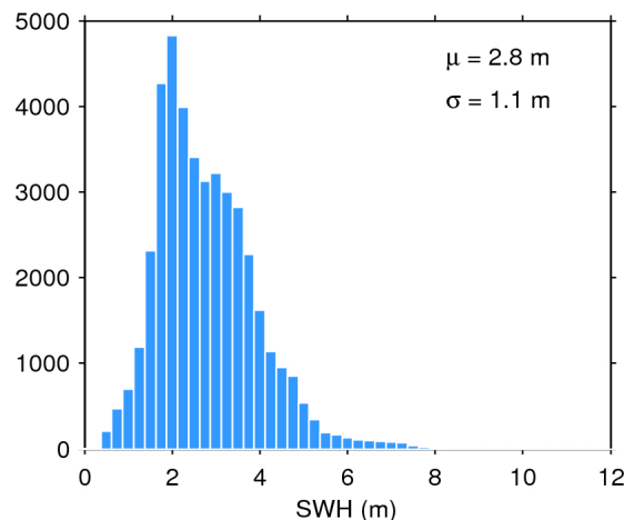
Figure 20. Histogram of science-valid SWH over oceans and lakes for 09/02/2018. The mean ( \mu ) and standard deviation ( \sigma ) are also shown. Note that values larger than 12 m are excluded from the histogram for the sake of readability but not from the computation of \mu and \sigma .
