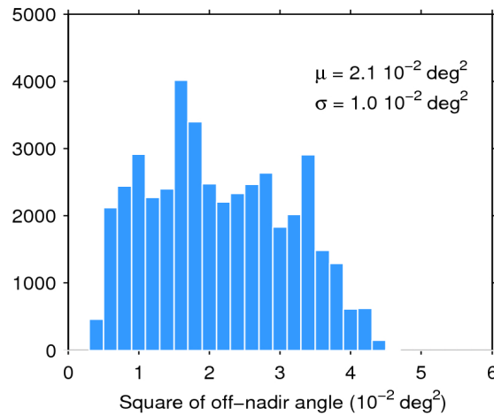
Figure 39. Histogram of flag-valid mispointing over oceans and lakes for 09/02/2018. The mean ( \mu ) and standard deviation ( \sigma ) are also shown. Note that values larger than 6 \cdot 10^{-2} \text{ deg}^2 are excluded from the histogram for the sake of readability but not from the computation of \mu and \sigma .
