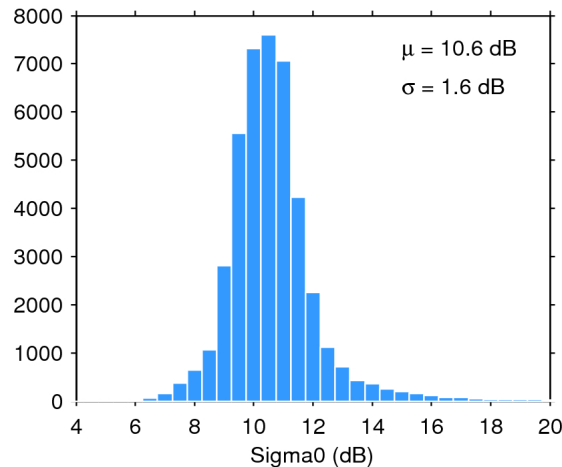
Figure 25. Histogram of flag-valid sigma0 over oceans and lakes for 09/02/2018. The mean ( \mu ) and standard deviation ( \sigma ) are also shown. Note that values outside [4 20] dB are excluded from the histogram for the sake of readability but not from the computation of \mu and \sigma .
