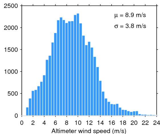
Figure 35. Histogram of science-valid wind over oceans and lakes for 09/02/2018. The mean ( \mu ) and standard deviation ( \sigma ) are also shown. Note that values larger than 24 m/s are excluded from the histogram for the sake of readability but not from the computation of \mu and \sigma .
