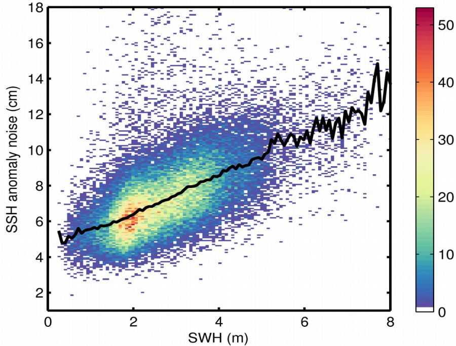
Figure 9. 2D histogram showing flag-valid SSH anomaly noise as a function of SWH for 09/02/2018. The black line denotes the median SSH anomaly noise as a function of SWH.
