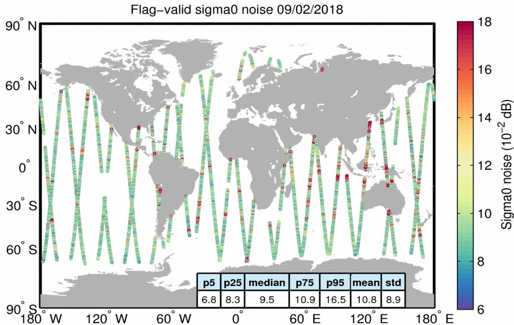
Figure 26. Geographical distribution of flag-valid 20-Hz sigma0 measurement noise over oceans and lakes for 09/02/2018. The statistical values shown in the table refer to the sigma0 noise and are calculated over all measurements shown in the figure.
