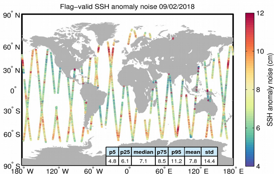
Figure 8. Geographical distribution of flag-valid 20-Hz SSH anomaly measurement noise over oceans and lakes for 09/02/2018. The statistical values shown in the table refer to the SSH anomaly noise and are calculated over all measurements shown in the figure.
