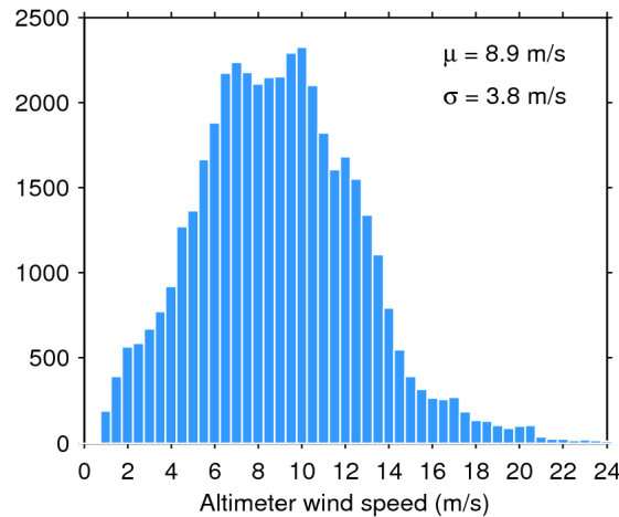
Figure 33. Histogram of flag-valid wind over oceans and lakes for 09/02/2018. The mean ( \mu ) and standard deviation ( \sigma ) are also shown. Note that values larger than 24 m/s are excluded from the histogram for the sake of readability but not from the computation of \mu and \sigma .
