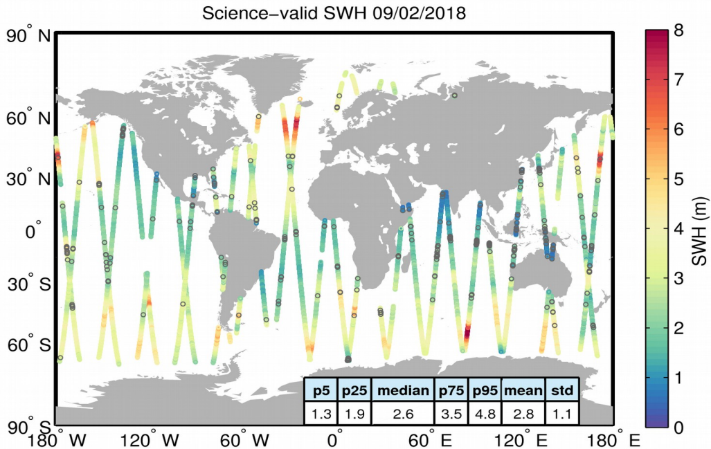
Figure 19. Geographical distribution of science-valid SWH data over oceans and lakes for 09/02/2018. The statistical values shown in the table refer to the SWH in m and are calculated over all measurements shown in the figure. Gray circles denote records that have been rejected based on the editing criteria described in Table 3.
