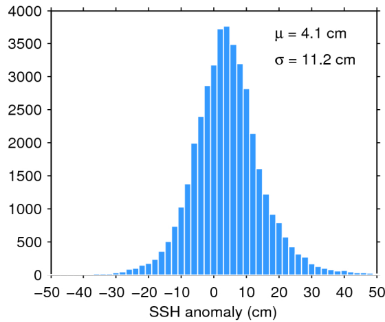
Figure 11. Histogram of science-valid SSH anomaly over oceans and lakes for 09/02/2018. The mean ( \mu ) and standard deviation ( \sigma ) are also shown. Note that values outside [-50 50] cm are excluded from the histogram for the sake of readability but not from the computation of \mu and \sigma .
