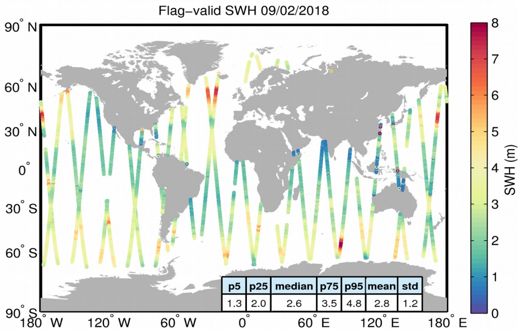
Figure 15. Geographical distribution of flag-valid SWH data over oceans and lakes for 09/02/2018. The statistical values shown in the table refer to the SWH in m and are calculated over all measurements shown in the figure.
