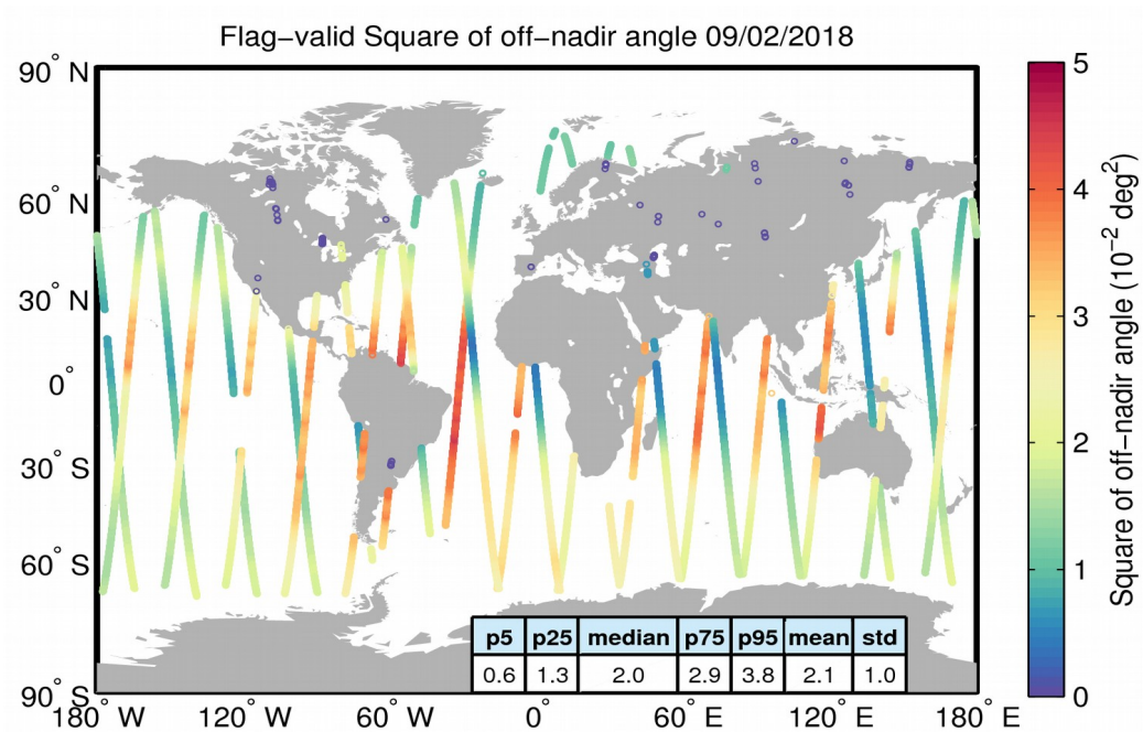
Figure 37. Geographical distribution of flag-valid mispointing data over oceans and lakes for 09/02/2018. The statistical values shown in the table refer to the mispointing in 10^{-2} \text{deg}^2 and are calculated over all measurements shown in the figure.
