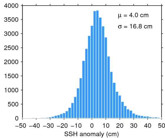
Figure 7. Histogram of flag-valid SSH anomaly over oceans and lakes for 09/02/2018. The mean ( \mu ) and standard deviation ( \sigma ) are also shown. Note that values outside [-50 50] cm are excluded from the histogram for the sake of readability but not from the computation of \mu and \sigma .
