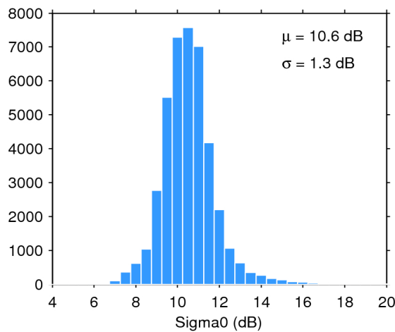
Figure 28. Histogram of science-valid sigma0 over oceans and lakes for 09/02/2018. The mean ( \mu ) and standard deviation ( \sigma ) are also shown. Note that values outside [4 20] dB are excluded from the histogram for the sake of readability but not from the computation of \mu and \sigma .
