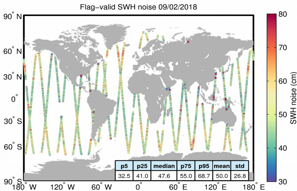
Figure 18. Geographical distribution of flag-valid 20-Hz SWH measurement noise over oceans and lakes for 09/02/2018. The statistical values shown in the table refer to the SWH noise and are calculated over all measurements shown in the figure.
