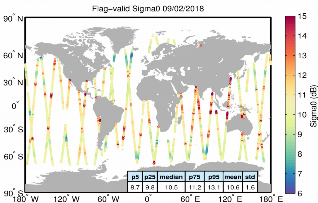
Figure 23. Geographical distribution of flag-valid sigma0 data over oceans and lakes for 09/02/2018. The statistical values shown in the table refer to the sigma0 in dB and are calculated over all measurements shown in the figure.
