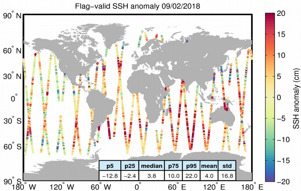
Figure 5. Geographical distribution of flag-valid 1-Hz SSH anomaly data over oceans and lakes for 09/02/2018. The statistical values shown in the table refer to the SSH anomaly in cm and are calculated over all measurements shown in the figure.
