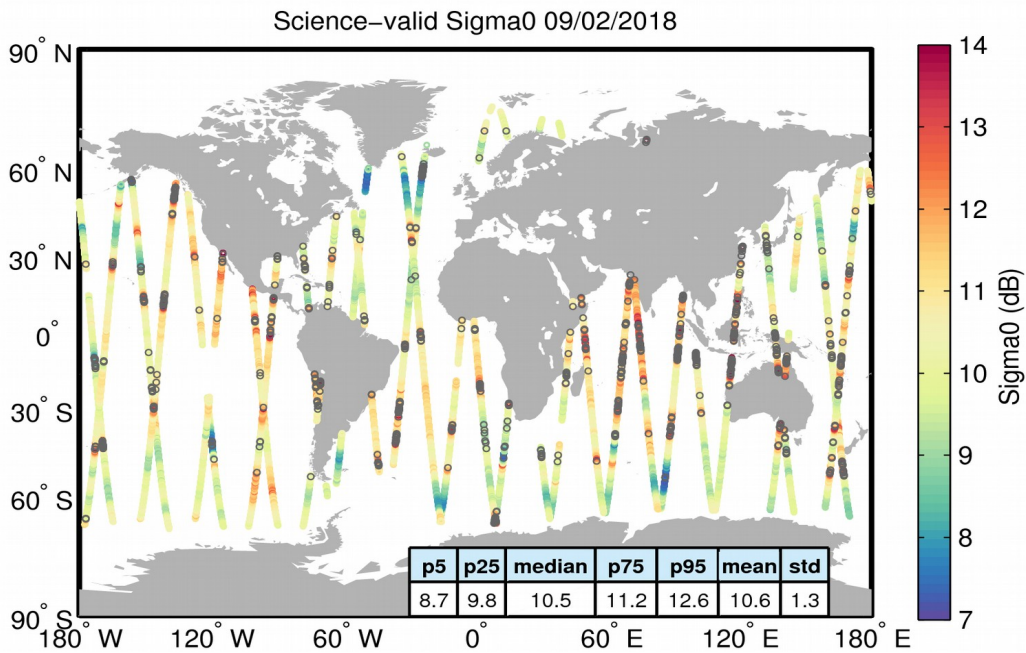
Figure 27. Geographical distribution of science-valid sigma0 data over oceans and lakes for 09/02/2018. The statistical values shown in the table refer to the sigma0 in dB and are calculated over all measurements shown in the figure. Gray circles denote records that have been rejected based on the editing criteria described in Table 4.
