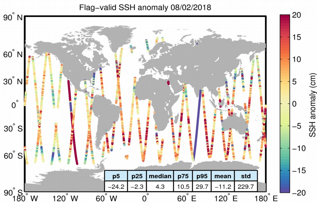
Figure 5. Geographical distribution of flag-valid 1-Hz SSH anomaly data over oceans and lakes for 08/02/2018. The statistical values shown in the table refer to the SSH anomaly in cm and are calculated over all measurements shown in the figure.
