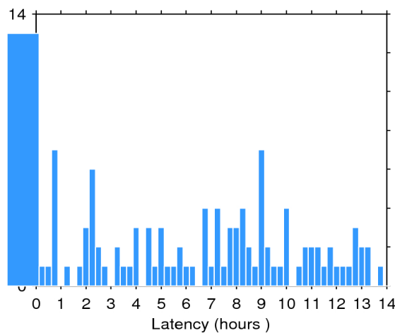
Figure 2. Histogram of the data latency for 08/02/2018. The y-axis denotes the number of files that are made available with a delay of x-hours with respect to the mean time of the records stored in the file.
