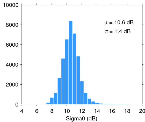
Figure 28. Histogram of science-valid sigma0 over oceans and lakes for 08/02/2018. The mean ( \mu ) and standard deviation ( \sigma ) are also shown. Note that values outside [4 20] dB are excluded from the histogram for the sake of readability but not from the computation of \mu and \sigma .
