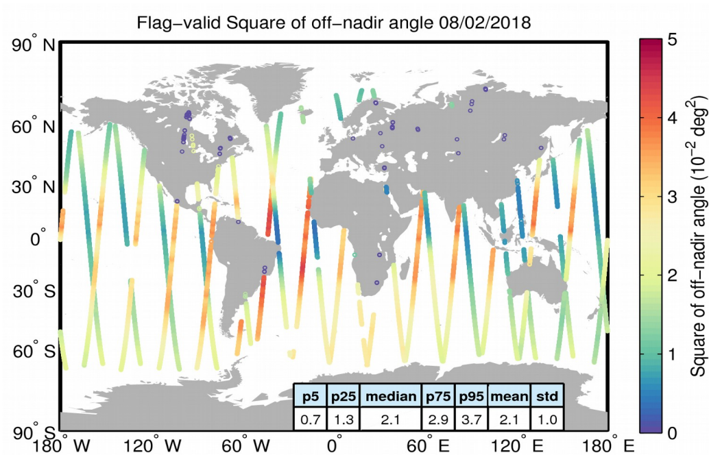
Figure 37. Geographical distribution of flag-valid mispointing data over oceans and lakes for 08/02/2018. The statistical values shown in the table refer to the mispointing in 10^{-2} deg 2 and are calculated over all measurements shown in the figure.
