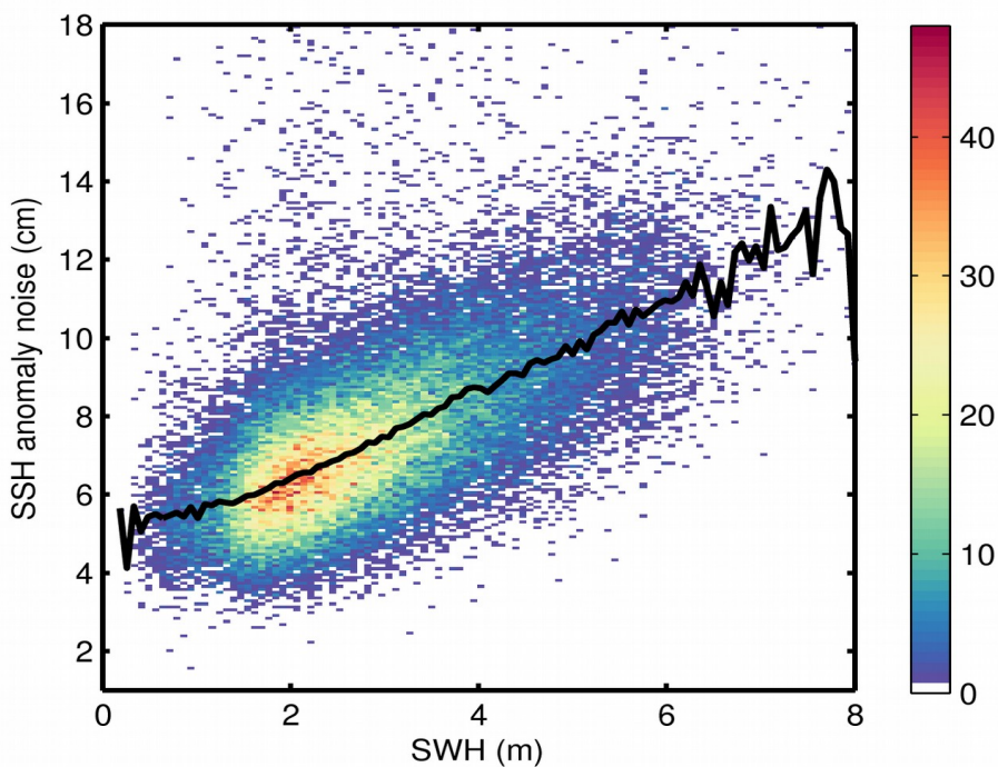
Figure 9. 2D histogram showing flag-valid SSH anomaly noise as a function of SWH for 08/02/2018. The black line denotes the median SSH anomaly noise as a function of SWH.
