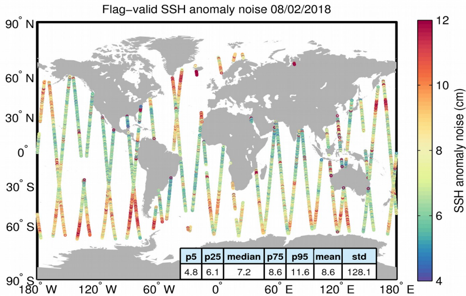
Figure 8. Geographical distribution of flag-valid 20-Hz SSH anomaly measurement noise over oceans and lakes for 08/02/2018. The statistical values shown in the table refer to the SSH anomaly noise and are calculated over all measurements shown in the figure.
