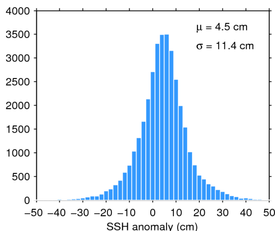
Figure 11. Histogram of science-valid SSH anomaly over oceans and lakes for 08/02/2018. The mean ( \mu ) and standard deviation ( \sigma ) are also shown. Note that values outside [-50 50] cm are excluded from the histogram for the sake of readability but not from the computation of \mu and \sigma .
