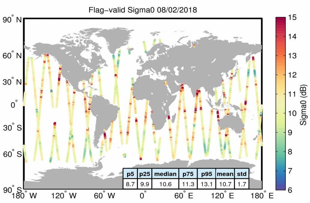
Figure 23. Geographical distribution of flag-valid sigma0 data over oceans and lakes for 08/02/2018. The statistical values shown in the table refer to the sigma0 in dB and are calculated over all measurements shown in the figure.
