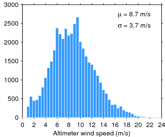
Figure 33. Histogram of flag-valid wind over oceans and lakes for 08/02/2018. The mean ( \mu ) and standard deviation ( \sigma ) are also shown. Note that values larger than 24 m/s are excluded from the histogram for the sake of readability but not from the computation of \mu and \sigma .
