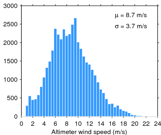
Figure 35. Histogram of science-valid wind over oceans and lakes for 08/02/2018. The mean ( \mu ) and standard deviation ( \sigma ) are also shown. Note that values larger than 24 m/s are excluded from the histogram for the sake of readability but not from the computation of \mu and \sigma .
