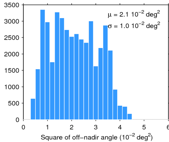
Figure 39. Histogram of flag-valid mispointing over oceans and lakes for 08/02/2018. The mean ( \mu ) and standard deviation ( \sigma ) are also shown. Note that values larger than 6 \cdot 10^{-2} \text{ deg}^2 are excluded from the histogram for the sake of readability but not from the computation of \mu and \sigma .
