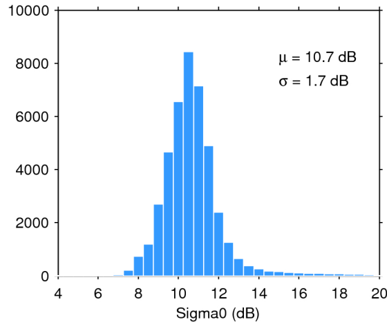
Figure 25. Histogram of flag-valid sigma0 over oceans and lakes for 08/02/2018. The mean ( \mu ) and standard deviation ( \sigma ) are also shown. Note that values outside [4 20] dB are excluded from the histogram for the sake of readability but not from the computation of \mu and \sigma .
