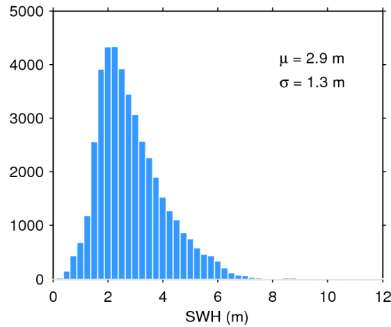
Figure 17. Histogram of flag-valid SWH over oceans and lakes for 08/02/2018. The mean ( \mu ) and standard deviation ( \sigma ) are also shown. Note that values larger than 12 m are excluded from the histogram for the sake of readability but not from the computation of \mu and \sigma .
