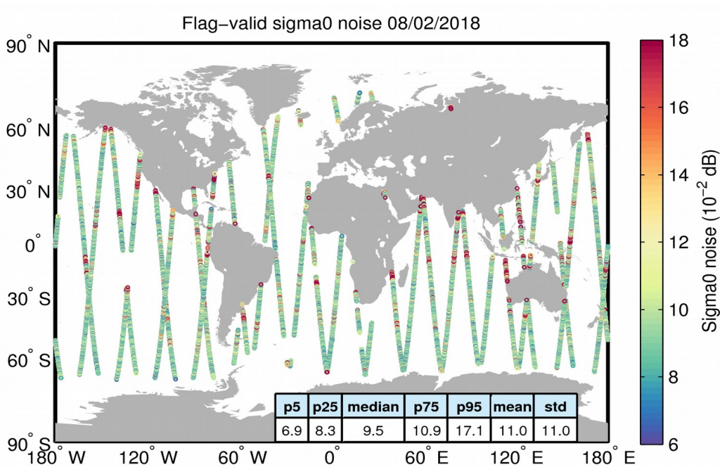
Figure 26. Geographical distribution of flag-valid 20-Hz sigma0 measurement noise over oceans and lakes for 08/02/2018. The statistical values shown in the table refer to the sigma0 noise and are calculated over all measurements shown in the figure.
