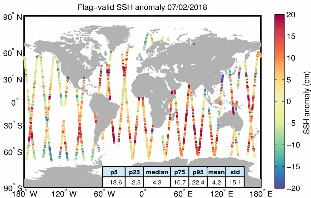
Figure 5. Geographical distribution of flag-valid 1-Hz SSH anomaly data over oceans and lakes for 07/02/2018. The statistical values shown in the table refer to the SSH anomaly in cm and are calculated over all measurements shown in the figure.
