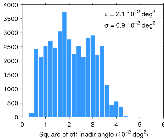
Figure 39. Histogram of flag-valid mispointing over oceans and lakes for 07/02/2018. The mean ( \mu ) and standard deviation ( \sigma ) are also shown. Note that values larger than 6 \cdot 10^{-2} \text{ deg}^2 are excluded from the histogram for the sake of readability but not from the computation of \mu and \sigma .
