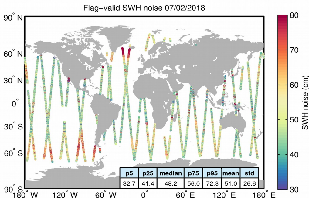
Figure 18. Geographical distribution of flag-valid 20-Hz SWH measurement noise over oceans and lakes for 07/02/2018. The statistical values shown in the figure refer to the SWH noise and are calculated over all measurements shown in the figure.
