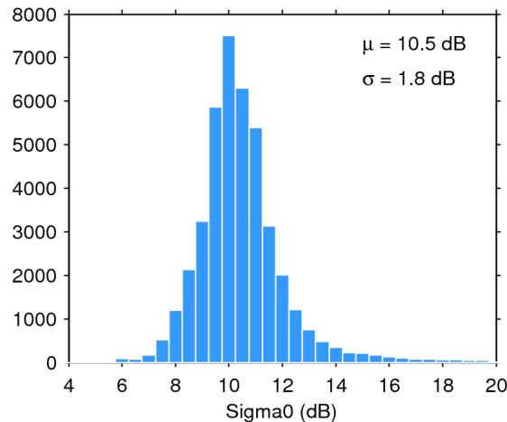
Figure 25. Histogram of flag-valid sigma0 over oceans and lakes for 07/02/2018. The mean ( \mu ) and standard deviation ( \sigma ) are also shown. Note that values outside [4 20] dB are excluded from the histogram for the sake of readability but not from the computation of \mu and \sigma .
