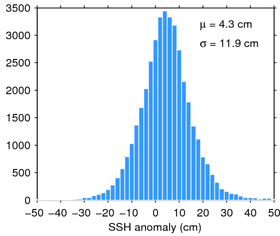
Figure 11. Histogram of science-valid SSH anomaly over oceans and lakes for 07/02/2018. The mean ( \mu ) and standard deviation ( \sigma ) are also shown. Note that values outside [-50 50] cm are excluded from the histogram for the sake of readability but not from the computation of \mu and \sigma .
