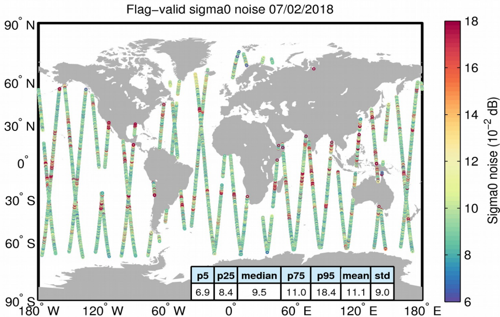
Figure 26. Geographical distribution of flag-valid 20-Hz sigma0 measurement noise over oceans and lakes for 07/02/2018. The statistical values shown in the table refer to the sigma0 noise and are calculated over all measurements shown in the figure.
