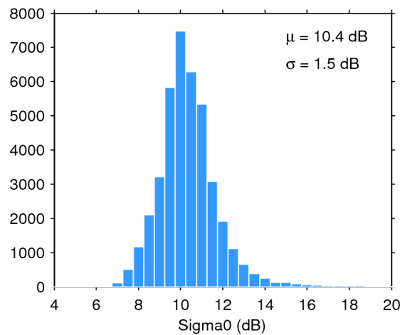
Figure 28. Histogram of science-valid sigma0 over oceans and lakes for 07/02/2018. The mean ( \mu ) and standard deviation ( \sigma ) are also shown. Note that values outside [4 20] dB are excluded from the histogram for the sake of readability but not from the computation of \mu and \sigma .
