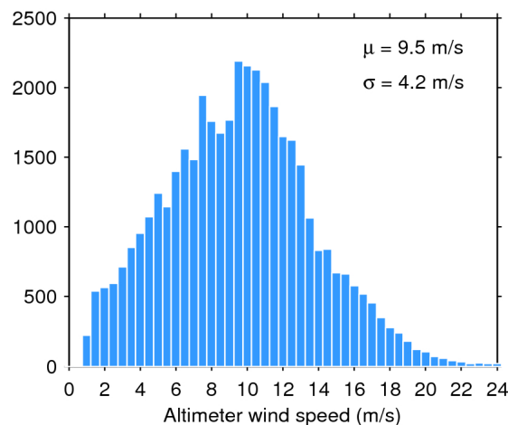
Figure 35. Histogram of science-valid wind over oceans and lakes for 07/02/2018. The mean ( \mu ) and standard deviation ( \sigma ) are also shown. Note that values larger than 24 m/s are excluded from the histogram for the sake of readability but not from the computation of \mu and \sigma .
