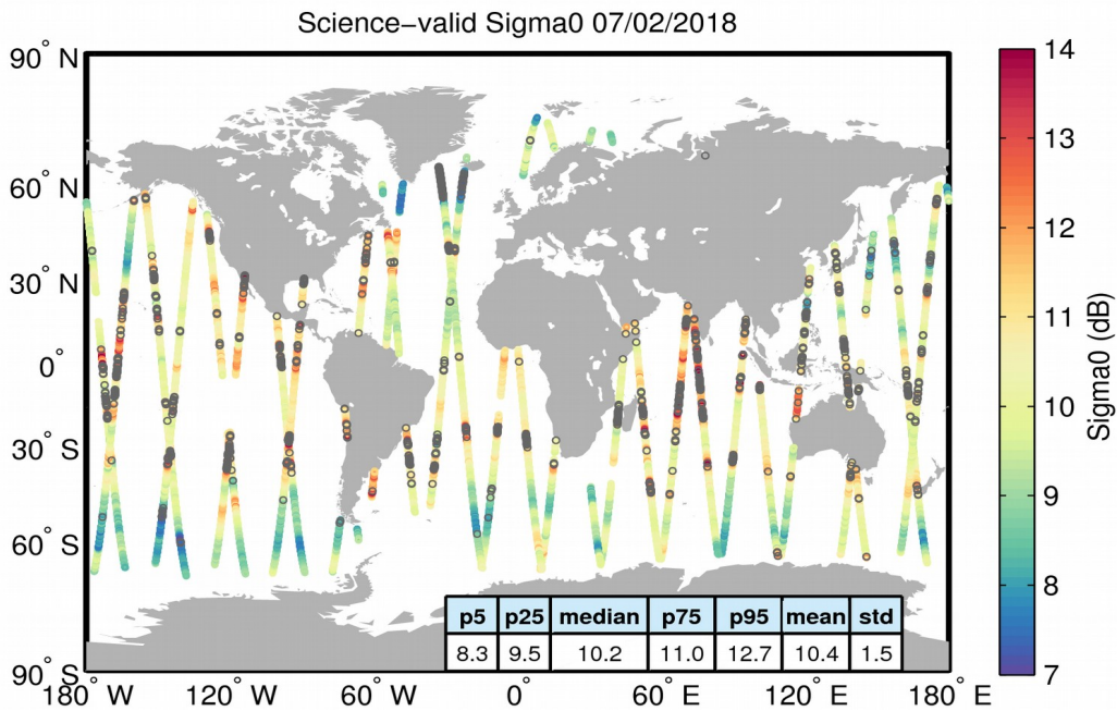
Figure 27. Geographical distribution of science-valid sigma0 data over oceans and lakes for 07/02/2018. The statistical values shown in the table refer to the sigma0 in dB and are calculated over all measurements shown in the figure. Gray circles denote records that have been rejected based on the editing criteria described in Table 4.
