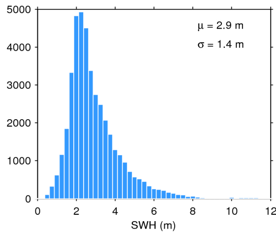
Figure 17. Histogram of flag-valid SWH over oceans and lakes for 07/02/2018. The mean ( \mu ) and standard deviation ( \sigma ) are also shown. Note that values larger than 12 m are excluded from the histogram for the sake of readability but not from the computation of \mu and \sigma .
