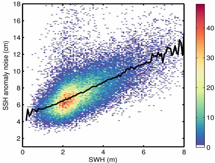
Figure 9. 2D histogram showing flag-valid SSH anomaly noise as a function of SWH for 07/02/2018. The black line denotes the median SSH anomaly noise as a function of SWH.
