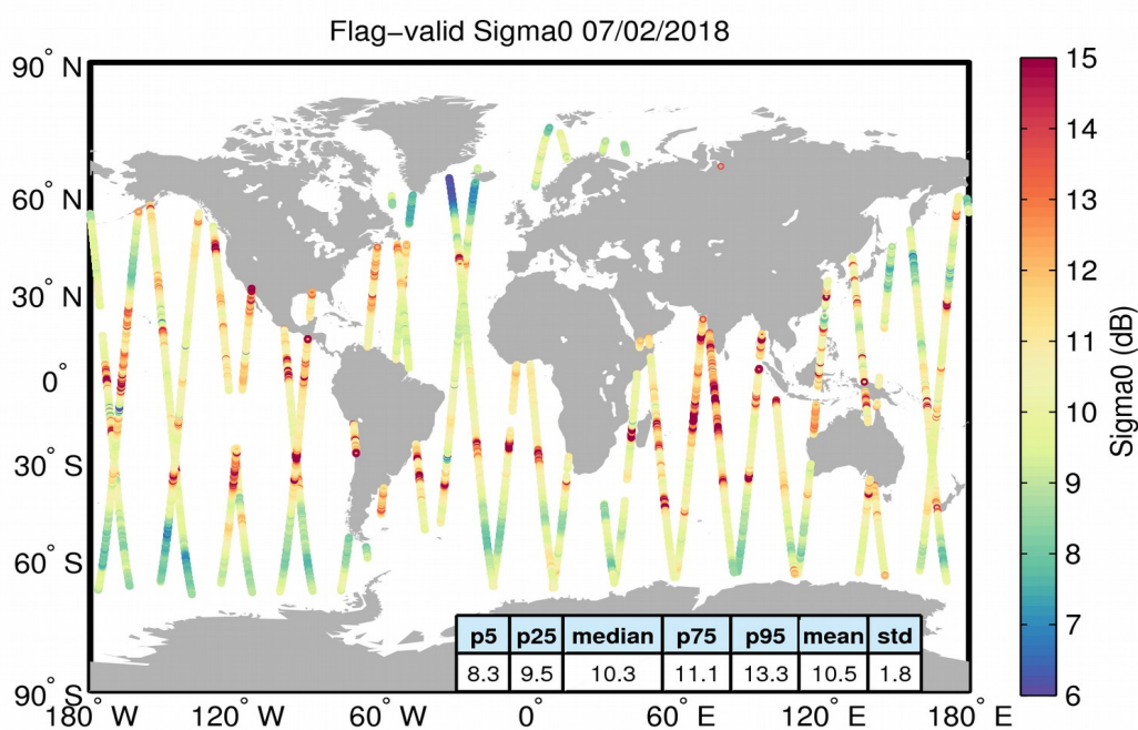
Figure 23. Geographical distribution of flag-valid sigma0 data over oceans and lakes for 07/02/2018. The statistical values shown in the table refer to the sigma0 in dB and are calculated over all measurements shown in the figure.
