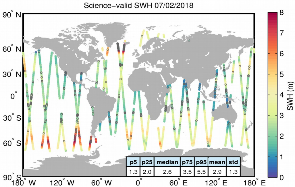
Figure 19. Geographical distribution of science-valid SWH data over oceans and lakes for 07/02/2018. The statistical values shown in the table refer to the SWH in m and are calculated over all measurements shown in the figure. Gray circles denote records that have been rejected based on the editing criteria described in Table 3.
