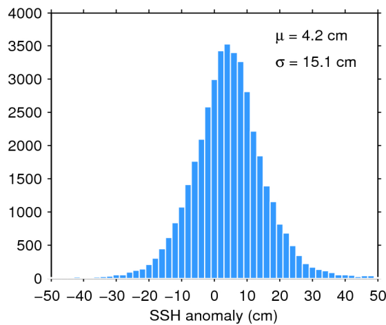
Figure 7. Histogram of flag-valid SSH anomaly over oceans and lakes for 07/02/2018. The mean ( \mu ) and standard deviation ( \sigma ) are also shown. Note that values outside [-50 50] cm are excluded from the histogram for the sake of readability but not from the computation of \mu and \sigma .
