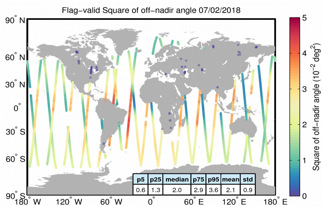
Figure 37. Geographical distribution of flag-valid mispointing data over oceans and lakes for 07/02/2018. The statistical values shown in the table refer to the mispointing in 10^{-2} \text{ deg}^2 and are calculated over all measurements shown in the figure.
