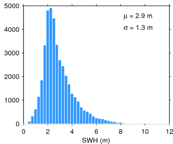
Figure 20. Histogram of science-valid SWH over oceans and lakes for 07/02/2018. The mean ( \mu ) and standard deviation ( \sigma ) are also shown. Note that values larger than 12 m are excluded from the histogram for the sake of readability but not from the computation of \mu and \sigma .
