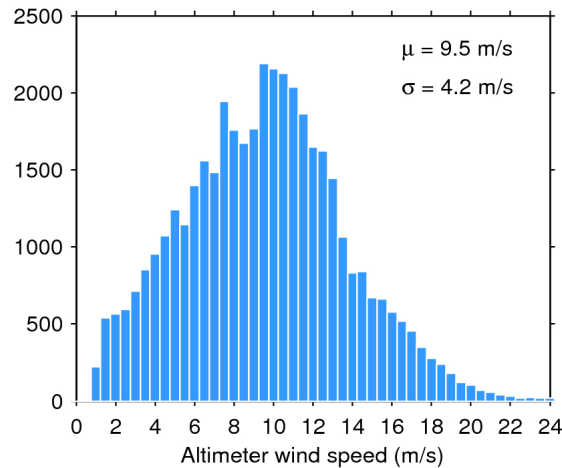
Figure 33. Histogram of flag-valid wind over oceans and lakes for 07/02/2018. The mean ( \mu ) and standard deviation ( \sigma ) are also shown. Note that values larger than 24 m/s are excluded from the histogram for the sake of readability but not from the computation of \mu and \sigma .
