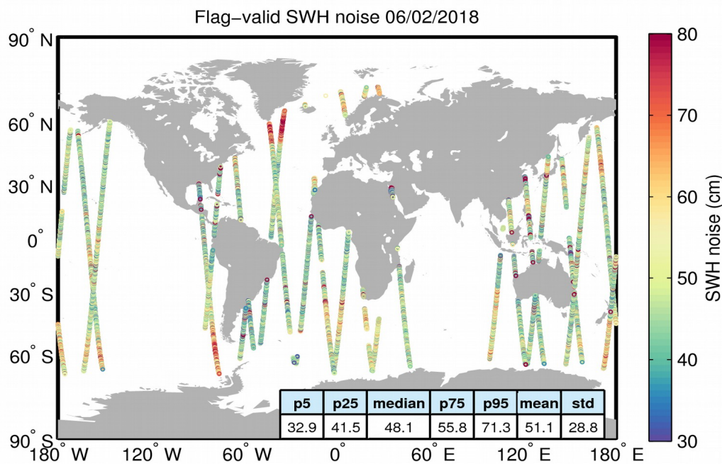
Figure 18. Geographical distribution of flag-valid 20-Hz SWH measurement noise over oceans and lakes for 06/02/2018. The statistical values shown in the figure refer to the SWH noise and are calculated over all measurements shown in the figure.
