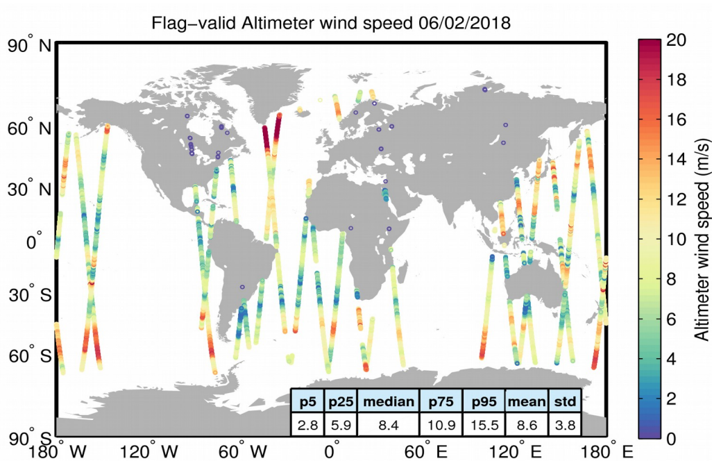
Figure 31. Geographical distribution of flag-valid wind data over oceans and lakes for 06/02/2018. The statistical values shown in the table refer to the wind in m/s and are calculated over all measurements shown in the figure.
