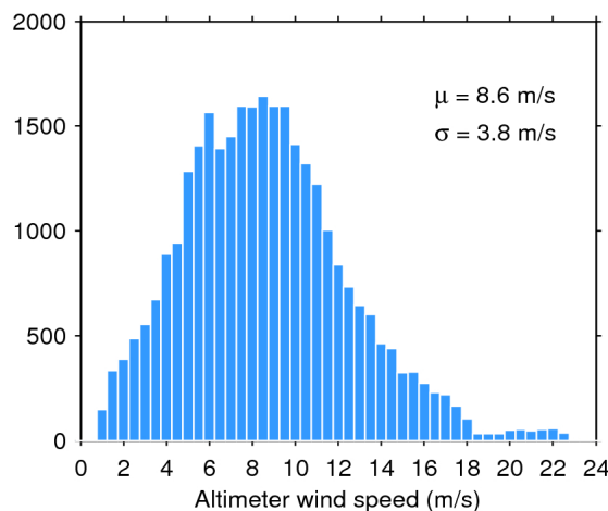
Figure 35. Histogram of science-valid wind over oceans and lakes for 06/02/2018. The mean ( \mu ) and standard deviation ( \sigma ) are also shown. Note that values larger than 24 m/s are excluded from the histogram for the sake of readability but not from the computation of \mu and \sigma .
