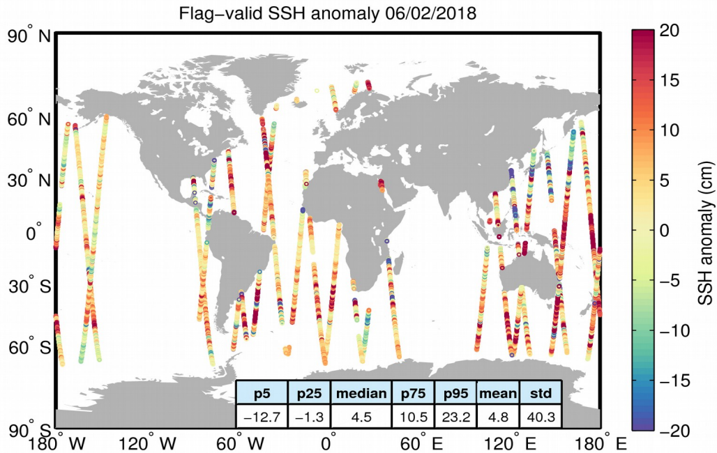
Figure 5. Geographical distribution of flag-valid 1-Hz SSH anomaly data over oceans and lakes for 06/02/2018. The statistical values shown in the table refer to the SSH anomaly in cm and are calculated over all measurements shown in the figure.
