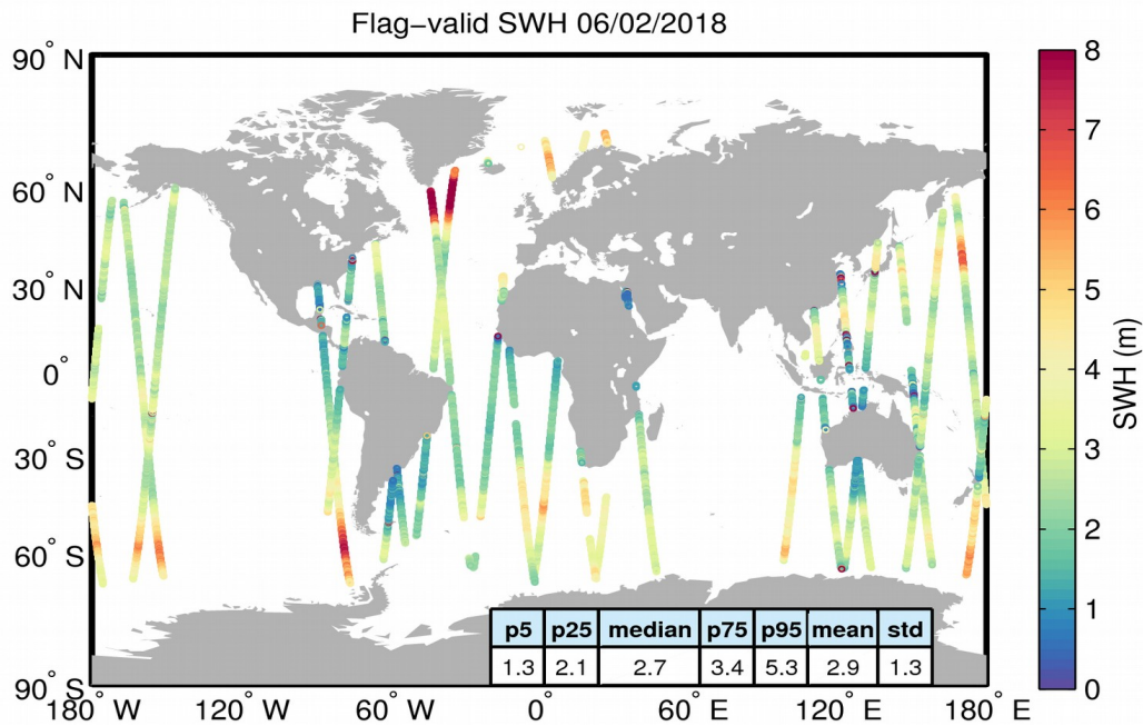
Figure 15. Geographical distribution of flag-valid SWH data over oceans and lakes for 06/02/2018. The statistical values shown in the table refer to the SWH in m and are calculated over all measurements shown in the figure.
