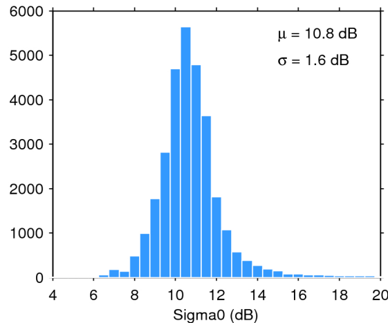
Figure 25. Histogram of flag-valid sigma0 over oceans and lakes for 06/02/2018. The mean ( \mu ) and standard deviation ( \sigma ) are also shown. Note that values outside [4 20] dB are excluded from the histogram for the sake of readability but not from the computation of \mu and \sigma .
