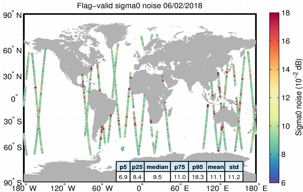
Figure 26. Geographical distribution of flag-valid 20-Hz sigma0 measurement noise over oceans and lakes for 06/02/2018. The statistical values shown in the table refer to the sigma0 noise and are calculated over all measurements shown in the figure.
