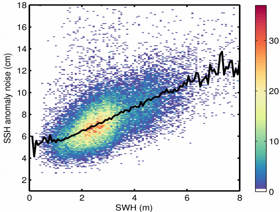
Figure 9. 2D histogram showing flag-valid SSH anomaly noise as a function of SWH for 06/02/2018. The black line denotes the median SSH anomaly noise as a function of SWH.
