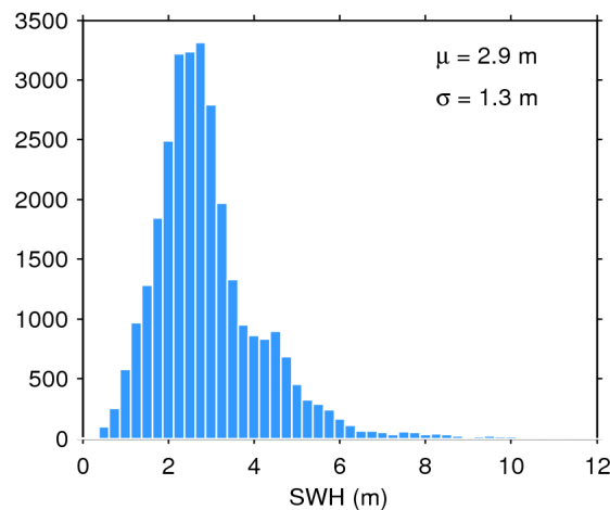
Figure 20. Histogram of science-valid SWH over oceans and lakes for 06/02/2018. The mean ( \mu ) and standard deviation ( \sigma ) are also shown. Note that values larger than 12 m are excluded from the histogram for the sake of readability but not from the computation of \mu and \sigma .
