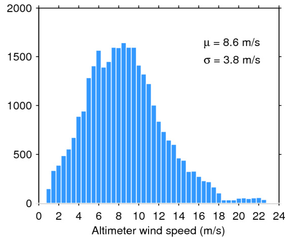
Figure 33. Histogram of flag-valid wind over oceans and lakes for 06/02/2018. The mean ( \mu ) and standard deviation ( \sigma ) are also shown. Note that values larger than 24 m/s are excluded from the histogram for the sake of readability but not from the computation of \mu and \sigma .
