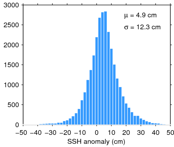
Figure 11. Histogram of science-valid SSH anomaly over oceans and lakes for 06/02/2018. The mean ( \mu ) and standard deviation ( \sigma ) are also shown. Note that values outside [-50 50] cm are excluded from the histogram for the sake of readability but not from the computation of \mu and \sigma .
