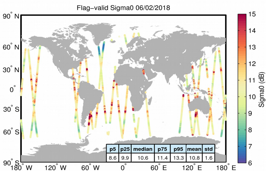
Figure 23. Geographical distribution of flag-valid sigma0 data over oceans and lakes for 06/02/2018. The statistical values shown in the table refer to the sigma0 in dB and are calculated over all measurements shown in the figure.
