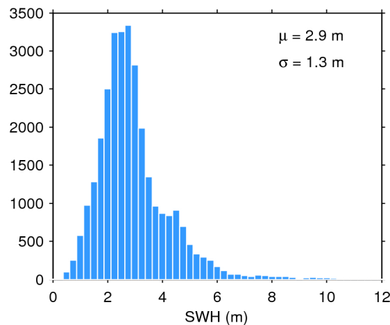
Figure 17. Histogram of flag-valid SWH over oceans and lakes for 06/02/2018. The mean ( \mu ) and standard deviation ( \sigma ) are also shown. Note that values larger than 12 m are excluded from the histogram for the sake of readability but not from the computation of \mu and \sigma .
