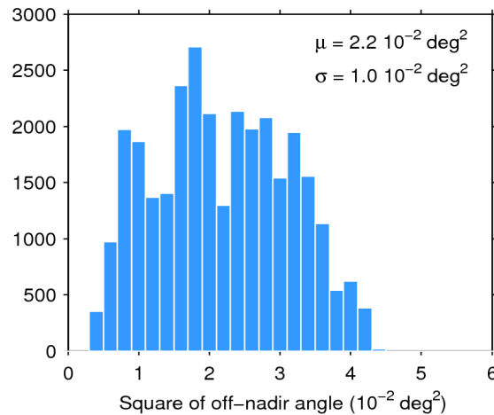
Figure 39. Histogram of flag-valid mispointing over oceans and lakes for 06/02/2018. The mean ( \mu ) and standard deviation ( \sigma ) are also shown. Note that values larger than 6 \cdot 10^{-2} \text{ deg}^2 are excluded from the histogram for the sake of readability but not from the computation of \mu and \sigma .
