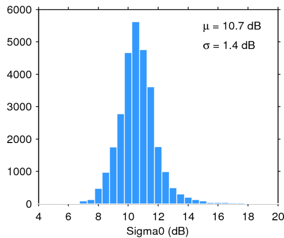
Figure 28. Histogram of science-valid sigma0 over oceans and lakes for 06/02/2018. The mean ( \mu ) and standard deviation ( \sigma ) are also shown. Note that values outside [4 20] dB are excluded from the histogram for the sake of readability but not from the computation of \mu and \sigma .
