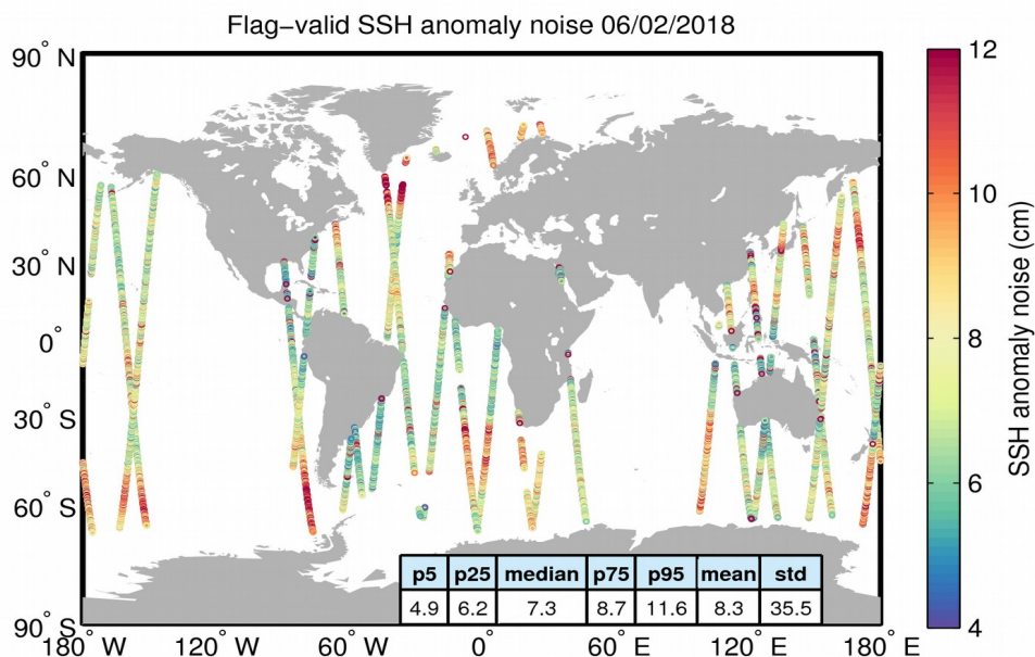
Figure 8. Geographical distribution of flag-valid 20-Hz SSH anomaly measurement noise over oceans and lakes for 06/02/2018. The statistical values shown in the table refer to the SSH anomaly noise and are calculated over all measurements shown in the figure.
