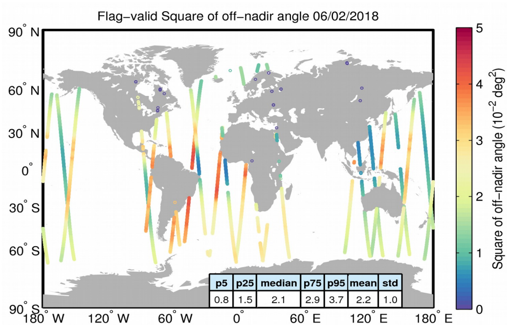
Figure 37. Geographical distribution of flag-valid mispointing data over oceans and lakes for 06/02/2018. The statistical values shown in the table refer to the mispointing in 10^{-2} deg 2 and are calculated over all measurements shown in the figure.
