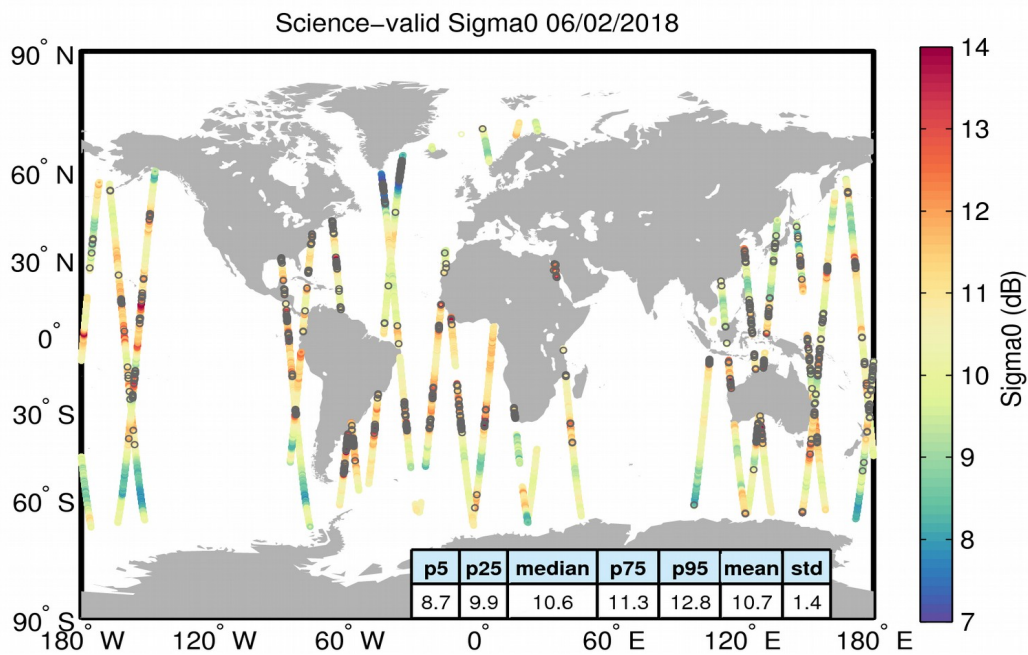
Figure 27. Geographical distribution of science-valid sigma0 data over oceans and lakes for 06/02/2018. The statistical values shown in the table refer to the sigma0 in dB and are calculated over all measurements shown in the figure. Gray circles denote records that have been rejected based on the editing criteria described in Table 4.
