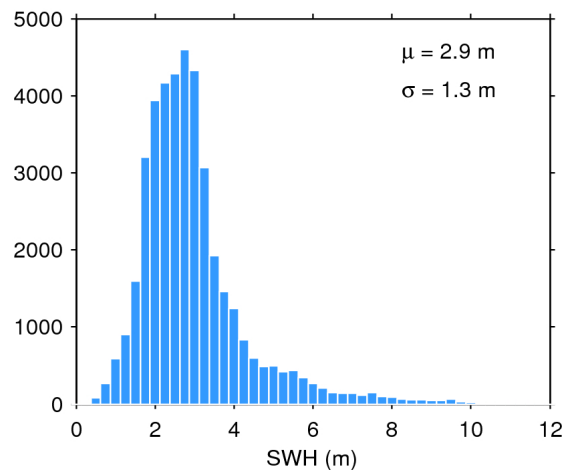
Figure 20. Histogram of science-valid SWH over oceans and lakes for 05/02/2018. The mean ( \mu ) and standard deviation ( \sigma ) are also shown. Note that values larger than 12 m are excluded from the histogram for the sake of readability but not from the computation of \mu and \sigma .
