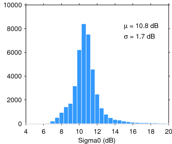
Figure 25. Histogram of flag-valid sigma0 over oceans and lakes for 05/02/2018. The mean ( \mu ) and standard deviation ( \sigma ) are also shown. Note that values outside [4 20] dB are excluded from the histogram for the sake of readability but not from the computation of \mu and \sigma .
