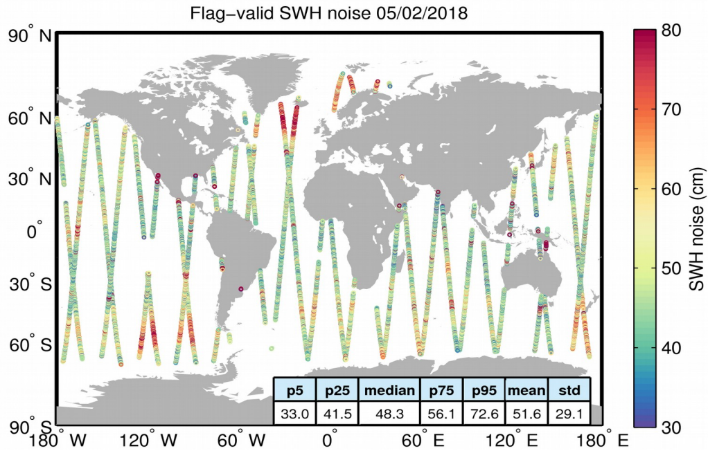
Figure 18. Geographical distribution of flag-valid 20-Hz SWH measurement noise over oceans and lakes for 05/02/2018. The statistical values shown in the figure refer to the SWH noise and are calculated over all measurements shown in the figure.
