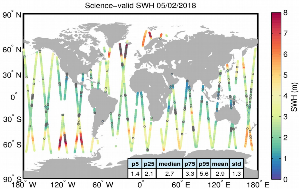
Figure 19. Geographical distribution of science-valid SWH data over oceans and lakes for 05/02/2018. The statistical values shown in the table refer to the SWH in m and are calculated over all measurements shown in the figure. Gray circles denote records that have been rejected based on the editing criteria described in Table 3.
