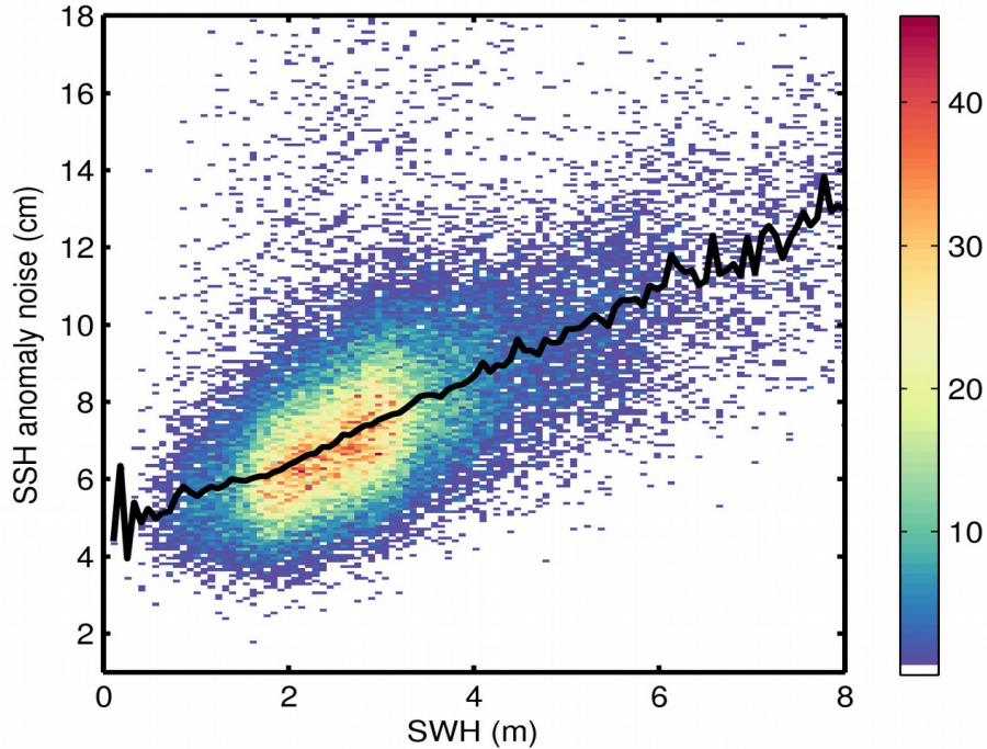
Figure 9. 2D histogram showing flag-valid SSH anomaly noise as a function of SWH for 05/02/2018. The black line denotes the median SSH anomaly noise as a function of SWH.
