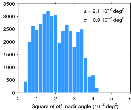
Figure 39. Histogram of flag-valid mispointing over oceans and lakes for 05/02/2018. The mean ( \mu ) and standard deviation ( \sigma ) are also shown. Note that values larger than 6 \cdot 10^{-2} \text{ deg}^2 are excluded from the histogram for the sake of readability but not from the computation of \mu and \sigma .
