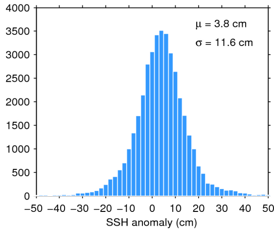
Figure 11. Histogram of science-valid SSH anomaly over oceans and lakes for 05/02/2018. The mean ( \mu ) and standard deviation ( \sigma ) are also shown. Note that values outside [-50 50] cm are excluded from the histogram for the sake of readability but not from the computation of \mu and \sigma .
