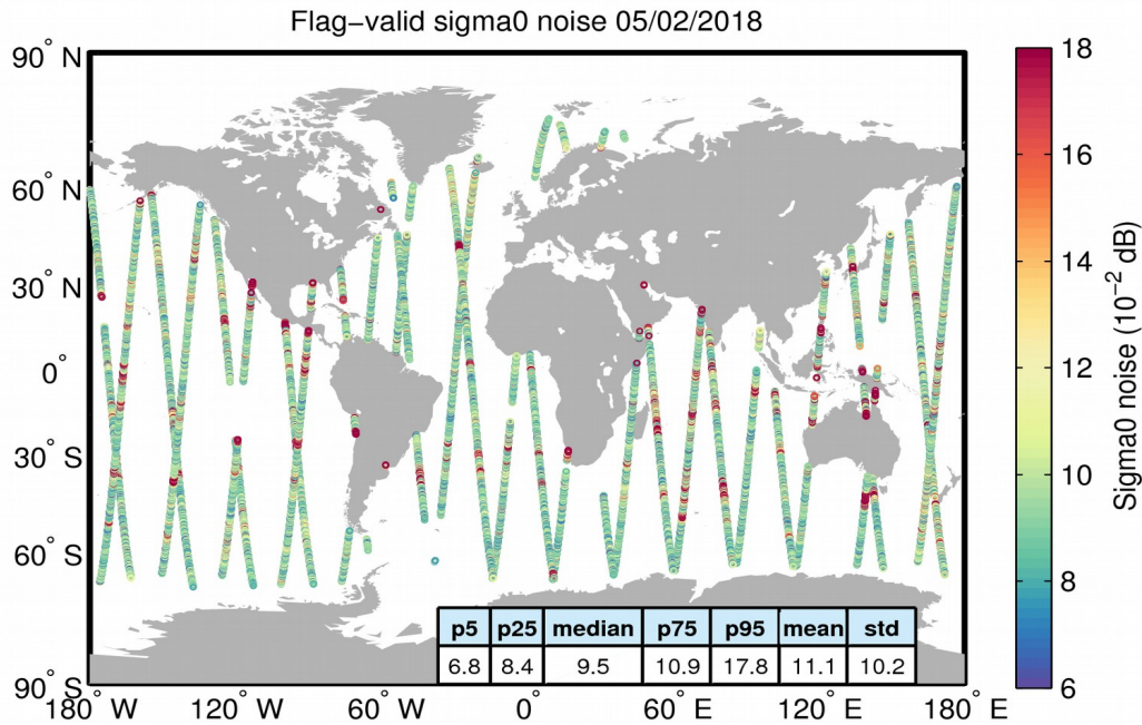
Figure 26. Geographical distribution of flag-valid 20-Hz sigma0 measurement noise over oceans and lakes for 05/02/2018. The statistical values shown in the table refer to the sigma0 noise and are calculated over all measurements shown in the figure.
