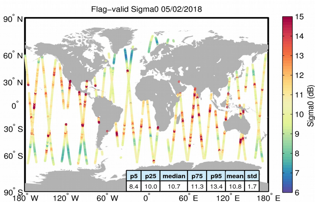
Figure 23. Geographical distribution of flag-valid sigma0 data over oceans and lakes for 05/02/2018. The statistical values shown in the table refer to the sigma0 in dB and are calculated over all measurements shown in the figure.
