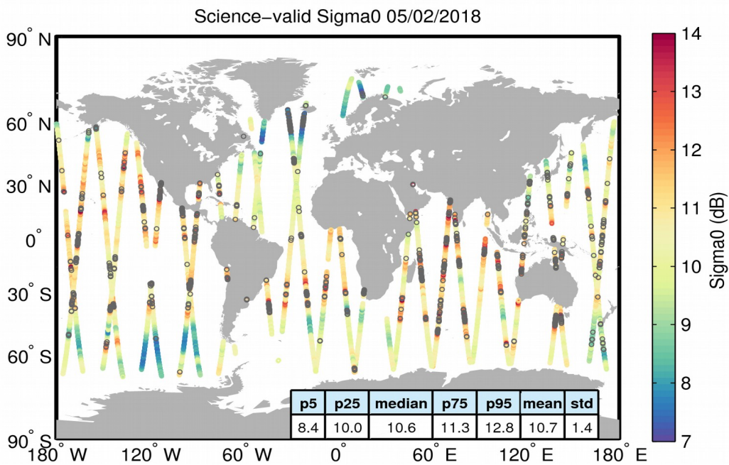
Figure 27. Geographical distribution of science-valid sigma0 data over oceans and lakes for 05/02/2018. The statistical values shown in the table refer to the sigma0 in dB and are calculated over all measurements shown in the figure. Gray circles denote records that have been rejected based on the editing criteria described in Table 4.
