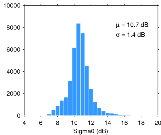
Figure 28. Histogram of science-valid sigma0 over oceans and lakes for 05/02/2018. The mean ( \mu ) and standard deviation ( \sigma ) are also shown. Note that values outside [4 20] dB are excluded from the histogram for the sake of readability but not from the computation of \mu and \sigma .
