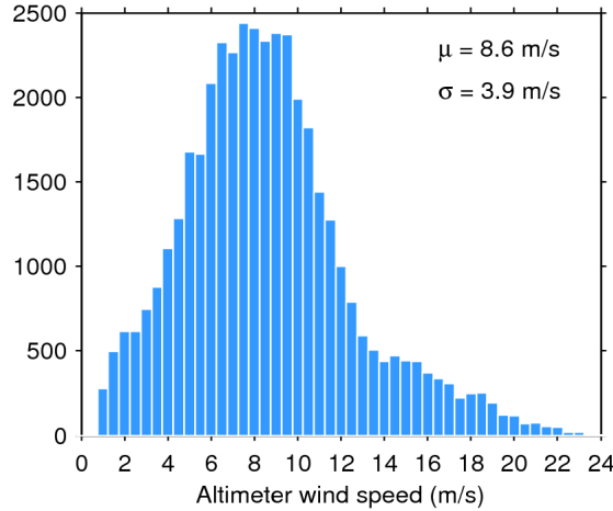
Figure 33. Histogram of flag-valid wind over oceans and lakes for 05/02/2018. The mean ( \mu ) and standard deviation ( \sigma ) are also shown. Note that values larger than 24 m/s are excluded from the histogram for the sake of readability but not from the computation of \mu and \sigma .
