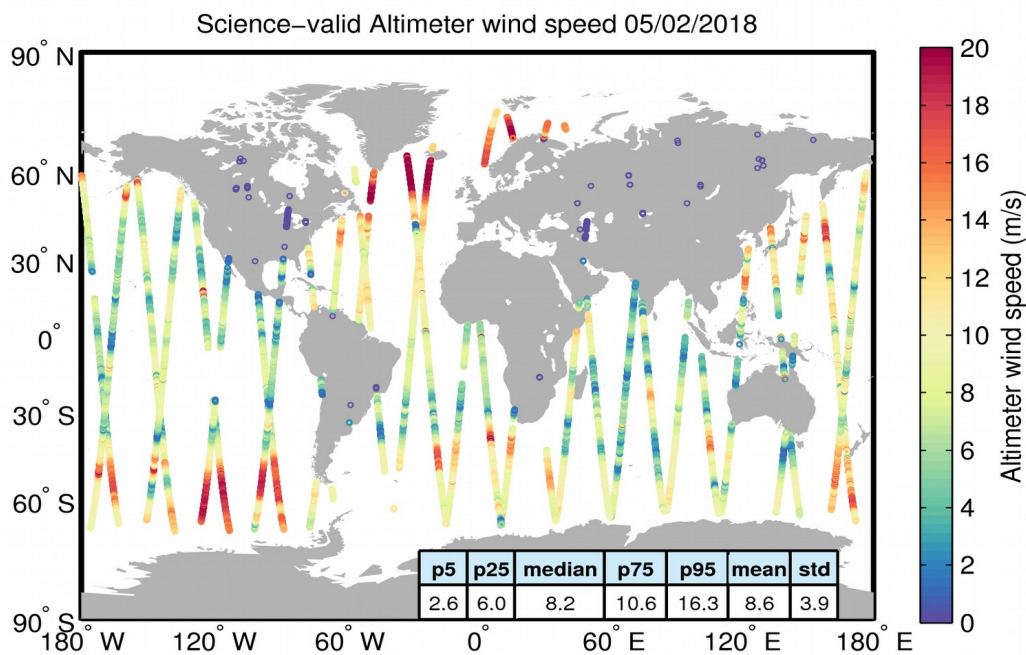
Figure 34. Geographical distribution of science-valid wind data over oceans and lakes for 05/02/2018. The statistical values shown in the table refer to the wind in m/s and are calculated over all measurements shown in the figure. Gray circles denote records that have been rejected based on the editing criteria described in Table 5.
