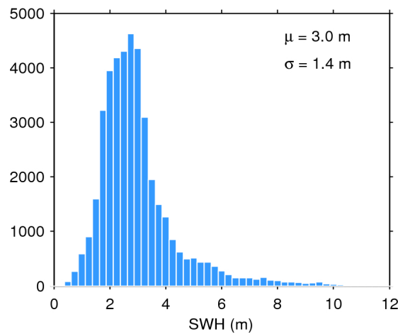
Figure 17. Histogram of flag-valid SWH over oceans and lakes for 05/02/2018. The mean ( \mu ) and standard deviation ( \sigma ) are also shown. Note that values larger than 12 m are excluded from the histogram for the sake of readability but not from the computation of \mu and \sigma .
