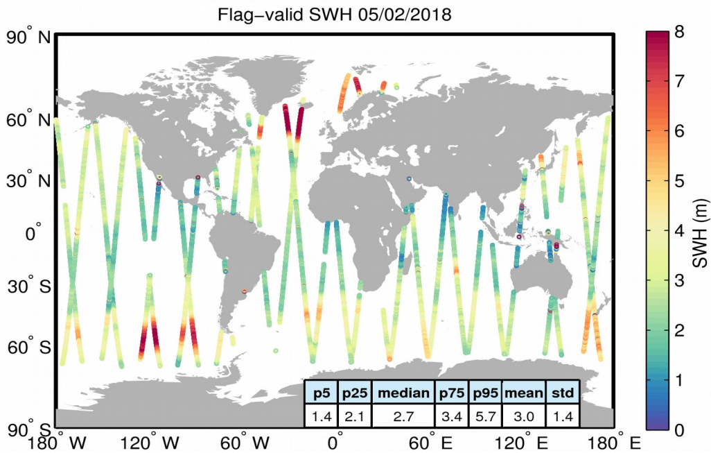
Figure 15. Geographical distribution of flag-valid SWH data over oceans and lakes for 05/02/2018. The statistical values shown in the table refer to the SWH in m and are calculated over all measurements shown in the figure.
