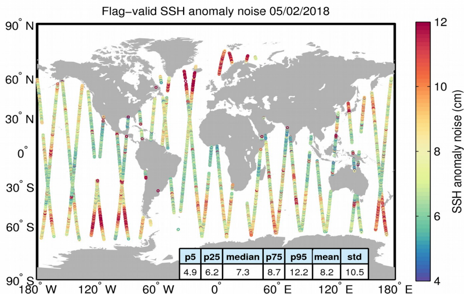
Figure 8. Geographical distribution of flag-valid 20-Hz SSH anomaly measurement noise over oceans and lakes for 05/02/2018. The statistical values shown in the table refer to the SSH anomaly noise and are calculated over all measurements shown in the figure.
