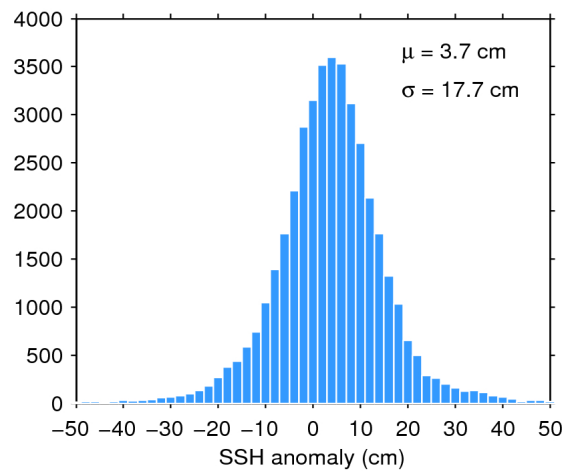
Figure 7. Histogram of flag-valid SSH anomaly over oceans and lakes for 05/02/2018. The mean ( \mu ) and standard deviation ( \sigma ) are also shown. Note that values outside [-50\ 50] cm are excluded from the histogram for the sake of readability but not from the computation of \mu and \sigma .
