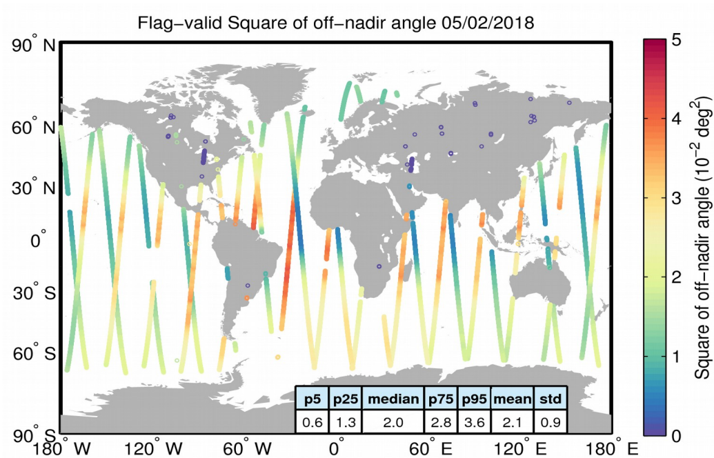
Figure 37. Geographical distribution of flag-valid mispointing data over oceans and lakes for 05/02/2018. The statistical values shown in the table refer to the mispointing in 10^{-2} \text{ deg}^2 and are calculated over all measurements shown in the figure.
