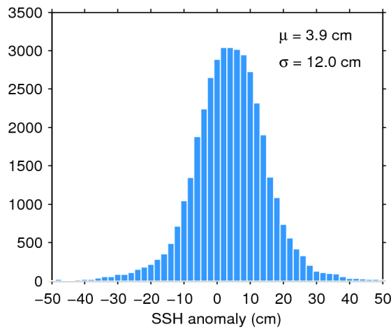
Figure 11. Histogram of science-valid SSH anomaly over oceans and lakes for 03/02/2018. The mean ( \mu ) and standard deviation ( \sigma ) are also shown. Note that values outside [-50 50] cm are excluded from the histogram for the sake of readability but not from the computation of \mu and \sigma .
