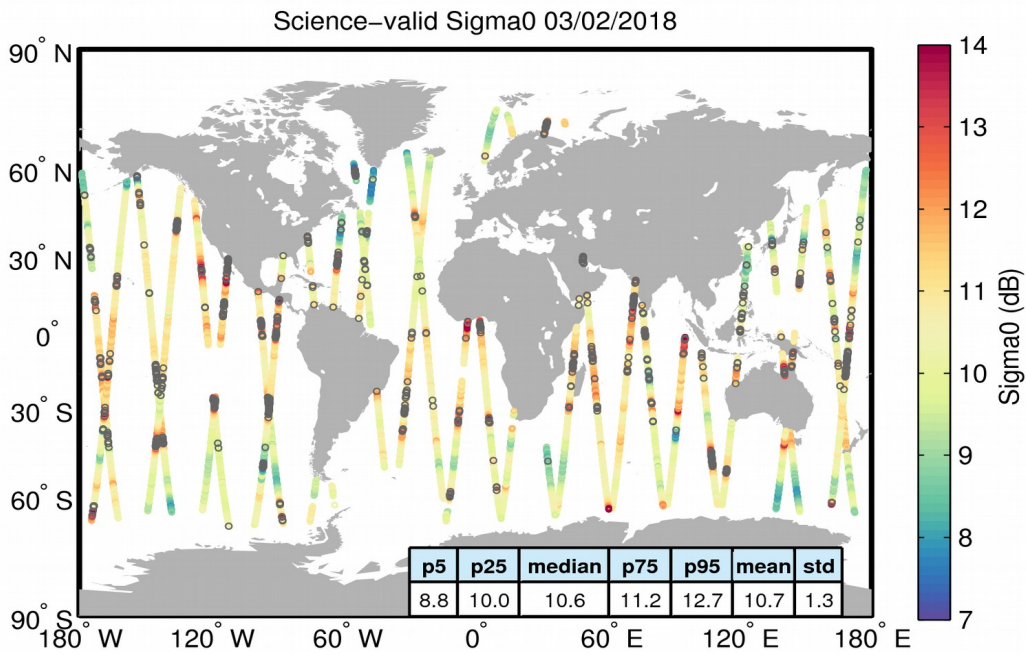
Figure 27. Geographical distribution of science-valid sigma0 data over oceans and lakes for 03/02/2018. The statistical values shown in the table refer to the sigma0 in dB and are calculated over all measurements shown in the figure. Gray circles denote records that have been rejected based on the editing criteria described in Table 4.
