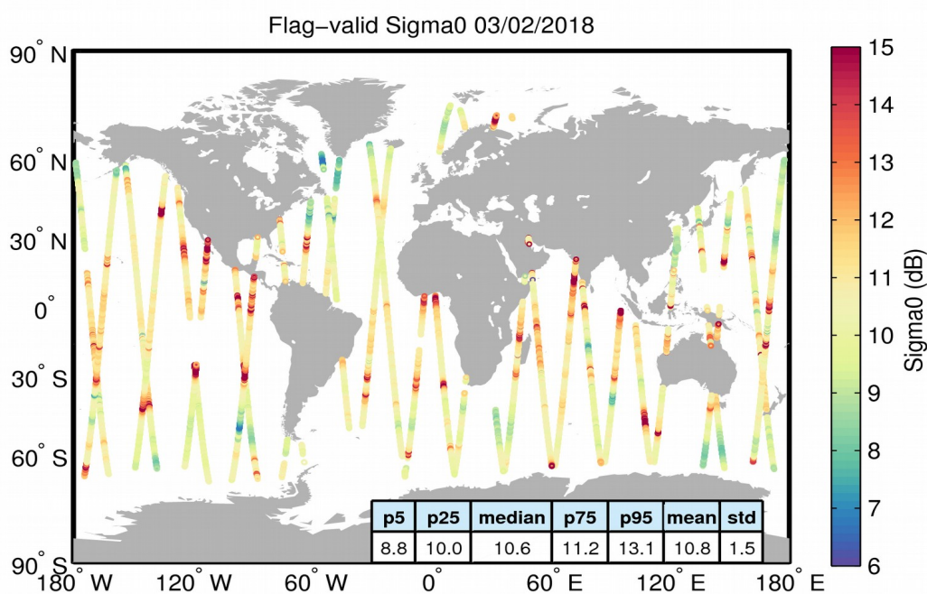
Figure 23. Geographical distribution of flag-valid sigma0 data over oceans and lakes for 03/02/2018. The statistical values shown in the table refer to the sigma0 in dB and are calculated over all measurements shown in the figure.
