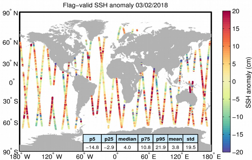
Figure 5. Geographical distribution of flag-valid 1-Hz SSH anomaly data over oceans and lakes for 03/02/2018. The statistical values shown in the table refer to the SSH anomaly in cm and are calculated over all measurements shown in the figure.
