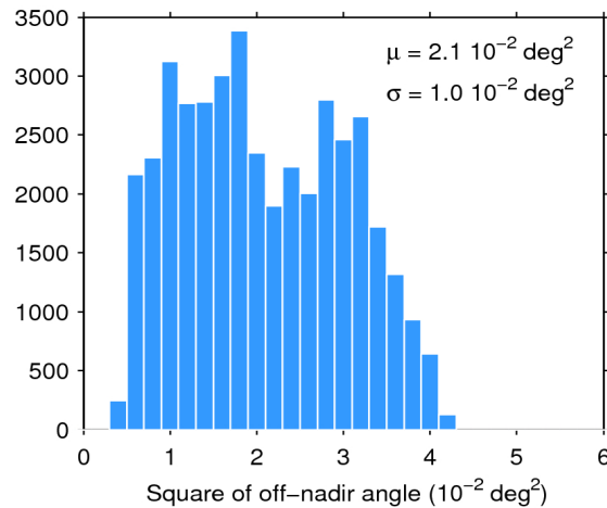
Figure 39. Histogram of flag-valid mispointing over oceans and lakes for 03/02/2018. The mean ( \mu ) and standard deviation ( \sigma ) are also shown. Note that values larger than 6 \cdot 10^{-2} \text{ deg}^2 are excluded from the histogram for the sake of readability but not from the computation of \mu and \sigma .
