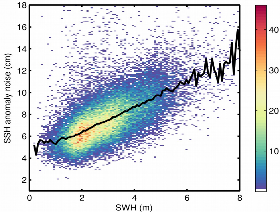
Figure 9. 2D histogram showing flag-valid SSH anomaly noise as a function of SWH for 03/02/2018. The black line denotes the median SSH anomaly noise as a function of SWH.
