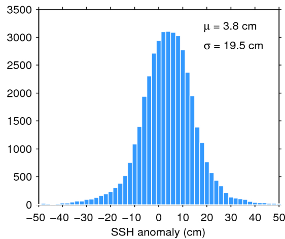
Figure 7. Histogram of flag-valid SSH anomaly over oceans and lakes for 03/02/2018. The mean ( \mu ) and standard deviation ( \sigma ) are also shown. Note that values outside [-50\ 50] cm are excluded from the histogram for the sake of readability but not from the computation of \mu and \sigma .
