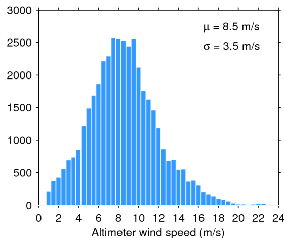
Figure 35. Histogram of science-valid wind over oceans and lakes for 03/02/2018. The mean ( \mu ) and standard deviation ( \sigma ) are also shown. Note that values larger than 24 m/s are excluded from the histogram for the sake of readability but not from the computation of \mu and \sigma .
