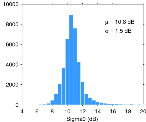
Figure 25. Histogram of flag-valid sigma0 over oceans and lakes for 03/02/2018. The mean ( \mu ) and standard deviation ( \sigma ) are also shown. Note that values outside [4 20] dB are excluded from the histogram for the sake of readability but not from the computation of \mu and \sigma .
