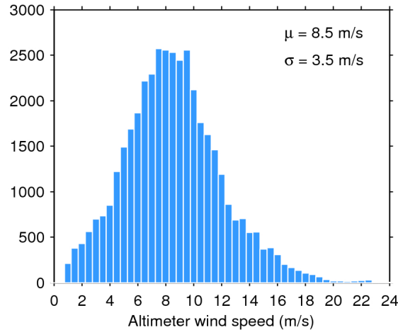
Figure 33. Histogram of flag-valid wind over oceans and lakes for 03/02/2018. The mean ( \mu ) and standard deviation ( \sigma ) are also shown. Note that values larger than 24 m/s are excluded from the histogram for the sake of readability but not from the computation of \mu and \sigma .
