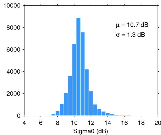
Figure 28. Histogram of science-valid sigma0 over oceans and lakes for 03/02/2018. The mean ( \mu ) and standard deviation ( \sigma ) are also shown. Note that values outside [4 20] dB are excluded from the histogram for the sake of readability but not from the computation of \mu and \sigma .
