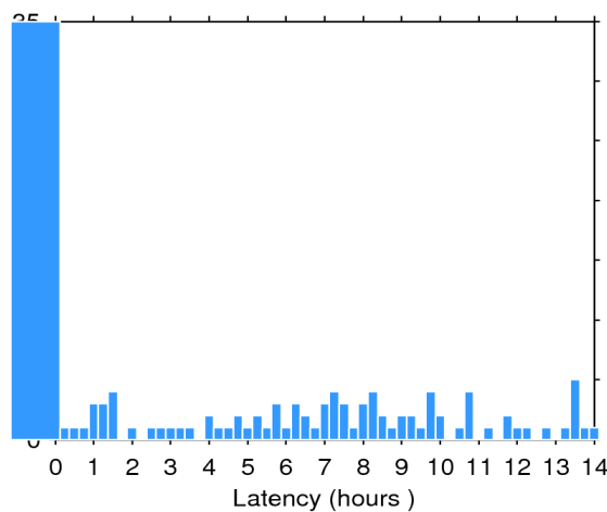
Figure 2. Histogram of the data latency for 03/02/2018. The y-axis denotes the number of files that are made available with a delay of x-hours with respect to the mean time of the records stored in the file.
