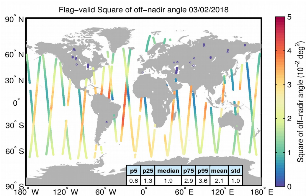
Figure 37. Geographical distribution of flag-valid mispointing data over oceans and lakes for 03/02/2018. The statistical values shown in the table refer to the mispointing in 10^{-2} deg 2 and are calculated over all measurements shown in the figure.
