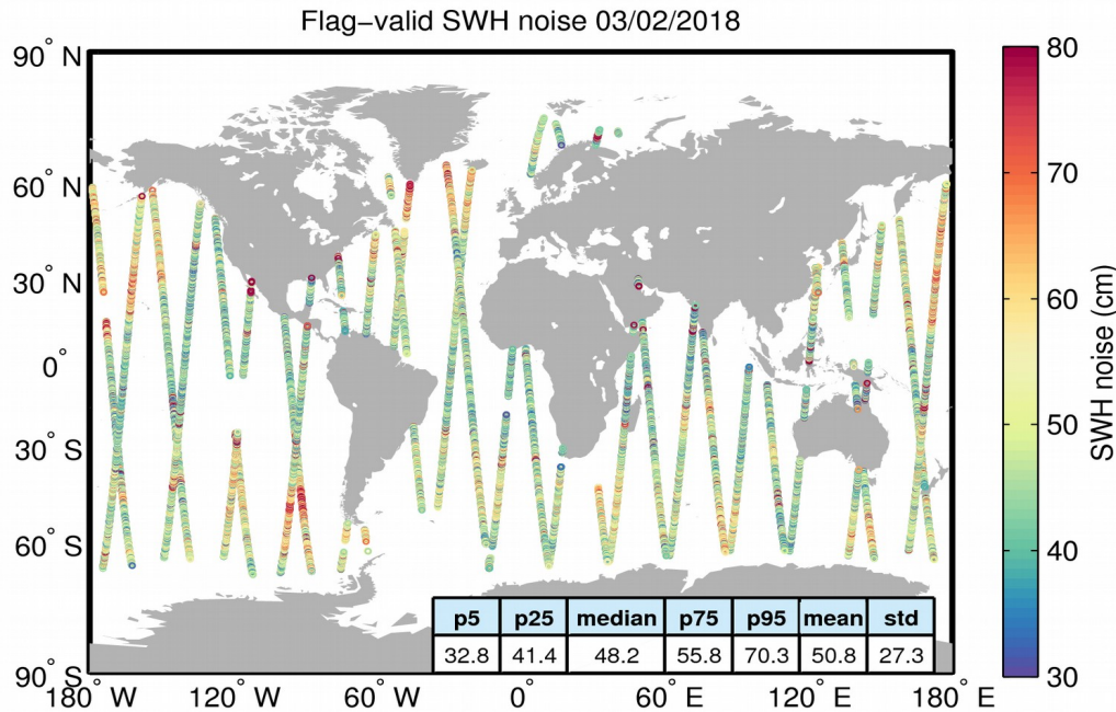
Figure 18. Geographical distribution of flag-valid 20-Hz SWH measurement noise over oceans and lakes for 03/02/2018. The statistical values shown in the figure refer to the SWH noise and are calculated over all measurements shown in the figure.
