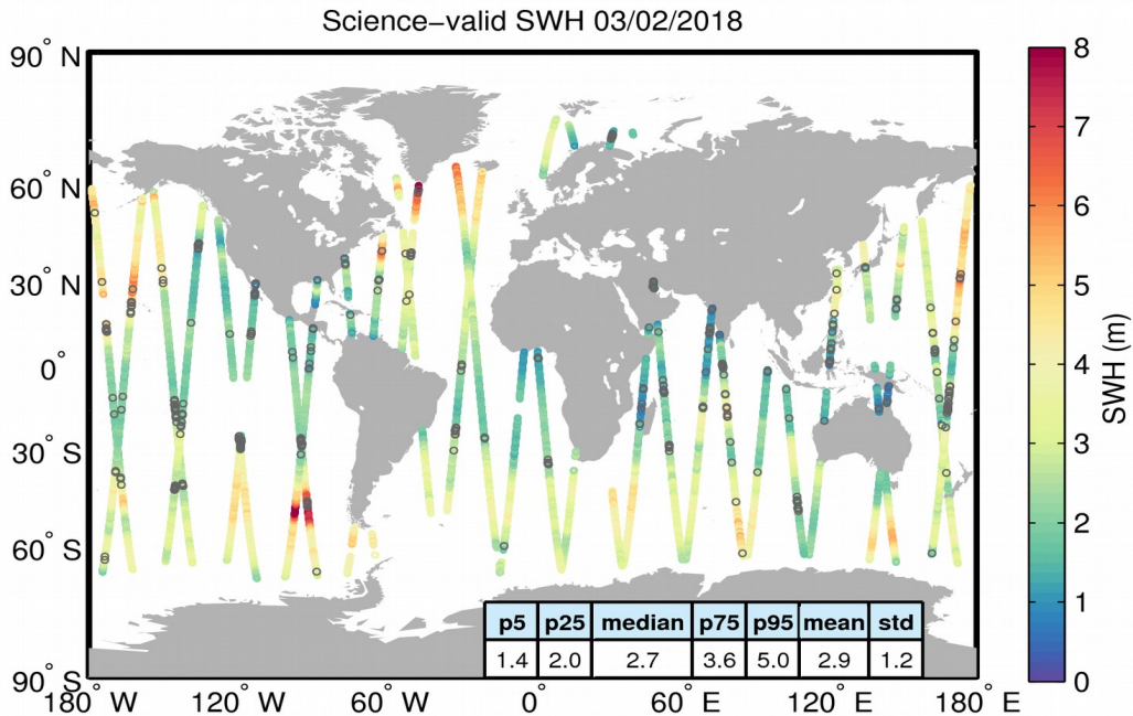
Figure 19. Geographical distribution of science-valid SWH data over oceans and lakes for 03/02/2018. The statistical values shown in the table refer to the SWH in m and are calculated over all measurements shown in the figure. Gray circles denote records that have been rejected based on the editing criteria described in Table 3.
