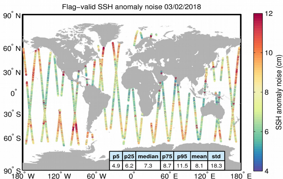
Figure 8. Geographical distribution of flag-valid 20-Hz SSH anomaly measurement noise over oceans and lakes for 03/02/2018. The statistical values shown in the table refer to the SSH anomaly noise and are calculated over all measurements shown in the figure.
