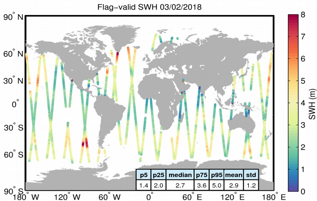
Figure 15. Geographical distribution of flag-valid SWH data over oceans and lakes for 03/02/2018. The statistical values shown in the table refer to the SWH in m and are calculated over all measurements shown in the figure.
