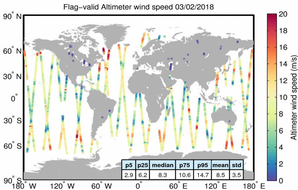
Figure 31. Geographical distribution of flag-valid wind data over oceans and lakes for 03/02/2018. The statistical values shown in the table refer to the wind in m/s and are calculated over all measurements shown in the figure.
