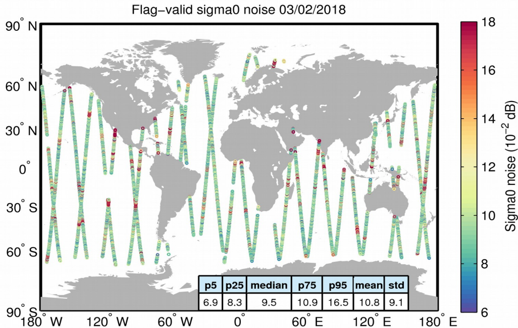
Figure 26. Geographical distribution of flag-valid 20-Hz sigma0 measurement noise over oceans and lakes for 03/02/2018. The statistical values shown in the table refer to the sigma0 noise and are calculated over all measurements shown in the figure.
