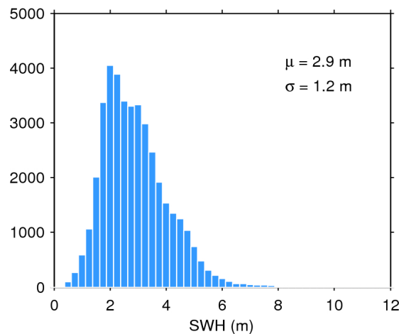
Figure 20. Histogram of science-valid SWH over oceans and lakes for 03/02/2018. The mean ( \mu ) and standard deviation ( \sigma ) are also shown. Note that values larger than 12 m are excluded from the histogram for the sake of readability but not from the computation of \mu and \sigma .
