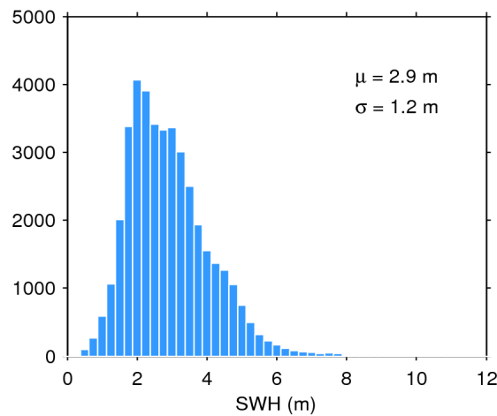
Figure 17. Histogram of flag-valid SWH over oceans and lakes for 03/02/2018. The mean ( \mu ) and standard deviation ( \sigma ) are also shown. Note that values larger than 12 m are excluded from the histogram for the sake of readability but not from the computation of \mu and \sigma .
