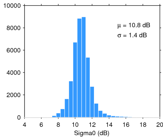
Figure 28. Histogram of science-valid sigma0 over oceans and lakes for 02/02/2018. The mean ( \mu ) and standard deviation ( \sigma ) are also shown. Note that values outside [4 20] dB are excluded from the histogram for the sake of readability but not from the computation of \mu and \sigma .
