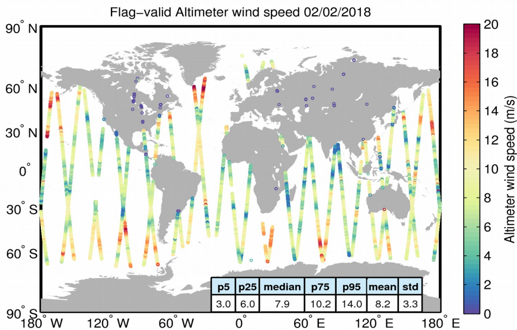
Figure 31. Geographical distribution of flag-valid wind data over oceans and lakes for 02/02/2018. The statistical values shown in the table refer to the wind in m/s and are calculated over all measurements shown in the figure.
