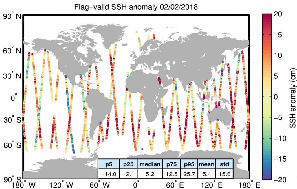
Figure 5. Geographical distribution of flag-valid 1-Hz SSH anomaly data over oceans and lakes for 02/02/2018. The statistical values shown in the table refer to the SSH anomaly in cm and are calculated over all measurements shown in the figure.
