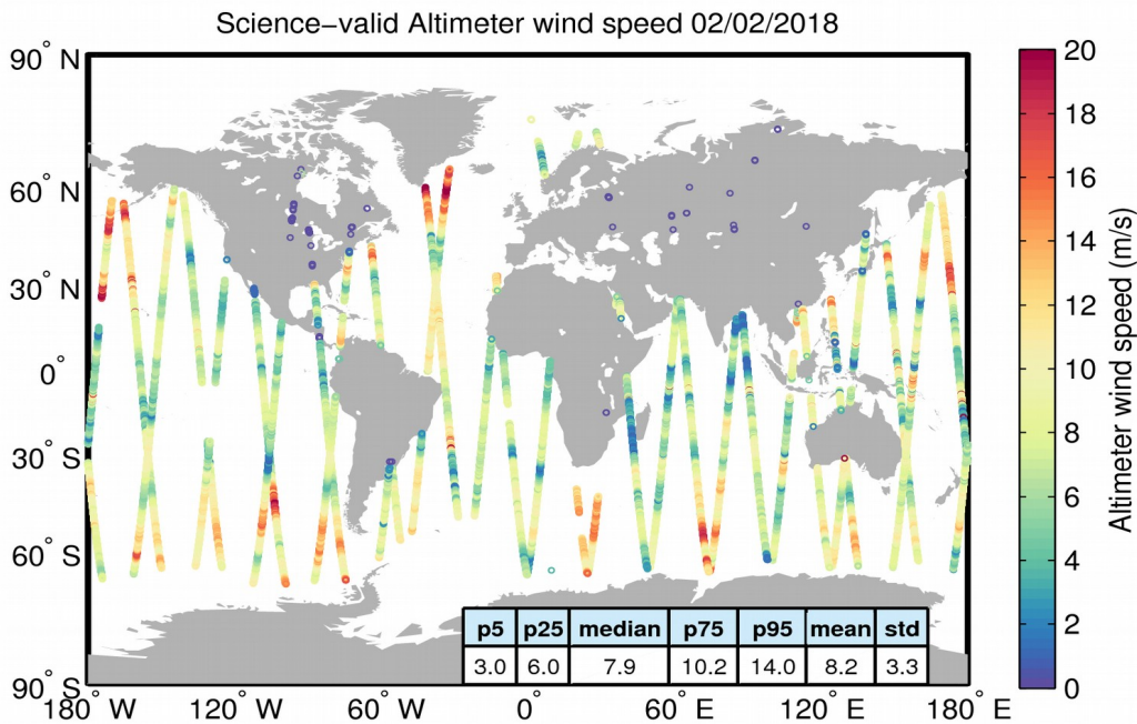
Figure 34. Geographical distribution of science-valid wind data over oceans and lakes for 02/02/2018. The statistical values shown in the table refer to the wind in m/s and are calculated over all measurements shown in the figure. Gray circles denote records that have been rejected based on the editing criteria described in Table 5.
