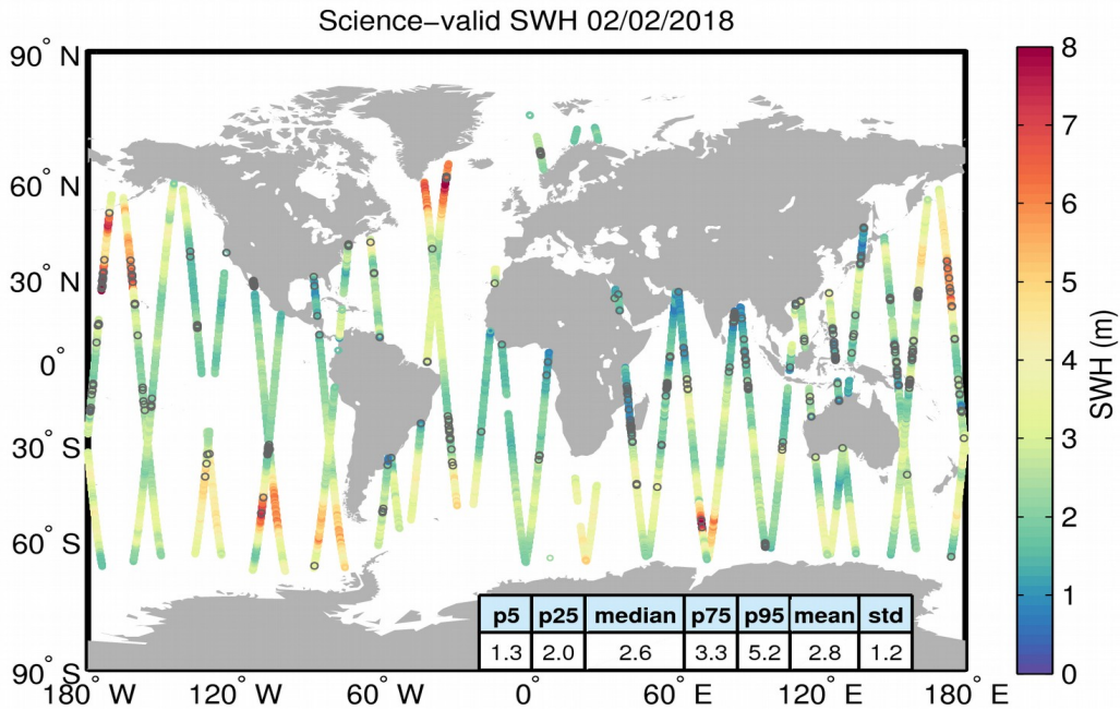
Figure 19. Geographical distribution of science-valid SWH data over oceans and lakes for 02/02/2018. The statistical values shown in the table refer to the SWH in m and are calculated over all measurements shown in the figure. Gray circles denote records that have been rejected based on the editing criteria described in Table 3.
