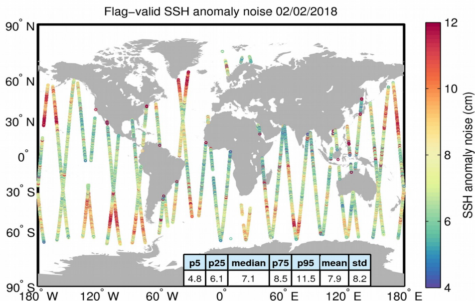
Figure 8. Geographical distribution of flag-valid 20-Hz SSH anomaly measurement noise over oceans and lakes for 02/02/2018. The statistical values shown in the table refer to the SSH anomaly noise and are calculated over all measurements shown in the figure.
