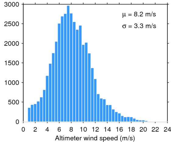
Figure 33. Histogram of flag-valid wind over oceans and lakes for 02/02/2018. The mean ( \mu ) and standard deviation ( \sigma ) are also shown. Note that values larger than 24 m/s are excluded from the histogram for the sake of readability but not from the computation of \mu and \sigma .
