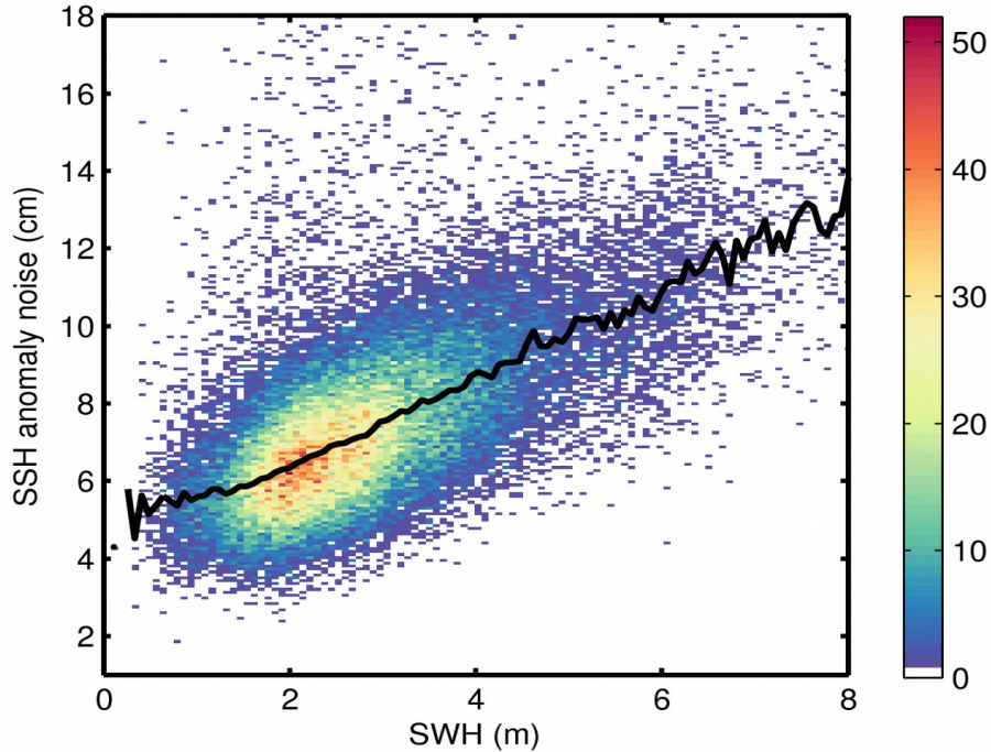
Figure 9. 2D histogram showing flag-valid SSH anomaly noise as a function of SWH for 02/02/2018. The black line denotes the median SSH anomaly noise as a function of SWH.
