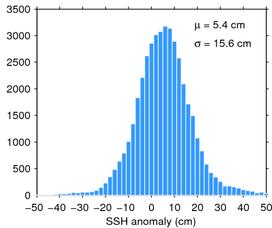
Figure 7. Histogram of flag-valid SSH anomaly over oceans and lakes for 02/02/2018. The mean ( \mu ) and standard deviation ( \sigma ) are also shown. Note that values outside [-50\ 50] cm are excluded from the histogram for the sake of readability but not from the computation of \mu and \sigma .
