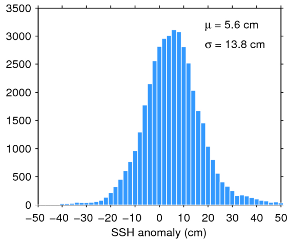
Figure 11. Histogram of science-valid SSH anomaly over oceans and lakes for 02/02/2018. The mean ( \mu ) and standard deviation ( \sigma ) are also shown. Note that values outside [-50 50] cm are excluded from the histogram for the sake of readability but not from the computation of \mu and \sigma .
