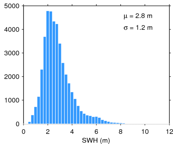
Figure 20. Histogram of science-valid SWH over oceans and lakes for 02/02/2018. The mean ( \mu ) and standard deviation ( \sigma ) are also shown. Note that values larger than 12 m are excluded from the histogram for the sake of readability but not from the computation of \mu and \sigma .
