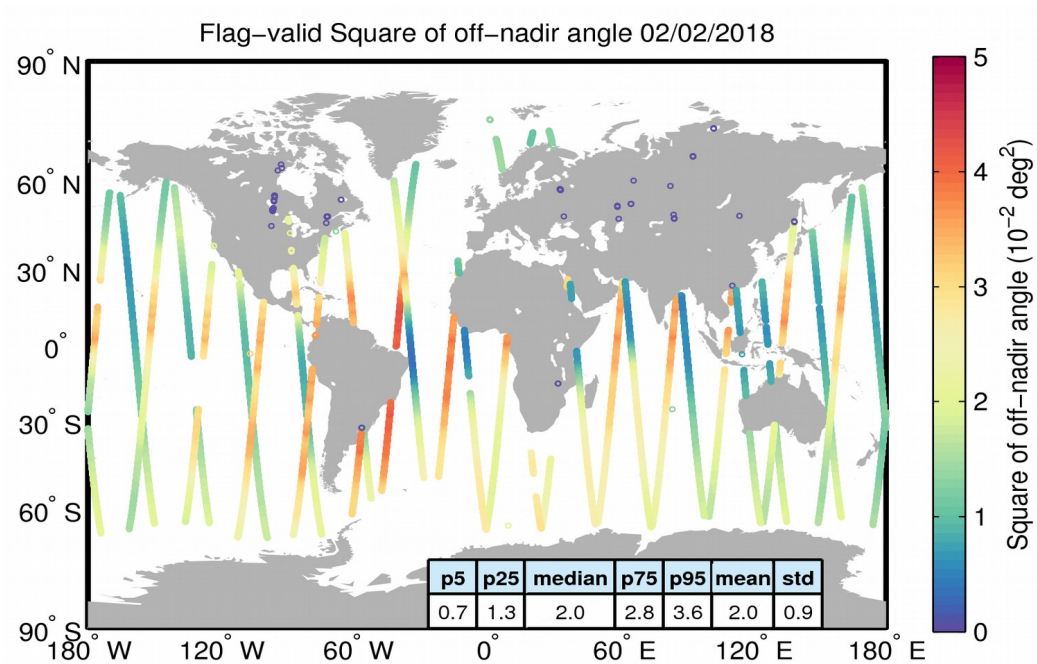
Figure 37. Geographical distribution of flag-valid mispointing data over oceans and lakes for 02/02/2018. The statistical values shown in the table refer to the mispointing in 10^{-2} deg 2 and are calculated over all measurements shown in the figure.
