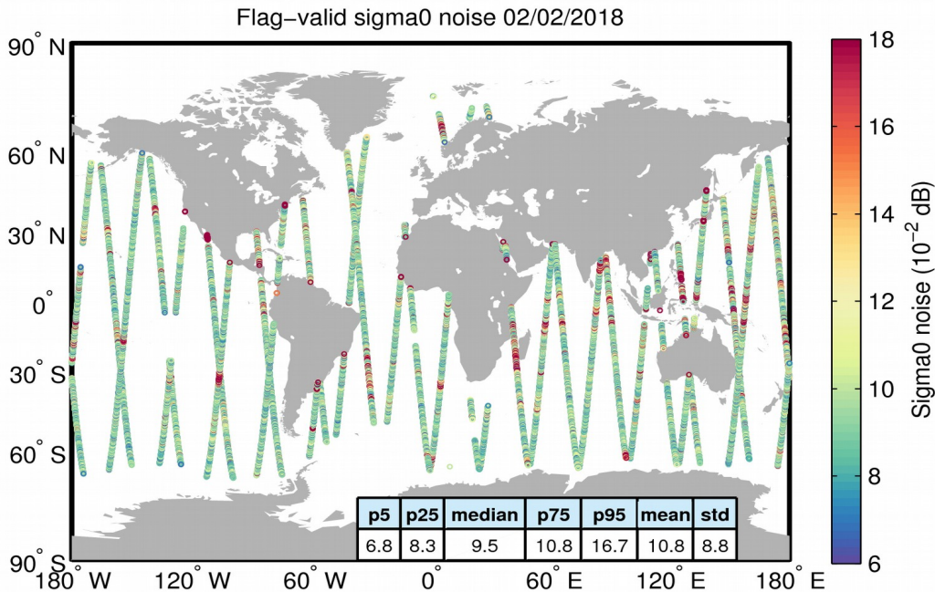
Figure 26. Geographical distribution of flag-valid 20-Hz sigma0 measurement noise over oceans and lakes for 02/02/2018. The statistical values shown in the table refer to the sigma0 noise and are calculated over all measurements shown in the figure.
