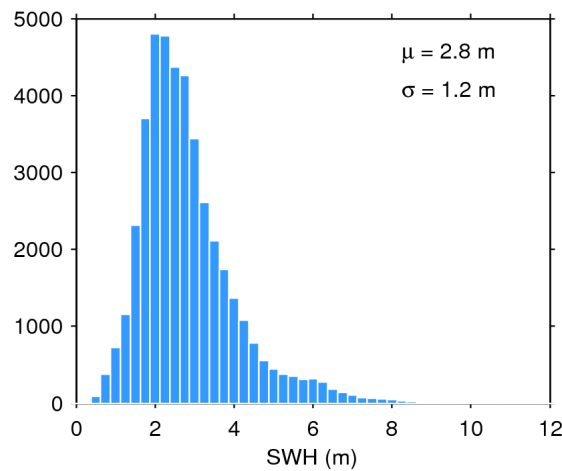
Figure 17. Histogram of flag-valid SWH over oceans and lakes for 02/02/2018. The mean ( \mu ) and standard deviation ( \sigma ) are also shown. Note that values larger than 12 m are excluded from the histogram for the sake of readability but not from the computation of \mu and \sigma .
