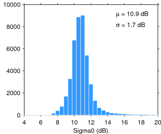
Figure 25. Histogram of flag-valid sigma0 over oceans and lakes for 02/02/2018. The mean ( \mu ) and standard deviation ( \sigma ) are also shown. Note that values outside [4 20] dB are excluded from the histogram for the sake of readability but not from the computation of \mu and \sigma .
