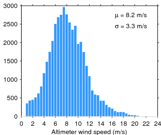
Figure 35. Histogram of science-valid wind over oceans and lakes for 02/02/2018. The mean ( \mu ) and standard deviation ( \sigma ) are also shown. Note that values larger than 24 m/s are excluded from the histogram for the sake of readability but not from the computation of \mu and \sigma .
