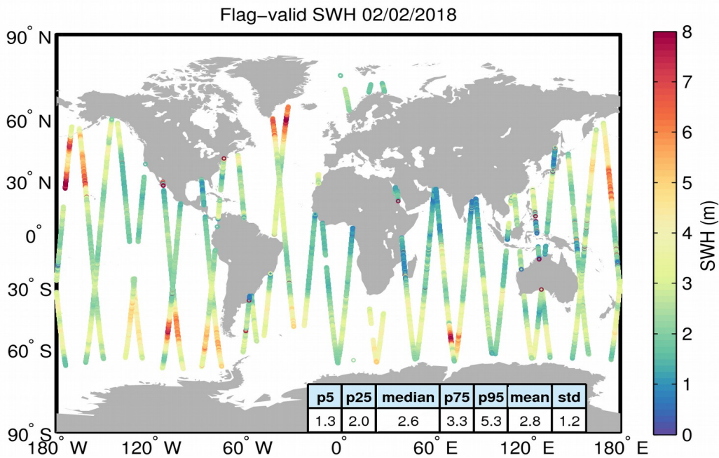
Figure 15. Geographical distribution of flag-valid SWH data over oceans and lakes for 02/02/2018. The statistical values shown in the table refer to the SWH in m and are calculated over all measurements shown in the figure.
