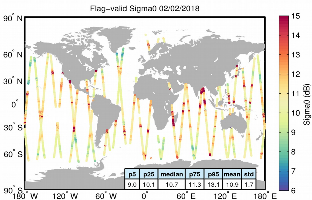
Figure 23. Geographical distribution of flag-valid sigma0 data over oceans and lakes for 02/02/2018. The statistical values shown in the table refer to the sigma0 in dB and are calculated over all measurements shown in the figure.
