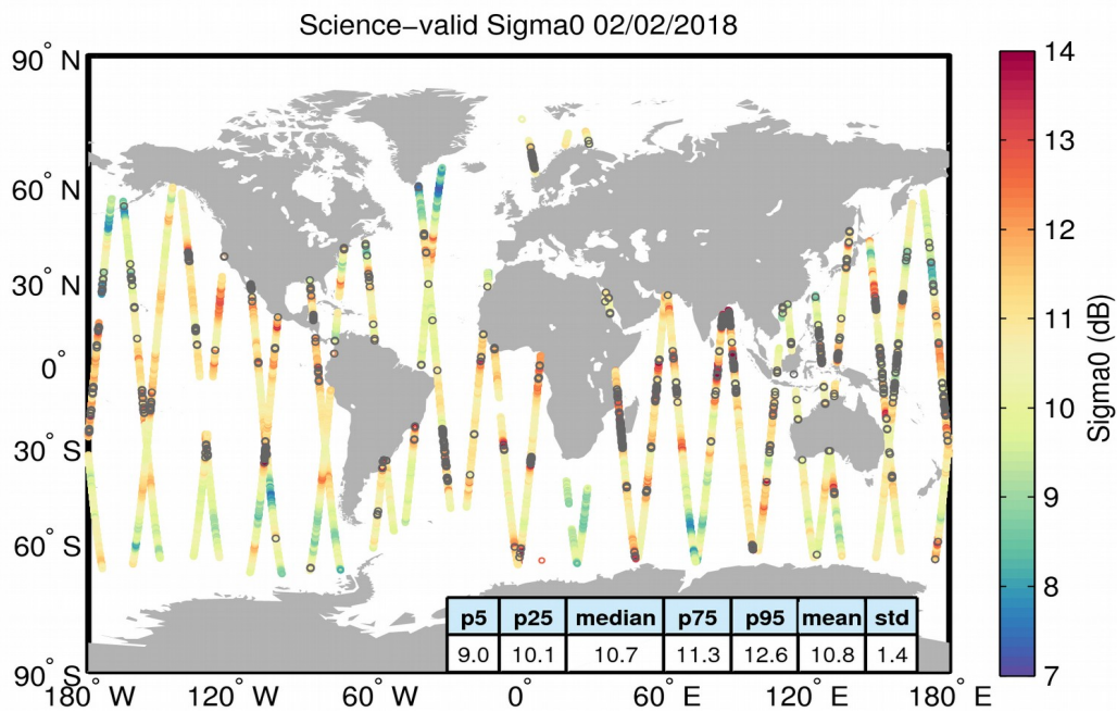
Figure 27. Geographical distribution of science-valid sigma0 data over oceans and lakes for 02/02/2018. The statistical values shown in the table refer to the sigma0 in dB and are calculated over all measurements shown in the figure. Gray circles denote records that have been rejected based on the editing criteria described in Table 4.
