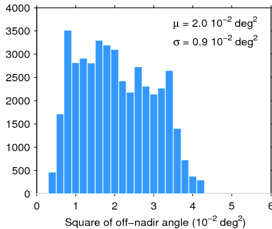
Figure 39. Histogram of flag-valid mispointing over oceans and lakes for 02/02/2018. The mean ( \mu ) and standard deviation ( \sigma ) are also shown. Note that values larger than 6 \cdot 10^{-2} \text{ deg}^2 are excluded from the histogram for the sake of readability but not from the computation of \mu and \sigma .
