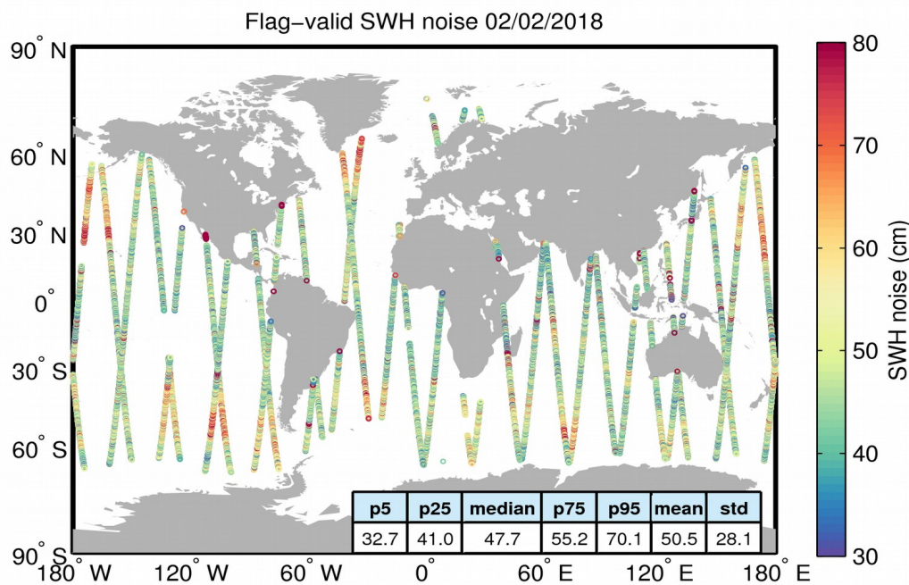
Figure 18. Geographical distribution of flag-valid 20-Hz SWH measurement noise over oceans and lakes for 02/02/2018. The statistical values shown in the table refer to the SWH noise and are calculated over all measurements shown in the figure.
