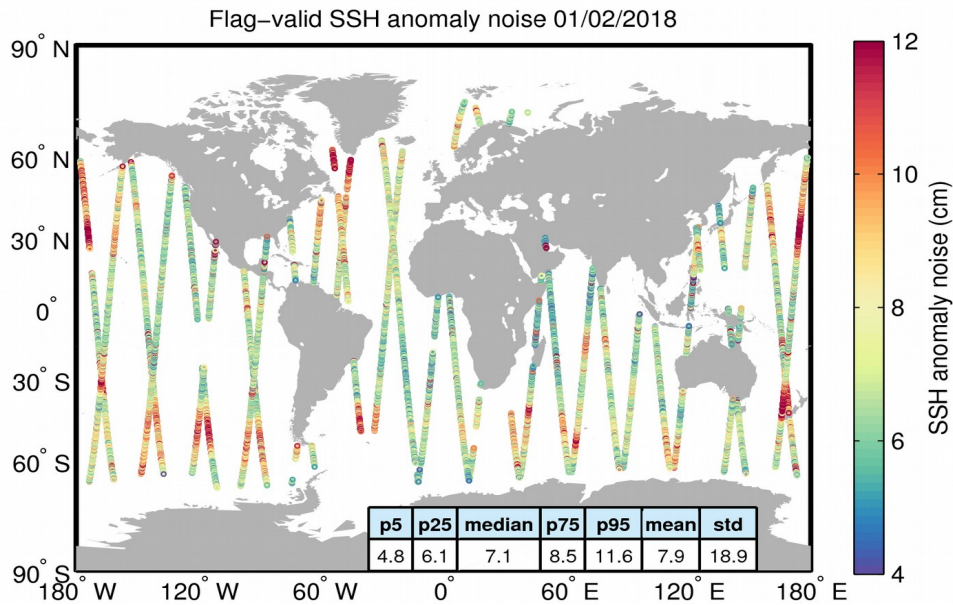
Figure 8. Geographical distribution of flag-valid 20-Hz SSH anomaly measurement noise over oceans and lakes for 01/02/2018. The statistical values shown in the table refer to the SSH anomaly noise and are calculated over all measurements shown in the figure.
