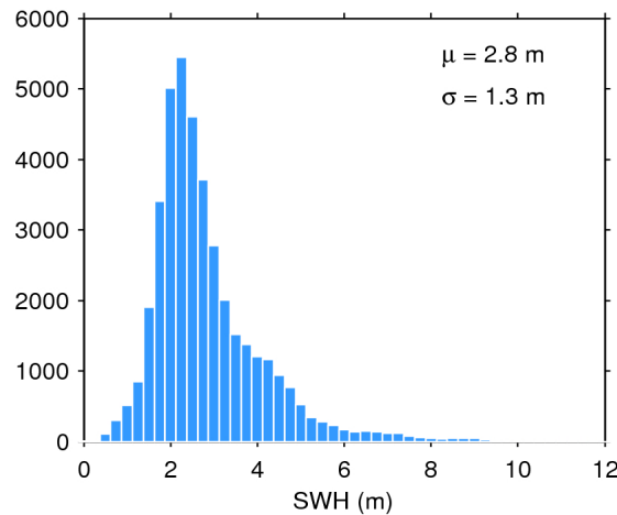
Figure 20. Histogram of science-valid SWH over oceans and lakes for 01/02/2018. The mean ( \mu ) and standard deviation ( \sigma ) are also shown. Note that values larger than 12 m are excluded from the histogram for the sake of readability but not from the computation of \mu and \sigma .
