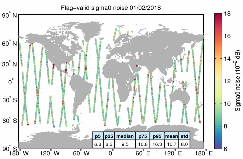
Figure 26. Geographical distribution of flag-valid 20-Hz sigma0 measurement noise over oceans and lakes for 01/02/2018. The statistical values shown in the figure refer to the sigma0 noise and are calculated over all measurements shown in the figure.
