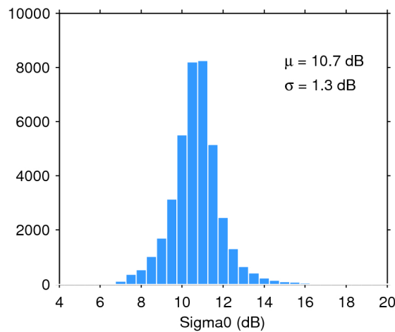
Figure 28. Histogram of science-valid sigma0 over oceans and lakes for 01/02/2018. The mean ( \mu ) and standard deviation ( \sigma ) are also shown. Note that values outside [4 20] dB are excluded from the histogram for the sake of readability but not from the computation of \mu and \sigma .
