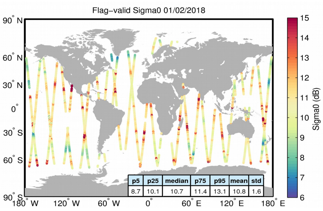
Figure 23. Geographical distribution of flag-valid sigma0 data over oceans and lakes for 01/02/2018. The statistical values shown in the table refer to the sigma0 in dB and are calculated over all measurements shown in the figure.
