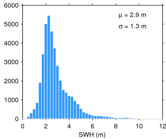
Figure 17. Histogram of flag-valid SWH over oceans and lakes for 01/02/2018. The mean ( \mu ) and standard deviation ( \sigma ) are also shown. Note that values larger than 12 m are excluded from the histogram for the sake of readability but not from the computation of \mu and \sigma .
