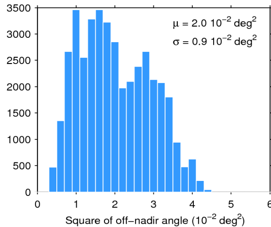
Figure 39. Histogram of flag-valid mispointing over oceans and lakes for 01/02/2018. The mean ( \mu ) and standard deviation ( \sigma ) are also shown. Note that values larger than 6 \cdot 10^{-2} \text{ deg}^2 are excluded from the histogram for the sake of readability but not from the computation of \mu and \sigma .
