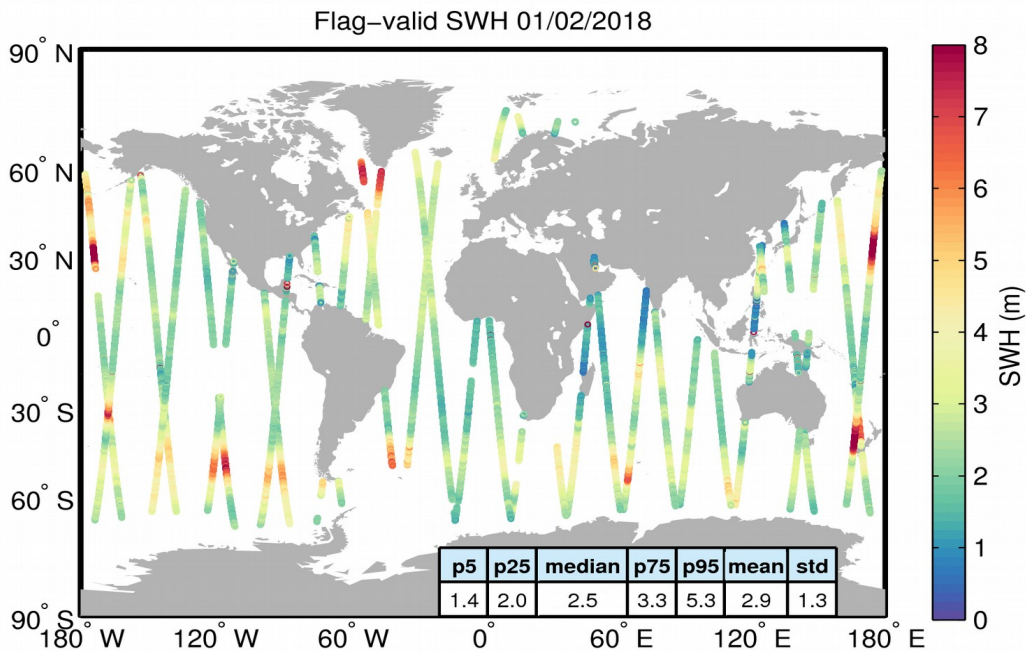
Figure 15. Geographical distribution of flag-valid SWH data over oceans and lakes for 01/02/2018. The statistical values shown in the table refer to the SWH in m and are calculated over all measurements shown in the figure.
