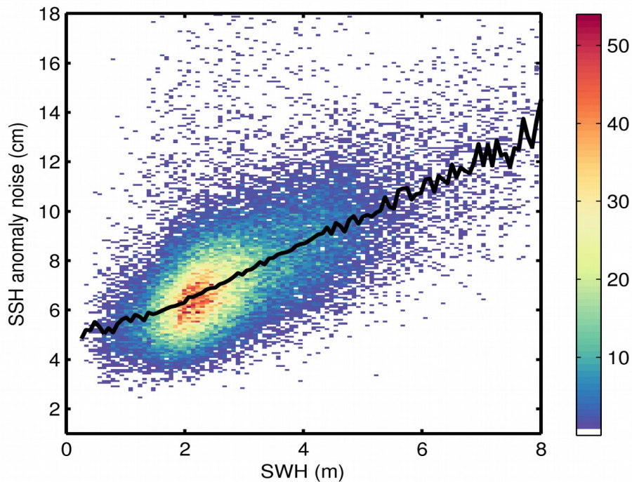
Figure 9. 2D histogram showing flag-valid SSH anomaly noise as a function of SWH for 01/02/2018. The black line denotes the median SSH anomaly noise as a function of SWH.
