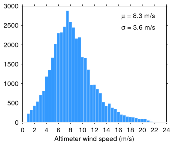
Figure 35. Histogram of science-valid wind over oceans and lakes for 01/02/2018. The mean ( \mu ) and standard deviation ( \sigma ) are also shown. Note that values larger than 24 m/s are excluded from the histogram for the sake of readability but not from the computation of \mu and \sigma .
