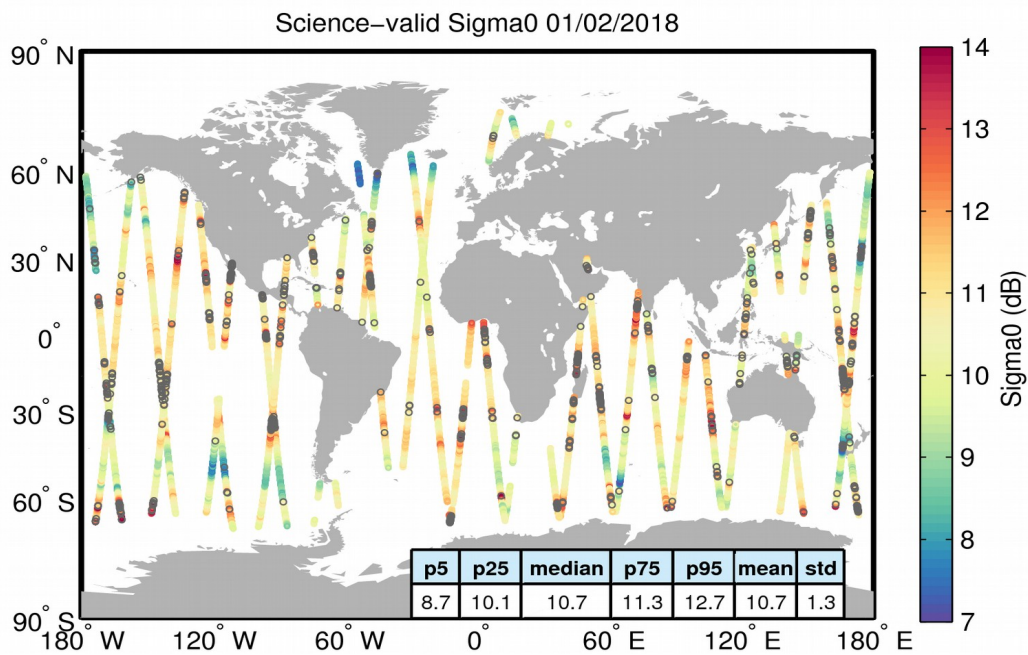
Figure 27. Geographical distribution of science-valid sigma0 data over oceans and lakes for 01/02/2018. The statistical values shown in the table refer to the sigma0 in dB and are calculated over all measurements shown in the figure. Gray circles denote records that have been rejected based on the editing criteria described in Table 4.
