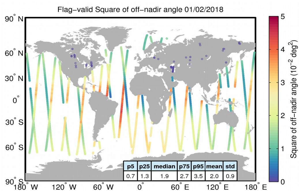
Figure 37. Geographical distribution of flag-valid mispointing data over oceans and lakes for 01/02/2018. The statistical values shown in the table refer to the mispointing in 10^{-2} \text{ deg}^2 and are calculated over all measurements shown in the figure.
