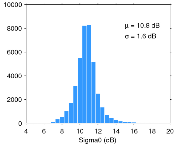
Figure 25. Histogram of flag-valid sigma0 over oceans and lakes for 01/02/2018. The mean ( \mu ) and standard deviation ( \sigma ) are also shown. Note that values outside [4 20] dB are excluded from the histogram for the sake of readability but not from the computation of \mu and \sigma .
