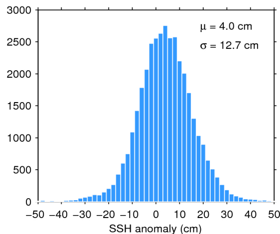
Figure 11. Histogram of science-valid SSH anomaly over oceans and lakes for 01/02/2018. The mean ( \mu ) and standard deviation ( \sigma ) are also shown. Note that values outside [-50 50] cm are excluded from the histogram for the sake of readability but not from the computation of \mu and \sigma .
