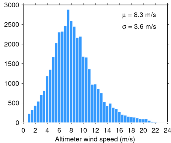
Figure 33. Histogram of flag-valid wind over oceans and lakes for 01/02/2018. The mean ( \mu ) and standard deviation ( \sigma ) are also shown. Note that values larger than 24 m/s are excluded from the histogram for the sake of readability but not from the computation of \mu and \sigma .
