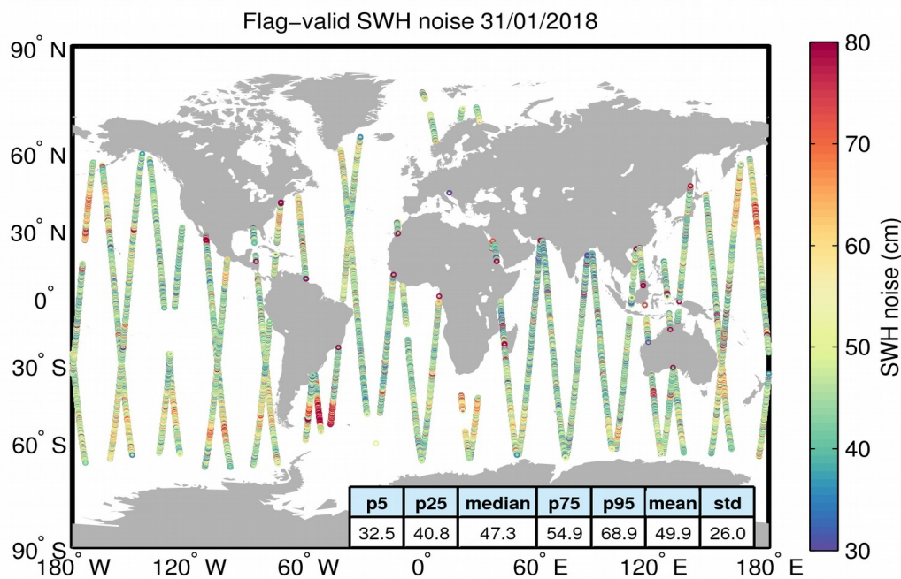
Figure 18. Geographical distribution of flag-valid 20-Hz SWH measurement noise over oceans and lakes for 31/01/2018. The statistical values shown in the figure refer to the SWH noise and are calculated over all measurements shown in the figure.
