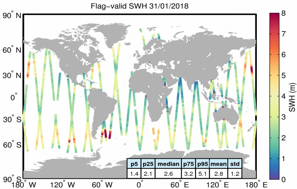
Figure 15. Geographical distribution of flag-valid SWH data over oceans and lakes for 31/01/2018. The statistical values shown in the table refer to the SWH in m and are calculated over all measurements shown in the figure.
