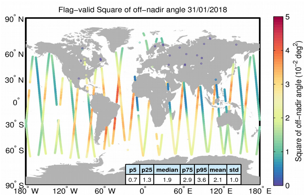
Figure 37. Geographical distribution of flag-valid mispointing data over oceans and lakes for 31/01/2018. The statistical values shown in the table refer to the mispointing in 10^{-2} \text{ deg}^2 and are calculated over all measurements shown in the figure.
