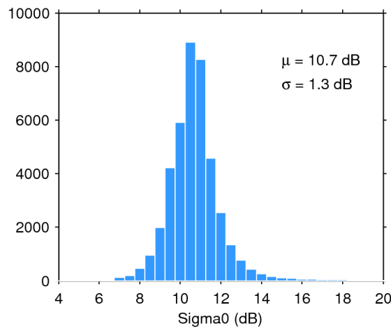
Figure 28. Histogram of science-valid sigma0 over oceans and lakes for 31/01/2018. The mean ( \mu ) and standard deviation ( \sigma ) are also shown. Note that values outside [4 20] dB are excluded from the histogram for the sake of readability but not from the computation of \mu and \sigma .
