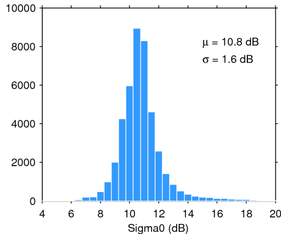
Figure 25. Histogram of flag-valid sigma0 over oceans and lakes for 31/01/2018. The mean ( \mu ) and standard deviation ( \sigma ) are also shown. Note that values outside [4 20] dB are excluded from the histogram for the sake of readability but not from the computation of \mu and \sigma .
