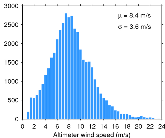
Figure 35. Histogram of science-valid wind over oceans and lakes for 31/01/2018. The mean ( \mu ) and standard deviation ( \sigma ) are also shown. Note that values larger than 24 m/s are excluded from the histogram for the sake of readability but not from the computation of \mu and \sigma .
