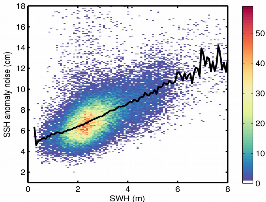
Figure 9. 2D histogram showing flag-valid SSH anomaly noise as a function of SWH for 31/01/2018. The black line denotes the median SSH anomaly noise as a function of SWH.
