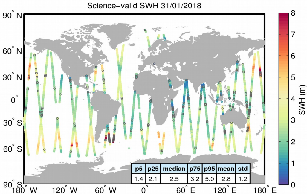
Figure 19. Geographical distribution of science-valid SWH data over oceans and lakes for 31/01/2018. The statistical values shown in the table refer to the SWH in m and are calculated over all measurements shown in the figure. Gray circles denote records that have been rejected based on the editing criteria described in Table 3.
