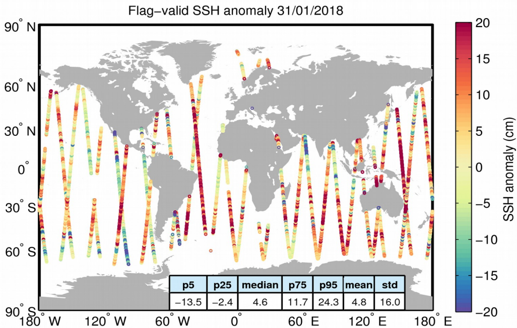
Figure 5. Geographical distribution of flag-valid 1-Hz SSH anomaly data over oceans and lakes for 31/01/2018. The statistical values shown in the table refer to the SSH anomaly in cm and are calculated over all measurements shown in the figure.
