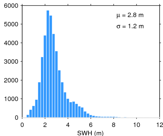
Figure 20. Histogram of science-valid SWH over oceans and lakes for 31/01/2018. The mean ( \mu ) and standard deviation ( \sigma ) are also shown. Note that values larger than 12 m are excluded from the histogram for the sake of readability but not from the computation of \mu and \sigma .
