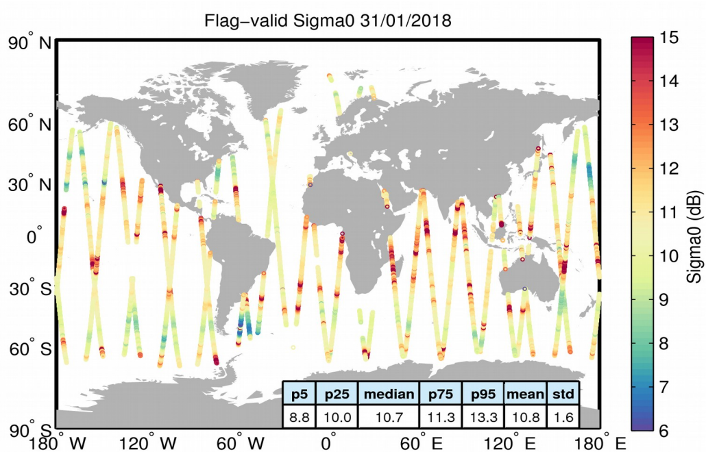
Figure 23. Geographical distribution of flag-valid sigma0 data over oceans and lakes for 31/01/2018. The statistical values shown in the table refer to the sigma0 in dB and are calculated over all measurements shown in the figure.
