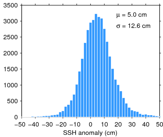
Figure 11. Histogram of science-valid SSH anomaly over oceans and lakes for 31/01/2018. The mean ( \mu ) and standard deviation ( \sigma ) are also shown. Note that values outside [-50 50] cm are excluded from the histogram for the sake of readability but not from the computation of \mu and \sigma .
