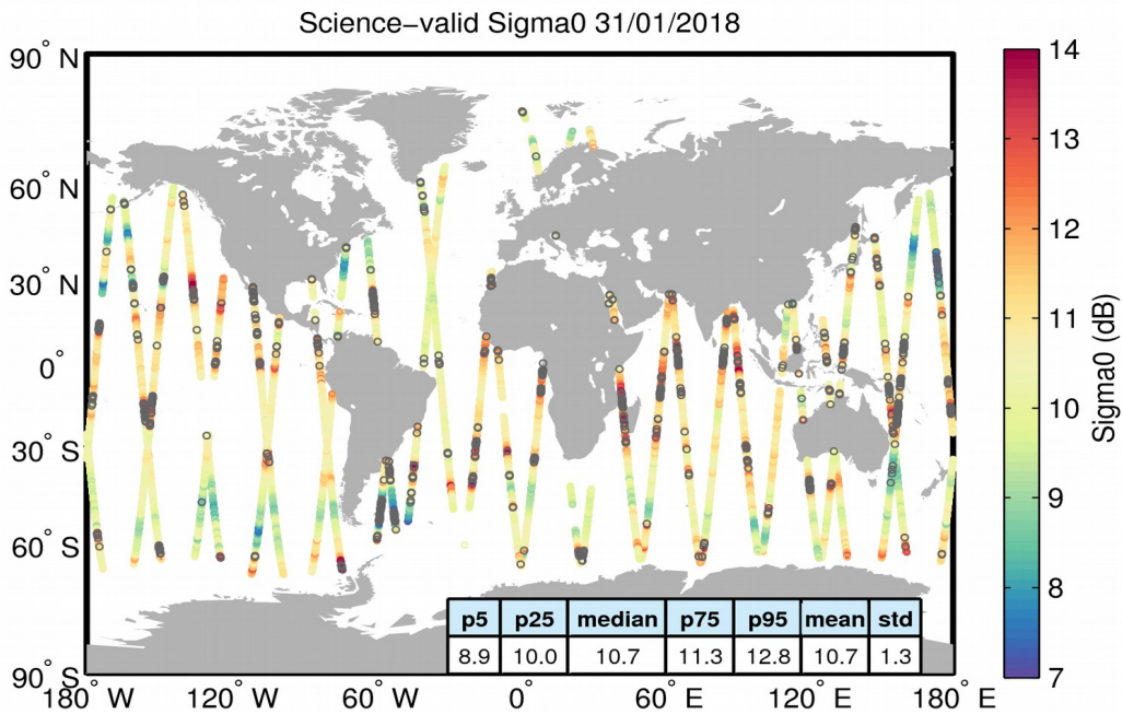
Figure 27. Geographical distribution of science-valid sigma0 data over oceans and lakes for 31/01/2018. The statistical values shown in the table refer to the sigma0 in dB and are calculated over all measurements shown in the figure. Gray circles denote records that have been rejected based on the editing criteria described in Table 4.
