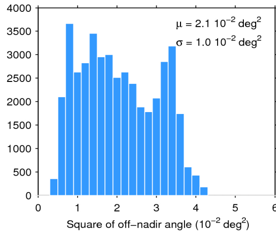
Figure 39. Histogram of flag-valid mispointing over oceans and lakes for 31/01/2018. The mean ( \mu ) and standard deviation ( \sigma ) are also shown. Note that values larger than 6 \cdot 10^{-2} \text{ deg}^2 are excluded from the histogram for the sake of readability but not from the computation of \mu and \sigma .
