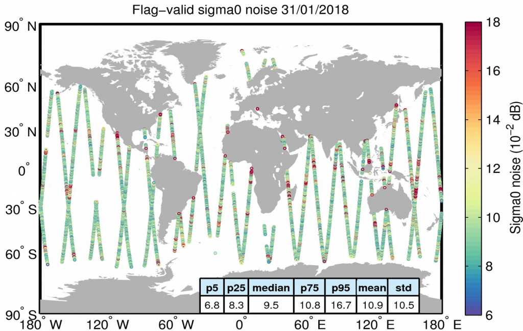
Figure 26. Geographical distribution of flag-valid 20-Hz sigma0 measurement noise over oceans and lakes for 31/01/2018. The statistical values shown in the table refer to the sigma0 noise and are calculated over all measurements shown in the figure.
