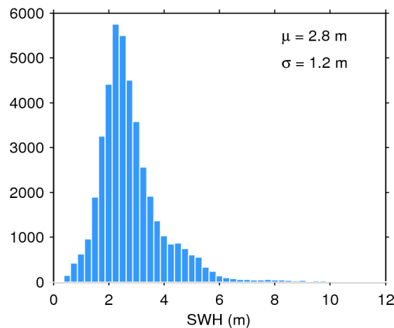
Figure 17. Histogram of flag-valid SWH over oceans and lakes for 31/01/2018. The mean ( \mu ) and standard deviation ( \sigma ) are also shown. Note that values larger than 12 m are excluded from the histogram for the sake of readability but not from the computation of \mu and \sigma .
