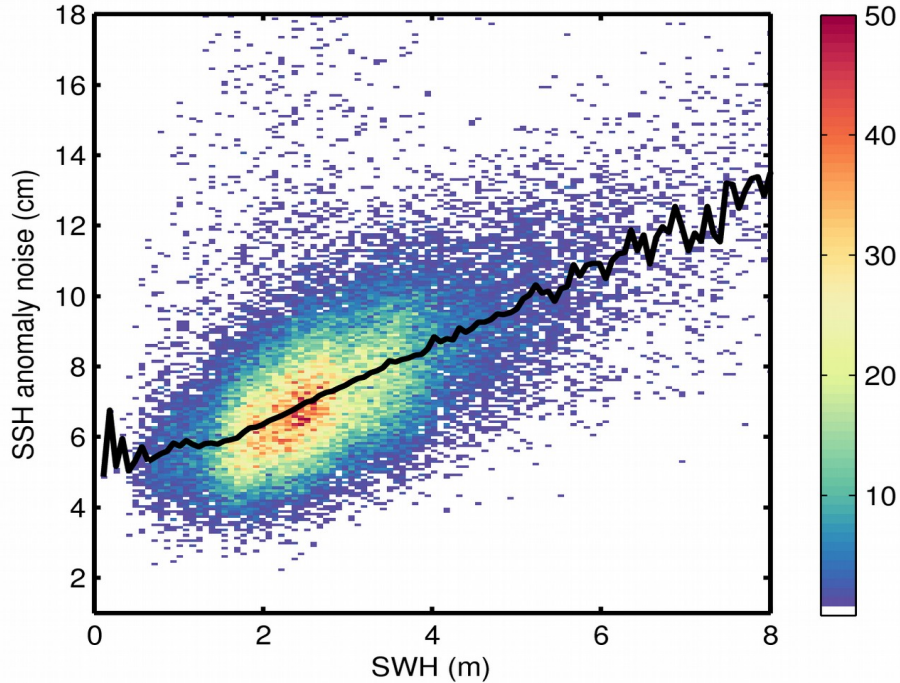
Figure 9. 2D histogram showing flag-valid SSH anomaly noise as a function of SWH for 29/01/2018. The black line denotes the median SSH anomaly noise as a function of SWH.
