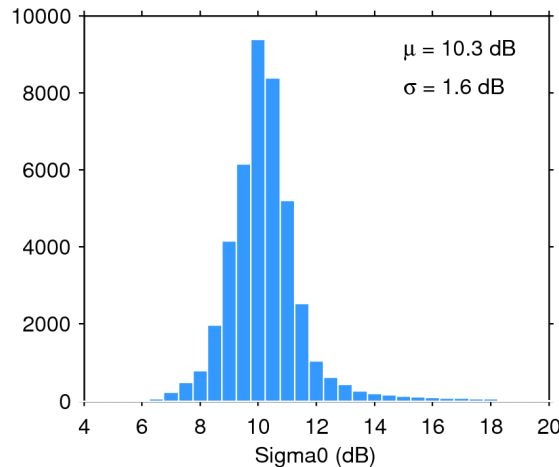
Figure 25. Histogram of flag-valid sigma0 over oceans and lakes for 29/01/2018. The mean ( \mu ) and standard deviation ( \sigma ) are also shown. Note that values outside [4 20] dB are excluded from the histogram for the sake of readability but not from the computation of \mu and \sigma .
