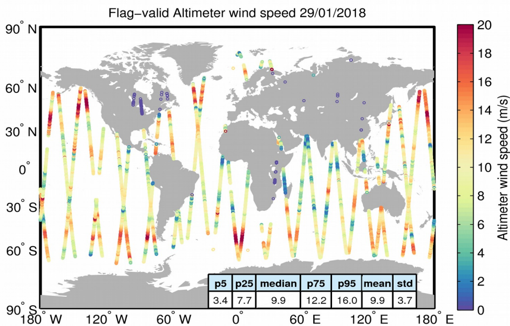
Figure 31. Geographical distribution of flag-valid wind data over oceans and lakes for 29/01/2018. The statistical values shown in the table refer to the wind in m/s and are calculated over all measurements shown in the figure.
