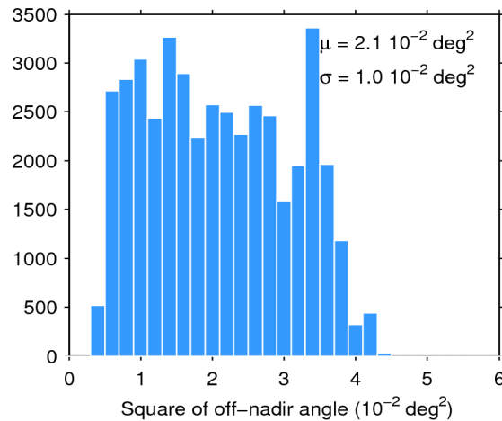
Figure 39. Histogram of flag-valid mispointing over oceans and lakes for 29/01/2018. The mean ( \mu ) and standard deviation ( \sigma ) are also shown. Note that values larger than 6 \cdot 10^{-2} \text{ deg}^2 are excluded from the histogram for the sake of readability but not from the computation of \mu and \sigma .
