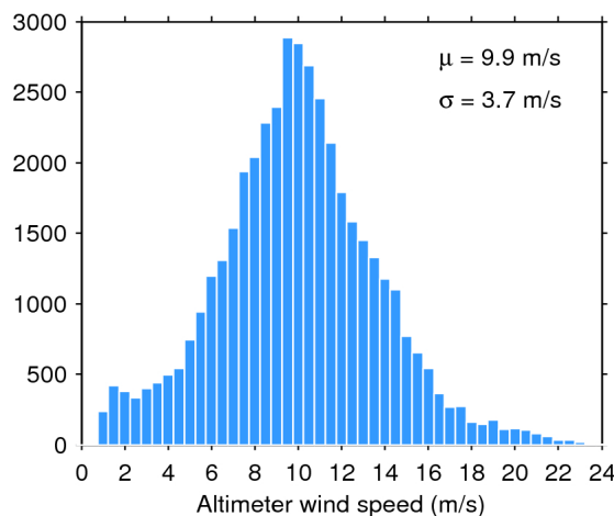
Figure 35. Histogram of science-valid wind over oceans and lakes for 29/01/2018. The mean ( \mu ) and standard deviation ( \sigma ) are also shown. Note that values larger than 24 m/s are excluded from the histogram for the sake of readability but not from the computation of \mu and \sigma .
