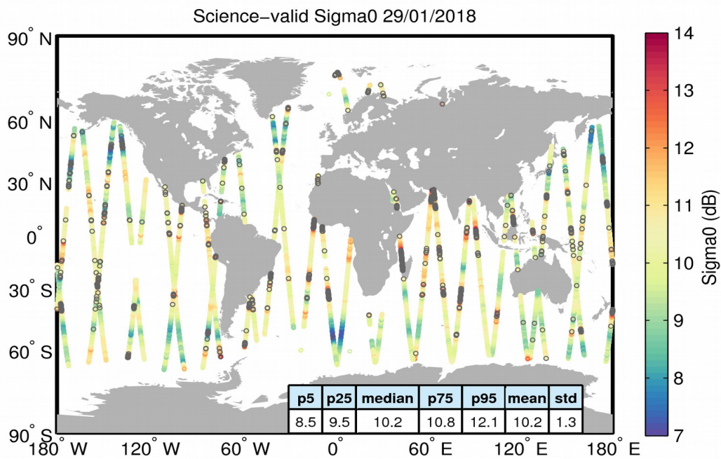
Figure 27. Geographical distribution of science-valid sigma0 data over oceans and lakes for 29/01/2018. The statistical values shown in the table refer to the sigma0 in dB and are calculated over all measurements shown in the figure. Gray circles denote records that have been rejected based on the editing criteria described in Table 4.
