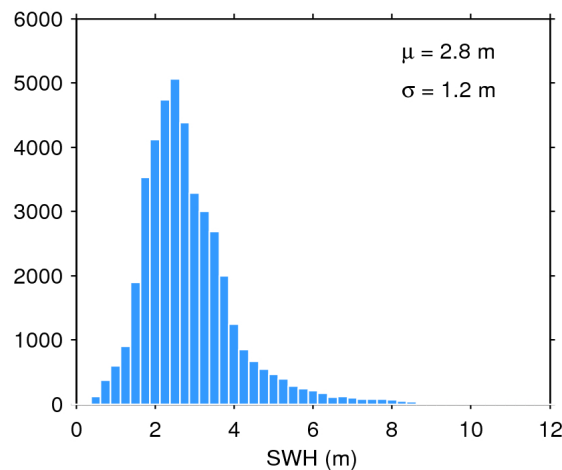
Figure 20. Histogram of science-valid SWH over oceans and lakes for 29/01/2018. The mean ( \mu ) and standard deviation ( \sigma ) are also shown. Note that values larger than 12 m are excluded from the histogram for the sake of readability but not from the computation of \mu and \sigma .
