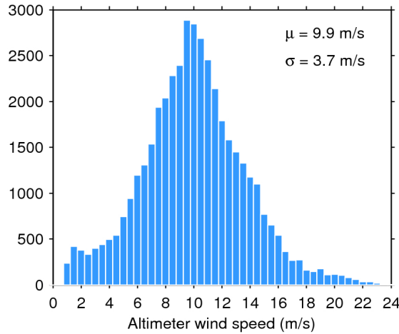
Figure 33. Histogram of flag-valid wind over oceans and lakes for 29/01/2018. The mean ( \mu ) and standard deviation ( \sigma ) are also shown. Note that values larger than 24 m/s are excluded from the histogram for the sake of readability but not from the computation of \mu and \sigma .
