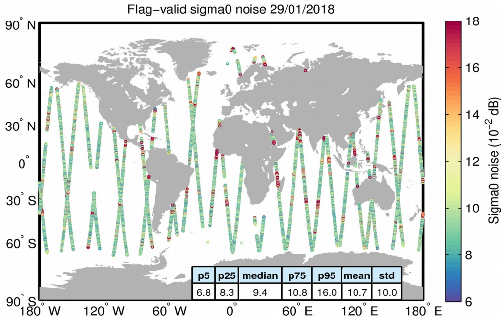
Figure 26. Geographical distribution of flag-valid 20-Hz sigma0 measurement noise over oceans and lakes for 29/01/2018. The statistical values shown in the table refer to the sigma0 noise and are calculated over all measurements shown in the figure.
