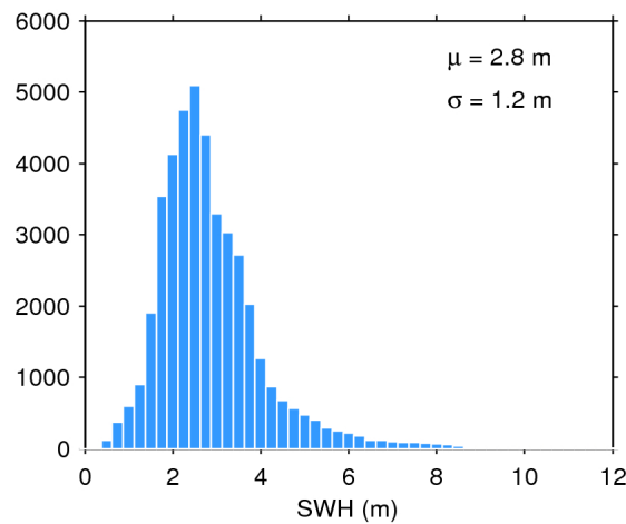
Figure 17. Histogram of flag-valid SWH over oceans and lakes for 29/01/2018. The mean ( \mu ) and standard deviation ( \sigma ) are also shown. Note that values larger than 12 m are excluded from the histogram for the sake of readability but not from the computation of \mu and \sigma .
