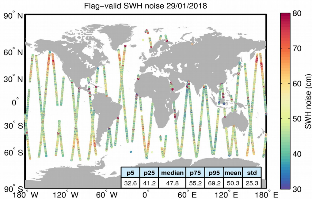
Figure 18. Geographical distribution of flag-valid 20-Hz SWH measurement noise over oceans and lakes for 29/01/2018. The statistical values shown in the figure refer to the SWH noise and are calculated over all measurements shown in the figure.
