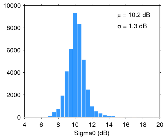
Figure 28. Histogram of science-valid sigma0 over oceans and lakes for 29/01/2018. The mean ( \mu ) and standard deviation ( \sigma ) are also shown. Note that values outside [4 20] dB are excluded from the histogram for the sake of readability but not from the computation of \mu and \sigma .
