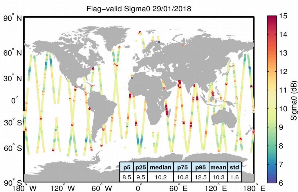
Figure 23. Geographical distribution of flag-valid sigma0 data over oceans and lakes for 29/01/2018. The statistical values shown in the table refer to the sigma0 in dB and are calculated over all measurements shown in the figure.
