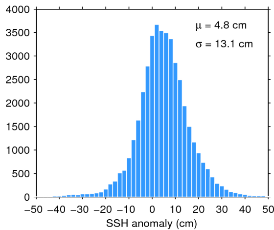
Figure 7. Histogram of flag-valid SSH anomaly over oceans and lakes for 29/01/2018. The mean ( \mu ) and standard deviation ( \sigma ) are also shown. Note that values outside [-50\ 50] cm are excluded from the histogram for the sake of readability but not from the computation of \mu and \sigma .
