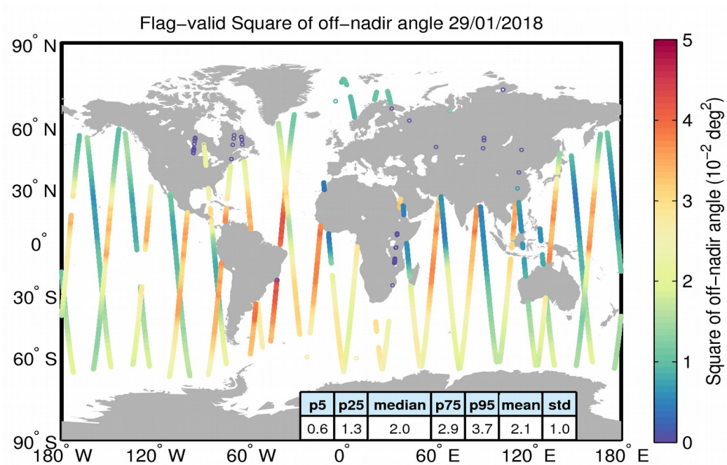
Figure 37. Geographical distribution of flag-valid mispointing data over oceans and lakes for 29/01/2018. The statistical values shown in the table refer to the mispointing in 10^{-2} \text{ deg}^2 and are calculated over all measurements shown in the figure.
