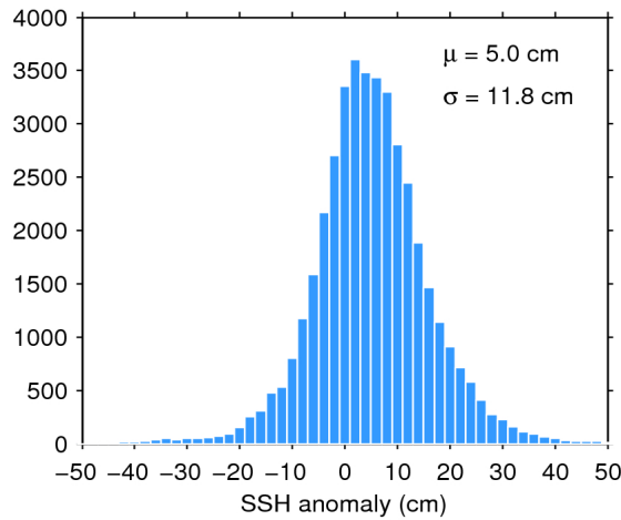
Figure 11. Histogram of science-valid SSH anomaly over oceans and lakes for 29/01/2018. The mean ( \mu ) and standard deviation ( \sigma ) are also shown. Note that values outside [-50 50] cm are excluded from the histogram for the sake of readability but not from the computation of \mu and \sigma .
