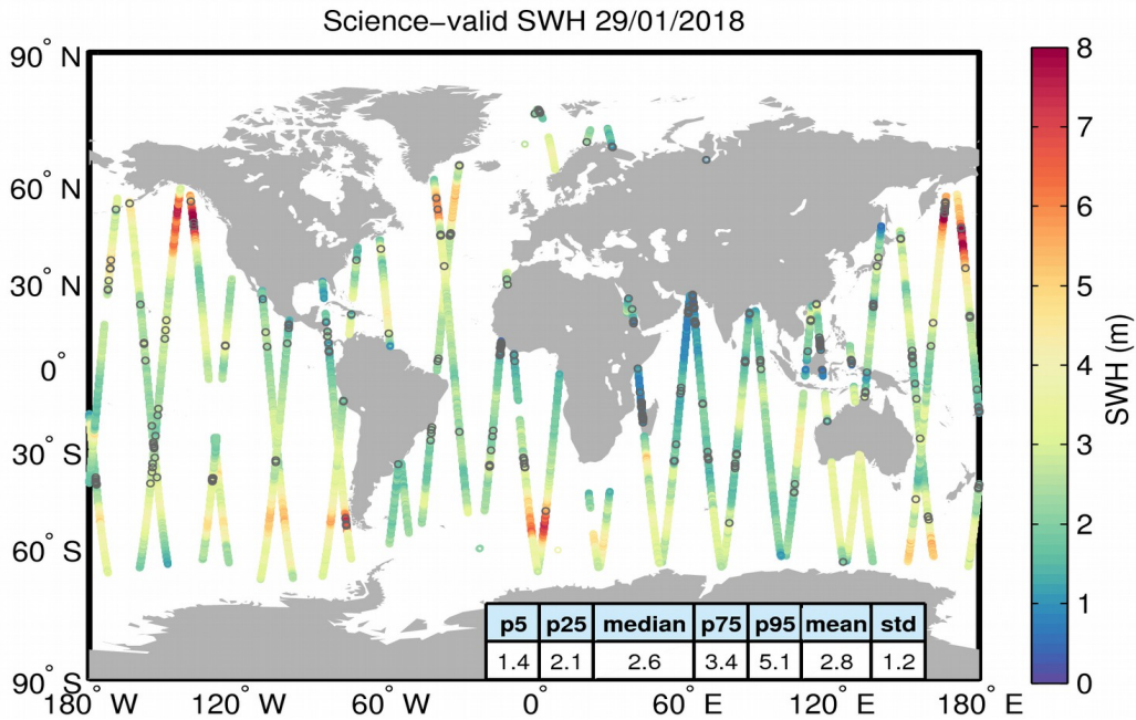
Figure 19. Geographical distribution of science-valid SWH data over oceans and lakes for 29/01/2018. The statistical values shown in the table refer to the SWH in m and are calculated over all measurements shown in the figure. Gray circles denote records that have been rejected based on the editing criteria described in Table 3.
