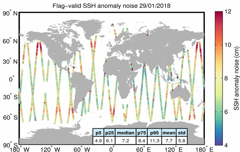
Figure 8. Geographical distribution of flag-valid 20-Hz SSH anomaly measurement noise over oceans and lakes for 29/01/2018. The statistical values shown in the table refer to the SSH anomaly noise and are calculated over all measurements shown in the figure.
