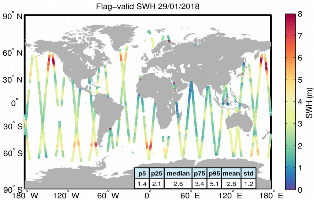
Figure 15. Geographical distribution of flag-valid SWH data over oceans and lakes for 29/01/2018. The statistical values shown in the table refer to the SWH in m and are calculated over all measurements shown in the figure.
