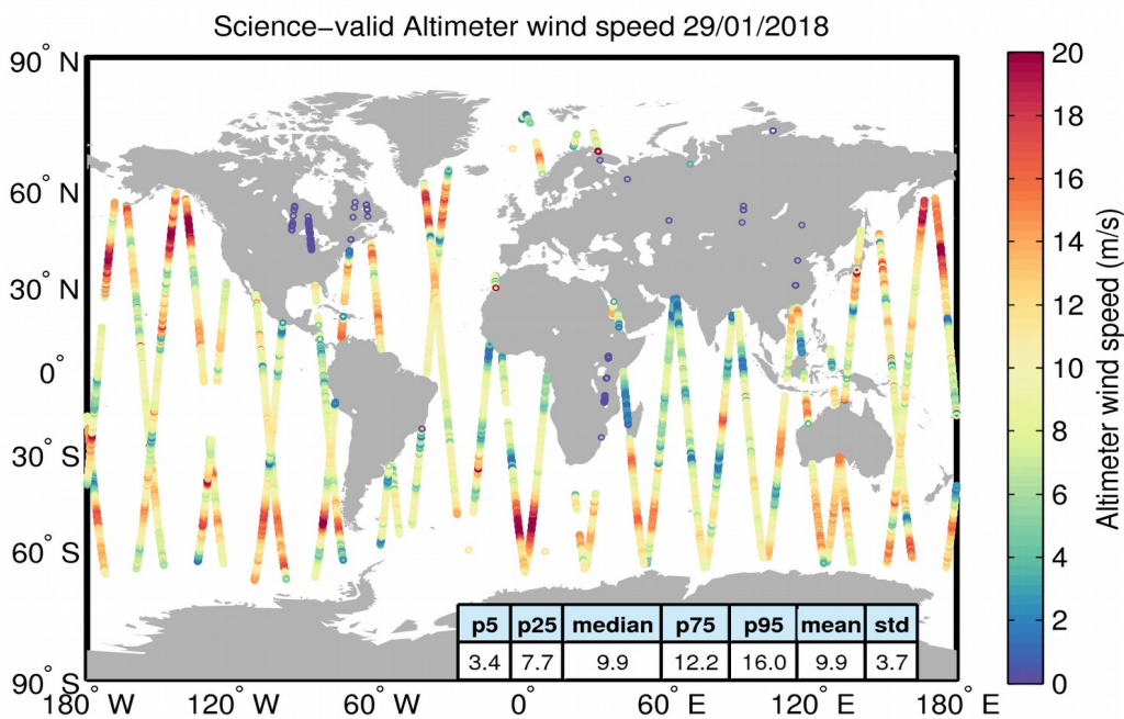
Figure 34. Geographical distribution of science-valid wind data over oceans and lakes for 29/01/2018. The statistical values shown in the table refer to the wind in m/s and are calculated over all measurements shown in the figure. Gray circles denote records that have been rejected based on the editing criteria described in Table 5.
