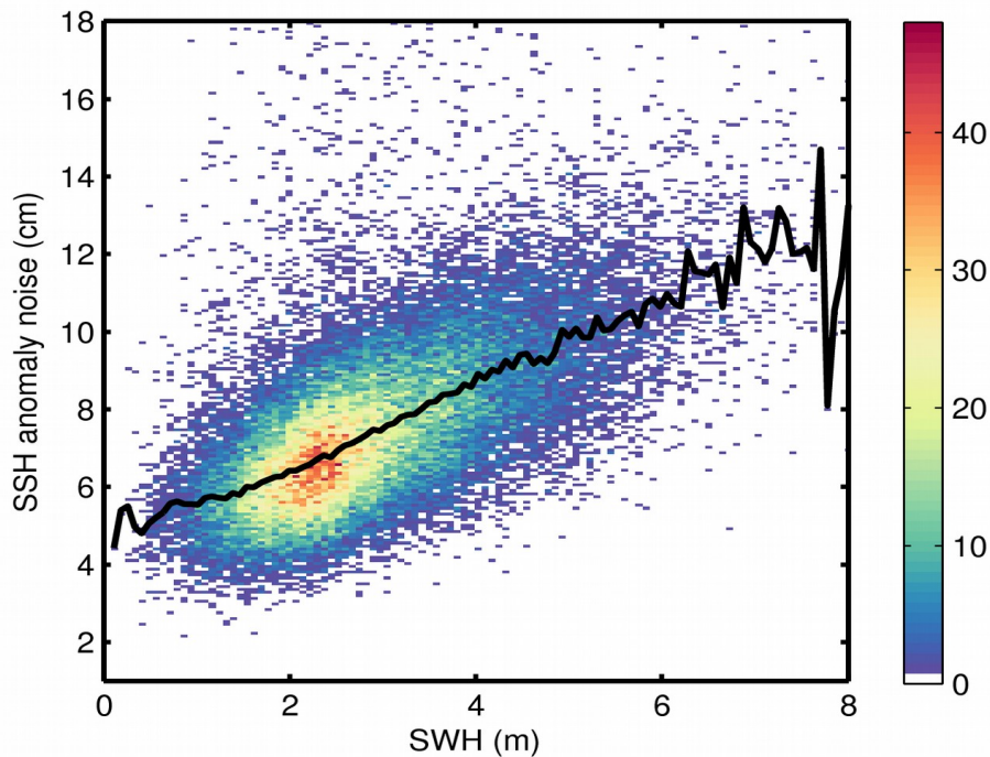
Figure 9. 2D histogram showing flag-valid SSH anomaly noise as a function of SWH for 26/01/2018. The black line denotes the median SSH anomaly noise as a function of SWH.
