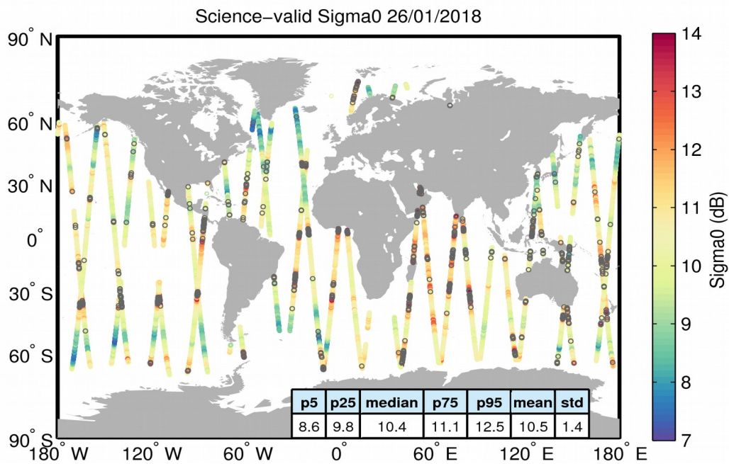
Figure 27. Geographical distribution of science-valid sigma0 data over oceans and lakes for 26/01/2018. The statistical values shown in the table refer to the sigma0 in dB and are calculated over all measurements shown in the figure. Gray circles denote records that have been rejected based on the editing criteria described in Table 4.
