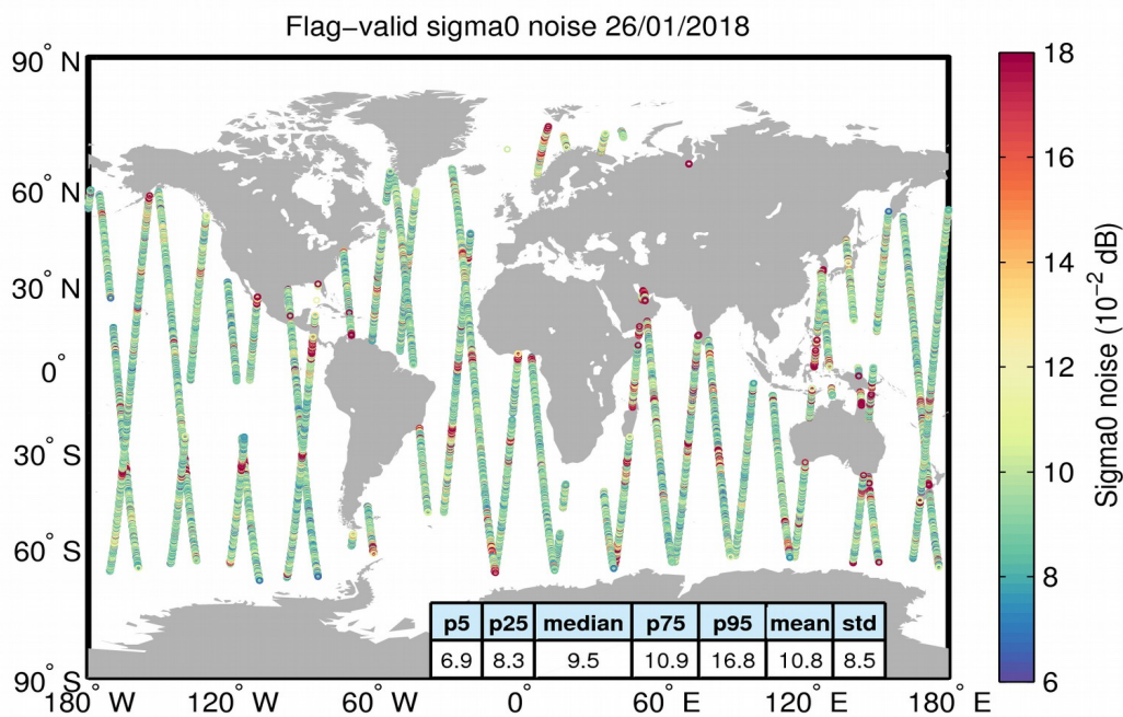
Figure 26. Geographical distribution of flag-valid 20-Hz sigma0 measurement noise over oceans and lakes for 26/01/2018. The statistical values shown in the table refer to the sigma0 noise and are calculated over all measurements shown in the figure.
