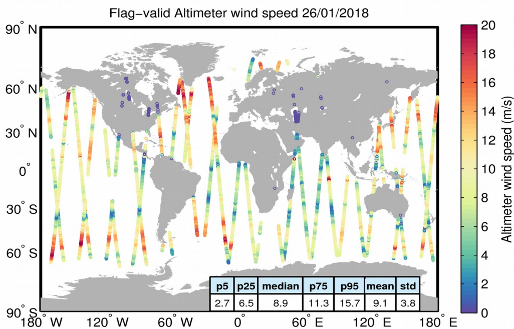
Figure 31. Geographical distribution of flag-valid wind data over oceans and lakes for 26/01/2018. The statistical values shown in the table refer to the wind in m/s and are calculated over all measurements shown in the figure.
