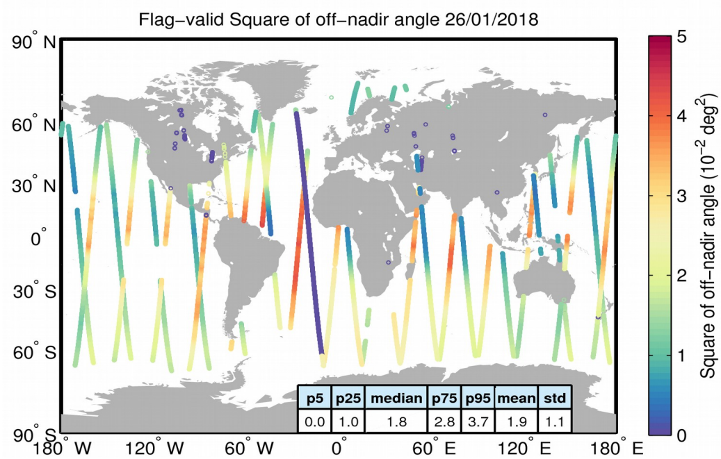
Figure 37. Geographical distribution of flag-valid mispointing data over oceans and lakes for 26/01/2018. The statistical values shown in the table refer to the mispointing in 10^{-2} \text{ deg}^2 and are calculated over all measurements shown in the figure.
