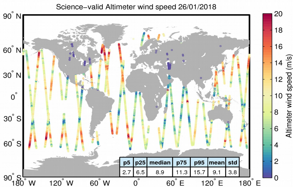
Figure 34. Geographical distribution of science-valid wind data over oceans and lakes for 26/01/2018. The statistical values shown in the table refer to the wind in m/s and are calculated over all measurements shown in the figure. Gray circles denote records that have been rejected based on the editing criteria described in Table 5.
