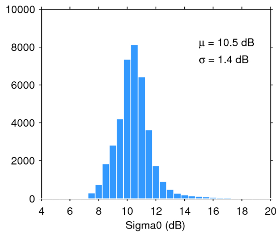
Figure 28. Histogram of science-valid sigma0 over oceans and lakes for 26/01/2018. The mean ( \mu ) and standard deviation ( \sigma ) are also shown. Note that values outside [4 20] dB are excluded from the histogram for the sake of readability but not from the computation of \mu and \sigma .
