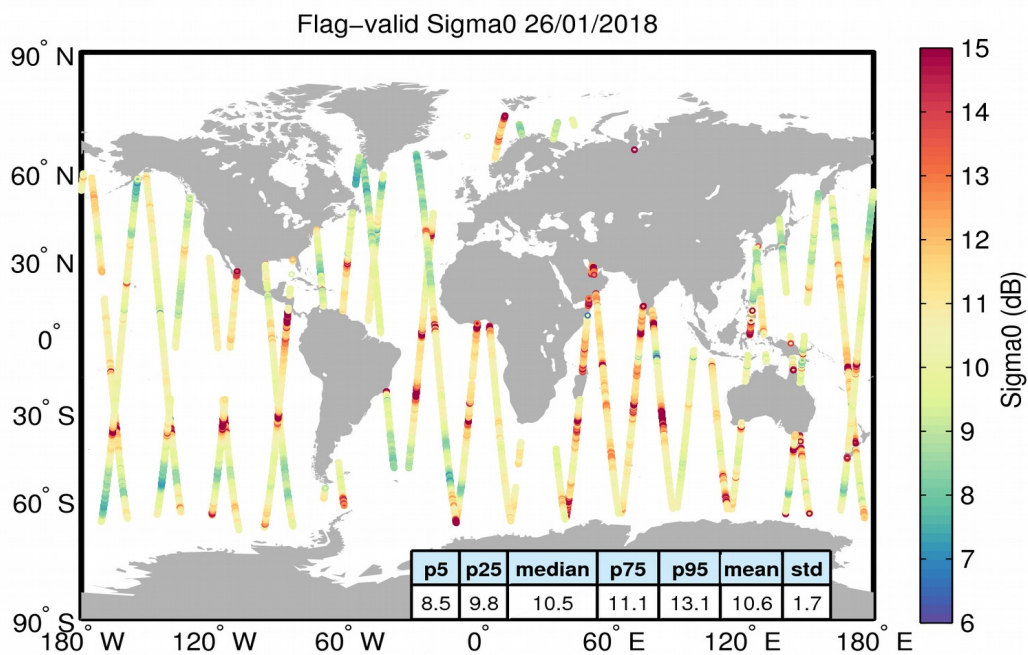
Figure 23. Geographical distribution of flag-valid sigma0 data over oceans and lakes for 26/01/2018. The statistical values shown in the table refer to the sigma0 in dB and are calculated over all measurements shown in the figure.
