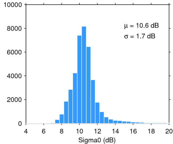
Figure 25. Histogram of flag-valid sigma0 over oceans and lakes for 26/01/2018. The mean ( \mu ) and standard deviation ( \sigma ) are also shown. Note that values outside [4 20] dB are excluded from the histogram for the sake of readability but not from the computation of \mu and \sigma .
