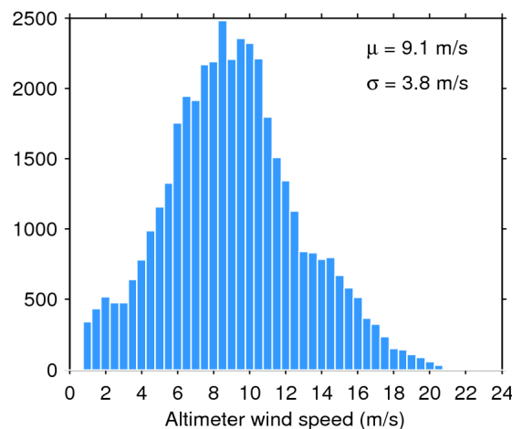
Figure 35. Histogram of science-valid wind over oceans and lakes for 26/01/2018. The mean ( \mu ) and standard deviation ( \sigma ) are also shown. Note that values larger than 24 m/s are excluded from the histogram for the sake of readability but not from the computation of \mu and \sigma .
