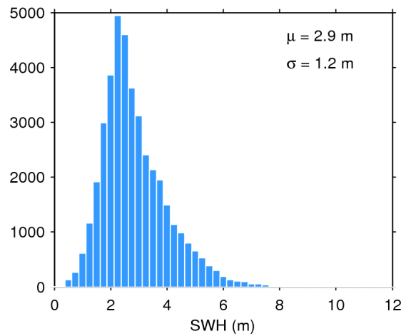
Figure 17. Histogram of flag-valid SWH over oceans and lakes for 26/01/2018. The mean ( \mu ) and standard deviation ( \sigma ) are also shown. Note that values larger than 12 m are excluded from the histogram for the sake of readability but not from the computation of \mu and \sigma .
