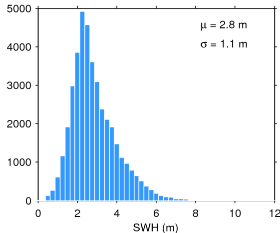
Figure 20. Histogram of science-valid SWH over oceans and lakes for 26/01/2018. The mean ( \mu ) and standard deviation ( \sigma ) are also shown. Note that values larger than 12 m are excluded from the histogram for the sake of readability but not from the computation of \mu and \sigma .
