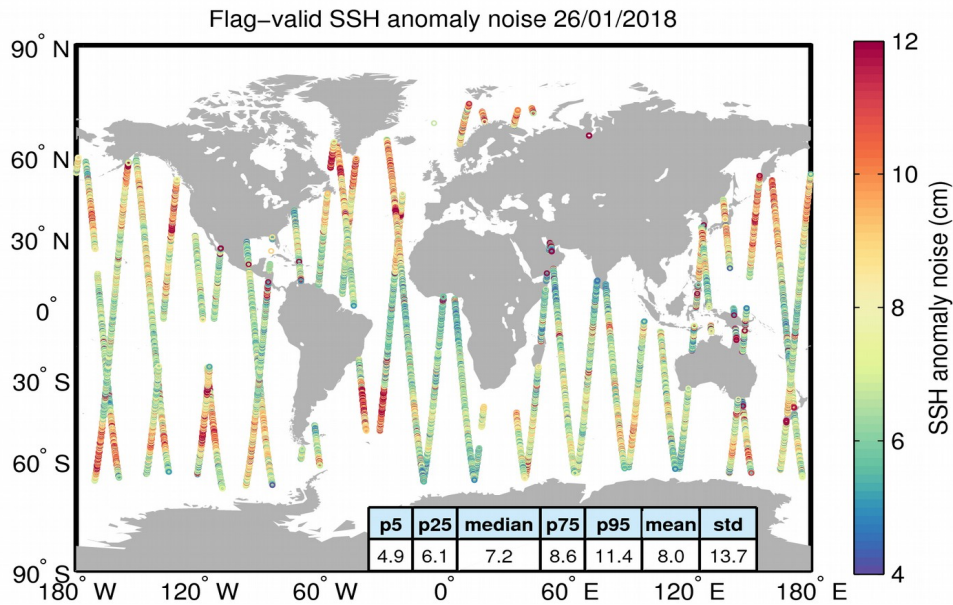
Figure 8. Geographical distribution of flag-valid 20-Hz SSH anomaly measurement noise over oceans and lakes for 26/01/2018. The statistical values shown in the table refer to the SSH anomaly noise and are calculated over all measurements shown in the figure.
