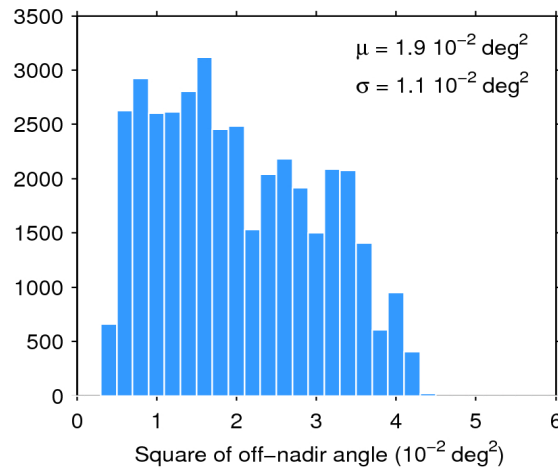
Figure 39. Histogram of flag-valid mispointing over oceans and lakes for 26/01/2018. The mean ( \mu ) and standard deviation ( \sigma ) are also shown. Note that values larger than 6 \cdot 10^{-2} \text{ deg}^2 are excluded from the histogram for the sake of readability but not from the computation of \mu and \sigma .
