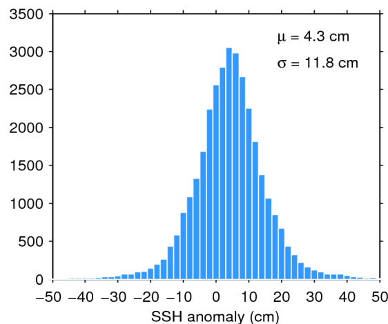
Figure 11. Histogram of science-valid SSH anomaly over oceans and lakes for 26/01/2018. The mean ( \mu ) and standard deviation ( \sigma ) are also shown. Note that values outside [-50 50] cm are excluded from the histogram for the sake of readability but not from the computation of \mu and \sigma .
