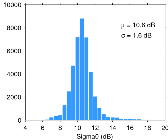
Figure 25. Histogram of flag-valid sigma0 over oceans and lakes for 25/01/2018. The mean ( \mu ) and standard deviation ( \sigma ) are also shown. Note that values outside [4 20] dB are excluded from the histogram for the sake of readability but not from the computation of \mu and \sigma .
