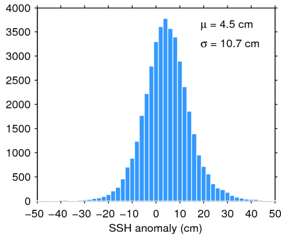
Figure 11. Histogram of science-valid SSH anomaly over oceans and lakes for 25/01/2018. The mean ( \mu ) and standard deviation ( \sigma ) are also shown. Note that values outside [-50 50] cm are excluded from the histogram for the sake of readability but not from the computation of \mu and \sigma .
