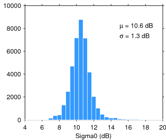
Figure 28. Histogram of science-valid sigma0 over oceans and lakes for 25/01/2018. The mean ( \mu ) and standard deviation ( \sigma ) are also shown. Note that values outside [4 20] dB are excluded from the histogram for the sake of readability but not from the computation of \mu and \sigma .
