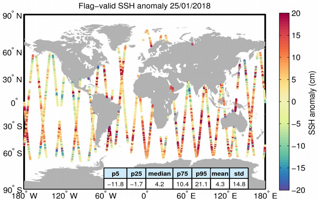
Figure 5. Geographical distribution of flag-valid 1-Hz SSH anomaly data over oceans and lakes for 25/01/2018. The statistical values shown in the table refer to the SSH anomaly in cm and are calculated over all measurements shown in the figure.
