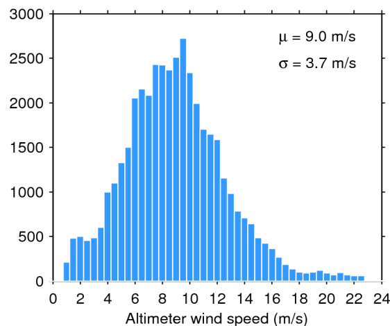
Figure 35. Histogram of science-valid wind over oceans and lakes for 25/01/2018. The mean ( \mu ) and standard deviation ( \sigma ) are also shown. Note that values larger than 24 m/s are excluded from the histogram for the sake of readability but not from the computation of \mu and \sigma .
