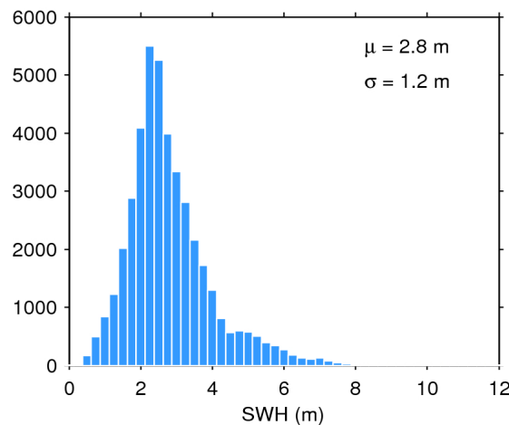
Figure 17. Histogram of flag-valid SWH over oceans and lakes for 25/01/2018. The mean ( \mu ) and standard deviation ( \sigma ) are also shown. Note that values larger than 12 m are excluded from the histogram for the sake of readability but not from the computation of \mu and \sigma .
