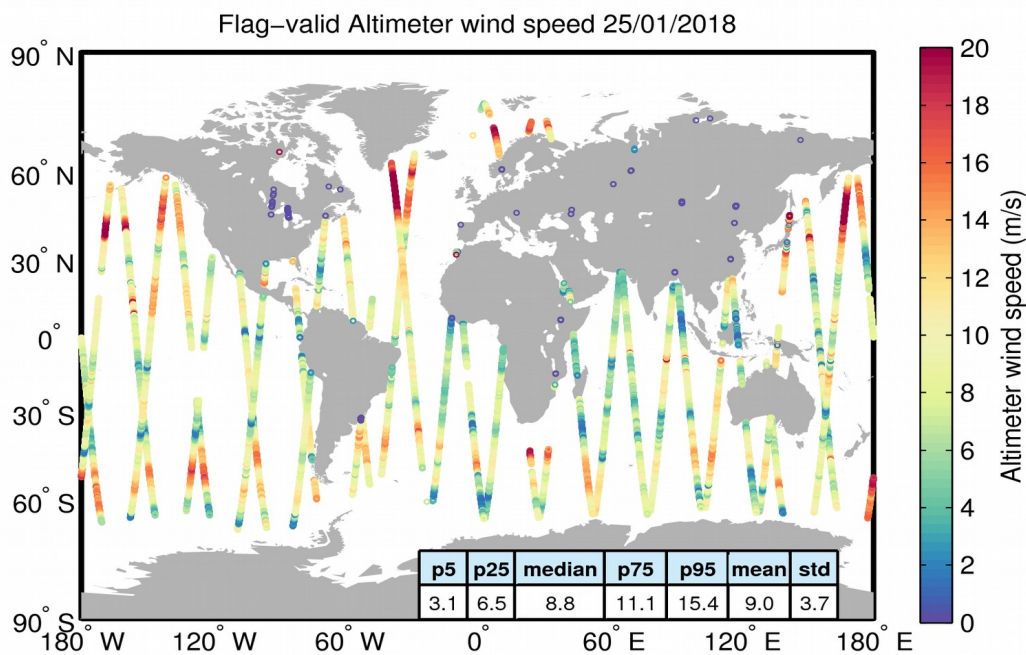
Figure 31. Geographical distribution of flag-valid wind data over oceans and lakes for 25/01/2018. The statistical values shown in the table refer to the wind in m/s and are calculated over all measurements shown in the figure.
