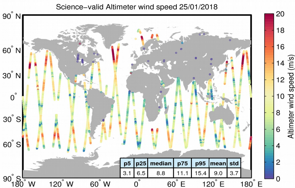
Figure 34. Geographical distribution of science-valid wind data over oceans and lakes for 25/01/2018. The statistical values shown in the table refer to the wind in m/s and are calculated over all measurements shown in the figure. Gray circles denote records that have been rejected based on the editing criteria described in Table 5.
