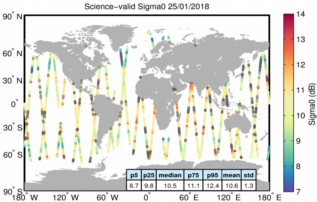
Figure 27. Geographical distribution of science-valid sigma0 data over oceans and lakes for 25/01/2018. The statistical values shown in the table refer to the sigma0 in dB and are calculated over all measurements shown in the figure. Gray circles denote records that have been rejected based on the editing criteria described in Table 4.
