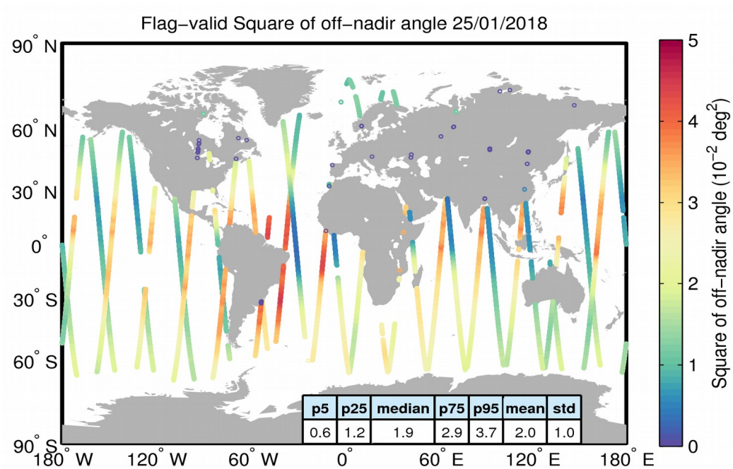
Figure 37. Geographical distribution of flag-valid mispointing data over oceans and lakes for 25/01/2018. The statistical values shown in the table refer to the mispointing in 10^{-2} \text{ deg}^2 and are calculated over all measurements shown in the figure.
