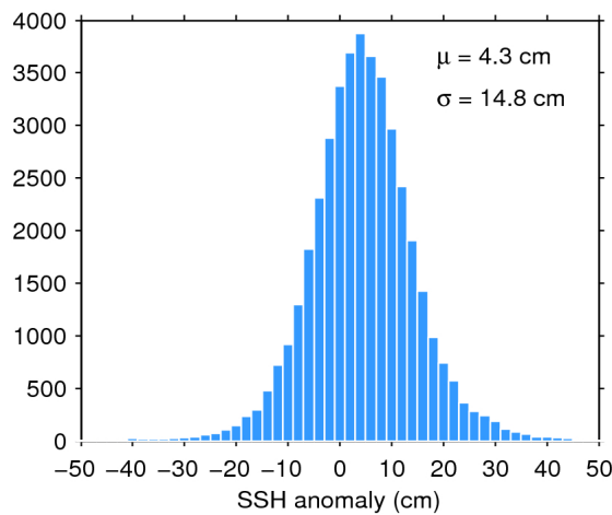
Figure 7. Histogram of flag-valid SSH anomaly over oceans and lakes for 25/01/2018. The mean ( \mu ) and standard deviation ( \sigma ) are also shown. Note that values outside [-50 50] cm are excluded from the histogram for the sake of readability but not from the computation of \mu and \sigma .
