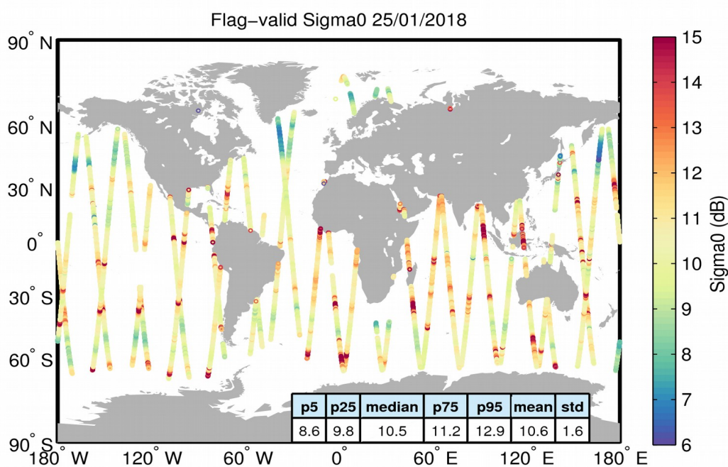
Figure 23. Geographical distribution of flag-valid sigma0 data over oceans and lakes for 25/01/2018. The statistical values shown in the table refer to the sigma0 in dB and are calculated over all measurements shown in the figure.
