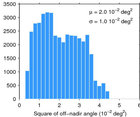
Figure 39. Histogram of flag-valid mispointing over oceans and lakes for 25/01/2018. The mean ( \mu ) and standard deviation ( \sigma ) are also shown. Note that values larger than 6 \cdot 10^{-2} \text{ deg}^2 are excluded from the histogram for the sake of readability but not from the computation of \mu and \sigma .
