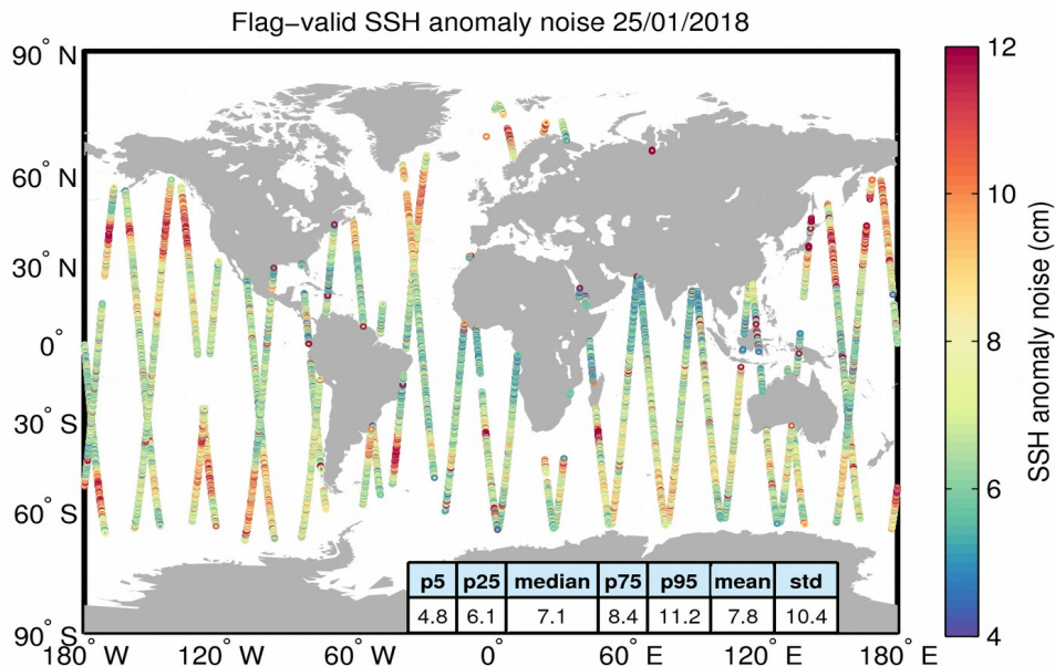
Figure 8. Geographical distribution of flag-valid 20-Hz SSH anomaly measurement noise over oceans and lakes for 25/01/2018. The statistical values shown in the table refer to the SSH anomaly noise and are calculated over all measurements shown in the figure.
