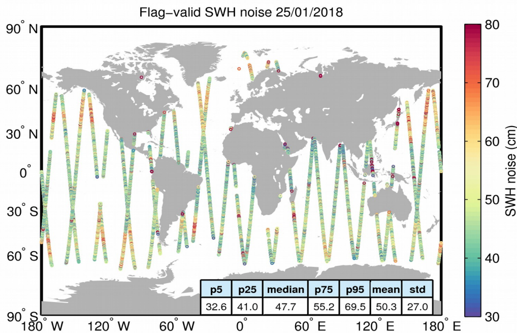
Figure 18. Geographical distribution of flag-valid 20-Hz SWH measurement noise over oceans and lakes for 25/01/2018. The statistical values shown in the figure refer to the SWH noise and are calculated over all measurements shown in the figure.
