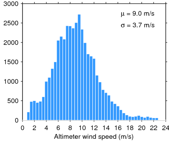
Figure 33. Histogram of flag-valid wind over oceans and lakes for 25/01/2018. The mean ( \mu ) and standard deviation ( \sigma ) are also shown. Note that values larger than 24 m/s are excluded from the histogram for the sake of readability but not from the computation of \mu and \sigma .
