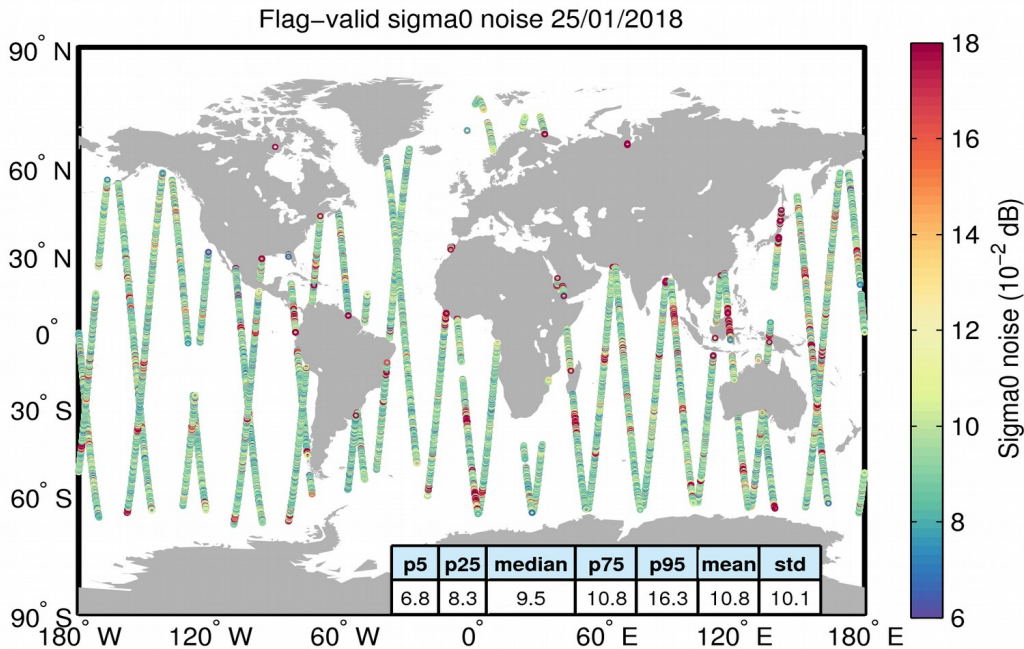
Figure 26. Geographical distribution of flag-valid 20-Hz sigma0 measurement noise over oceans and lakes for 25/01/2018. The statistical values shown in the table refer to the sigma0 noise and are calculated over all measurements shown in the figure.
