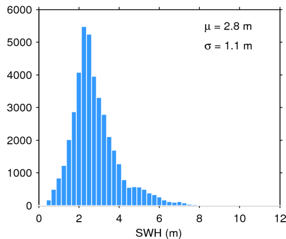
Figure 20. Histogram of science-valid SWH over oceans and lakes for 25/01/2018. The mean ( \mu ) and standard deviation ( \sigma ) are also shown. Note that values larger than 12 m are excluded from the histogram for the sake of readability but not from the computation of \mu and \sigma .
