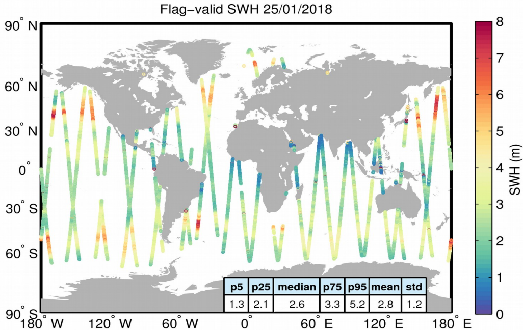
Figure 15. Geographical distribution of flag-valid SWH data over oceans and lakes for 25/01/2018. The statistical values shown in the table refer to the SWH in m and are calculated over all measurements shown in the figure.
