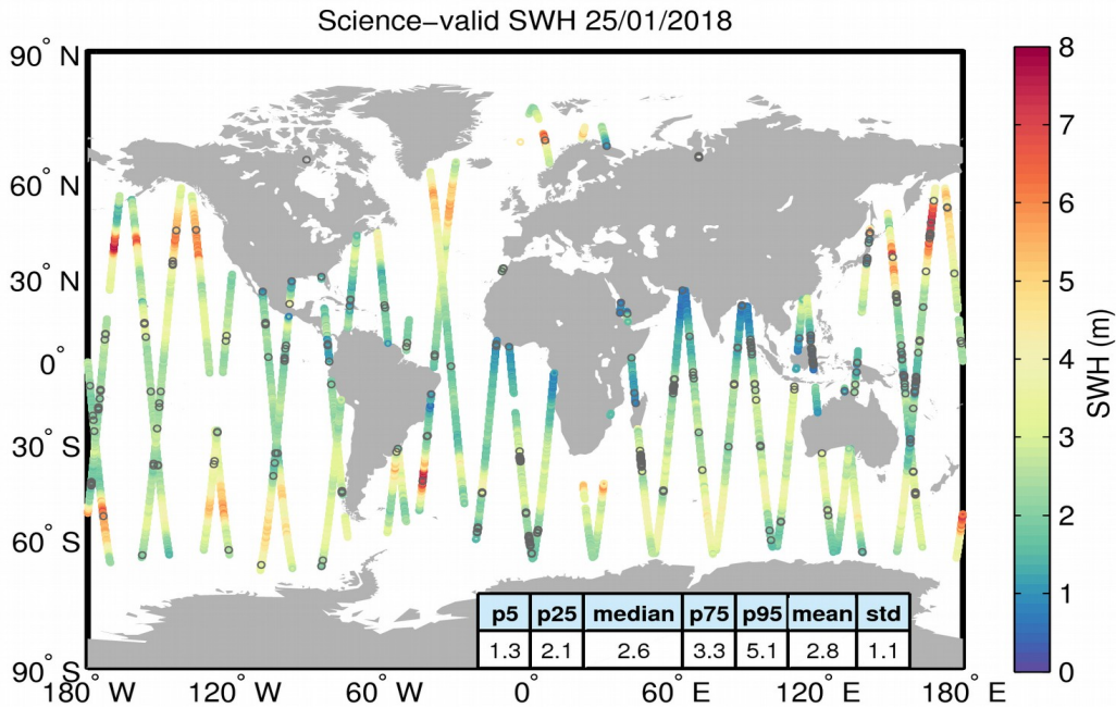
Figure 19. Geographical distribution of science-valid SWH data over oceans and lakes for 25/01/2018. The statistical values shown in the table refer to the SWH in m and are calculated over all measurements shown in the figure. Gray circles denote records that have been rejected based on the editing criteria described in Table 3.
