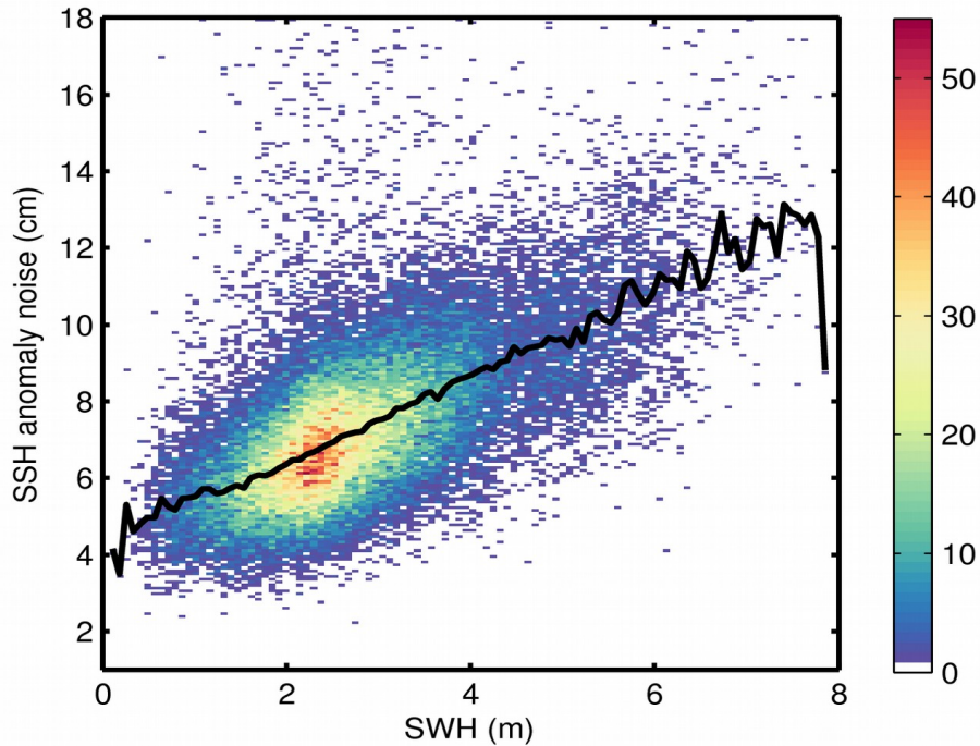
Figure 9. 2D histogram showing flag-valid SSH anomaly noise as a function of SWH for 25/01/2018. The black line denotes the median SSH anomaly noise as a function of SWH.
