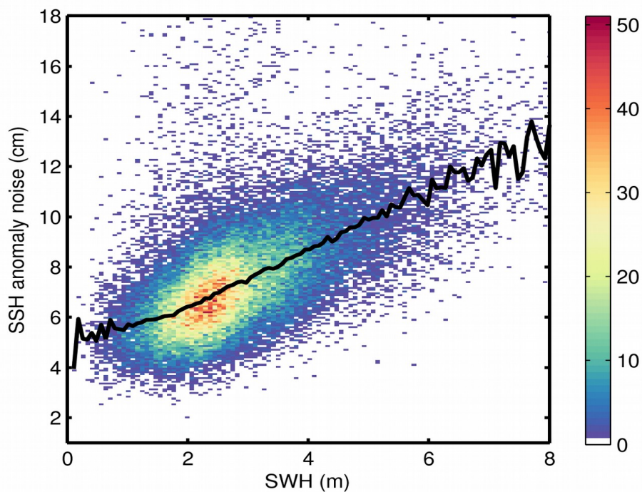
Figure 9. 2D histogram showing flag-valid SSH anomaly noise as a function of SWH for 24/01/2018. The black line denotes the median SSH anomaly noise as a function of SWH.
