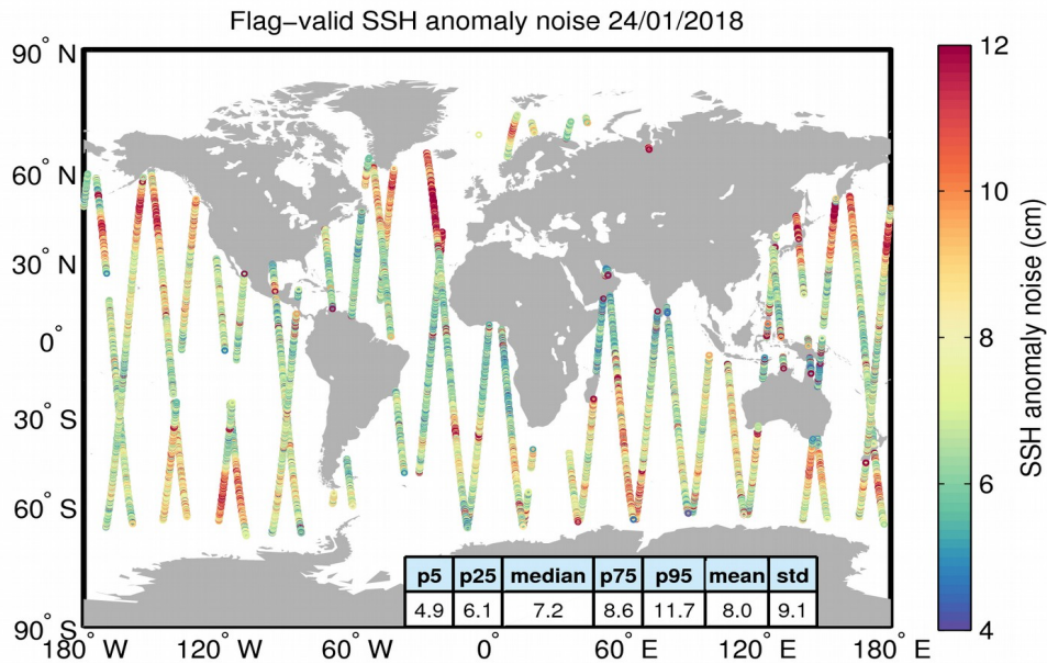
Figure 8. Geographical distribution of flag-valid 20-Hz SSH anomaly measurement noise over oceans and lakes for 24/01/2018. The statistical values shown in the table refer to the SSH anomaly noise and are calculated over all measurements shown in the figure.
