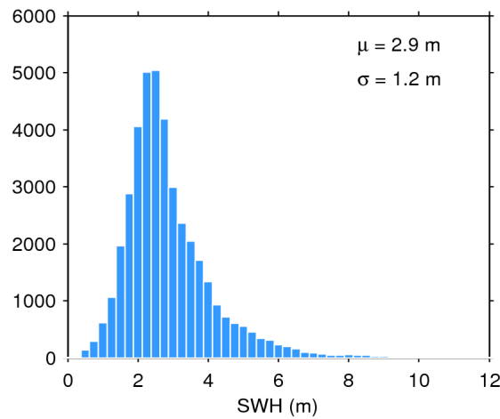
Figure 17. Histogram of flag-valid SWH over oceans and lakes for 24/01/2018. The mean ( \mu ) and standard deviation ( \sigma ) are also shown. Note that values larger than 12 m are excluded from the histogram for the sake of readability but not from the computation of \mu and \sigma .
