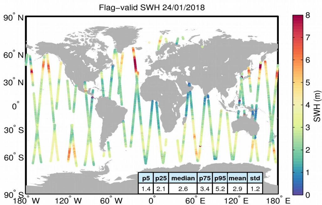
Figure 15. Geographical distribution of flag-valid SWH data over oceans and lakes for 24/01/2018. The statistical values shown in the table refer to the SWH in m and are calculated over all measurements shown in the figure.
