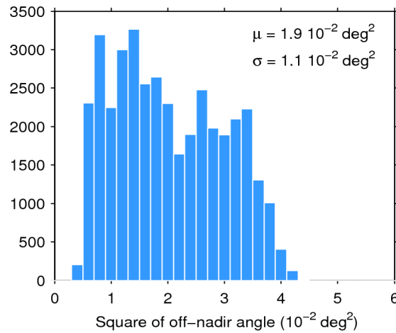
Figure 39. Histogram of flag-valid mispointing over oceans and lakes for 24/01/2018. The mean ( \mu ) and standard deviation ( \sigma ) are also shown. Note that values larger than 6 \cdot 10^{-2} \text{ deg}^2 are excluded from the histogram for the sake of readability but not from the computation of \mu and \sigma .
