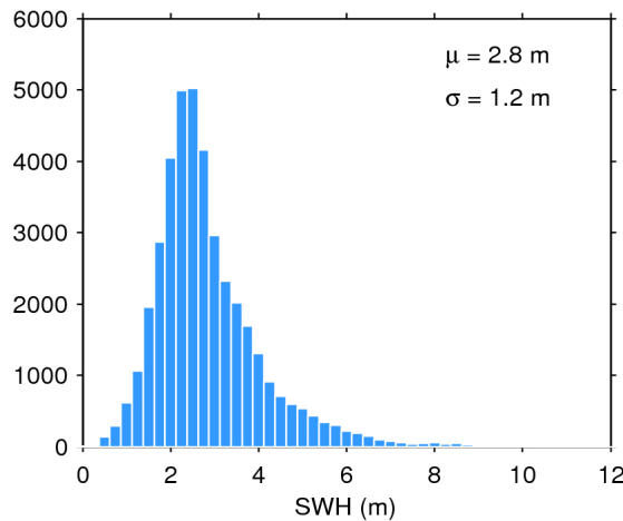
Figure 20. Histogram of science-valid SWH over oceans and lakes for 24/01/2018. The mean ( \mu ) and standard deviation ( \sigma ) are also shown. Note that values larger than 12 m are excluded from the histogram for the sake of readability but not from the computation of \mu and \sigma .
