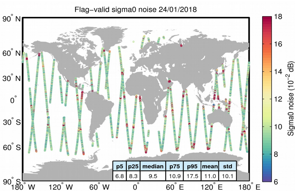
Figure 26. Geographical distribution of flag-valid 20-Hz sigma0 measurement noise over oceans and lakes for 24/01/2018. The statistical values shown in the table refer to the sigma0 noise and are calculated over all measurements shown in the figure.
