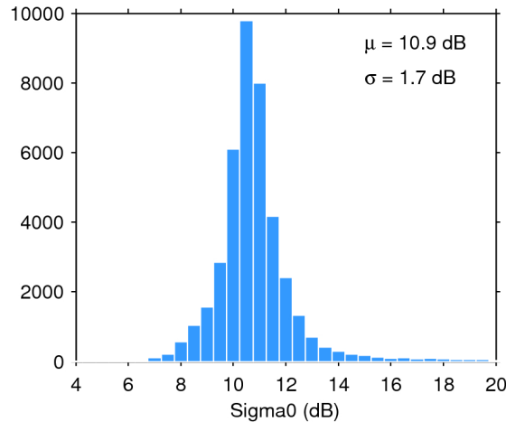
Figure 25. Histogram of flag-valid sigma0 over oceans and lakes for 24/01/2018. The mean ( \mu ) and standard deviation ( \sigma ) are also shown. Note that values outside [4 20] dB are excluded from the histogram for the sake of readability but not from the computation of \mu and \sigma .
