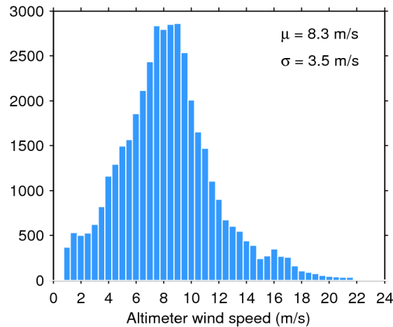
Figure 33. Histogram of flag-valid wind over oceans and lakes for 24/01/2018. The mean ( \mu ) and standard deviation ( \sigma ) are also shown. Note that values larger than 24 m/s are excluded from the histogram for the sake of readability but not from the computation of \mu and \sigma .
