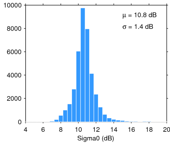
Figure 28. Histogram of science-valid sigma0 over oceans and lakes for 24/01/2018. The mean ( \mu ) and standard deviation ( \sigma ) are also shown. Note that values outside [4 20] dB are excluded from the histogram for the sake of readability but not from the computation of \mu and \sigma .
