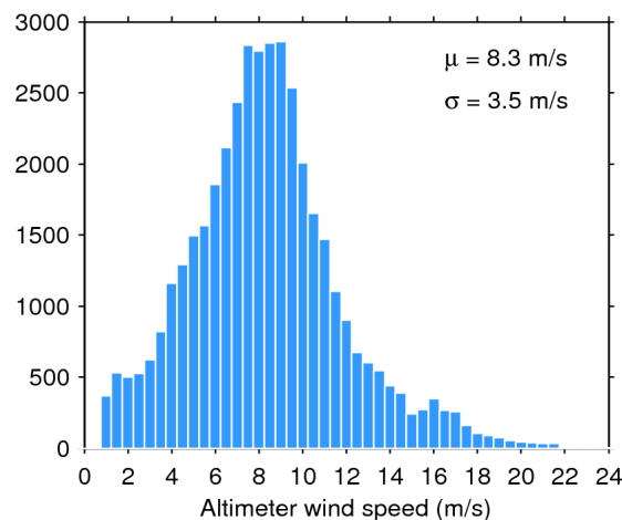
Figure 35. Histogram of science-valid wind over oceans and lakes for 24/01/2018. The mean ( \mu ) and standard deviation ( \sigma ) are also shown. Note that values larger than 24 m/s are excluded from the histogram for the sake of readability but not from the computation of \mu and \sigma .
