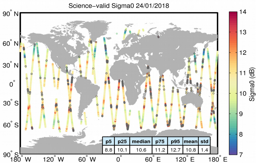
Figure 27. Geographical distribution of science-valid sigma0 data over oceans and lakes for 24/01/2018. The statistical values shown in the table refer to the sigma0 in dB and are calculated over all measurements shown in the figure. Gray circles denote records that have been rejected based on the editing criteria described in Table 4.
