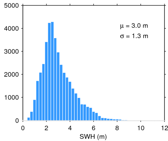
Figure 17. Histogram of flag-valid SWH over oceans and lakes for 21/01/2018. The mean ( \mu ) and standard deviation ( \sigma ) are also shown. Note that values larger than 12 m are excluded from the histogram for the sake of readability but not from the computation of \mu and \sigma .
