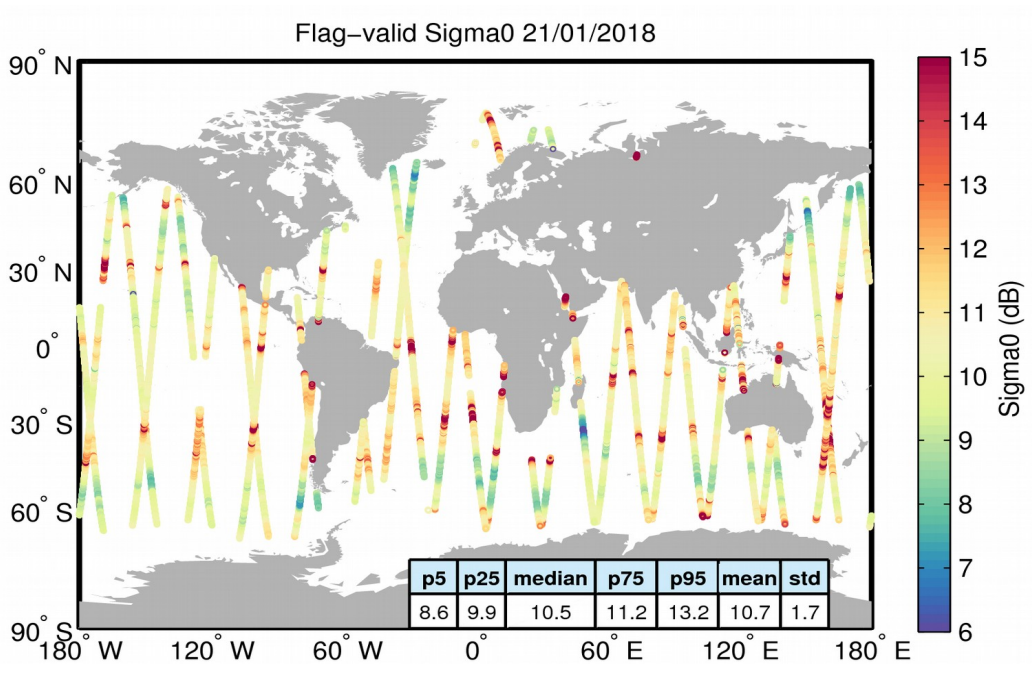
Figure 23. Geographical distribution of flag-valid sigma0 data over oceans and lakes for 21/01/2018. The statistical values shown in the table refer to the sigma0 in dB and are calculated over all measurements shown in the figure.
