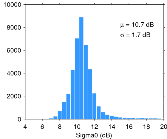
Figure 25. Histogram of flag-valid sigma0 over oceans and lakes for 21/01/2018. The mean ( \mu ) and standard deviation ( \sigma ) are also shown. Note that values outside [4 20] dB are excluded from the histogram for the sake of readability but not from the computation of \mu and \sigma .
