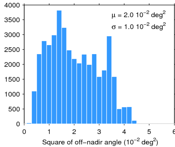
Figure 39. Histogram of flag-valid mispointing over oceans and lakes for 21/01/2018. The mean ( \mu ) and standard deviation ( \sigma ) are also shown. Note that values larger than 6 \cdot 10^{-2} \text{ deg}^2 are excluded from the histogram for the sake of readability but not from the computation of \mu and \sigma .
