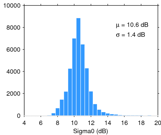
Figure 28. Histogram of science-valid sigma0 over oceans and lakes for 21/01/2018. The mean ( \mu ) and standard deviation ( \sigma ) are also shown. Note that values outside [4 20] dB are excluded from the histogram for the sake of readability but not from the computation of \mu and \sigma .
