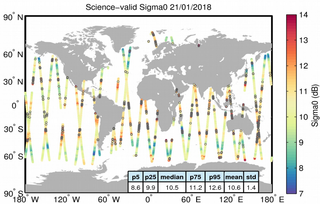
Figure 27. Geographical distribution of science-valid sigma0 data over oceans and lakes for 21/01/2018. The statistical values shown in the table refer to the sigma0 in dB and are calculated over all measurements shown in the figure. Gray circles denote records that have been rejected based on the editing criteria described in Table 4.
