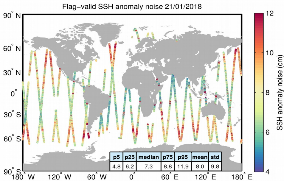
Figure 8. Geographical distribution of flag-valid 20-Hz SSH anomaly measurement noise over oceans and lakes for 21/01/2018. The statistical values shown in the table refer to the SSH anomaly noise and are calculated over all measurements shown in the figure.
