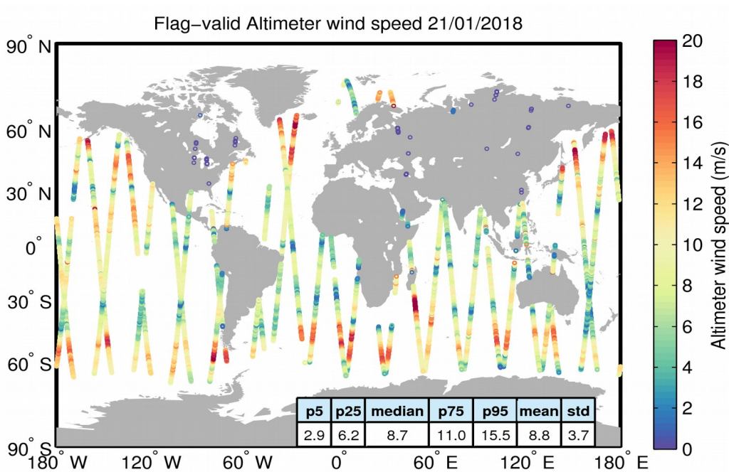
Figure 31. Geographical distribution of flag-valid wind data over oceans and lakes for 21/01/2018. The statistical values shown in the table refer to the wind in m/s and are calculated over all measurements shown in the figure.
