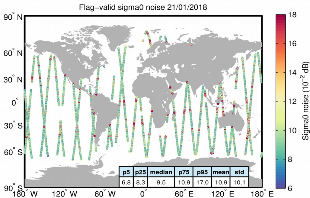
Figure 26. Geographical distribution of flag-valid 20-Hz sigma0 measurement noise over oceans and lakes for 21/01/2018. The statistical values shown in the table refer to the sigma0 noise and are calculated over all measurements shown in the figure.
