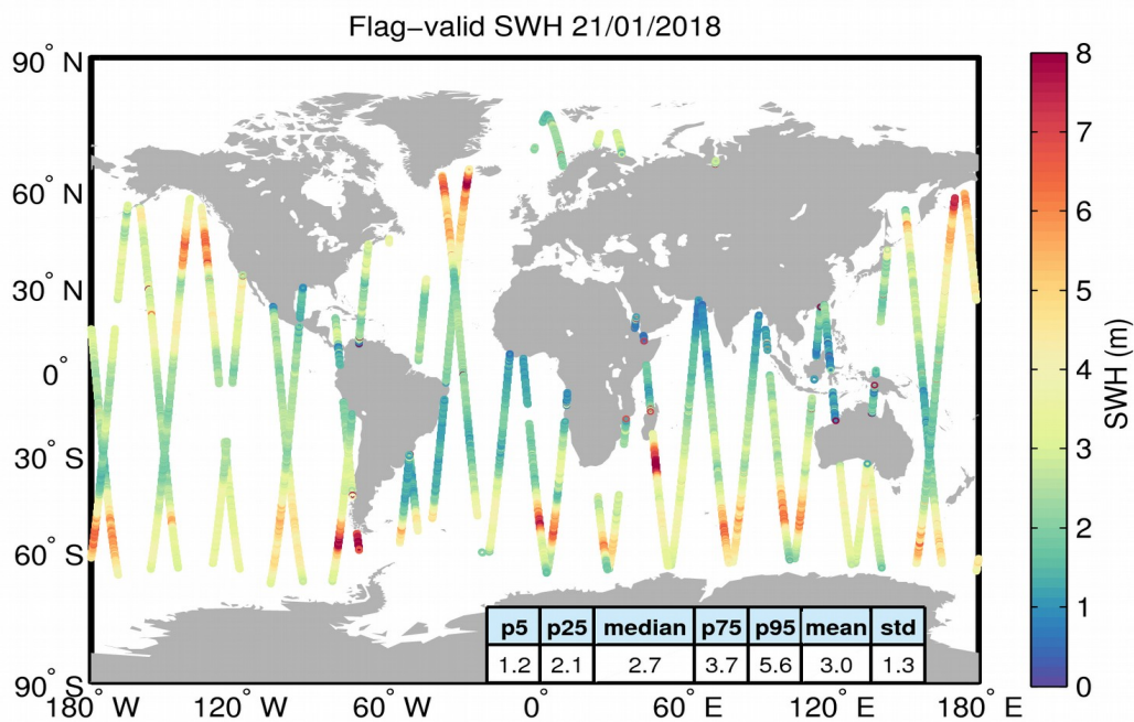
Figure 15. Geographical distribution of flag-valid SWH data over oceans and lakes for 21/01/2018. The statistical values shown in the table refer to the SWH in m and are calculated over all measurements shown in the figure.
