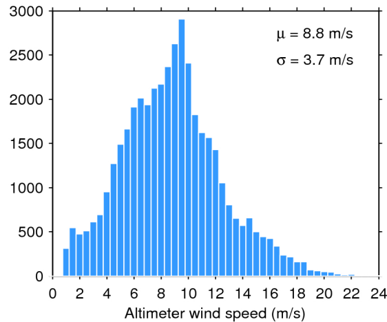
Figure 33. Histogram of flag-valid wind over oceans and lakes for 21/01/2018. The mean ( \mu ) and standard deviation ( \sigma ) are also shown. Note that values larger than 24 m/s are excluded from the histogram for the sake of readability but not from the computation of \mu and \sigma .
