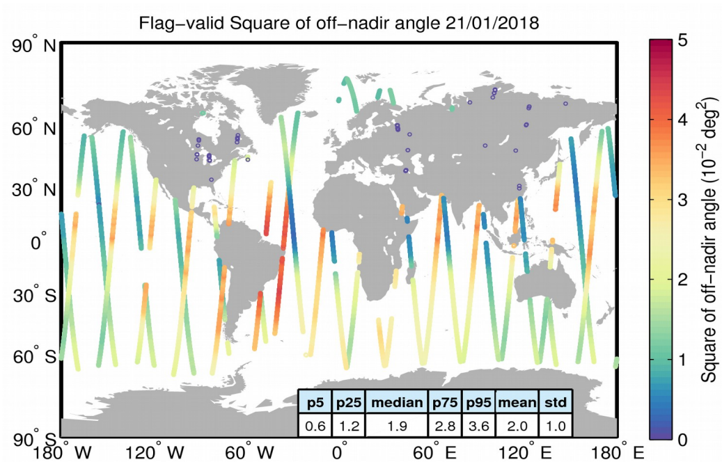
Figure 37. Geographical distribution of flag-valid mispointing data over oceans and lakes for 21/01/2018. The statistical values shown in the table refer to the mispointing in 10^{-2} \text{ deg}^2 and are calculated over all measurements shown in the figure.
