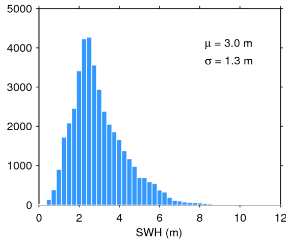
Figure 20. Histogram of science-valid SWH over oceans and lakes for 21/01/2018. The mean ( \mu ) and standard deviation ( \sigma ) are also shown. Note that values larger than 12 m are excluded from the histogram for the sake of readability but not from the computation of \mu and \sigma .
