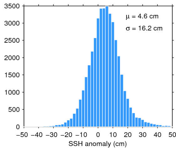
Figure 7. Histogram of flag-valid SSH anomaly over oceans and lakes for 21/01/2018. The mean ( \mu ) and standard deviation ( \sigma ) are also shown. Note that values outside [-50 50] cm are excluded from the histogram for the sake of readability but not from the computation of \mu and \sigma .
