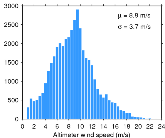
Figure 35. Histogram of science-valid wind over oceans and lakes for 21/01/2018. The mean ( \mu ) and standard deviation ( \sigma ) are also shown. Note that values larger than 24 m/s are excluded from the histogram for the sake of readability but not from the computation of \mu and \sigma .
