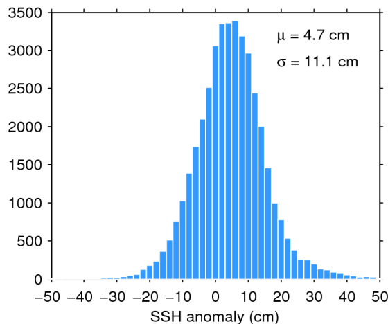
Figure 11. Histogram of science-valid SSH anomaly over oceans and lakes for 21/01/2018. The mean ( \mu ) and standard deviation ( \sigma ) are also shown. Note that values outside [-50 50] cm are excluded from the histogram for the sake of readability but not from the computation of \mu and \sigma .
