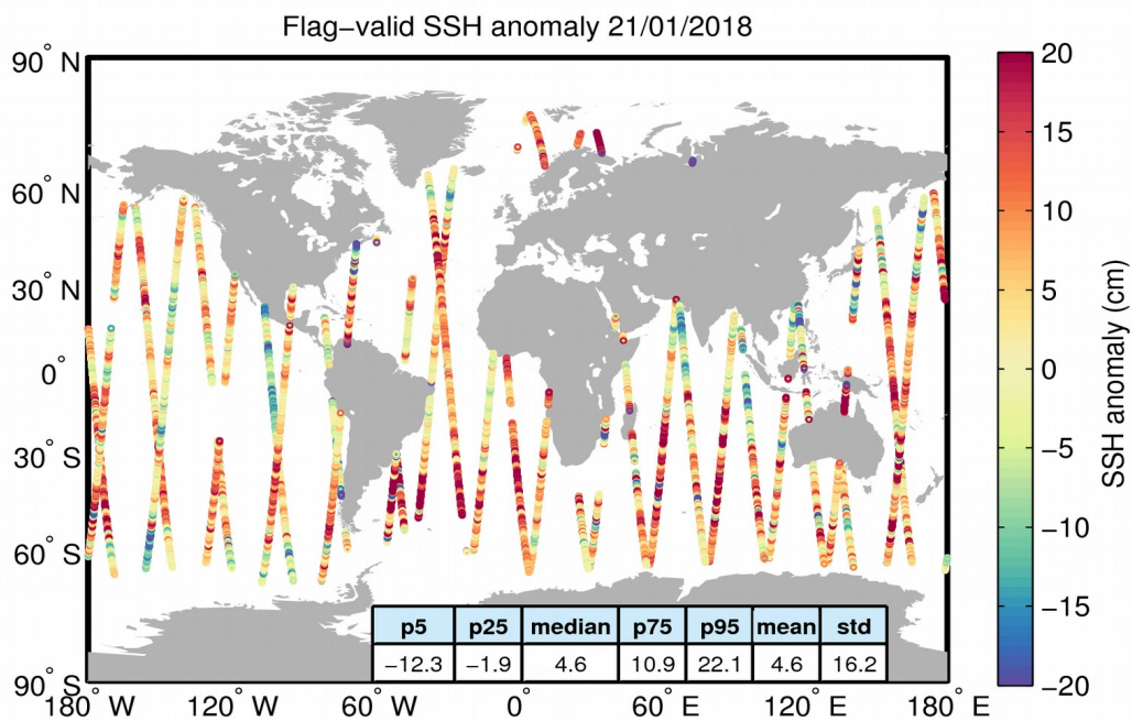
Figure 5. Geographical distribution of flag-valid 1-Hz SSH anomaly data over oceans and lakes for 21/01/2018. The statistical values shown in the table refer to the SSH anomaly in cm and are calculated over all measurements shown in the figure.
