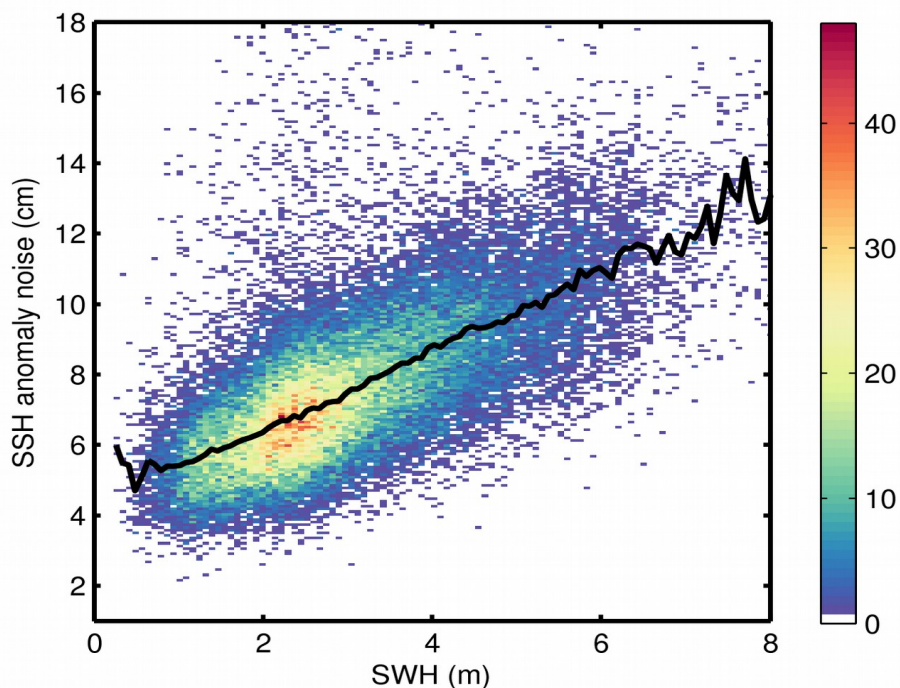
Figure 9. 2D histogram showing flag-valid SSH anomaly noise as a function of SWH for 21/01/2018. The black line denotes the median SSH anomaly noise as a function of SWH.
