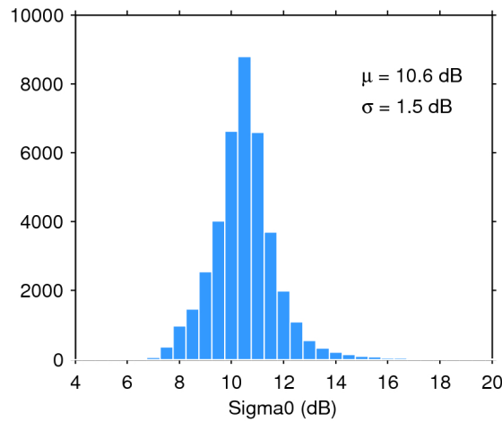
Figure 28. Histogram of science-valid sigma0 over oceans and lakes for 20/01/2018. The mean ( \mu ) and standard deviation ( \sigma ) are also shown. Note that values outside [4 20] dB are excluded from the histogram for the sake of readability but not from the computation of \mu and \sigma .
