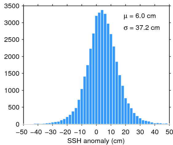
Figure 7. Histogram of flag-valid SSH anomaly over oceans and lakes for 20/01/2018. The mean ( \mu ) and standard deviation ( \sigma ) are also shown. Note that values outside [-50\ 50] cm are excluded from the histogram for the sake of readability but not from the computation of \mu and \sigma .
