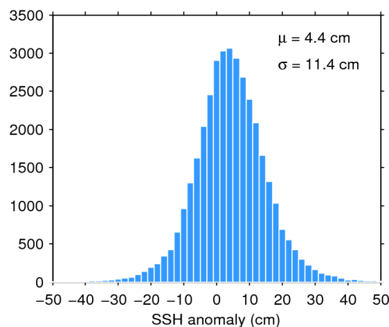
Figure 11. Histogram of science-valid SSH anomaly over oceans and lakes for 20/01/2018. The mean ( \mu ) and standard deviation ( \sigma ) are also shown. Note that values outside [-50 50] cm are excluded from the histogram for the sake of readability but not from the computation of \mu and \sigma .
