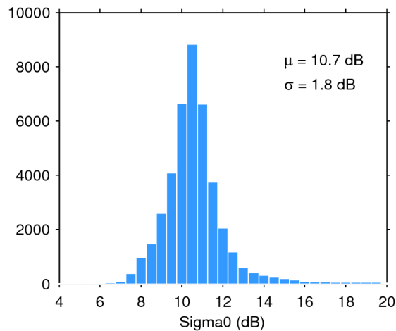
Figure 25. Histogram of flag-valid sigma0 over oceans and lakes for 20/01/2018. The mean ( \mu ) and standard deviation ( \sigma ) are also shown. Note that values outside [4 20] dB are excluded from the histogram for the sake of readability but not from the computation of \mu and \sigma .
