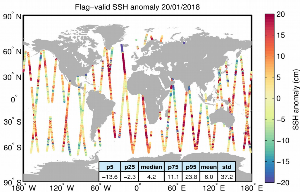
Figure 5. Geographical distribution of flag-valid 1-Hz SSH anomaly data over oceans and lakes for 20/01/2018. The statistical values shown in the table refer to the SSH anomaly in cm and are calculated over all measurements shown in the figure.
