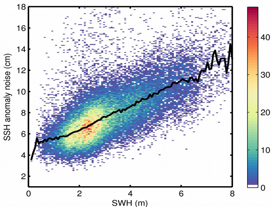
Figure 9. 2D histogram showing flag-valid SSH anomaly noise as a function of SWH for 20/01/2018. The black line denotes the median SSH anomaly noise as a function of SWH.
