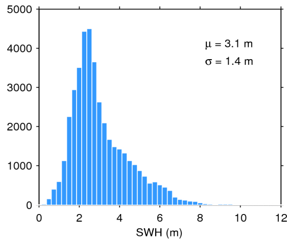
Figure 17. Histogram of flag-valid SWH over oceans and lakes for 20/01/2018. The mean ( \mu ) and standard deviation ( \sigma ) are also shown. Note that values larger than 12 m are excluded from the histogram for the sake of readability but not from the computation of \mu and \sigma .
