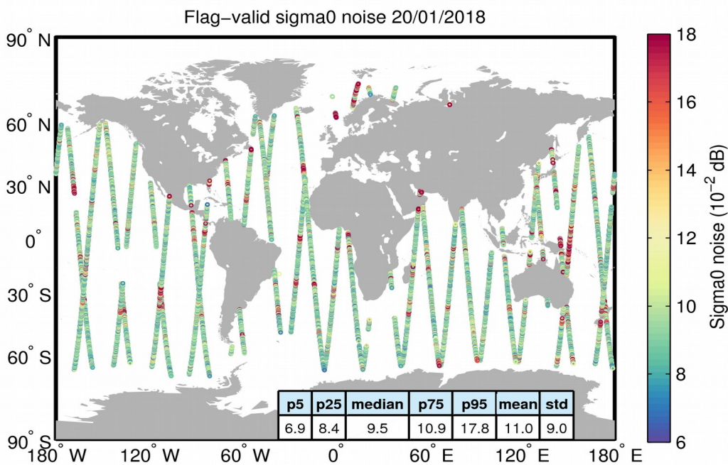
Figure 26. Geographical distribution of flag-valid 20-Hz sigma0 measurement noise over oceans and lakes for 20/01/2018. The statistical values shown in the table refer to the sigma0 noise and are calculated over all measurements shown in the figure.
