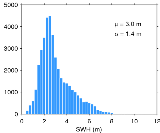
Figure 20. Histogram of science-valid SWH over oceans and lakes for 20/01/2018. The mean ( \mu ) and standard deviation ( \sigma ) are also shown. Note that values larger than 12 m are excluded from the histogram for the sake of readability but not from the computation of \mu and \sigma .
