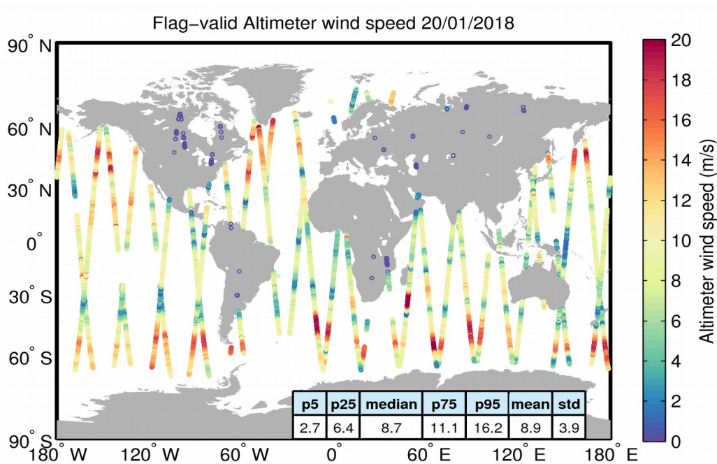
Figure 31. Geographical distribution of flag-valid wind data over oceans and lakes for 20/01/2018. The statistical values shown in the table refer to the wind in m/s and are calculated over all measurements shown in the figure.
