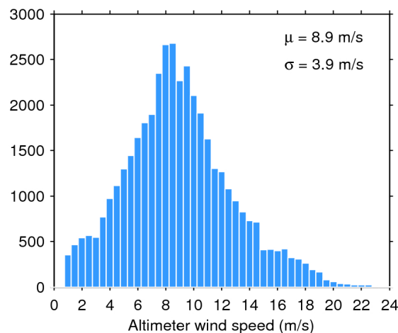
Figure 35. Histogram of science-valid wind over oceans and lakes for 20/01/2018. The mean ( \mu ) and standard deviation ( \sigma ) are also shown. Note that values larger than 24 m/s are excluded from the histogram for the sake of readability but not from the computation of \mu and \sigma .
