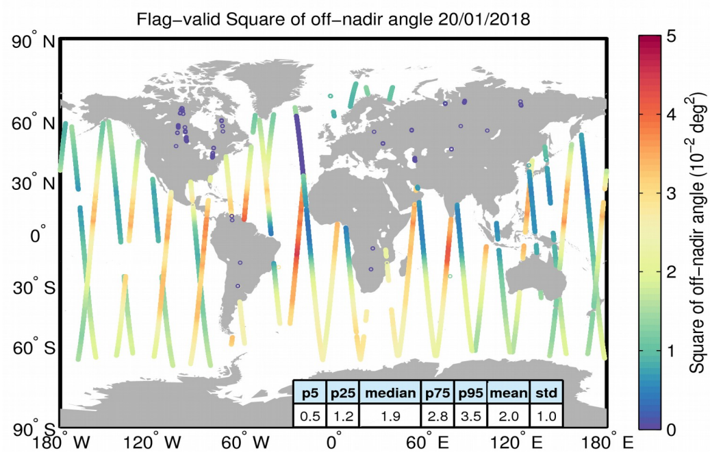
Figure 37. Geographical distribution of flag-valid mispointing data over oceans and lakes for 20/01/2018. The statistical values shown in the table refer to the mispointing in 10^{-2} deg 2 and are calculated over all measurements shown in the figure.
