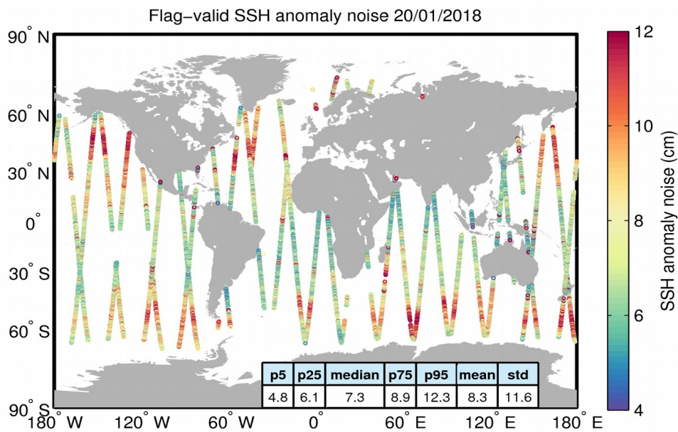
Figure 8. Geographical distribution of flag-valid 20-Hz SSH anomaly measurement noise over oceans and lakes for 20/01/2018. The statistical values shown in the table refer to the SSH anomaly noise and are calculated over all measurements shown in the figure.
