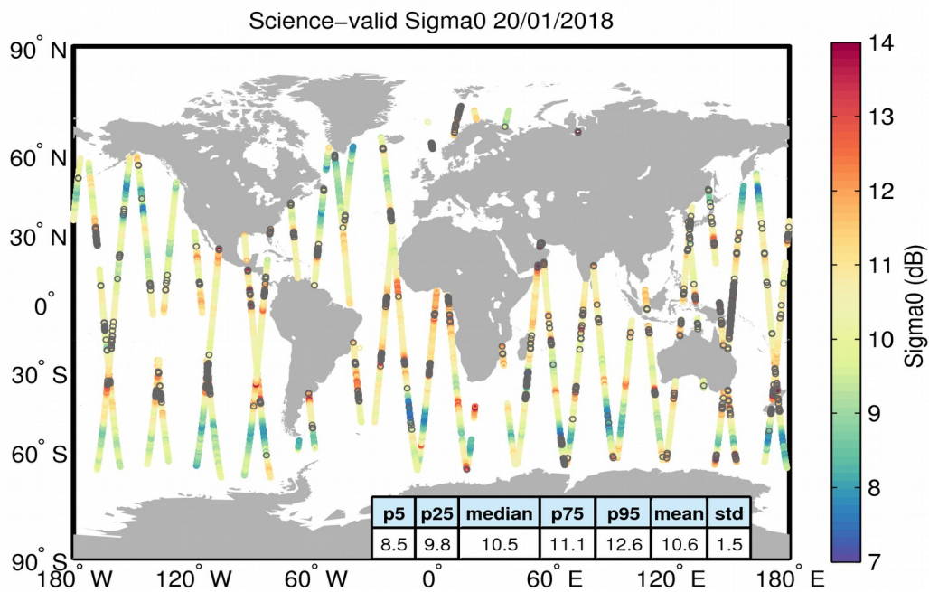
Figure 27. Geographical distribution of science-valid sigma0 data over oceans and lakes for 20/01/2018. The statistical values shown in the table refer to the sigma0 in dB and are calculated over all measurements shown in the figure. Gray circles denote records that have been rejected based on the editing criteria described in Table 4.
