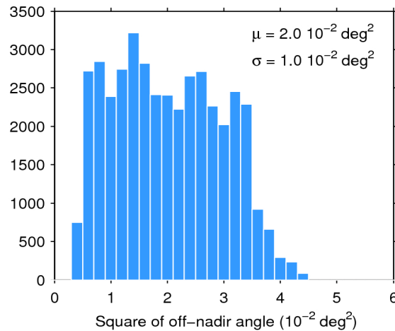
Figure 39. Histogram of flag-valid mispointing over oceans and lakes for 20/01/2018. The mean ( \mu ) and standard deviation ( \sigma ) are also shown. Note that values larger than 6 \cdot 10^{-2} \text{ deg}^2 are excluded from the histogram for the sake of readability but not from the computation of \mu and \sigma .
