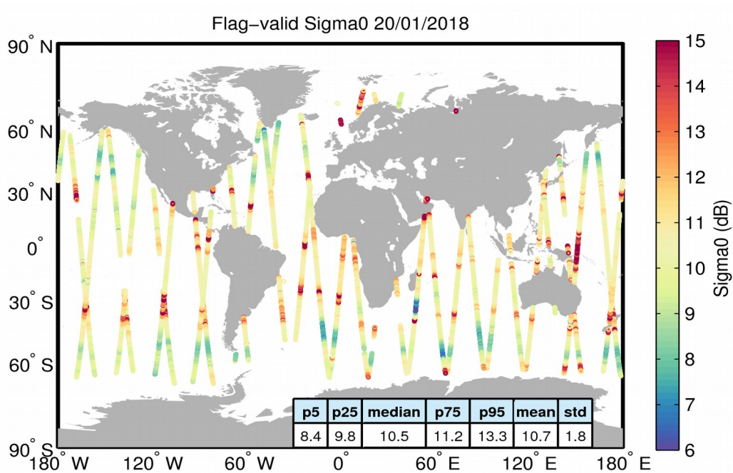
Figure 23. Geographical distribution of flag-valid sigma0 data over oceans and lakes for 20/01/2018. The statistical values shown in the table refer to the sigma0 in dB and are calculated over all measurements shown in the figure.
