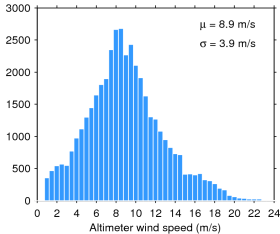
Figure 33. Histogram of flag-valid wind over oceans and lakes for 20/01/2018. The mean ( \mu ) and standard deviation ( \sigma ) are also shown. Note that values larger than 24 m/s are excluded from the histogram for the sake of readability but not from the computation of \mu and \sigma .
