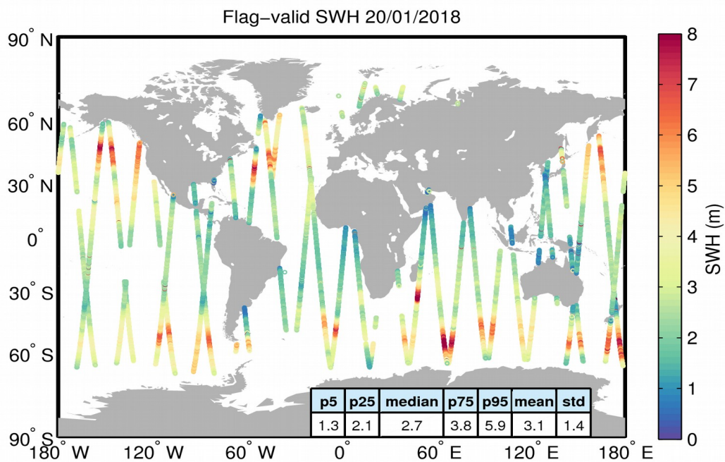
Figure 15. Geographical distribution of flag-valid SWH data over oceans and lakes for 20/01/2018. The statistical values shown in the table refer to the SWH in m and are calculated over all measurements shown in the figure.
