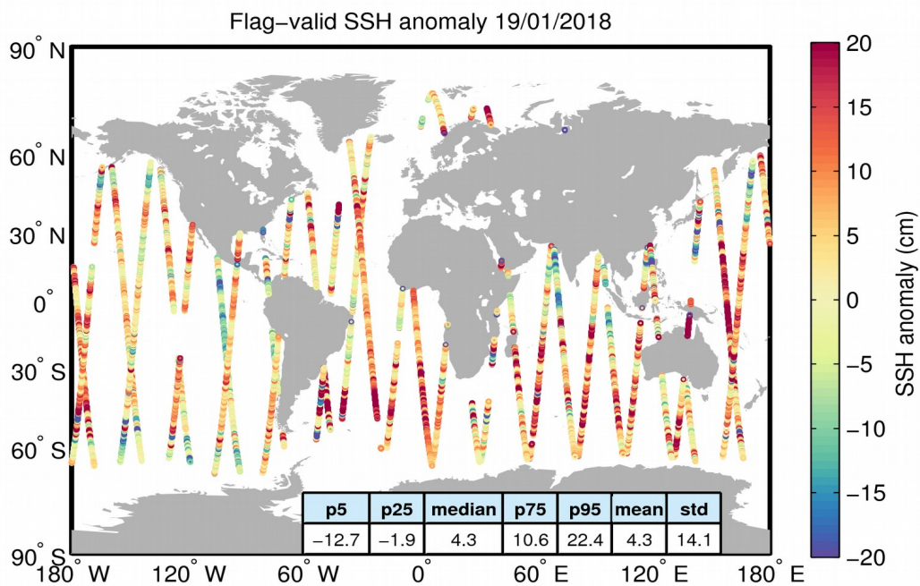
Figure 5. Geographical distribution of flag-valid 1-Hz SSH anomaly data over oceans and lakes for 19/01/2018. The statistical values shown in the table refer to the SSH anomaly in cm and are calculated over all measurements shown in the figure.
