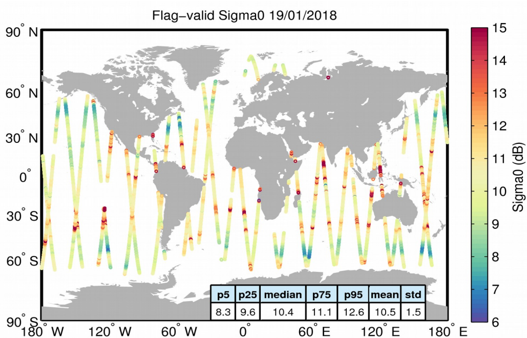
Figure 23. Geographical distribution of flag-valid sigma0 data over oceans and lakes for 19/01/2018. The statistical values shown in the table refer to the sigma0 in dB and are calculated over all measurements shown in the figure.
