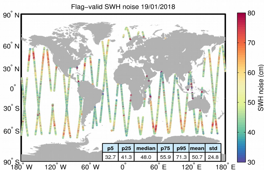
Figure 18. Geographical distribution of flag-valid 20-Hz SWH measurement noise over oceans and lakes for 19/01/2018. The statistical values shown in the figure refer to the SWH noise and are calculated over all measurements shown in the figure.
