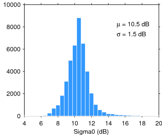
Figure 25. Histogram of flag-valid sigma0 over oceans and lakes for 19/01/2018. The mean ( \mu ) and standard deviation ( \sigma ) are also shown. Note that values outside [4 20] dB are excluded from the histogram for the sake of readability but not from the computation of \mu and \sigma .
