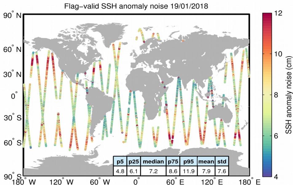
Figure 8. Geographical distribution of flag-valid 20-Hz SSH anomaly measurement noise over oceans and lakes for 19/01/2018. The statistical values shown in the table refer to the SSH anomaly noise and are calculated over all measurements shown in the figure.
