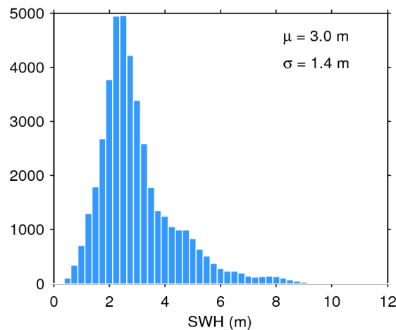
Figure 17. Histogram of flag-valid SWH over oceans and lakes for 19/01/2018. The mean ( \mu ) and standard deviation ( \sigma ) are also shown. Note that values larger than 12 m are excluded from the histogram for the sake of readability but not from the computation of \mu and \sigma .
