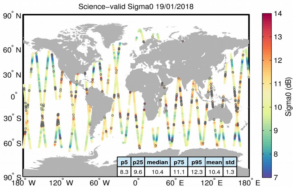
Figure 27. Geographical distribution of science-valid sigma0 data over oceans and lakes for 19/01/2018. The statistical values shown in the table refer to the sigma0 in dB and are calculated over all measurements shown in the figure. Gray circles denote records that have been rejected based on the editing criteria described in Table 4.
