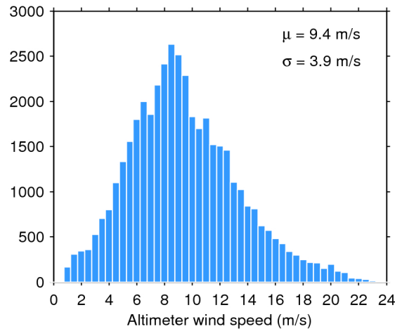
Figure 33. Histogram of flag-valid wind over oceans and lakes for 19/01/2018. The mean ( \mu ) and standard deviation ( \sigma ) are also shown. Note that values larger than 24 m/s are excluded from the histogram for the sake of readability but not from the computation of \mu and \sigma .
