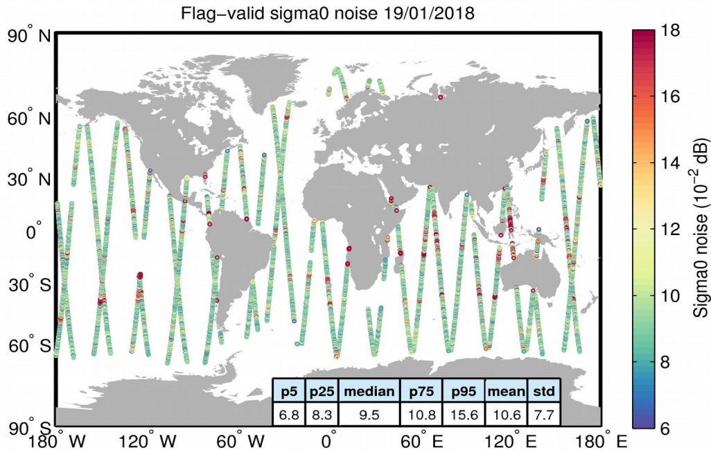
Figure 26. Geographical distribution of flag-valid 20-Hz sigma0 measurement noise over oceans and lakes for 19/01/2018. The statistical values shown in the table refer to the sigma0 noise and are calculated over all measurements shown in the figure.
