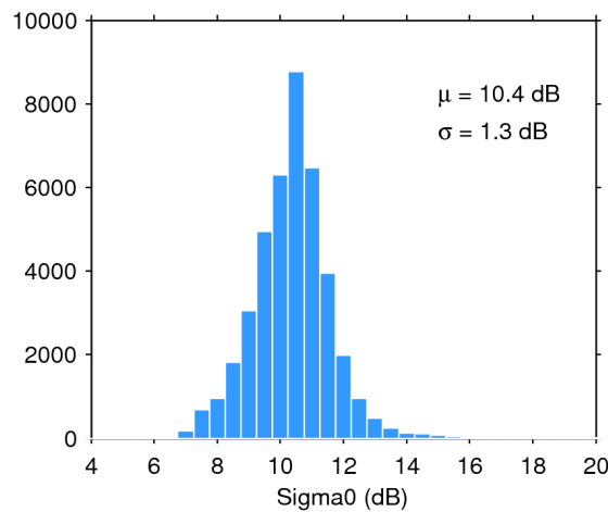
Figure 28. Histogram of science-valid sigma0 over oceans and lakes for 19/01/2018. The mean ( \mu ) and standard deviation ( \sigma ) are also shown. Note that values outside [4 20] dB are excluded from the histogram for the sake of readability but not from the computation of \mu and \sigma .
