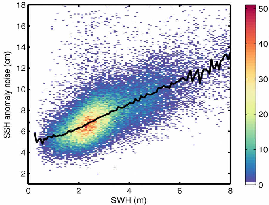
Figure 9. 2D histogram showing flag-valid SSH anomaly noise as a function of SWH for 19/01/2018. The black line denotes the median SSH anomaly noise as a function of SWH.
