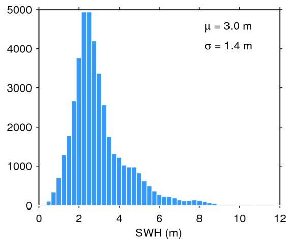
Figure 20. Histogram of science-valid SWH over oceans and lakes for 19/01/2018. The mean ( \mu ) and standard deviation ( \sigma ) are also shown. Note that values larger than 12 m are excluded from the histogram for the sake of readability but not from the computation of \mu and \sigma .
