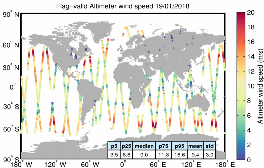
Figure 31. Geographical distribution of flag-valid wind data over oceans and lakes for 19/01/2018. The statistical values shown in the table refer to the wind in m/s and are calculated over all measurements shown in the figure.
