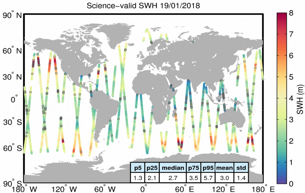
Figure 19. Geographical distribution of science-valid SWH data over oceans and lakes for 19/01/2018. The statistical values shown in the table refer to the SWH in m and are calculated over all measurements shown in the figure. Gray circles denote records that have been rejected based on the editing criteria described in Table 3.
