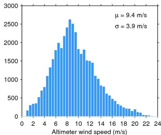
Figure 35. Histogram of science-valid wind over oceans and lakes for 19/01/2018. The mean ( \mu ) and standard deviation ( \sigma ) are also shown. Note that values larger than 24 m/s are excluded from the histogram for the sake of readability but not from the computation of \mu and \sigma .
