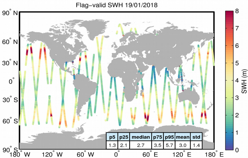
Figure 15. Geographical distribution of flag-valid SWH data over oceans and lakes for 19/01/2018. The statistical values shown in the table refer to the SWH in m and are calculated over all measurements shown in the figure.
