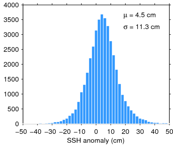
Figure 11. Histogram of science-valid SSH anomaly over oceans and lakes for 19/01/2018. The mean ( \mu ) and standard deviation ( \sigma ) are also shown. Note that values outside [-50 50] cm are excluded from the histogram for the sake of readability but not from the computation of \mu and \sigma .
