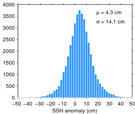
Figure 7. Histogram of flag-valid SSH anomaly over oceans and lakes for 19/01/2018. The mean ( \mu ) and standard deviation ( \sigma ) are also shown. Note that values outside [-50 50] cm are excluded from the histogram for the sake of readability but not from the computation of \mu and \sigma .
