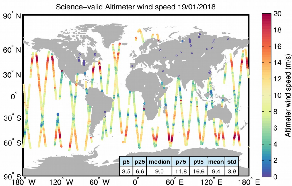
Figure 34. Geographical distribution of science-valid wind data over oceans and lakes for 19/01/2018. The statistical values shown in the table refer to the wind in m/s and are calculated over all measurements shown in the figure. Gray circles denote records that have been rejected based on the editing criteria described in Table 5.
