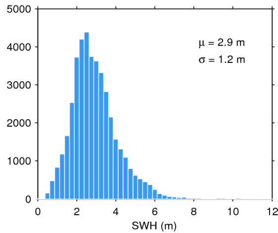
Figure 17. Histogram of flag-valid SWH over oceans and lakes for 17/01/2018. The mean ( \mu ) and standard deviation ( \sigma ) are also shown. Note that values larger than 12 m are excluded from the histogram for the sake of readability but not from the computation of \mu and \sigma .
