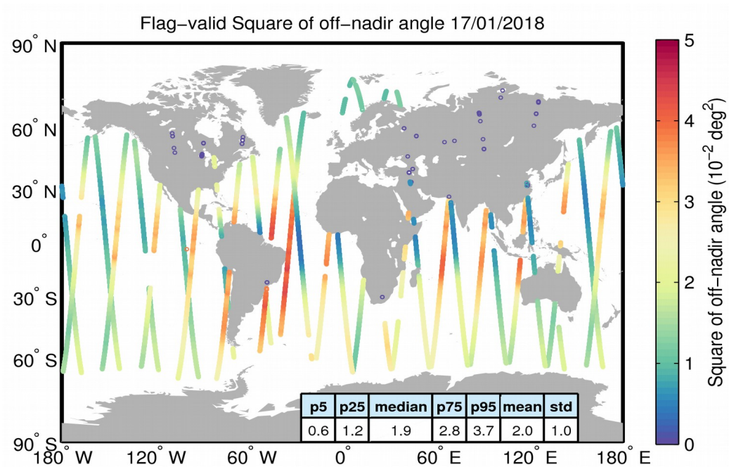
Figure 37. Geographical distribution of flag-valid mispointing data over oceans and lakes for 17/01/2018. The statistical values shown in the table refer to the mispointing in 10^{-2} \text{ deg}^2 and are calculated over all measurements shown in the figure.
