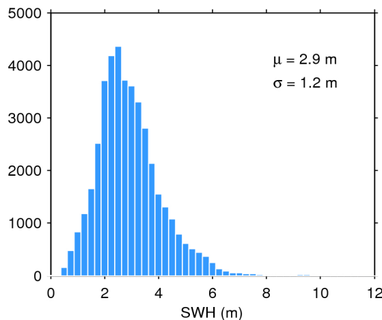
Figure 20. Histogram of science-valid SWH over oceans and lakes for 17/01/2018. The mean ( \mu ) and standard deviation ( \sigma ) are also shown. Note that values larger than 12 m are excluded from the histogram for the sake of readability but not from the computation of \mu and \sigma .
