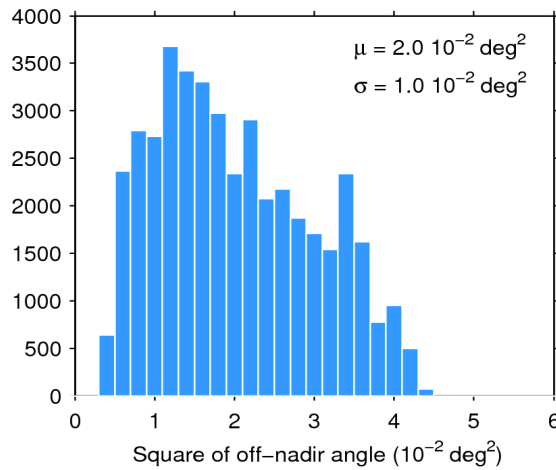
Figure 39. Histogram of flag-valid mispointing over oceans and lakes for 17/01/2018. The mean ( \mu ) and standard deviation ( \sigma ) are also shown. Note that values larger than 6 \cdot 10^{-2} \text{ deg}^2 are excluded from the histogram for the sake of readability but not from the computation of \mu and \sigma .
