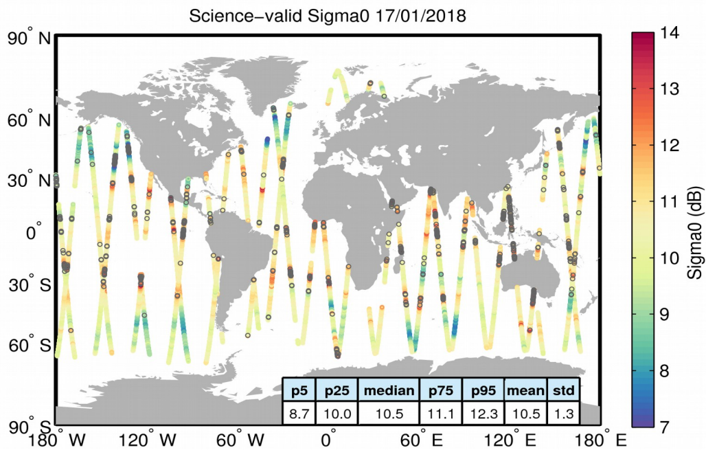
Figure 27. Geographical distribution of science-valid sigma0 data over oceans and lakes for 17/01/2018. The statistical values shown in the table refer to the sigma0 in dB and are calculated over all measurements shown in the figure. Gray circles denote records that have been rejected based on the editing criteria described in Table 4.
