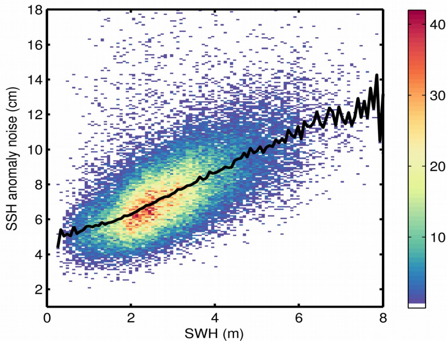
Figure 9. 2D histogram showing flag-valid SSH anomaly noise as a function of SWH for 17/01/2018. The black line denotes the median SSH anomaly noise as a function of SWH.
