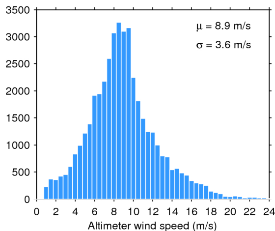
Figure 35. Histogram of science-valid wind over oceans and lakes for 17/01/2018. The mean ( \mu ) and standard deviation ( \sigma ) are also shown. Note that values larger than 24 m/s are excluded from the histogram for the sake of readability but not from the computation of \mu and \sigma .
