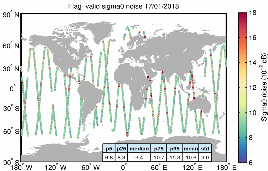
Figure 26. Geographical distribution of flag-valid 20-Hz sigma0 measurement noise over oceans and lakes for 17/01/2018. The statistical values shown in the table refer to the sigma0 noise and are calculated over all measurements shown in the figure.
