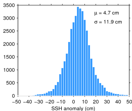
Figure 11. Histogram of science-valid SSH anomaly over oceans and lakes for 17/01/2018. The mean ( \mu ) and standard deviation ( \sigma ) are also shown. Note that values outside [-50 50] cm are excluded from the histogram for the sake of readability but not from the computation of \mu and \sigma .
