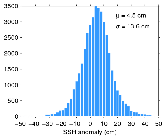
Figure 7. Histogram of flag-valid SSH anomaly over oceans and lakes for 17/01/2018. The mean ( \mu ) and standard deviation ( \sigma ) are also shown. Note that values outside [-50\ 50] cm are excluded from the histogram for the sake of readability but not from the computation of \mu and \sigma .
