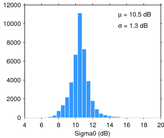
Figure 28. Histogram of science-valid sigma0 over oceans and lakes for 17/01/2018. The mean ( \mu ) and standard deviation ( \sigma ) are also shown. Note that values outside [4 20] dB are excluded from the histogram for the sake of readability but not from the computation of \mu and \sigma .
