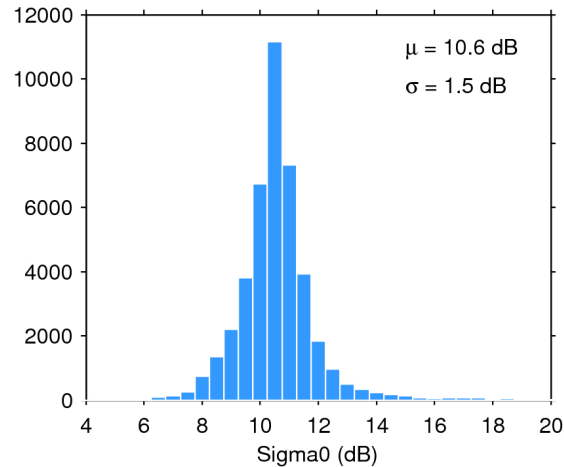
Figure 25. Histogram of flag-valid sigma0 over oceans and lakes for 17/01/2018. The mean ( \mu ) and standard deviation ( \sigma ) are also shown. Note that values outside [4 20] dB are excluded from the histogram for the sake of readability but not from the computation of \mu and \sigma .
