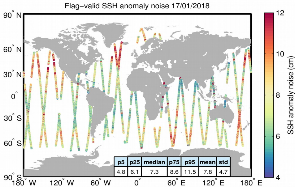
Figure 8. Geographical distribution of flag-valid 20-Hz SSH anomaly measurement noise over oceans and lakes for 17/01/2018. The statistical values shown in the table refer to the SSH anomaly noise and are calculated over all measurements shown in the figure.
