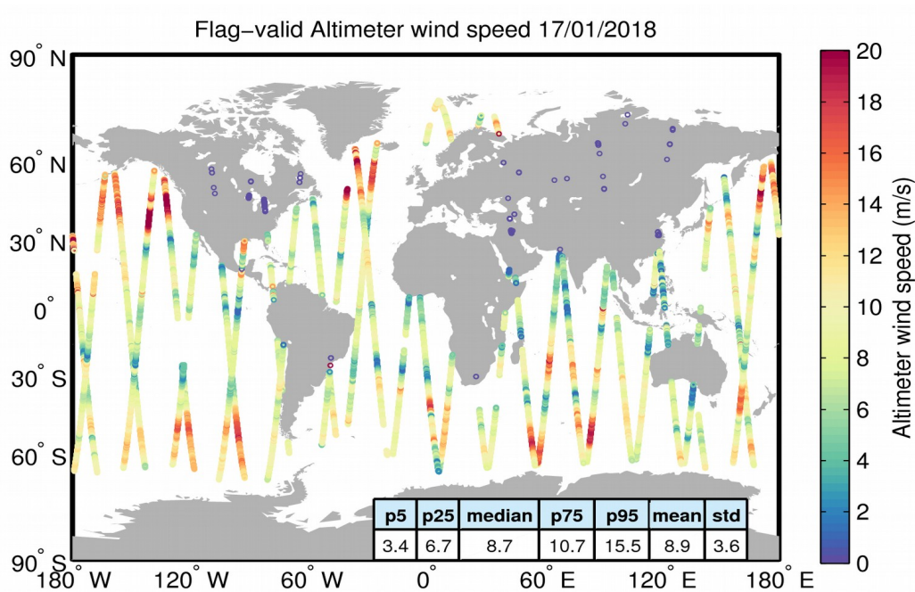
Figure 31. Geographical distribution of flag-valid wind data over oceans and lakes for 17/01/2018. The statistical values shown in the table refer to the wind in m/s and are calculated over all measurements shown in the figure.
