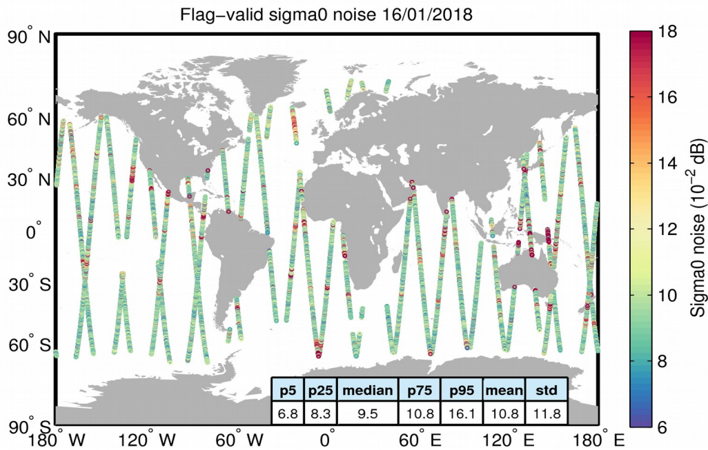
Figure 26. Geographical distribution of flag-valid 20-Hz sigma0 measurement noise over oceans and lakes for 16/01/2018. The statistical values shown in the table refer to the sigma0 noise and are calculated over all measurements shown in the figure.
