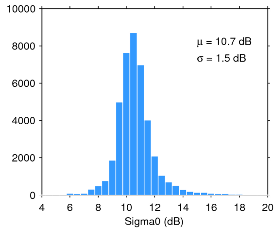
Figure 25. Histogram of flag-valid sigma0 over oceans and lakes for 16/01/2018. The mean ( \mu ) and standard deviation ( \sigma ) are also shown. Note that values outside [4 20] dB are excluded from the histogram for the sake of readability but not from the computation of \mu and \sigma .
