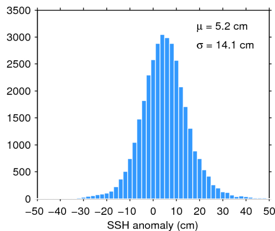
Figure 11. Histogram of science-valid SSH anomaly over oceans and lakes for 16/01/2018. The mean ( \mu ) and standard deviation ( \sigma ) are also shown. Note that values outside [-50 50] cm are excluded from the histogram for the sake of readability but not from the computation of \mu and \sigma .
