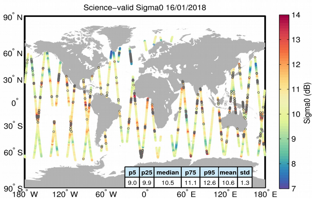
Figure 27. Geographical distribution of science-valid sigma0 data over oceans and lakes for 16/01/2018. The statistical values shown in the table refer to the sigma0 in dB and are calculated over all measurements shown in the figure. Gray circles denote records that have been rejected based on the editing criteria described in Table 4.
