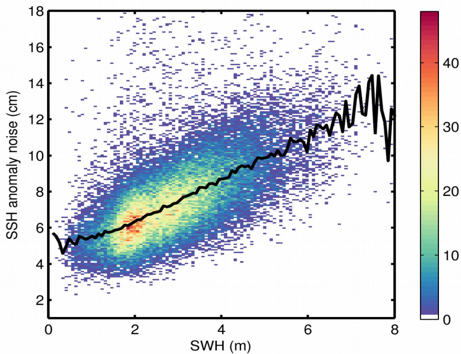
Figure 9. 2D histogram showing flag-valid SSH anomaly noise as a function of SWH for 16/01/2018. The black line denotes the median SSH anomaly noise as a function of SWH.
