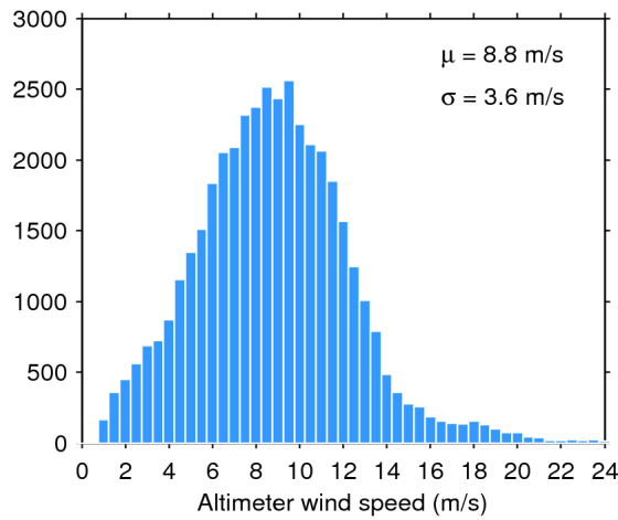
Figure 33. Histogram of flag-valid wind over oceans and lakes for 16/01/2018. The mean ( \mu ) and standard deviation ( \sigma ) are also shown. Note that values larger than 24 m/s are excluded from the histogram for the sake of readability but not from the computation of \mu and \sigma .
