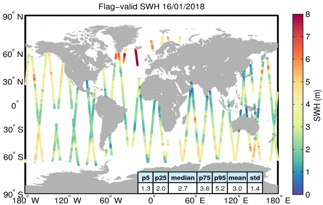
Figure 15. Geographical distribution of flag-valid SWH data over oceans and lakes for 16/01/2018. The statistical values shown in the table refer to the SWH in m and are calculated over all measurements shown in the figure.
