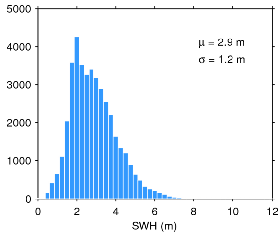
Figure 20. Histogram of science-valid SWH over oceans and lakes for 16/01/2018. The mean ( \mu ) and standard deviation ( \sigma ) are also shown. Note that values larger than 12 m are excluded from the histogram for the sake of readability but not from the computation of \mu and \sigma .
