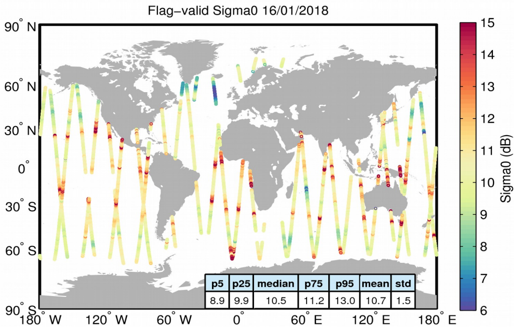
Figure 23. Geographical distribution of flag-valid sigma0 data over oceans and lakes for 16/01/2018. The statistical values shown in the table refer to the sigma0 in dB and are calculated over all measurements shown in the figure.
