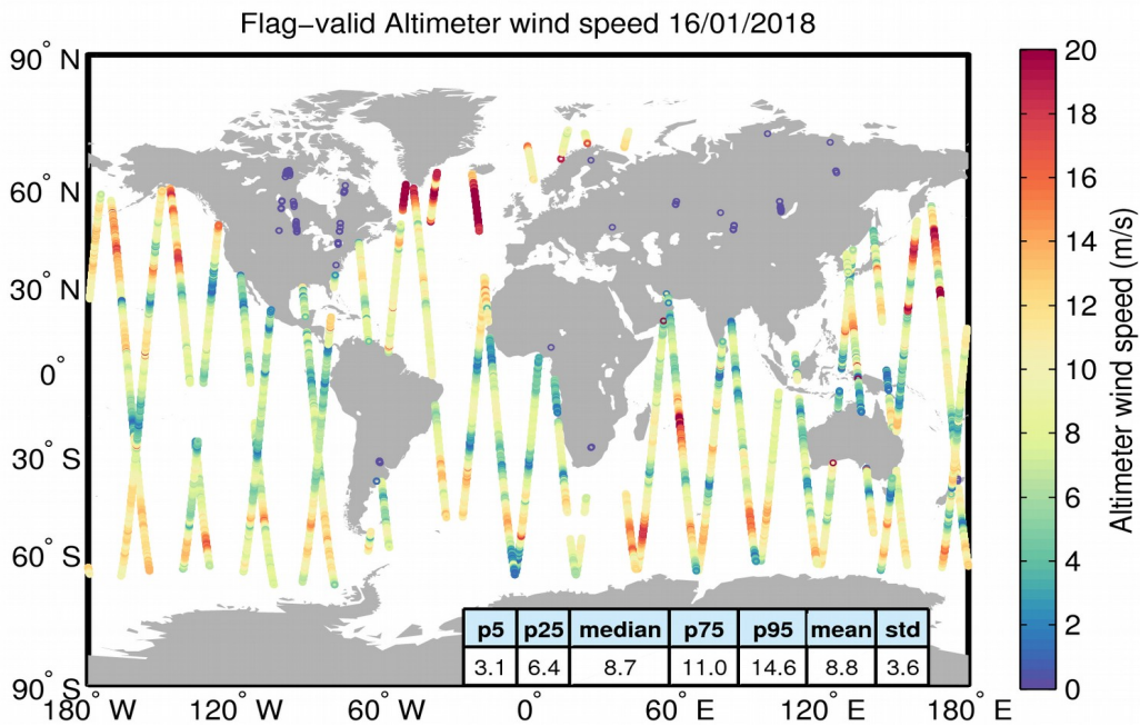
Figure 31. Geographical distribution of flag-valid wind data over oceans and lakes for 16/01/2018. The statistical values shown in the table refer to the wind in m/s and are calculated over all measurements shown in the figure.
