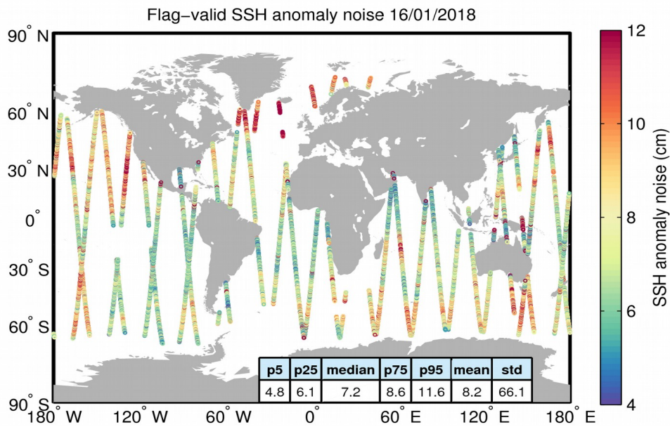
Figure 8. Geographical distribution of flag-valid 20-Hz SSH anomaly measurement noise over oceans and lakes for 16/01/2018. The statistical values shown in the table refer to the SSH anomaly noise and are calculated over all measurements shown in the figure.
