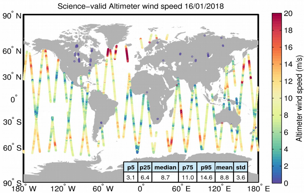
Figure 34. Geographical distribution of science-valid wind data over oceans and lakes for 16/01/2018. The statistical values shown in the table refer to the wind in m/s and are calculated over all measurements shown in the figure. Gray circles denote records that have been rejected based on the editing criteria described in Table 5.
