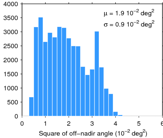
Figure 39. Histogram of flag-valid mispointing over oceans and lakes for 16/01/2018. The mean ( \mu ) and standard deviation ( \sigma ) are also shown. Note that values larger than 6 \cdot 10^{-2} \text{ deg}^2 are excluded from the histogram for the sake of readability but not from the computation of \mu and \sigma .
