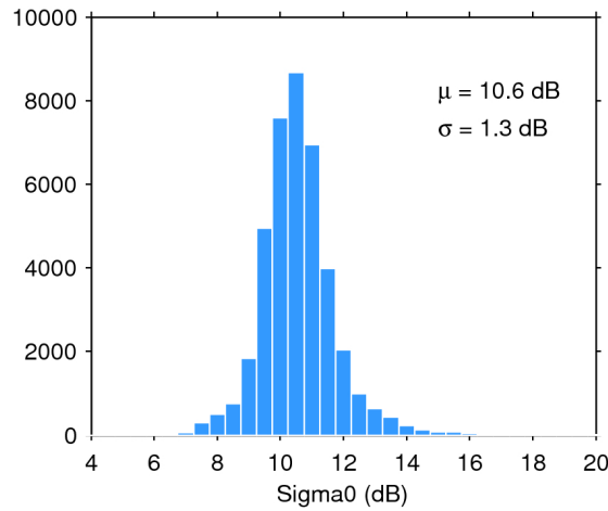
Figure 28. Histogram of science-valid sigma0 over oceans and lakes for 16/01/2018. The mean ( \mu ) and standard deviation ( \sigma ) are also shown. Note that values outside [4 20] dB are excluded from the histogram for the sake of readability but not from the computation of \mu and \sigma .
