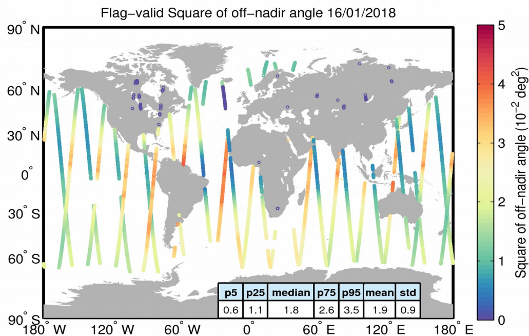
Figure 37. Geographical distribution of flag-valid mispointing data over oceans and lakes for 16/01/2018. The statistical values shown in the table refer to the mispointing in 10^{-2} deg 2 and are calculated over all measurements shown in the figure.
