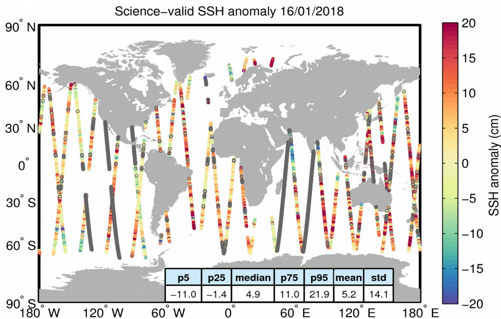
Figure 10. Geographical distribution of science-valid SSH anomaly data over oceans and lakes for 16/01/2018. The statistical values shown in the table refer to the SSH anomaly in cm and are calculated over all measurements shown in the figure. Gray circles denote records that have been rejected based on the editing criteria described in Table 2.
