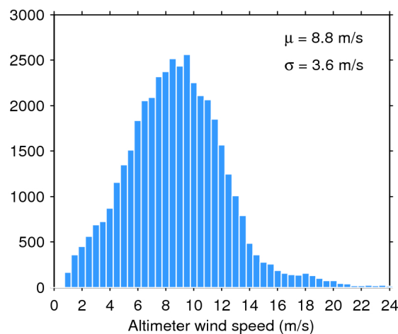
Figure 35. Histogram of science-valid wind over oceans and lakes for 16/01/2018. The mean ( \mu ) and standard deviation ( \sigma ) are also shown. Note that values larger than 24 m/s are excluded from the histogram for the sake of readability but not from the computation of \mu and \sigma .
