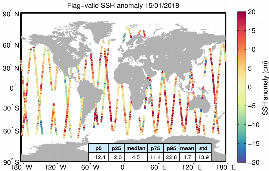
Figure 5. Geographical distribution of flag-valid 1-Hz SSH anomaly data over oceans and lakes for 15/01/2018. The statistical values shown in the table refer to the SSH anomaly in cm and are calculated over all measurements shown in the figure.
