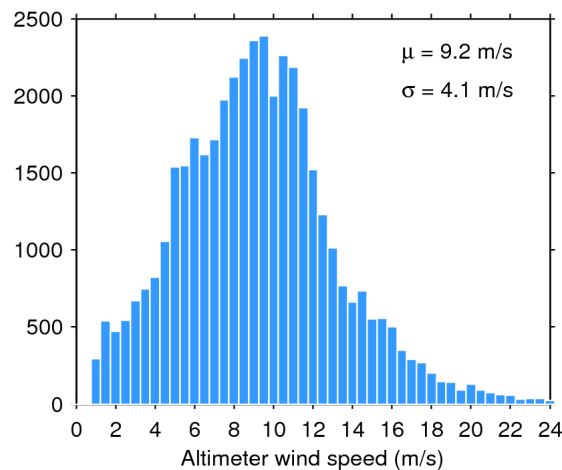
Figure 35. Histogram of science-valid wind over oceans and lakes for 15/01/2018. The mean ( \mu ) and standard deviation ( \sigma ) are also shown. Note that values larger than 24 m/s are excluded from the histogram for the sake of readability but not from the computation of \mu and \sigma .
