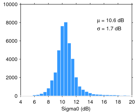
Figure 25. Histogram of flag-valid sigma0 over oceans and lakes for 15/01/2018. The mean ( \mu ) and standard deviation ( \sigma ) are also shown. Note that values outside [4 20] dB are excluded from the histogram for the sake of readability but not from the computation of \mu and \sigma .
