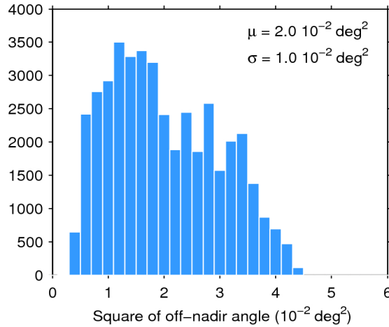
Figure 39. Histogram of flag-valid mispointing over oceans and lakes for 15/01/2018. The mean ( \mu ) and standard deviation ( \sigma ) are also shown. Note that values larger than 6 \cdot 10^{-2} \text{ deg}^2 are excluded from the histogram for the sake of readability but not from the computation of \mu and \sigma .
