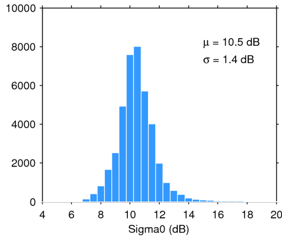
Figure 28. Histogram of science-valid sigma0 over oceans and lakes for 15/01/2018. The mean ( \mu ) and standard deviation ( \sigma ) are also shown. Note that values outside [4 20] dB are excluded from the histogram for the sake of readability but not from the computation of \mu and \sigma .
