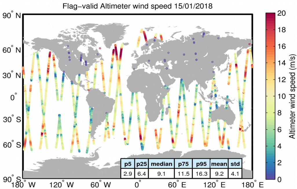
Figure 31. Geographical distribution of flag-valid wind data over oceans and lakes for 15/01/2018. The statistical values shown in the table refer to the wind in m/s and are calculated over all measurements shown in the figure.
