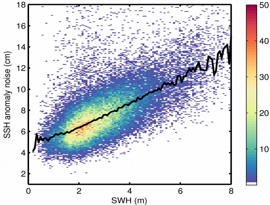
Figure 9. 2D histogram showing flag-valid SSH anomaly noise as a function of SWH for 15/01/2018. The black line denotes the median SSH anomaly noise as a function of SWH.
