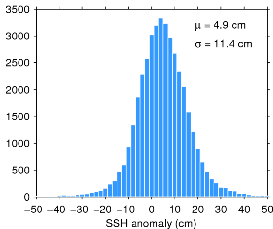
Figure 11. Histogram of science-valid SSH anomaly over oceans and lakes for 15/01/2018. The mean ( \mu ) and standard deviation ( \sigma ) are also shown. Note that values outside [-50 50] cm are excluded from the histogram for the sake of readability but not from the computation of \mu and \sigma .
