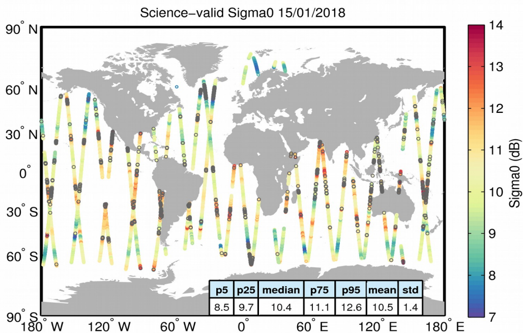
Figure 27. Geographical distribution of science-valid sigma0 data over oceans and lakes for 15/01/2018. The statistical values shown in the table refer to the sigma0 in dB and are calculated over all measurements shown in the figure. Gray circles denote records that have been rejected based on the editing criteria described in Table 4.
