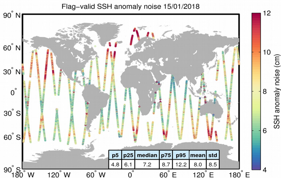
Figure 8. Geographical distribution of flag-valid 20-Hz SSH anomaly measurement noise over oceans and lakes for 15/01/2018. The statistical values shown in the table refer to the SSH anomaly noise and are calculated over all measurements shown in the figure.
