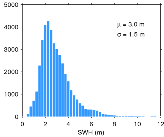
Figure 17. Histogram of flag-valid SWH over oceans and lakes for 15/01/2018. The mean ( \mu ) and standard deviation ( \sigma ) are also shown. Note that values larger than 12 m are excluded from the histogram for the sake of readability but not from the computation of \mu and \sigma .
