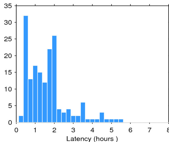
Figure 2. Histogram of the data latency for 15/01/2018. The y-axis denotes the number of files that are made available with a delay of x-hours with respect to the mean time of the records stored in the file.
