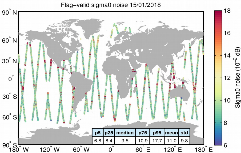
Figure 26. Geographical distribution of flag-valid 20-Hz sigma0 measurement noise over oceans and lakes for 15/01/2018. The statistical values shown in the table refer to the sigma0 noise and are calculated over all measurements shown in the figure.
