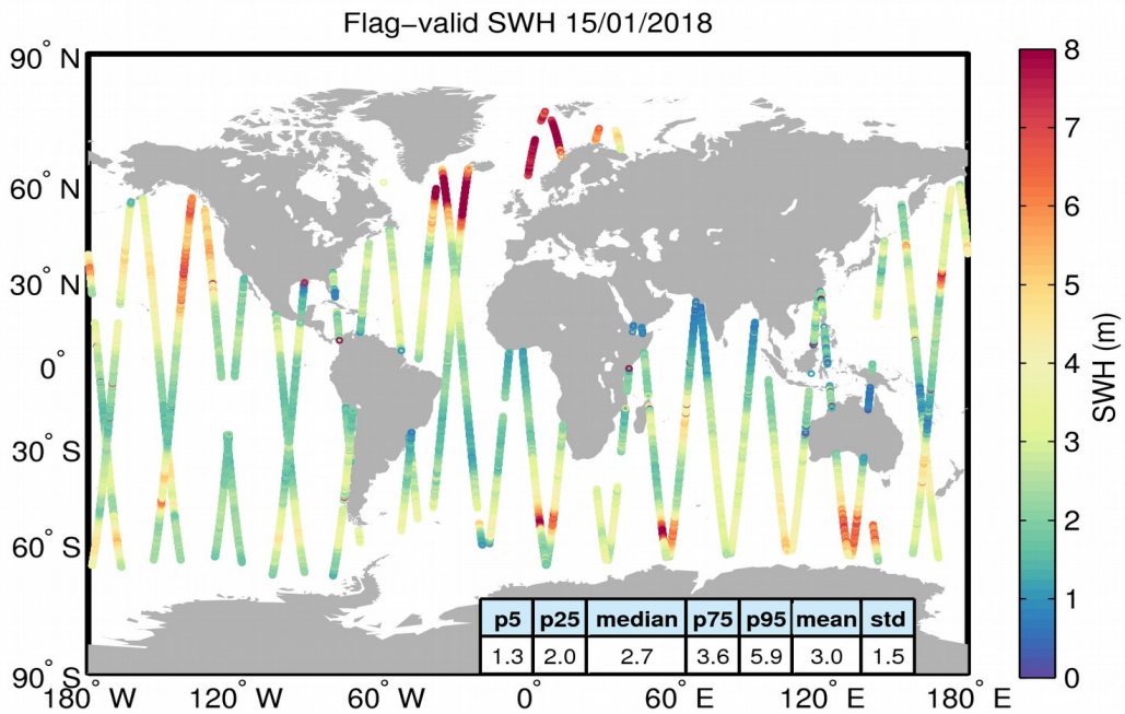
Figure 15. Geographical distribution of flag-valid SWH data over oceans and lakes for 15/01/2018. The statistical values shown in the table refer to the SWH in m and are calculated over all measurements shown in the figure.
