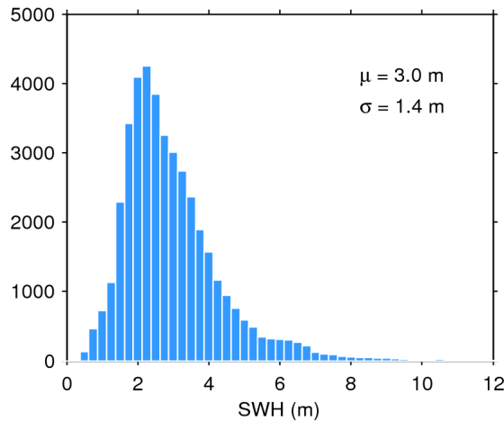
Figure 20. Histogram of science-valid SWH over oceans and lakes for 15/01/2018. The mean ( \mu ) and standard deviation ( \sigma ) are also shown. Note that values larger than 12 m are excluded from the histogram for the sake of readability but not from the computation of \mu and \sigma .
