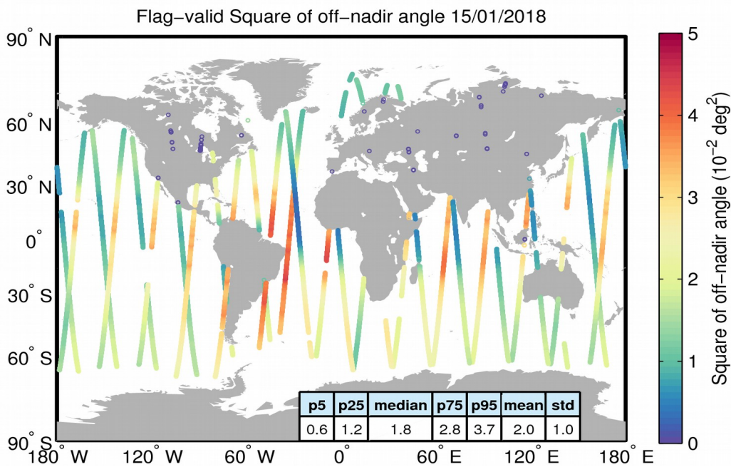
Figure 37. Geographical distribution of flag-valid mispointing data over oceans and lakes for 15/01/2018. The statistical values shown in the table refer to the mispointing in 10^{-2} deg 2 and are calculated over all measurements shown in the figure.
