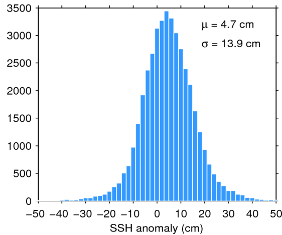
Figure 7. Histogram of flag-valid SSH anomaly over oceans and lakes for 15/01/2018. The mean ( \mu ) and standard deviation ( \sigma ) are also shown. Note that values outside [-50\ 50] cm are excluded from the histogram for the sake of readability but not from the computation of \mu and \sigma .
