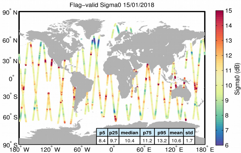
Figure 23. Geographical distribution of flag-valid sigma0 data over oceans and lakes for 15/01/2018. The statistical values shown in the table refer to the sigma0 in dB and are calculated over all measurements shown in the figure.
