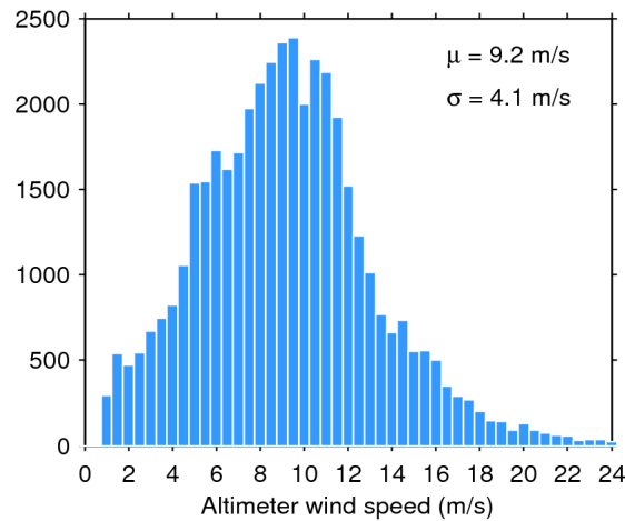
Figure 33. Histogram of flag-valid wind over oceans and lakes for 15/01/2018. The mean ( \mu ) and standard deviation ( \sigma ) are also shown. Note that values larger than 24 m/s are excluded from the histogram for the sake of readability but not from the computation of \mu and \sigma .
