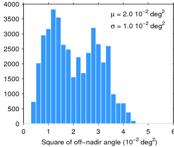
Figure 39. Histogram of flag-valid mispointing over oceans and lakes for 13/01/2018. The mean ( \mu ) and standard deviation ( \sigma ) are also shown. Note that values larger than 6 \cdot 10^{-2} \text{ deg}^2 are excluded from the histogram for the sake of readability but not from the computation of \mu and \sigma .
