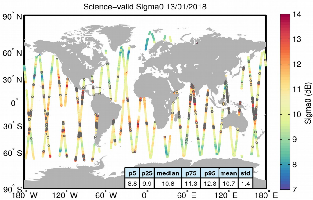
Figure 27. Geographical distribution of science-valid sigma0 data over oceans and lakes for 13/01/2018. The statistical values shown in the table refer to the sigma0 in dB and are calculated over all measurements shown in the figure. Gray circles denote records that have been rejected based on the editing criteria described in Table 4.
