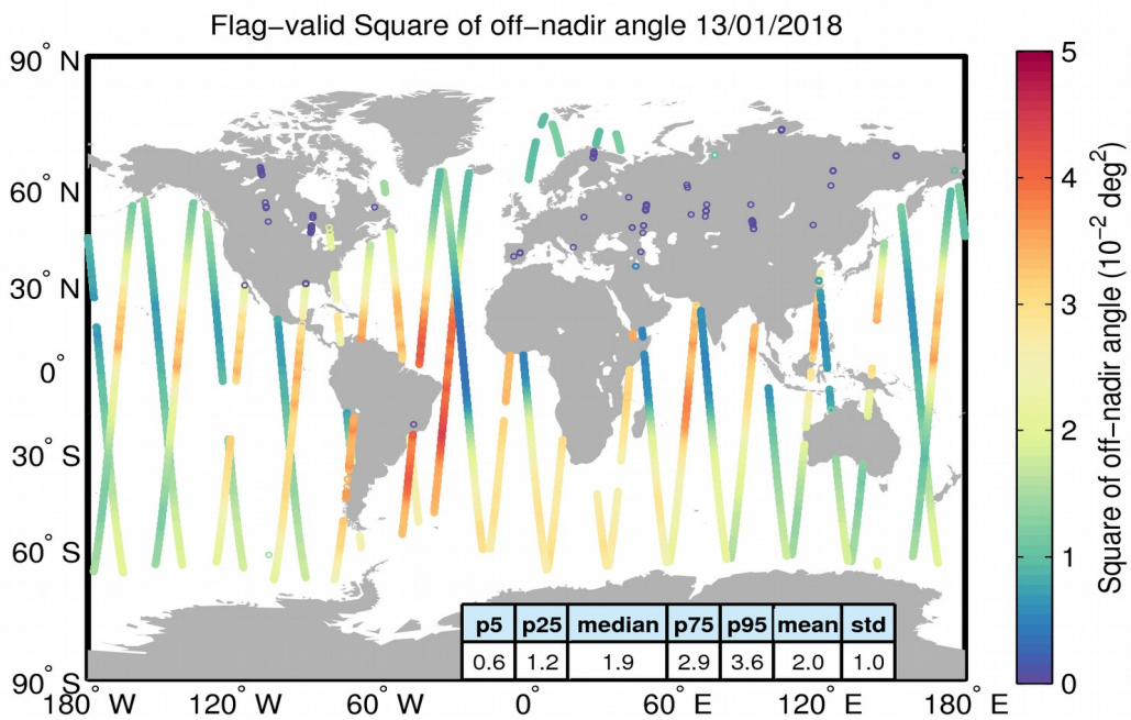
Figure 37. Geographical distribution of flag-valid mispointing data over oceans and lakes for 13/01/2018. The statistical values shown in the table refer to the mispointing in 10^{-2} deg 2 and are calculated over all measurements shown in the figure.
