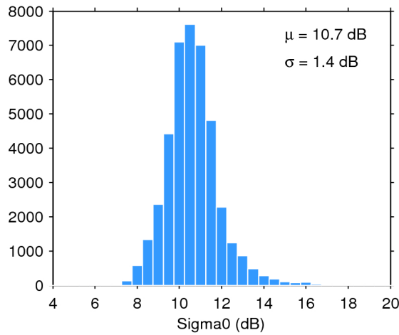
Figure 28. Histogram of science-valid sigma0 over oceans and lakes for 13/01/2018. The mean ( \mu ) and standard deviation ( \sigma ) are also shown. Note that values outside [4 20] dB are excluded from the histogram for the sake of readability but not from the computation of \mu and \sigma .
