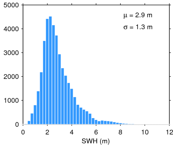
Figure 20. Histogram of science-valid SWH over oceans and lakes for 13/01/2018. The mean ( \mu ) and standard deviation ( \sigma ) are also shown. Note that values larger than 12 m are excluded from the histogram for the sake of readability but not from the computation of \mu and \sigma .
