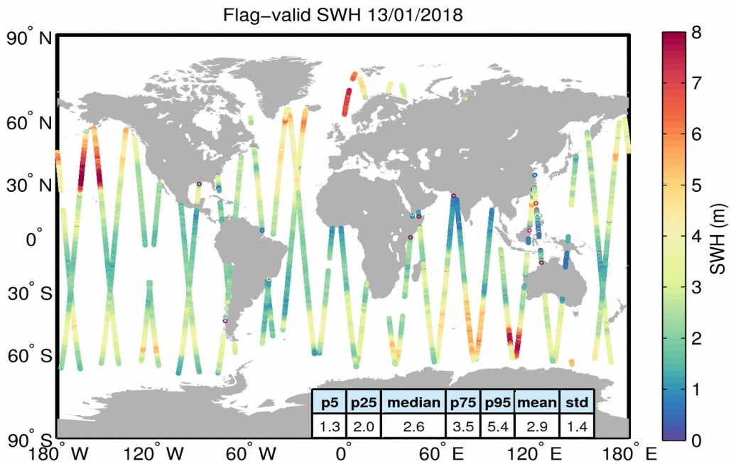
Figure 15. Geographical distribution of flag-valid SWH data over oceans and lakes for 13/01/2018. The statistical values shown in the table refer to the SWH in m and are calculated over all measurements shown in the figure.
