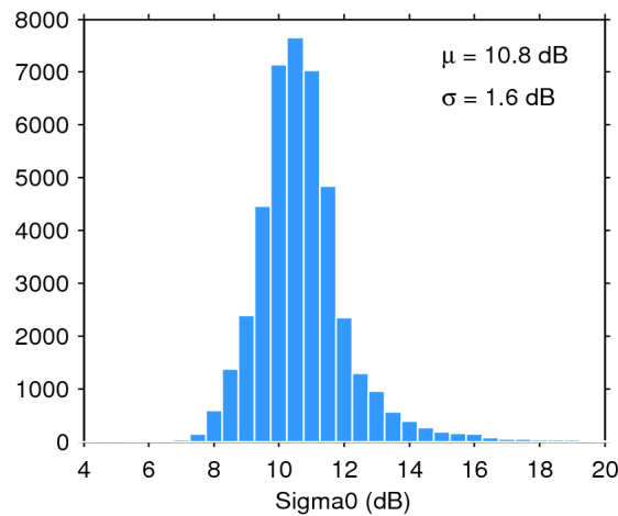
Figure 25. Histogram of flag-valid sigma0 over oceans and lakes for 13/01/2018. The mean ( \mu ) and standard deviation ( \sigma ) are also shown. Note that values outside [4 20] dB are excluded from the histogram for the sake of readability but not from the computation of \mu and \sigma .
