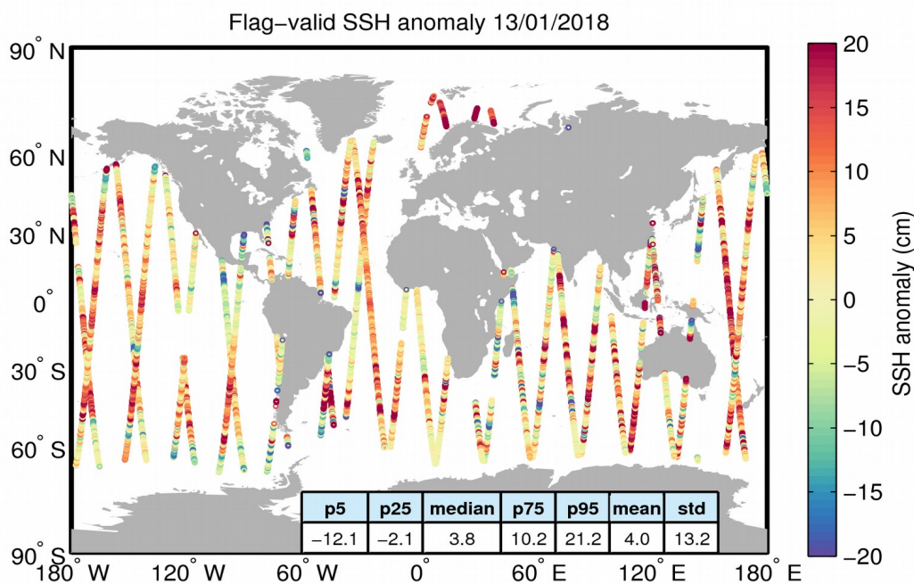
Figure 5. Geographical distribution of flag-valid 1-Hz SSH anomaly data over oceans and lakes for 13/01/2018. The statistical values shown in the table refer to the SSH anomaly in cm and are calculated over all measurements shown in the figure.
