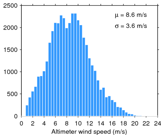
Figure 35. Histogram of science-valid wind over oceans and lakes for 13/01/2018. The mean ( \mu ) and standard deviation ( \sigma ) are also shown. Note that values larger than 24 m/s are excluded from the histogram for the sake of readability but not from the computation of \mu and \sigma .
