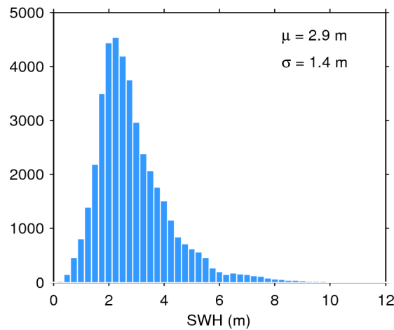
Figure 17. Histogram of flag-valid SWH over oceans and lakes for 13/01/2018. The mean ( \mu ) and standard deviation ( \sigma ) are also shown. Note that values larger than 12 m are excluded from the histogram for the sake of readability but not from the computation of \mu and \sigma .
