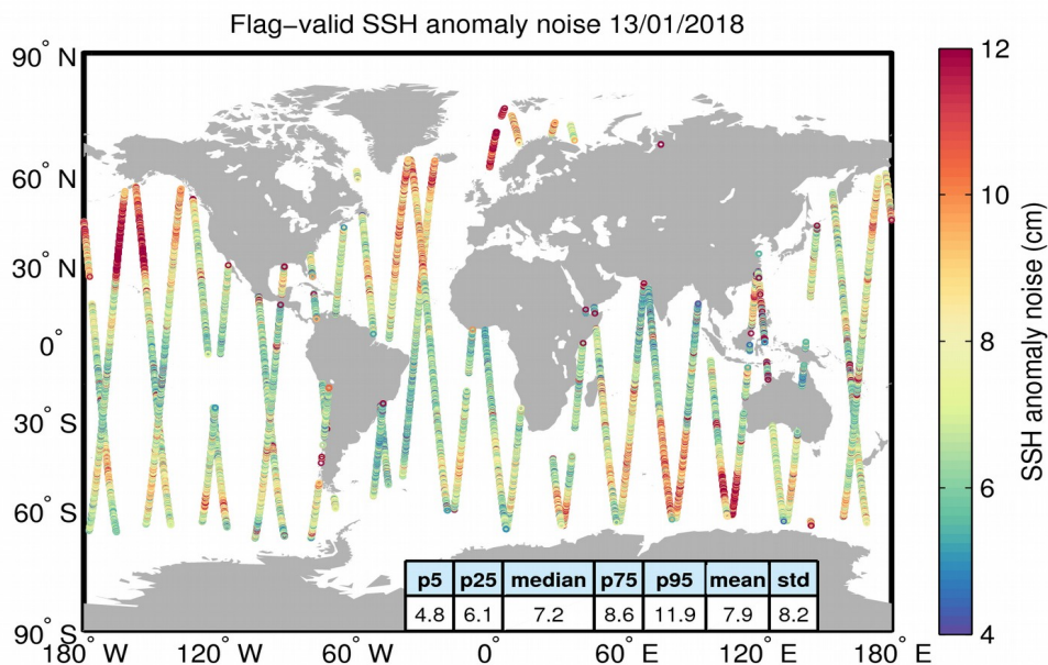
Figure 8. Geographical distribution of flag-valid 20-Hz SSH anomaly measurement noise over oceans and lakes for 13/01/2018. The statistical values shown in the table refer to the SSH anomaly noise and are calculated over all measurements shown in the figure.
