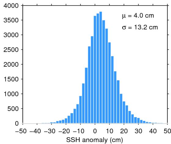
Figure 7. Histogram of flag-valid SSH anomaly over oceans and lakes for 13/01/2018. The mean ( \mu ) and standard deviation ( \sigma ) are also shown. Note that values outside [-50 50] cm are excluded from the histogram for the sake of readability but not from the computation of \mu and \sigma .
