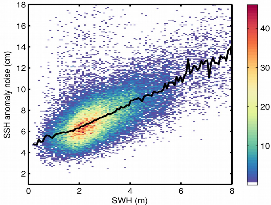
Figure 9. 2D histogram showing flag-valid SSH anomaly noise as a function of SWH for 13/01/2018. The black line denotes the median SSH anomaly noise as a function of SWH.
