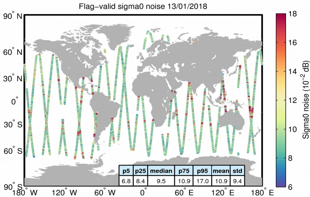
Figure 26. Geographical distribution of flag-valid 20-Hz sigma0 measurement noise over oceans and lakes for 13/01/2018. The statistical values shown in the table refer to the sigma0 noise and are calculated over all measurements shown in the figure.
