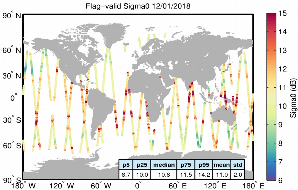
Figure 23. Geographical distribution of flag-valid sigma0 data over oceans and lakes for 12/01/2018. The statistical values shown in the table refer to the sigma0 in dB and are calculated over all measurements shown in the figure.
