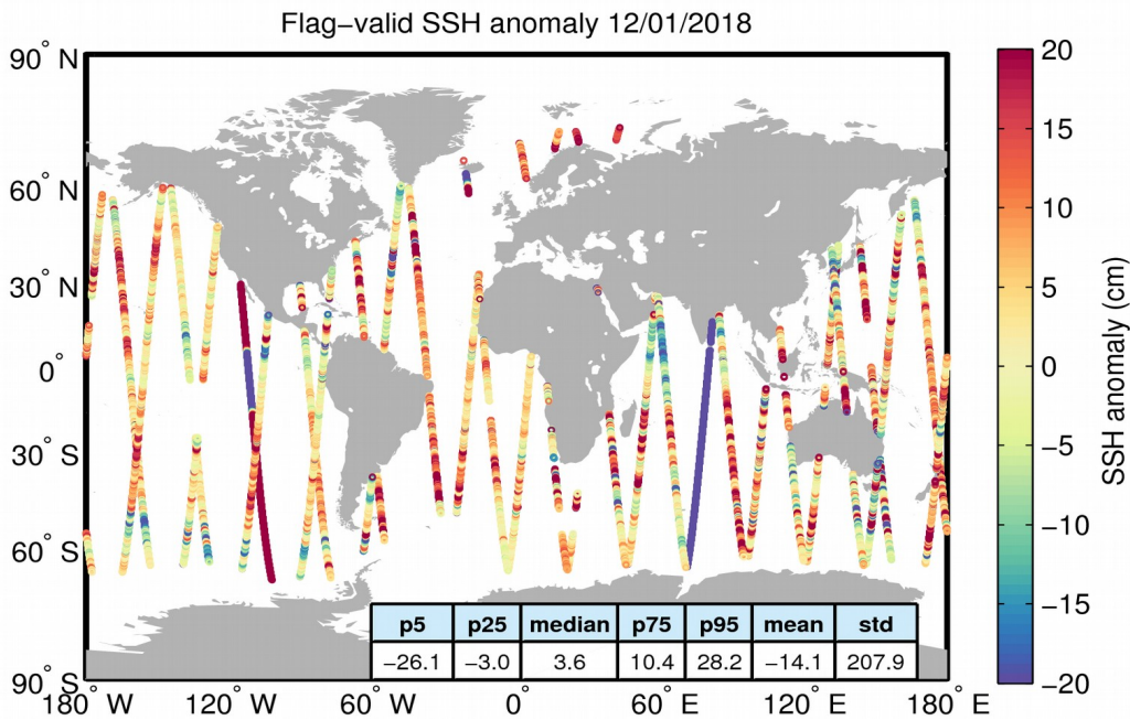
Figure 5. Geographical distribution of flag-valid 1-Hz SSH anomaly data over oceans and lakes for 12/01/2018. The statistical values shown in the table refer to the SSH anomaly in cm and are calculated over all measurements shown in the figure.
