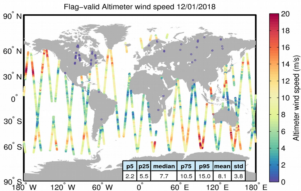
Figure 31. Geographical distribution of flag-valid wind data over oceans and lakes for 12/01/2018. The statistical values shown in the table refer to the wind in m/s and are calculated over all measurements shown in the figure.
