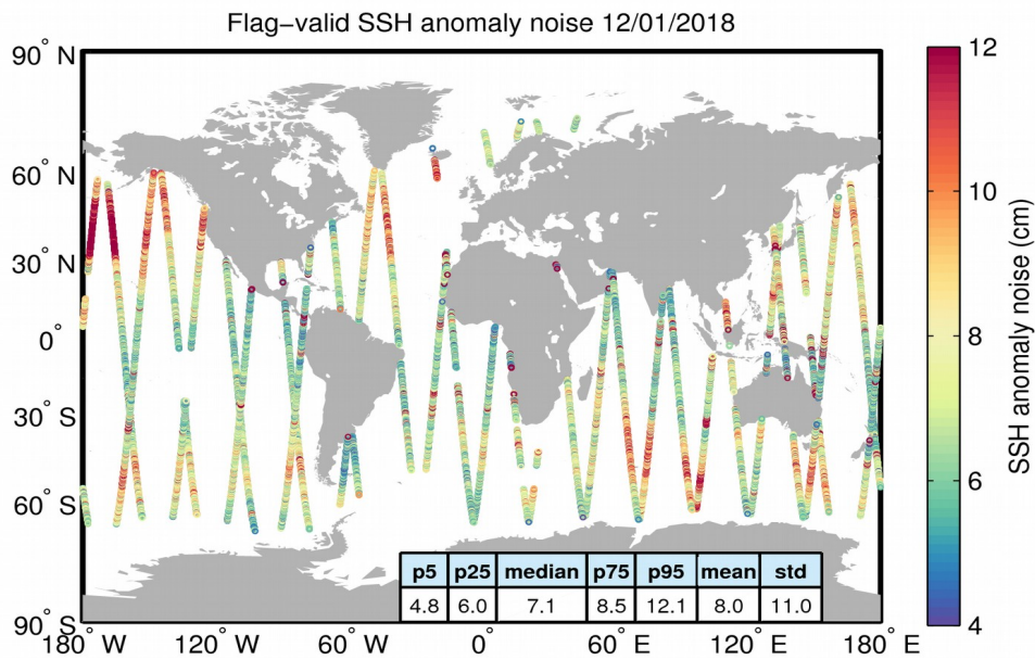
Figure 8. Geographical distribution of flag-valid 20-Hz SSH anomaly measurement noise over oceans and lakes for 12/01/2018. The statistical values shown in the table refer to the SSH anomaly noise and are calculated over all measurements shown in the figure.
