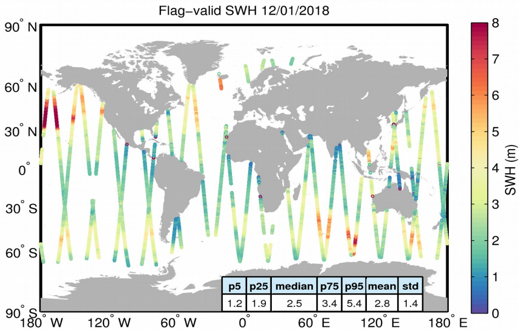
Figure 15. Geographical distribution of flag-valid SWH data over oceans and lakes for 12/01/2018. The statistical values shown in the table refer to the SWH in m and are calculated over all measurements shown in the figure.
