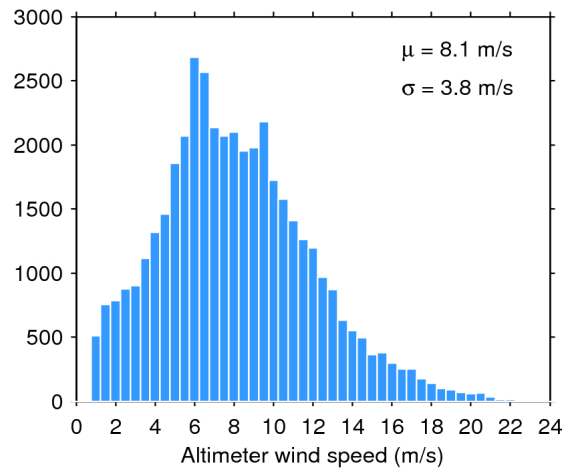
Figure 33. Histogram of flag-valid wind over oceans and lakes for 12/01/2018. The mean ( \mu ) and standard deviation ( \sigma ) are also shown. Note that values larger than 24 m/s are excluded from the histogram for the sake of readability but not from the computation of \mu and \sigma .
