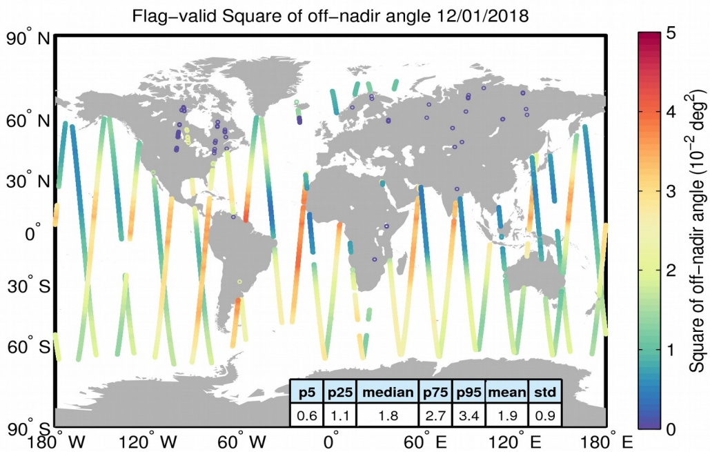
Figure 37. Geographical distribution of flag-valid mispointing data over oceans and lakes for 12/01/2018. The statistical values shown in the table refer to the mispointing in 10^{-2} deg 2 and are calculated over all measurements shown in the figure.
