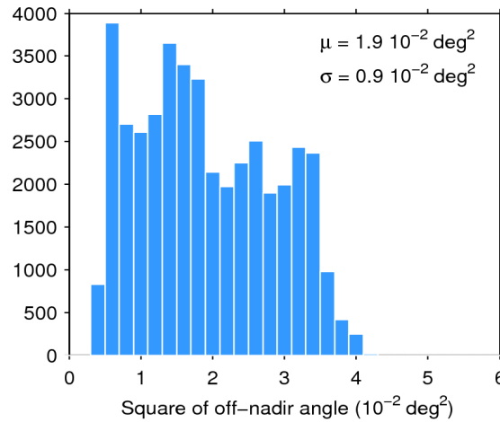
Figure 39. Histogram of flag-valid mispointing over oceans and lakes for 12/01/2018. The mean ( \mu ) and standard deviation ( \sigma ) are also shown. Note that values larger than 6 \cdot 10^{-2} \text{ deg}^2 are excluded from the histogram for the sake of readability but not from the computation of \mu and \sigma .
