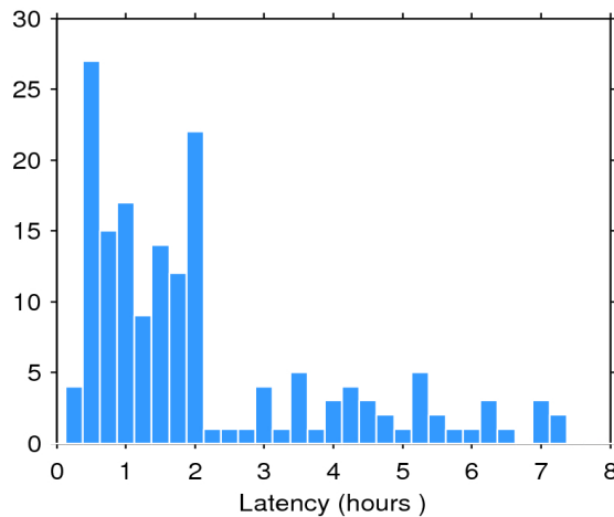
Figure 2. Histogram of the data latency for 12/01/2018. The y-axis denotes the number of files that are made available with a delay of x-hours with respect to the mean time of the records stored in the file.
