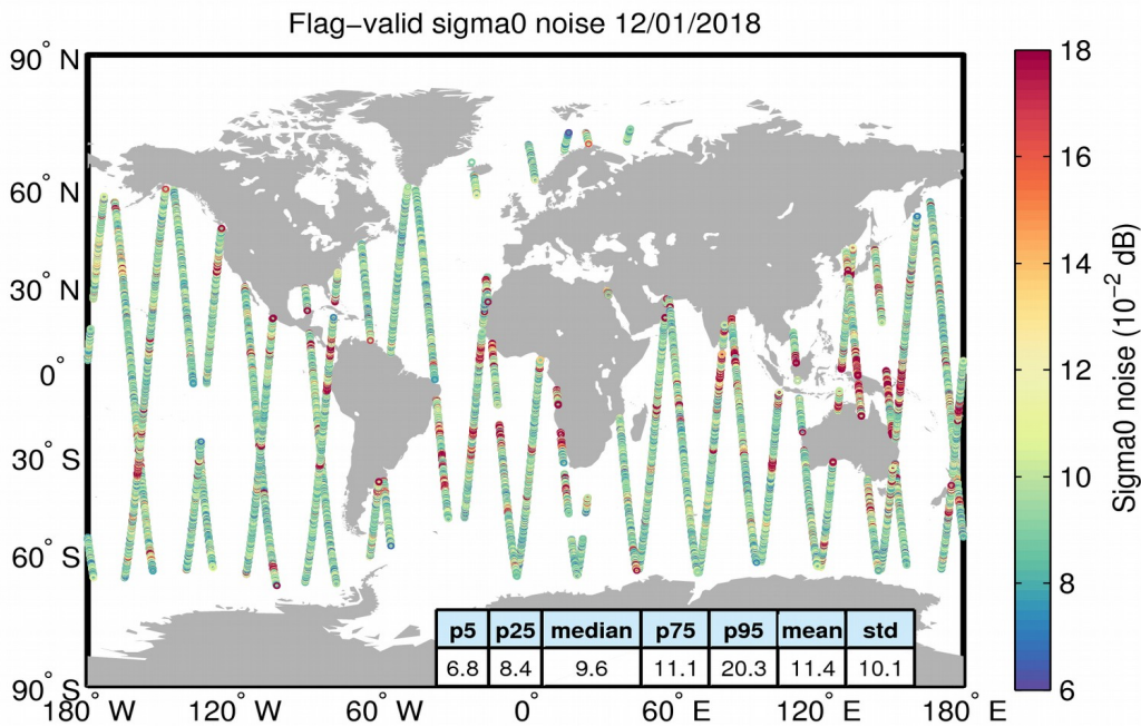
Figure 26. Geographical distribution of flag-valid 20-Hz sigma0 measurement noise over oceans and lakes for 12/01/2018. The statistical values shown in the table refer to the sigma0 noise and are calculated over all measurements shown in the figure.
