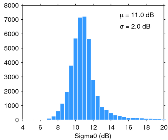
Figure 25. Histogram of flag-valid sigma0 over oceans and lakes for 12/01/2018. The mean ( \mu ) and standard deviation ( \sigma ) are also shown. Note that values outside [4 20] dB are excluded from the histogram for the sake of readability but not from the computation of \mu and \sigma .
