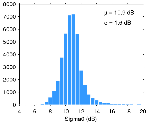
Figure 28. Histogram of science-valid sigma0 over oceans and lakes for 12/01/2018. The mean ( \mu ) and standard deviation ( \sigma ) are also shown. Note that values outside [4 20] dB are excluded from the histogram for the sake of readability but not from the computation of \mu and \sigma .
