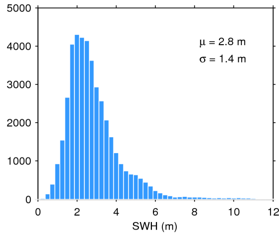
Figure 17. Histogram of flag-valid SWH over oceans and lakes for 12/01/2018. The mean ( \mu ) and standard deviation ( \sigma ) are also shown. Note that values larger than 12 m are excluded from the histogram for the sake of readability but not from the computation of \mu and \sigma .
