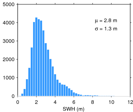
Figure 20. Histogram of science-valid SWH over oceans and lakes for 12/01/2018. The mean ( \mu ) and standard deviation ( \sigma ) are also shown. Note that values larger than 12 m are excluded from the histogram for the sake of readability but not from the computation of \mu and \sigma .
