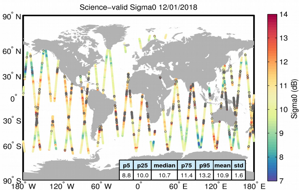
Figure 27. Geographical distribution of science-valid sigma0 data over oceans and lakes for 12/01/2018. The statistical values shown in the table refer to the sigma0 in dB and are calculated over all measurements shown in the figure. Gray circles denote records that have been rejected based on the editing criteria described in Table 4.
