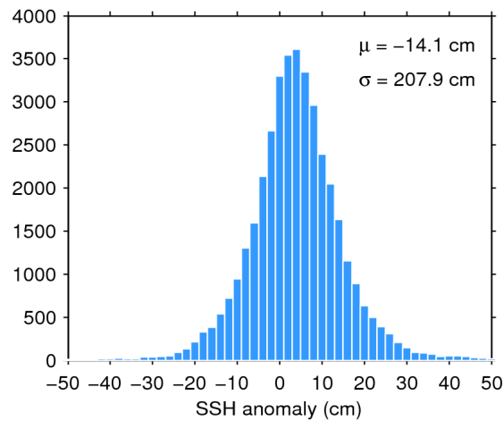
Figure 7. Histogram of flag-valid SSH anomaly over oceans and lakes for 12/01/2018. The mean ( \mu ) and standard deviation ( \sigma ) are also shown. Note that values outside [-50 50] cm are excluded from the histogram for the sake of readability but not from the computation of \mu and \sigma .
