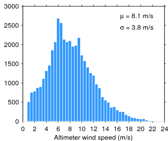
Figure 35. Histogram of science-valid wind over oceans and lakes for 12/01/2018. The mean ( \mu ) and standard deviation ( \sigma ) are also shown. Note that values larger than 24 m/s are excluded from the histogram for the sake of readability but not from the computation of \mu and \sigma .
