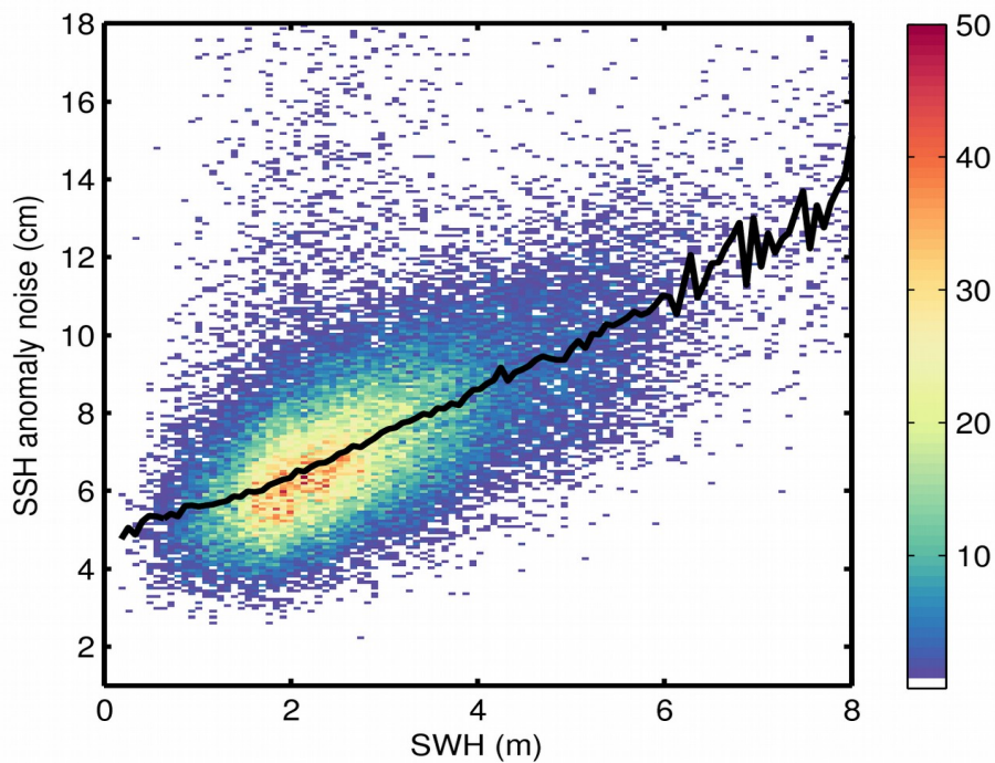
Figure 9. 2D histogram showing flag-valid SSH anomaly noise as a function of SWH for 12/01/2018. The black line denotes the median SSH anomaly noise as a function of SWH.
