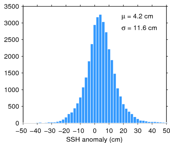
Figure 11. Histogram of science-valid SSH anomaly over oceans and lakes for 12/01/2018. The mean ( \mu ) and standard deviation ( \sigma ) are also shown. Note that values outside [-50 50] cm are excluded from the histogram for the sake of readability but not from the computation of \mu and \sigma .
