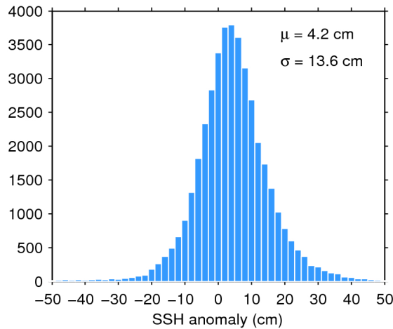
Figure 7. Histogram of flag-valid SSH anomaly over oceans and lakes for 09/01/2018. The mean ( \mu ) and standard deviation ( \sigma ) are also shown. Note that values outside [-50 50] cm are excluded from the histogram for the sake of readability but not from the computation of \mu and \sigma .
