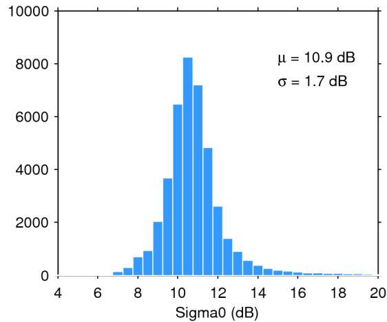
Figure 25. Histogram of flag-valid sigma0 over oceans and lakes for 09/01/2018. The mean ( \mu ) and standard deviation ( \sigma ) are also shown. Note that values outside [4 20] dB are excluded from the histogram for the sake of readability but not from the computation of \mu and \sigma .
