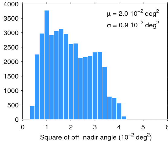
Figure 39. Histogram of flag-valid mispointing over oceans and lakes for 09/01/2018. The mean ( \mu ) and standard deviation ( \sigma ) are also shown. Note that values larger than 6 \cdot 10^{-2} \text{ deg}^2 are excluded from the histogram for the sake of readability but not from the computation of \mu and \sigma .
