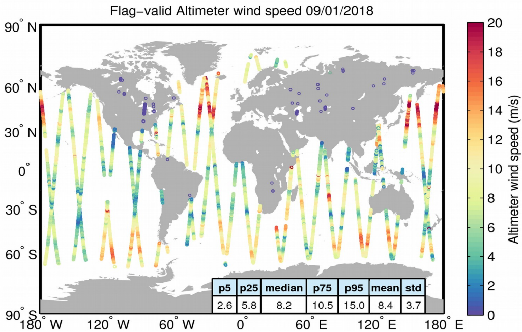
Figure 31. Geographical distribution of flag-valid wind data over oceans and lakes for 09/01/2018. The statistical values shown in the table refer to the wind in m/s and are calculated over all measurements shown in the figure.
