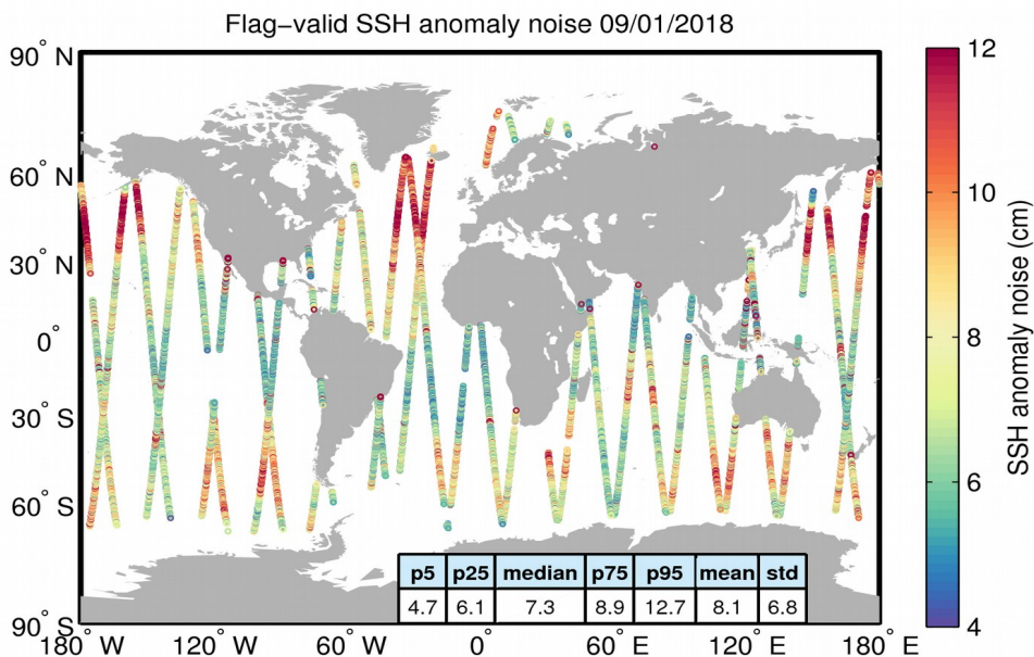
Figure 8. Geographical distribution of flag-valid 20-Hz SSH anomaly measurement noise over oceans and lakes for 09/01/2018. The statistical values shown in the table refer to the SSH anomaly noise and are calculated over all measurements shown in the figure.
