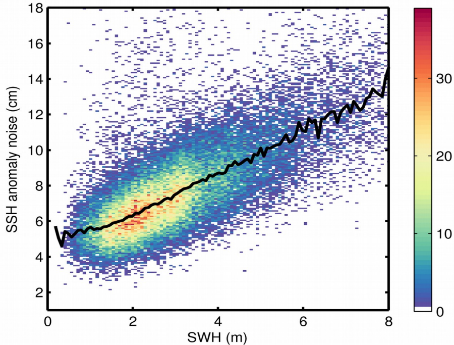
Figure 9. 2D histogram showing flag-valid SSH anomaly noise as a function of SWH for 09/01/2018. The black line denotes the median SSH anomaly noise as a function of SWH.
