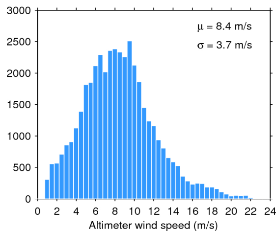
Figure 35. Histogram of science-valid wind over oceans and lakes for 09/01/2018. The mean ( \mu ) and standard deviation ( \sigma ) are also shown. Note that values larger than 24 m/s are excluded from the histogram for the sake of readability but not from the computation of \mu and \sigma .
