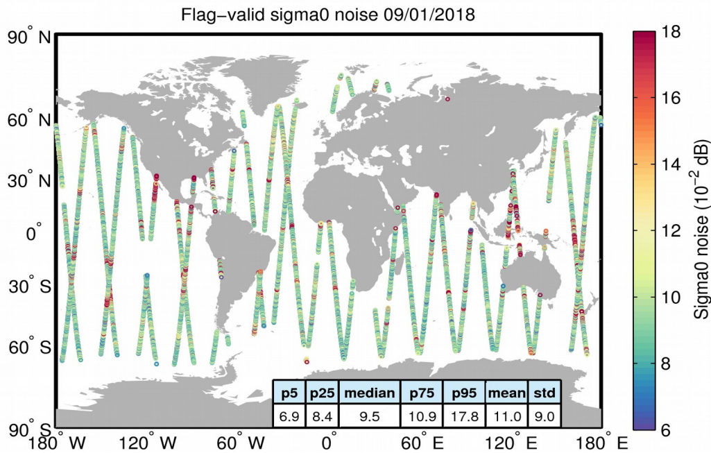
Figure 26. Geographical distribution of flag-valid 20-Hz sigma0 measurement noise over oceans and lakes for 09/01/2018. The statistical values shown in the table refer to the sigma0 noise and are calculated over all measurements shown in the figure.
