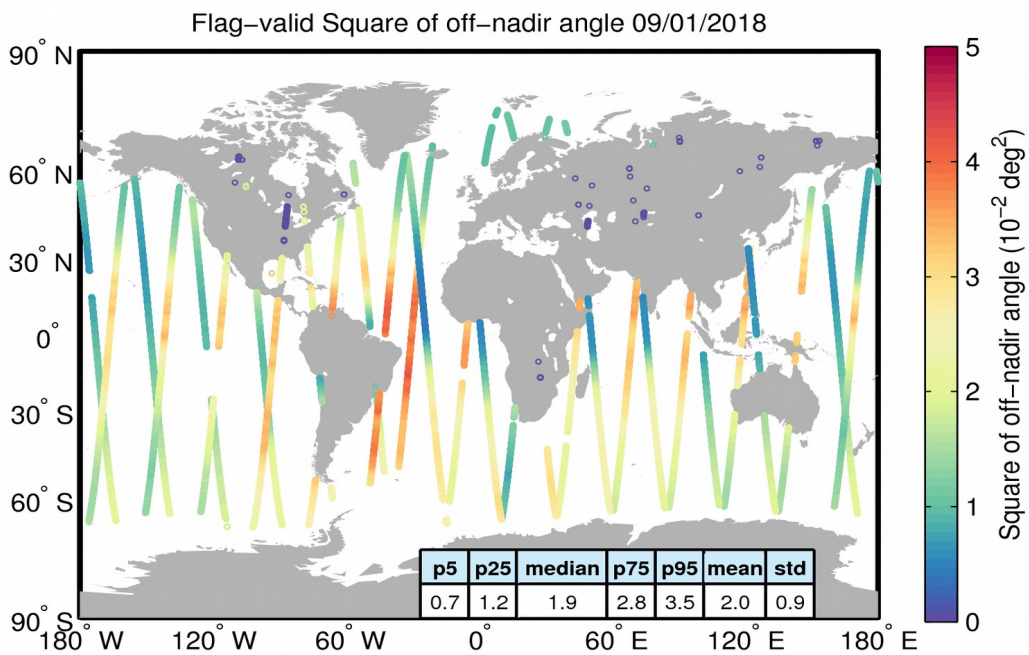
Figure 37. Geographical distribution of flag-valid mispointing data over oceans and lakes for 09/01/2018. The statistical values shown in the table refer to the mispointing in 10^{-2} deg 2 and are calculated over all measurements shown in the figure.
