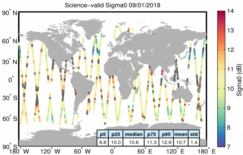
Figure 27. Geographical distribution of science-valid sigma0 data over oceans and lakes for 09/01/2018. The statistical values shown in the table refer to the sigma0 in dB and are calculated over all measurements shown in the figure. Gray circles denote records that have been rejected based on the editing criteria described in Table 4.
