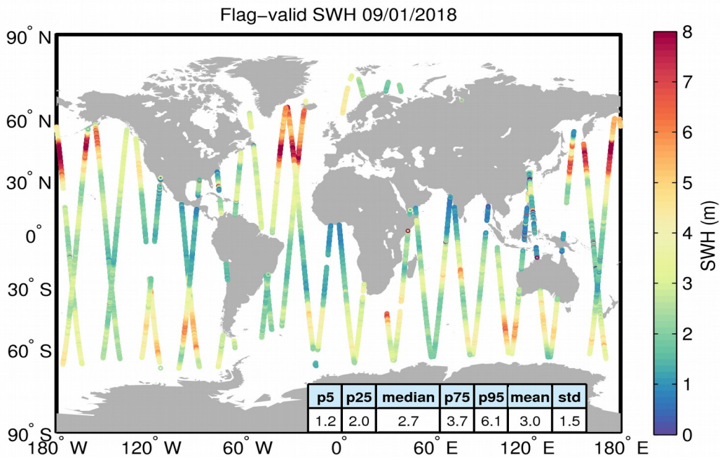
Figure 15. Geographical distribution of flag-valid SWH data over oceans and lakes for 09/01/2018. The statistical values shown in the table refer to the SWH in m and are calculated over all measurements shown in the figure.
