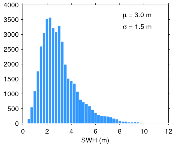
Figure 17. Histogram of flag-valid SWH over oceans and lakes for 09/01/2018. The mean ( \mu ) and standard deviation ( \sigma ) are also shown. Note that values larger than 12 m are excluded from the histogram for the sake of readability but not from the computation of \mu and \sigma .
