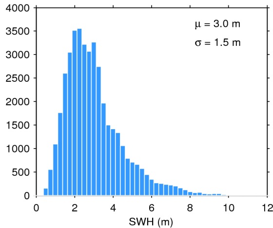
Figure 20. Histogram of science-valid SWH over oceans and lakes for 09/01/2018. The mean ( \mu ) and standard deviation ( \sigma ) are also shown. Note that values larger than 12 m are excluded from the histogram for the sake of readability but not from the computation of \mu and \sigma .
