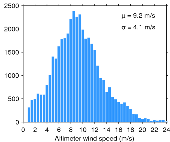
Figure 35. Histogram of science-valid wind over oceans and lakes for 07/01/2018. The mean ( \mu ) and standard deviation ( \sigma ) are also shown. Note that values larger than 24 m/s are excluded from the histogram for the sake of readability but not from the computation of \mu and \sigma .
