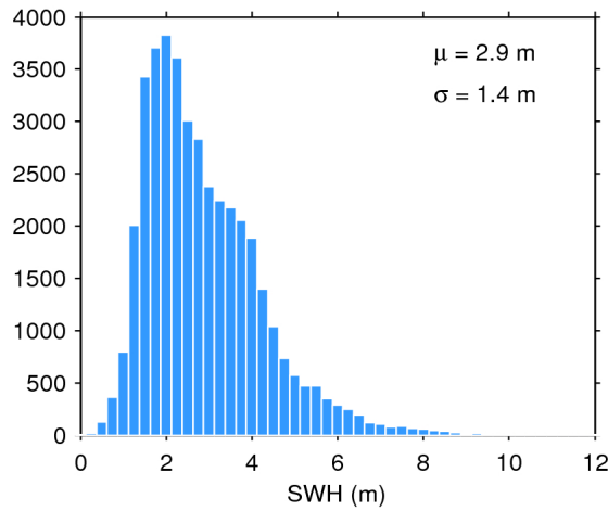
Figure 17. Histogram of flag-valid SWH over oceans and lakes for 07/01/2018. The mean ( \mu ) and standard deviation ( \sigma ) are also shown. Note that values larger than 12 m are excluded from the histogram for the sake of readability but not from the computation of \mu and \sigma .
