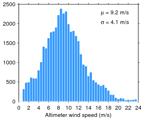
Figure 33. Histogram of flag-valid wind over oceans and lakes for 07/01/2018. The mean ( \mu ) and standard deviation ( \sigma ) are also shown. Note that values larger than 24 m/s are excluded from the histogram for the sake of readability but not from the computation of \mu and \sigma .
