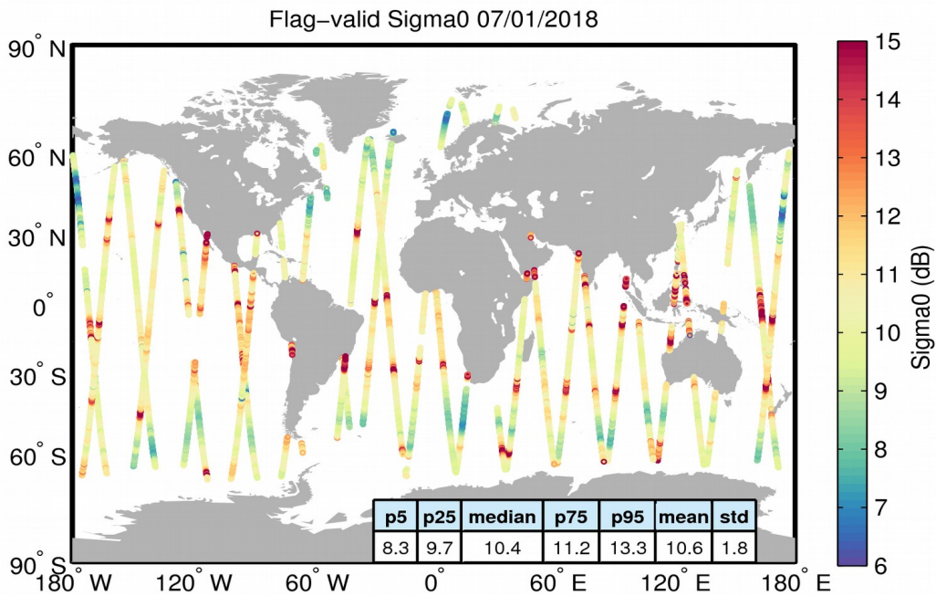
Figure 23. Geographical distribution of flag-valid sigma0 data over oceans and lakes for 07/01/2018. The statistical values shown in the table refer to the sigma0 in dB and are calculated over all measurements shown in the figure.
