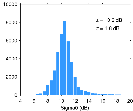
Figure 25. Histogram of flag-valid sigma0 over oceans and lakes for 07/01/2018. The mean ( \mu ) and standard deviation ( \sigma ) are also shown. Note that values outside [4 20] dB are excluded from the histogram for the sake of readability but not from the computation of \mu and \sigma .
