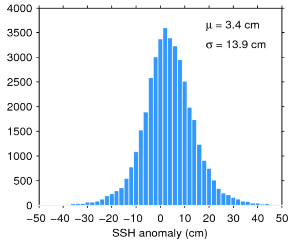
Figure 7. Histogram of flag-valid SSH anomaly over oceans and lakes for 07/01/2018. The mean ( \mu ) and standard deviation ( \sigma ) are also shown. Note that values outside [-50\ 50] cm are excluded from the histogram for the sake of readability but not from the computation of \mu and \sigma .
