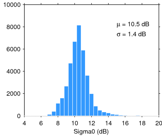
Figure 28. Histogram of science-valid sigma0 over oceans and lakes for 07/01/2018. The mean ( \mu ) and standard deviation ( \sigma ) are also shown. Note that values outside [4 20] dB are excluded from the histogram for the sake of readability but not from the computation of \mu and \sigma .
