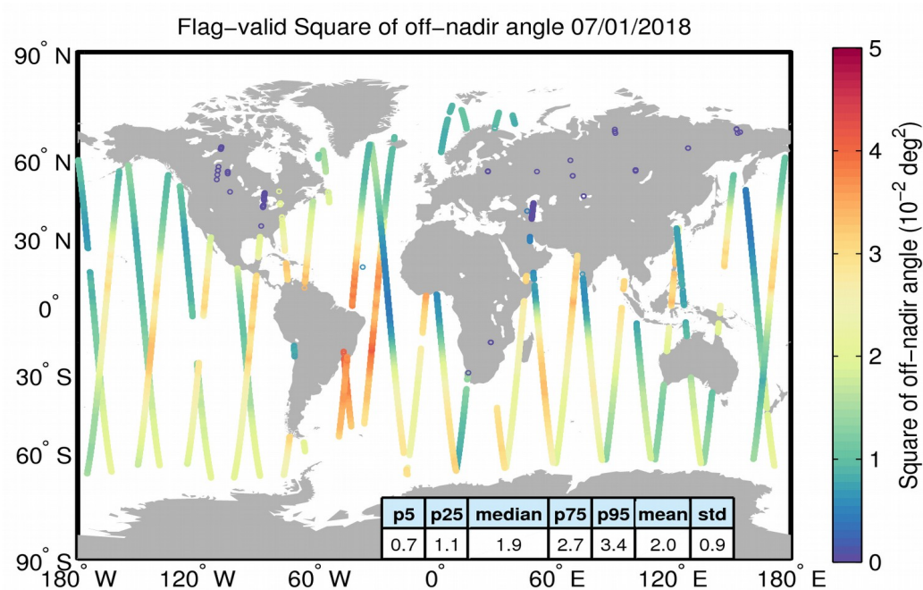
Figure 37. Geographical distribution of flag-valid mispointing data over oceans and lakes for 07/01/2018. The statistical values shown in the table refer to the mispointing in 10^{-2} deg 2 and are calculated over all measurements shown in the figure.
