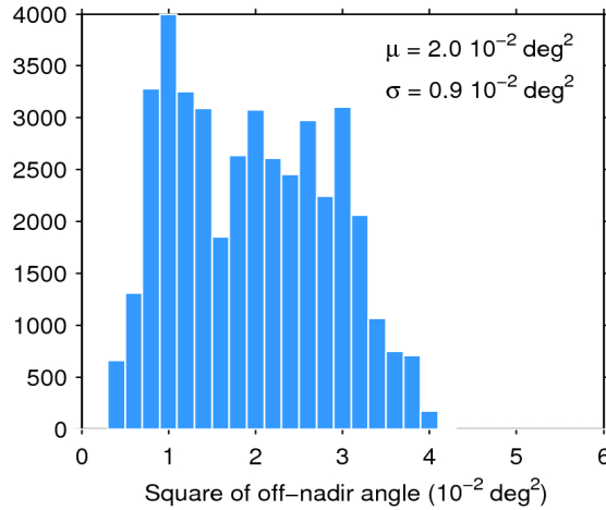
Figure 39. Histogram of flag-valid mispointing over oceans and lakes for 07/01/2018. The mean ( \mu ) and standard deviation ( \sigma ) are also shown. Note that values larger than 6 \cdot 10^{-2} \text{ deg}^2 are excluded from the histogram for the sake of readability but not from the computation of \mu and \sigma .
