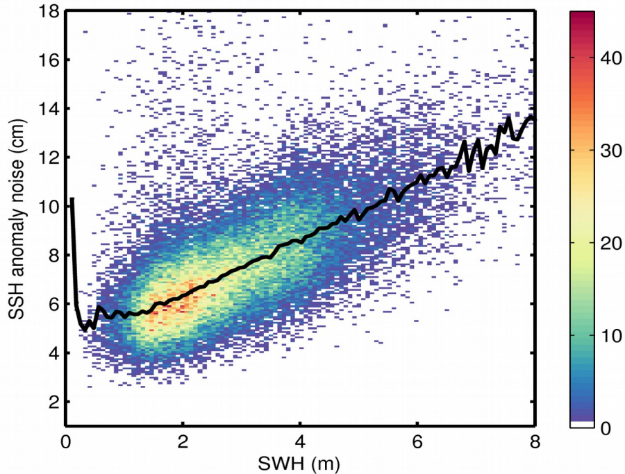
Figure 9. 2D histogram showing flag-valid SSH anomaly noise as a function of SWH for 07/01/2018. The black line denotes the median SSH anomaly noise as a function of SWH.
