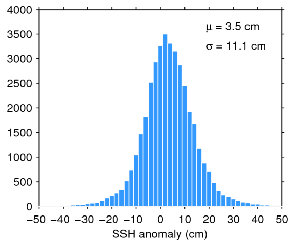
Figure 11. Histogram of science-valid SSH anomaly over oceans and lakes for 07/01/2018. The mean ( \mu ) and standard deviation ( \sigma ) are also shown. Note that values outside [-50 50] cm are excluded from the histogram for the sake of readability but not from the computation of \mu and \sigma .
