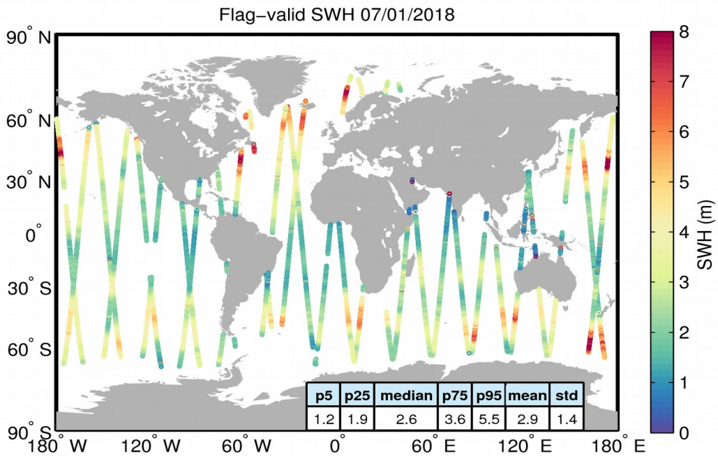
Figure 15. Geographical distribution of flag-valid SWH data over oceans and lakes for 07/01/2018. The statistical values shown in the table refer to the SWH in m and are calculated over all measurements shown in the figure.
