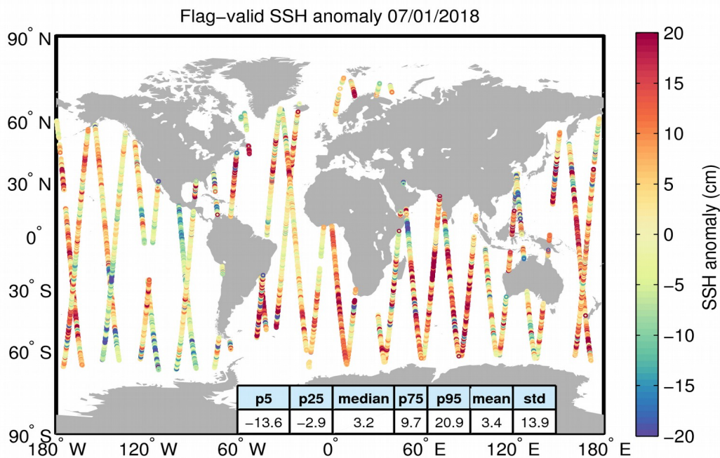
Figure 5. Geographical distribution of flag-valid 1-Hz SSH anomaly data over oceans and lakes for 07/01/2018. The statistical values shown in the table refer to the SSH anomaly in cm and are calculated over all measurements shown in the figure.
