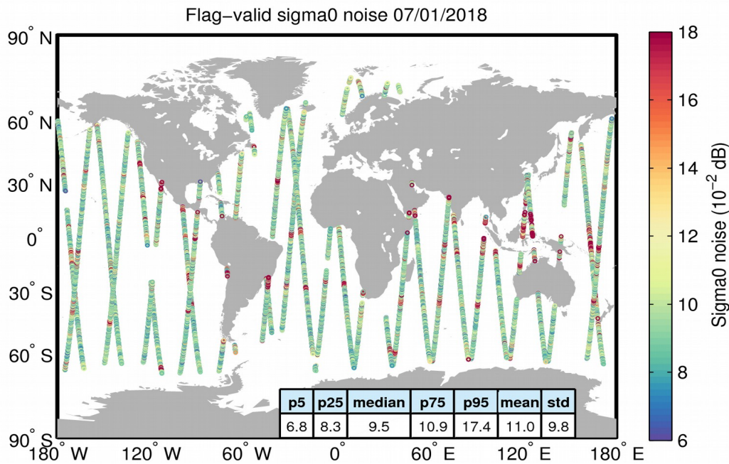
Figure 26. Geographical distribution of flag-valid 20-Hz sigma0 measurement noise over oceans and lakes for 07/01/2018. The statistical values shown in the table refer to the sigma0 noise and are calculated over all measurements shown in the figure.
