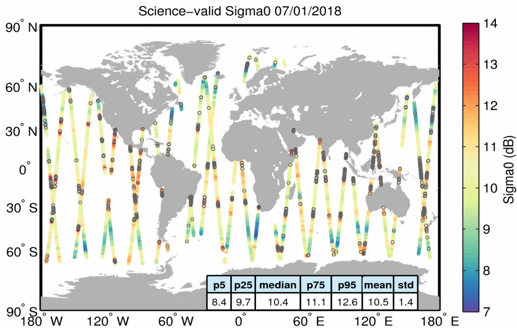
Figure 27. Geographical distribution of science-valid sigma0 data over oceans and lakes for 07/01/2018. The statistical values shown in the table refer to the sigma0 in dB and are calculated over all measurements shown in the figure. Gray circles denote records that have been rejected based on the editing criteria described in Table 4.
