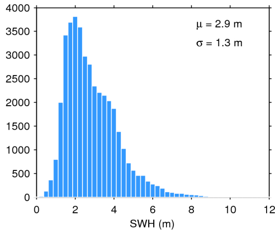
Figure 20. Histogram of science-valid SWH over oceans and lakes for 07/01/2018. The mean ( \mu ) and standard deviation ( \sigma ) are also shown. Note that values larger than 12 m are excluded from the histogram for the sake of readability but not from the computation of \mu and \sigma .
