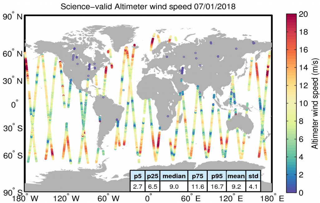
Figure 34. Geographical distribution of science-valid wind data over oceans and lakes for 07/01/2018. The statistical values shown in the table refer to the wind in m/s and are calculated over all measurements shown in the figure. Gray circles denote records that have been rejected based on the editing criteria described in Table 5.
