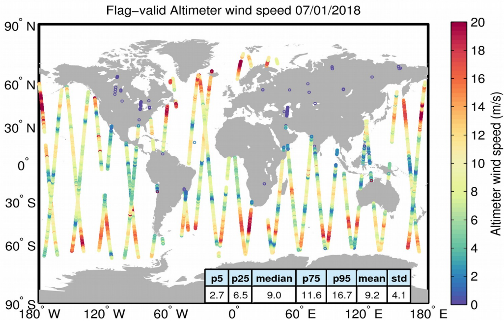
Figure 31. Geographical distribution of flag-valid wind data over oceans and lakes for 07/01/2018. The statistical values shown in the table refer to the wind in m/s and are calculated over all measurements shown in the figure.
