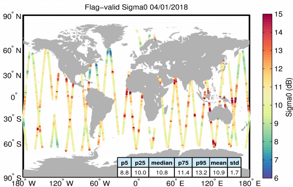
Figure 23. Geographical distribution of flag-valid sigma0 data over oceans and lakes for 04/01/2018. The statistical values shown in the table refer to the sigma0 in dB and are calculated over all measurements shown in the figure.
