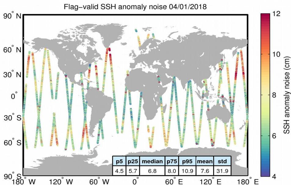
Figure 8. Geographical distribution of flag-valid 20-Hz SSH anomaly measurement noise over oceans and lakes for 04/01/2018. The statistical values shown in the table refer to the SSH anomaly noise and are calculated over all measurements shown in the figure.
