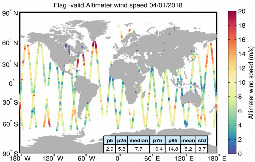
Figure 31. Geographical distribution of flag-valid wind data over oceans and lakes for 04/01/2018. The statistical values shown in the table refer to the wind in m/s and are calculated over all measurements shown in the figure.
