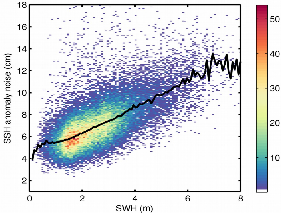
Figure 9. 2D histogram showing flag-valid SSH anomaly noise as a function of SWH for 04/01/2018. The black line denotes the median SSH anomaly noise as a function of SWH.
