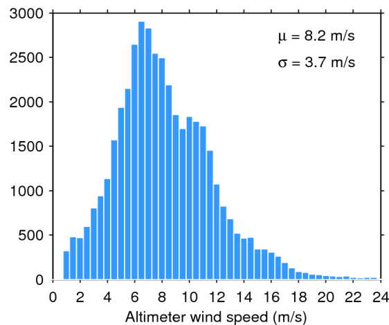
Figure 35. Histogram of science-valid wind over oceans and lakes for 04/01/2018. The mean ( \mu ) and standard deviation ( \sigma ) are also shown. Note that values larger than 24 m/s are excluded from the histogram for the sake of readability but not from the computation of \mu and \sigma .
