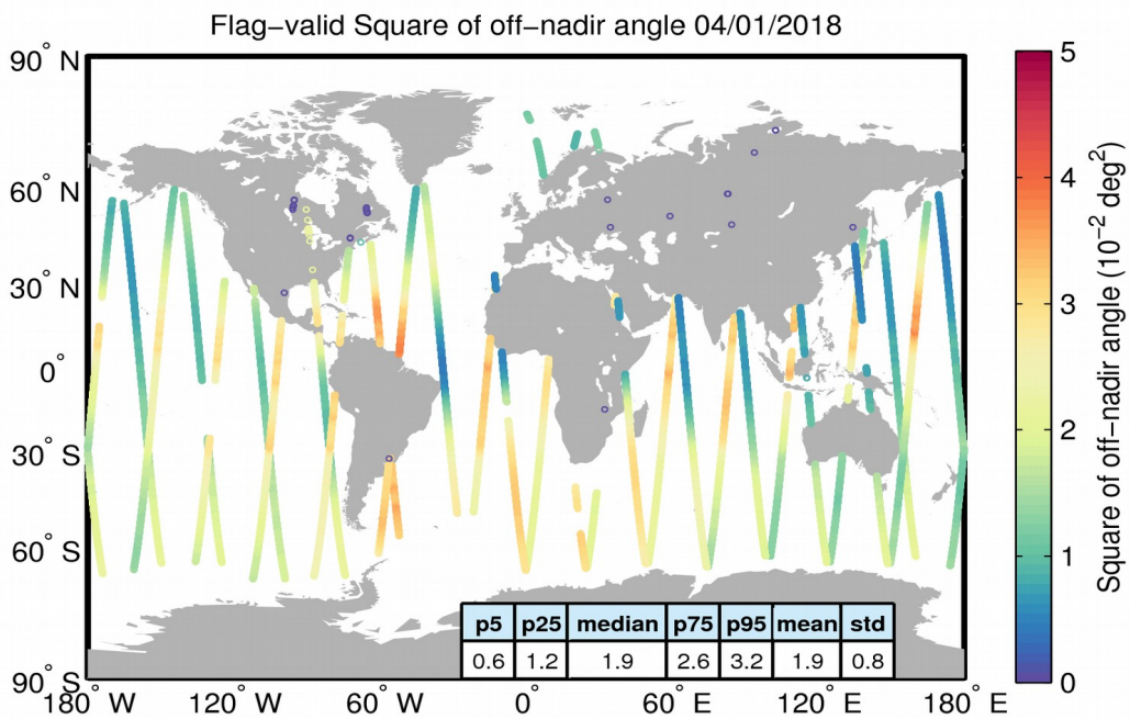
Figure 37. Geographical distribution of flag-valid mispointing data over oceans and lakes for 04/01/2018. The statistical values shown in the table refer to the mispointing in 10^{-2} deg 2 and are calculated over all measurements shown in the figure.
