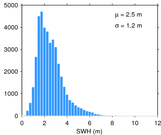
Figure 20. Histogram of science-valid SWH over oceans and lakes for 04/01/2018. The mean ( \mu ) and standard deviation ( \sigma ) are also shown. Note that values larger than 12 m are excluded from the histogram for the sake of readability but not from the computation of \mu and \sigma .
