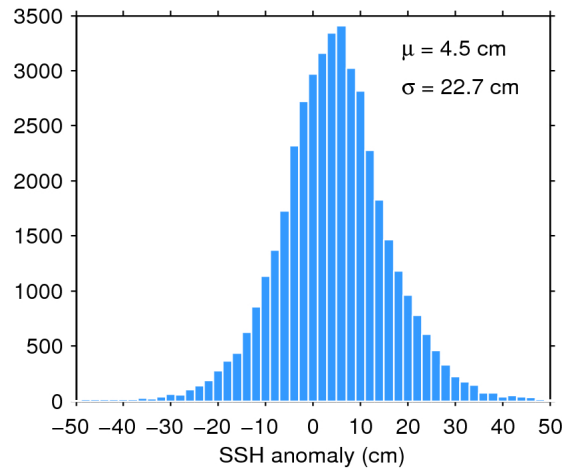
Figure 7. Histogram of flag-valid SSH anomaly over oceans and lakes for 04/01/2018. The mean ( \mu ) and standard deviation ( \sigma ) are also shown. Note that values outside [-50\ 50] cm are excluded from the histogram for the sake of readability but not from the computation of \mu and \sigma .
