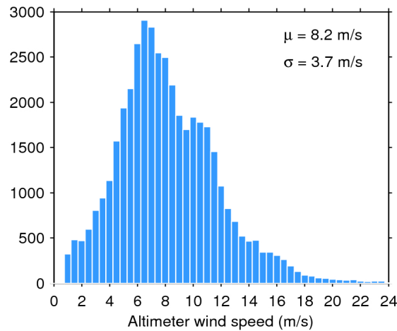
Figure 33. Histogram of flag-valid wind over oceans and lakes for 04/01/2018. The mean ( \mu ) and standard deviation ( \sigma ) are also shown. Note that values larger than 24 m/s are excluded from the histogram for the sake of readability but not from the computation of \mu and \sigma .
