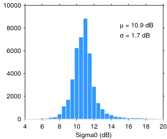
Figure 25. Histogram of flag-valid sigma0 over oceans and lakes for 04/01/2018. The mean ( \mu ) and standard deviation ( \sigma ) are also shown. Note that values outside [4 20] dB are excluded from the histogram for the sake of readability but not from the computation of \mu and \sigma .
