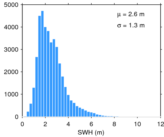
Figure 17. Histogram of flag-valid SWH over oceans and lakes for 04/01/2018. The mean ( \mu ) and standard deviation ( \sigma ) are also shown. Note that values larger than 12 m are excluded from the histogram for the sake of readability but not from the computation of \mu and \sigma .
