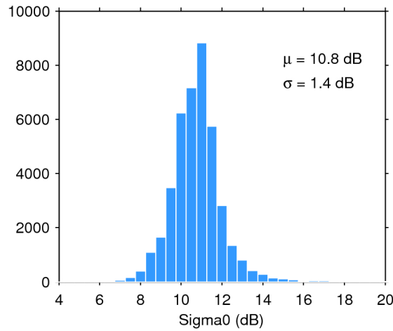
Figure 28. Histogram of science-valid sigma0 over oceans and lakes for 04/01/2018. The mean ( \mu ) and standard deviation ( \sigma ) are also shown. Note that values outside [4 20] dB are excluded from the histogram for the sake of readability but not from the computation of \mu and \sigma .
