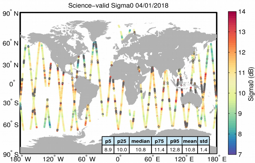
Figure 27. Geographical distribution of science-valid sigma0 data over oceans and lakes for 04/01/2018. The statistical values shown in the table refer to the sigma0 in dB and are calculated over all measurements shown in the figure. Gray circles denote records that have been rejected based on the editing criteria described in Table 4.
