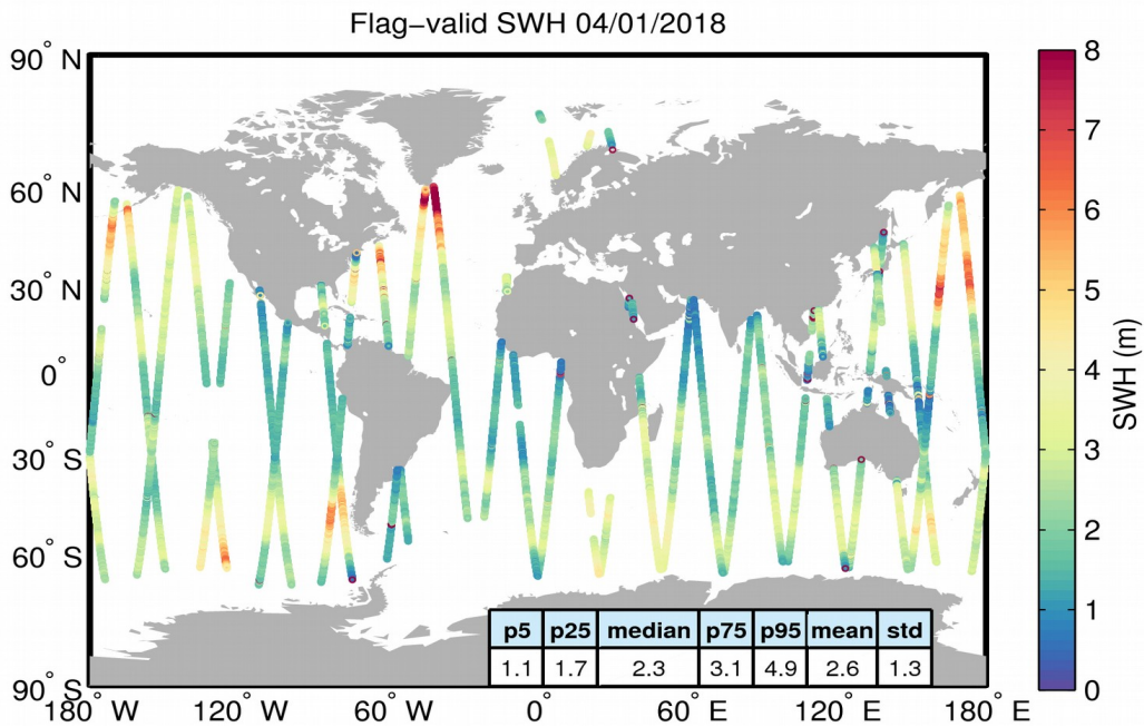
Figure 15. Geographical distribution of flag-valid SWH data over oceans and lakes for 04/01/2018. The statistical values shown in the table refer to the SWH in m and are calculated over all measurements shown in the figure.
