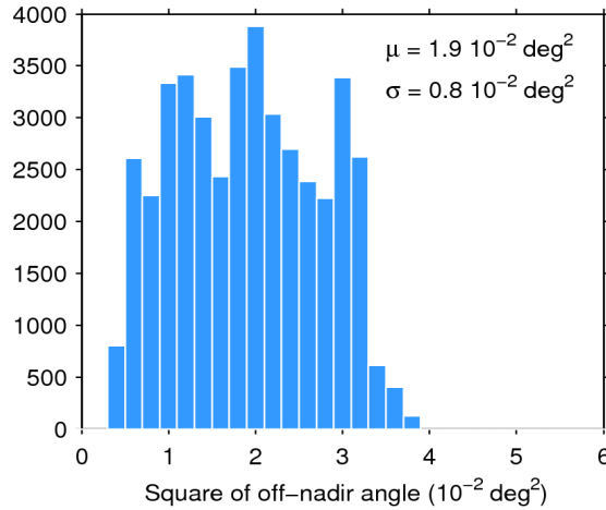
Figure 39. Histogram of flag-valid mispointing over oceans and lakes for 04/01/2018. The mean ( \mu ) and standard deviation ( \sigma ) are also shown. Note that values larger than 6 \cdot 10^{-2} \text{ deg}^2 are excluded from the histogram for the sake of readability but not from the computation of \mu and \sigma .
