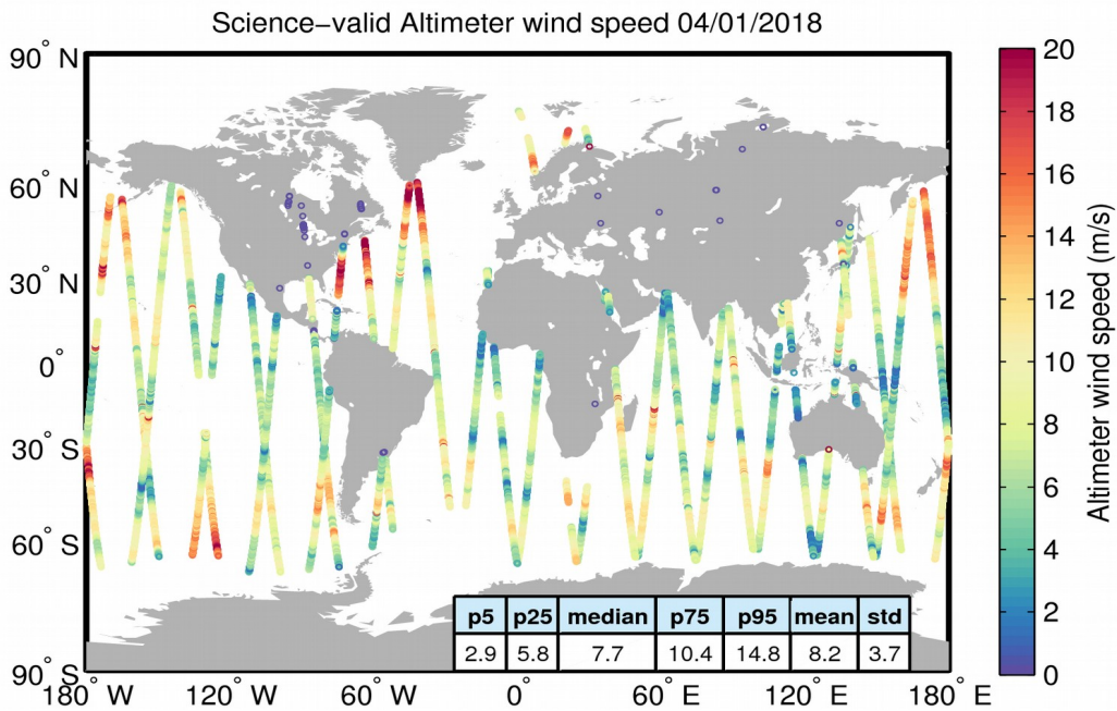
Figure 34. Geographical distribution of science-valid wind data over oceans and lakes for 04/01/2018. The statistical values shown in the table refer to the wind in m/s and are calculated over all measurements shown in the figure. Gray circles denote records that have been rejected based on the editing criteria described in Table 5.
