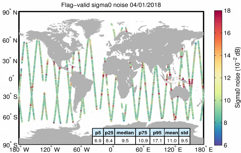
Figure 26. Geographical distribution of flag-valid 20-Hz sigma0 measurement noise over oceans and lakes for 04/01/2018. The statistical values shown in the table refer to the sigma0 noise and are calculated over all measurements shown in the figure.
