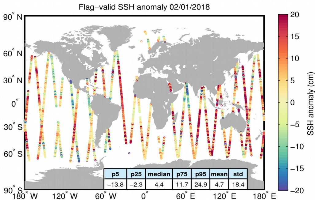
Figure 5. Geographical distribution of flag-valid 1-Hz SSH anomaly data over oceans and lakes for 02/01/2018. The statistical values shown in the table refer to the SSH anomaly in cm and are calculated over all measurements shown in the figure.
