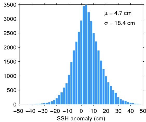
Figure 7. Histogram of flag-valid SSH anomaly over oceans and lakes for 02/01/2018. The mean ( \mu ) and standard deviation ( \sigma ) are also shown. Note that values outside [-50\ 50] cm are excluded from the histogram for the sake of readability but not from the computation of \mu and \sigma .
