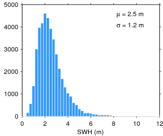
Figure 17. Histogram of flag-valid SWH over oceans and lakes for 02/01/2018. The mean ( \mu ) and standard deviation ( \sigma ) are also shown. Note that values larger than 12 m are excluded from the histogram for the sake of readability but not from the computation of \mu and \sigma .
