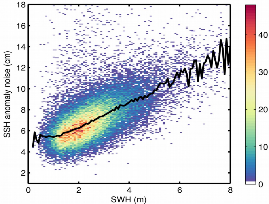
Figure 9. 2D histogram showing flag-valid SSH anomaly noise as a function of SWH for 02/01/2018. The black line denotes the median SSH anomaly noise as a function of SWH.
