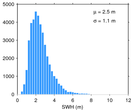
Figure 20. Histogram of science-valid SWH over oceans and lakes for 02/01/2018. The mean ( \mu ) and standard deviation ( \sigma ) are also shown. Note that values larger than 12 m are excluded from the histogram for the sake of readability but not from the computation of \mu and \sigma .
