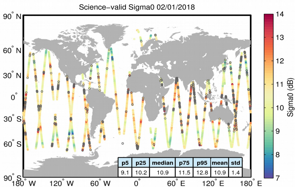
Figure 27. Geographical distribution of science-valid sigma0 data over oceans and lakes for 02/01/2018. The statistical values shown in the table refer to the sigma0 in dB and are calculated over all measurements shown in the figure. Gray circles denote records that have been rejected based on the editing criteria described in Table 4.
