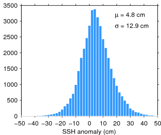
Figure 11. Histogram of science-valid SSH anomaly over oceans and lakes for 02/01/2018. The mean ( \mu ) and standard deviation ( \sigma ) are also shown. Note that values outside [-50 50] cm are excluded from the histogram for the sake of readability but not from the computation of \mu and \sigma .
