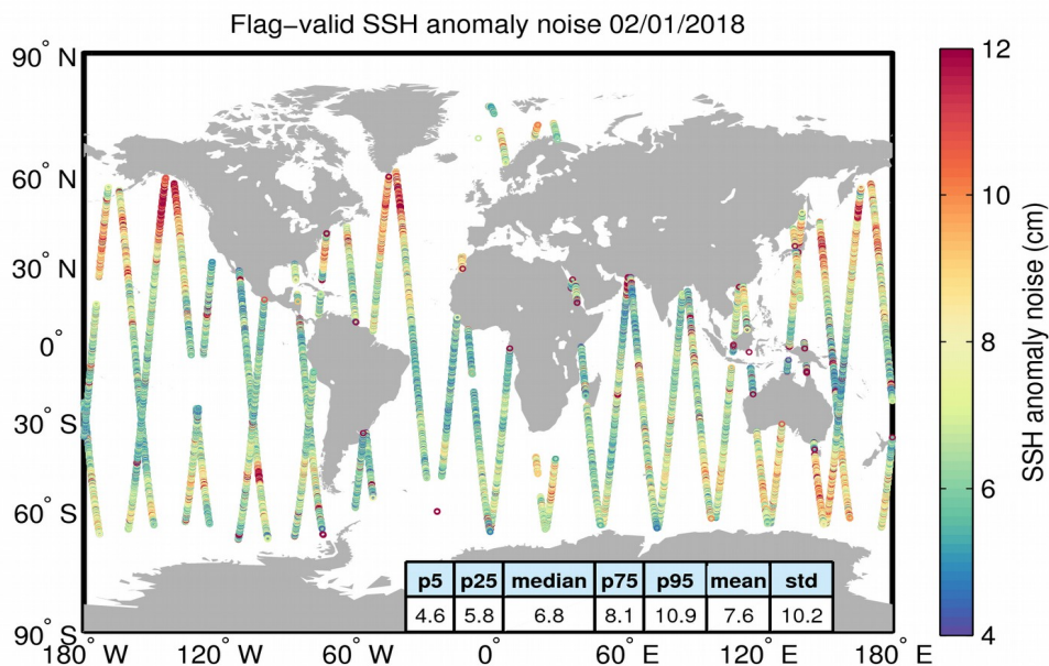
Figure 8. Geographical distribution of flag-valid 20-Hz SSH anomaly measurement noise over oceans and lakes for 02/01/2018. The statistical values shown in the table refer to the SSH anomaly noise and are calculated over all measurements shown in the figure.
