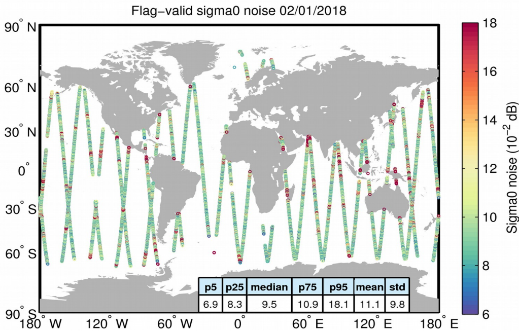
Figure 26. Geographical distribution of flag-valid 20-Hz sigma0 measurement noise over oceans and lakes for 02/01/2018. The statistical values shown in the table refer to the sigma0 noise and are calculated over all measurements shown in the figure.
