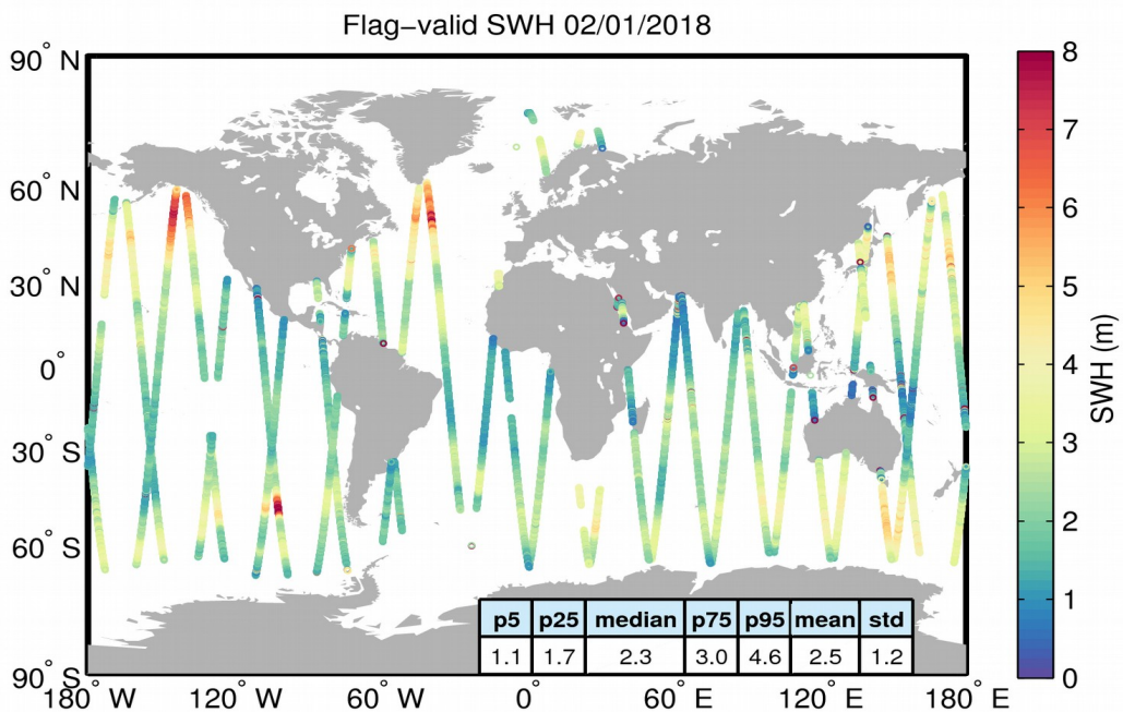
Figure 15. Geographical distribution of flag-valid SWH data over oceans and lakes for 02/01/2018. The statistical values shown in the table refer to the SWH in m and are calculated over all measurements shown in the figure.
