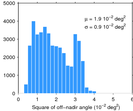
Figure 39. Histogram of flag-valid mispointing over oceans and lakes for 02/01/2018. The mean ( \mu ) and standard deviation ( \sigma ) are also shown. Note that values larger than 6 \cdot 10^{-2} \text{ deg}^2 are excluded from the histogram for the sake of readability but not from the computation of \mu and \sigma .
