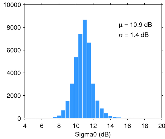
Figure 28. Histogram of science-valid sigma0 over oceans and lakes for 02/01/2018. The mean ( \mu ) and standard deviation ( \sigma ) are also shown. Note that values outside [4 20] dB are excluded from the histogram for the sake of readability but not from the computation of \mu and \sigma .
