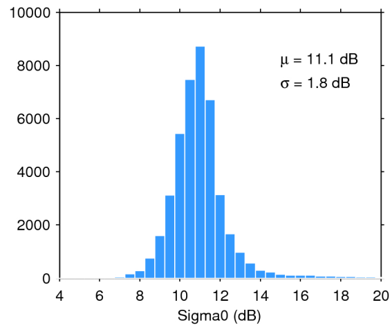
Figure 25. Histogram of flag-valid sigma0 over oceans and lakes for 02/01/2018. The mean ( \mu ) and standard deviation ( \sigma ) are also shown. Note that values outside [4 20] dB are excluded from the histogram for the sake of readability but not from the computation of \mu and \sigma .
