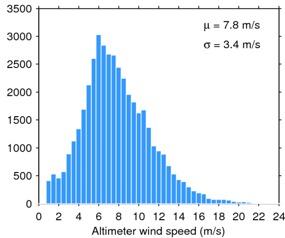
Figure 33. Histogram of flag-valid wind over oceans and lakes for 02/01/2018. The mean ( \mu ) and standard deviation ( \sigma ) are also shown. Note that values larger than 24 m/s are excluded from the histogram for the sake of readability but not from the computation of \mu and \sigma .
