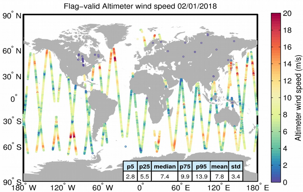
Figure 31. Geographical distribution of flag-valid wind data over oceans and lakes for 02/01/2018. The statistical values shown in the table refer to the wind in m/s and are calculated over all measurements shown in the figure.
