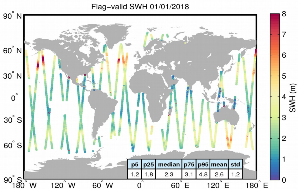
Figure 15. Geographical distribution of flag-valid SWH data over oceans and lakes for 01/01/2018. The statistical values shown in the table refer to the SWH in m and are calculated over all measurements shown in the figure.
