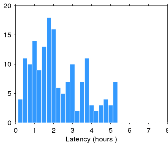
Figure 2. Histogram of the data latency for 01/01/2018. The y-axis denotes the number of files that are made available with a delay of x-hours with respect to the mean time of the records stored in the file.
