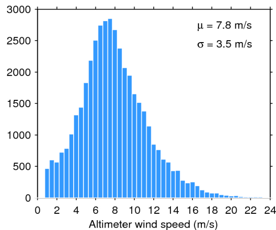
Figure 35. Histogram of science-valid wind over oceans and lakes for 01/01/2018. The mean ( \mu ) and standard deviation ( \sigma ) are also shown. Note that values larger than 24 m/s are excluded from the histogram for the sake of readability but not from the computation of \mu and \sigma .
