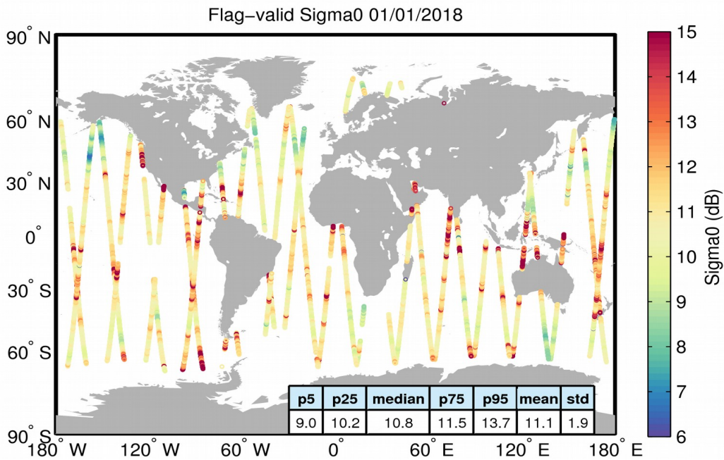
Figure 23. Geographical distribution of flag-valid sigma0 data over oceans and lakes for 01/01/2018. The statistical values shown in the table refer to the sigma0 in dB and are calculated over all measurements shown in the figure.
