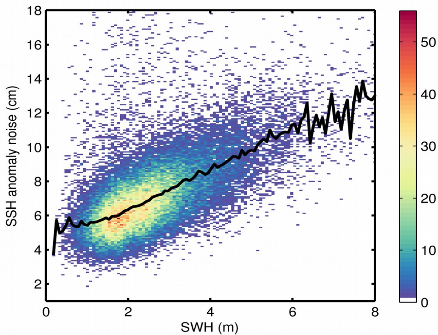
Figure 9. 2D histogram showing flag-valid SSH anomaly noise as a function of SWH for 01/01/2018. The black line denotes the median SSH anomaly noise as a function of SWH.
