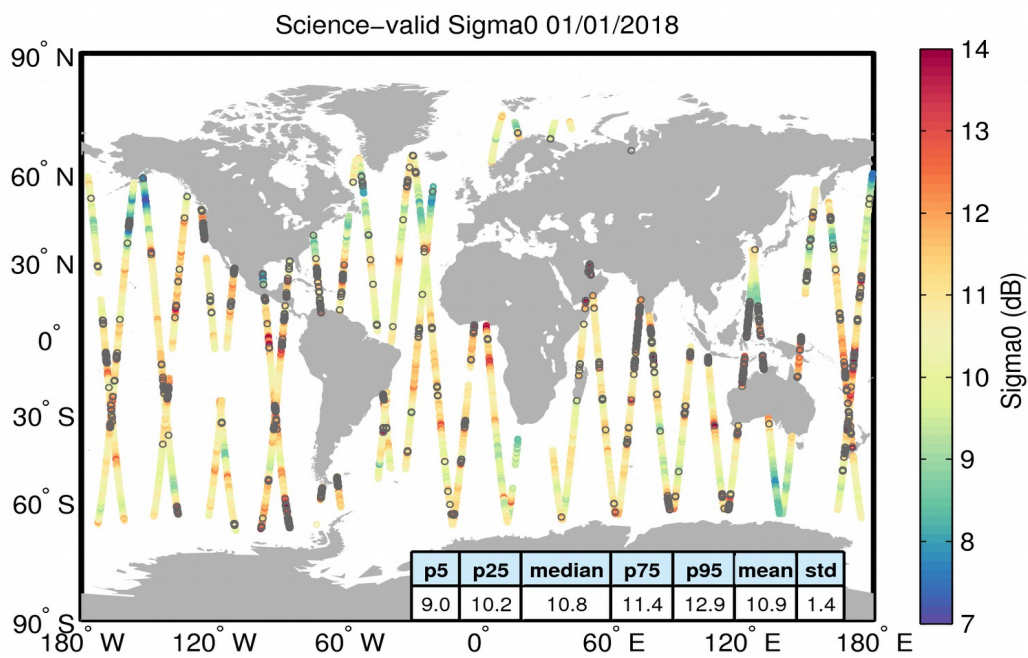
Figure 27. Geographical distribution of science-valid sigma0 data over oceans and lakes for 01/01/2018. The statistical values shown in the table refer to the sigma0 in dB and are calculated over all measurements shown in the figure. Gray circles denote records that have been rejected based on the editing criteria described in Table 4.
