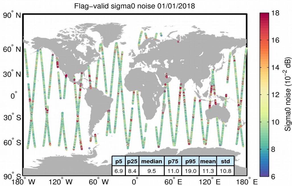
Figure 26. Geographical distribution of flag-valid 20-Hz sigma0 measurement noise over oceans and lakes for 01/01/2018. The statistical values shown in the table refer to the sigma0 noise and are calculated over all measurements shown in the figure.
