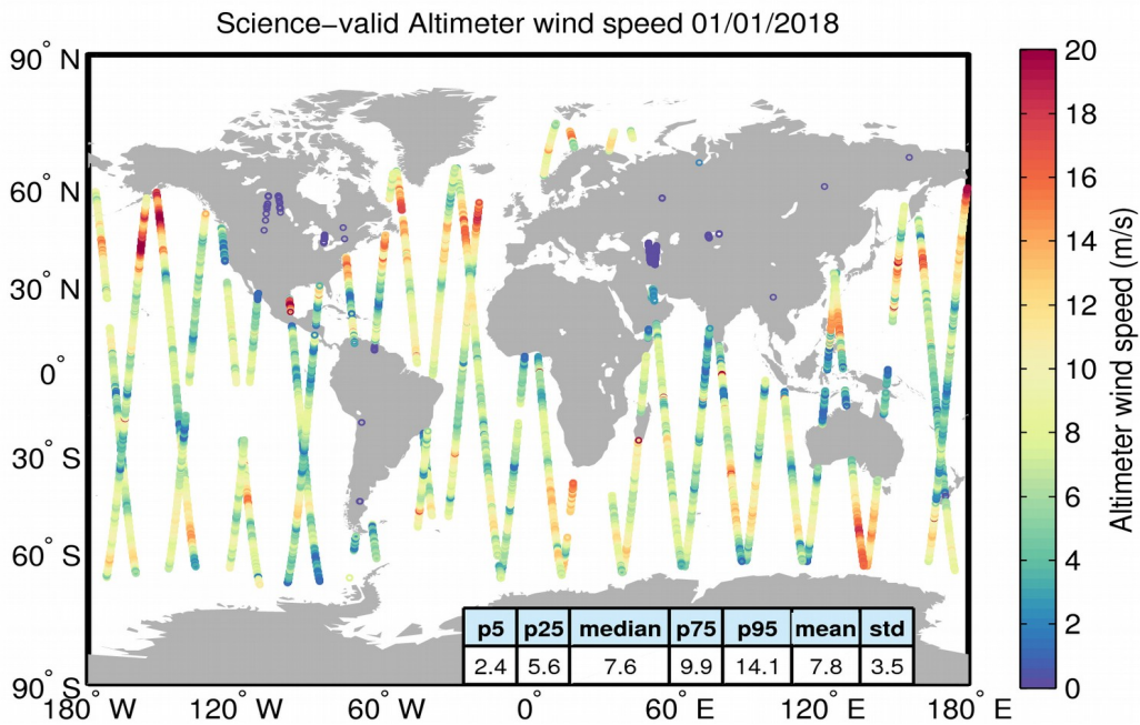
Figure 34. Geographical distribution of science-valid wind data over oceans and lakes for 01/01/2018. The statistical values shown in the table refer to the wind in m/s and are calculated over all measurements shown in the figure. Gray circles denote records that have been rejected based on the editing criteria described in Table 5.
