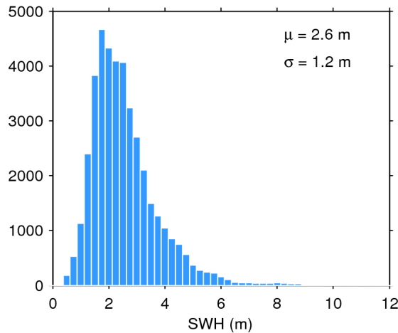
Figure 20. Histogram of science-valid SWH over oceans and lakes for 01/01/2018. The mean ( \mu ) and standard deviation ( \sigma ) are also shown. Note that values larger than 12 m are excluded from the histogram for the sake of readability but not from the computation of \mu and \sigma .
