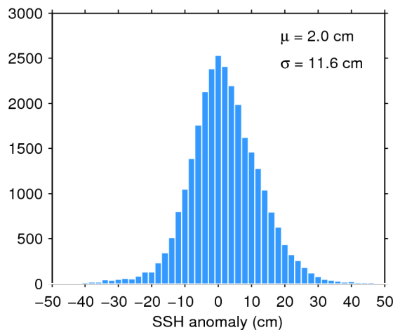
Figure 11. Histogram of science-valid SSH anomaly over oceans and lakes for 01/01/2018. The mean ( \mu ) and standard deviation ( \sigma ) are also shown. Note that values outside [-50 50] cm are excluded from the histogram for the sake of readability but not from the computation of \mu and \sigma .
