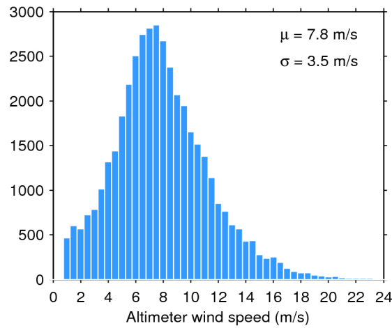
Figure 33. Histogram of flag-valid wind over oceans and lakes for 01/01/2018. The mean ( \mu ) and standard deviation ( \sigma ) are also shown. Note that values larger than 24 m/s are excluded from the histogram for the sake of readability but not from the computation of \mu and \sigma .
