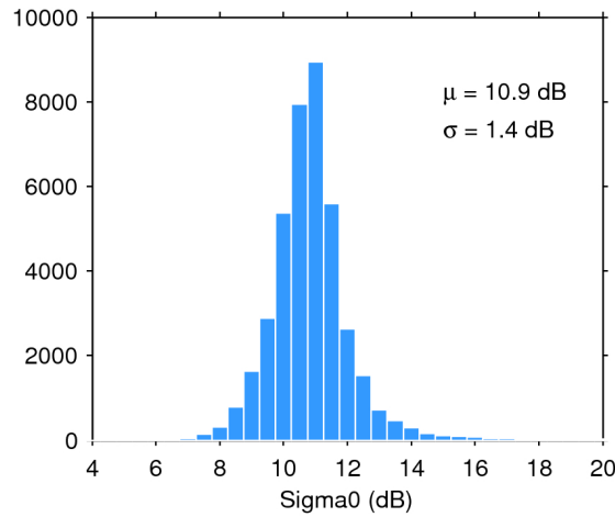
Figure 28. Histogram of science-valid sigma0 over oceans and lakes for 01/01/2018. The mean ( \mu ) and standard deviation ( \sigma ) are also shown. Note that values outside [4 20] dB are excluded from the histogram for the sake of readability but not from the computation of \mu and \sigma .
