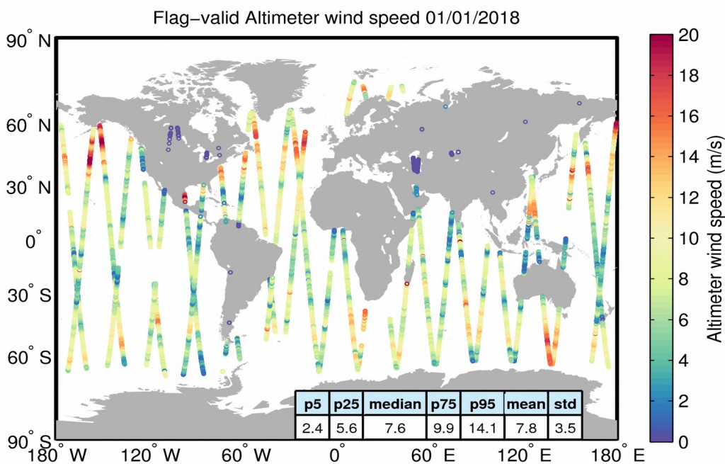
Figure 31. Geographical distribution of flag-valid wind data over oceans and lakes for 01/01/2018. The statistical values shown in the table refer to the wind in m/s and are calculated over all measurements shown in the figure.
