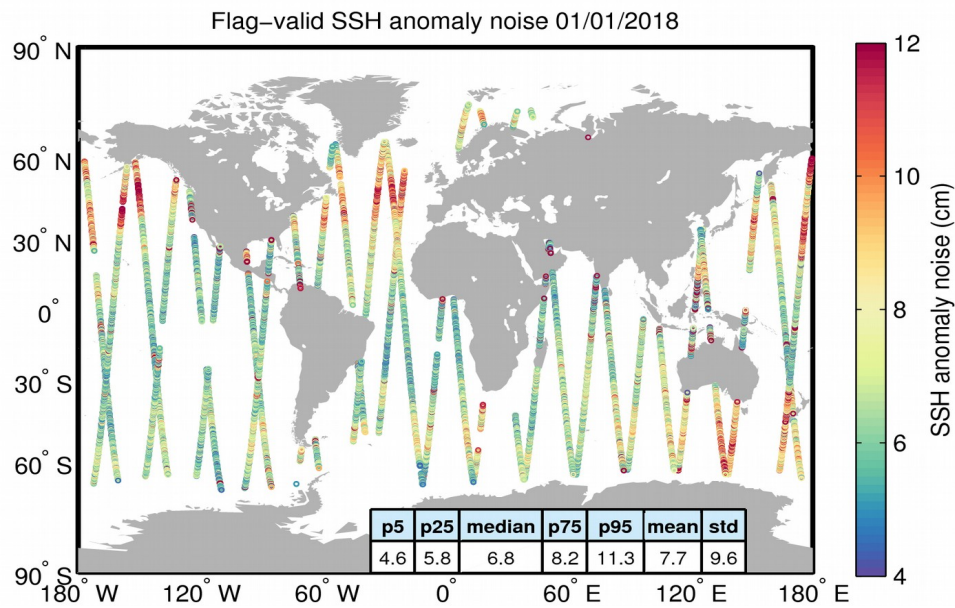
Figure 8. Geographical distribution of flag-valid 20-Hz SSH anomaly measurement noise over oceans and lakes for 01/01/2018. The statistical values shown in the table refer to the SSH anomaly noise and are calculated over all measurements shown in the figure.
