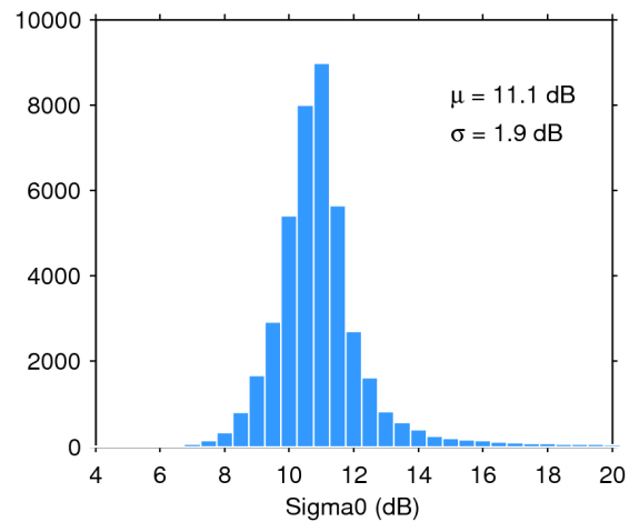
Figure 25. Histogram of flag-valid sigma0 over oceans and lakes for 01/01/2018. The mean ( \mu ) and standard deviation ( \sigma ) are also shown. Note that values outside [4 20] dB are excluded from the histogram for the sake of readability but not from the computation of \mu and \sigma .
