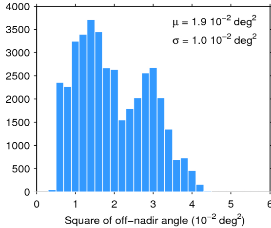
Figure 39. Histogram of flag-valid mispointing over oceans and lakes for 01/01/2018. The mean ( \mu ) and standard deviation ( \sigma ) are also shown. Note that values larger than 6 \cdot 10^{-2} \text{ deg}^2 are excluded from the histogram for the sake of readability but not from the computation of \mu and \sigma .
