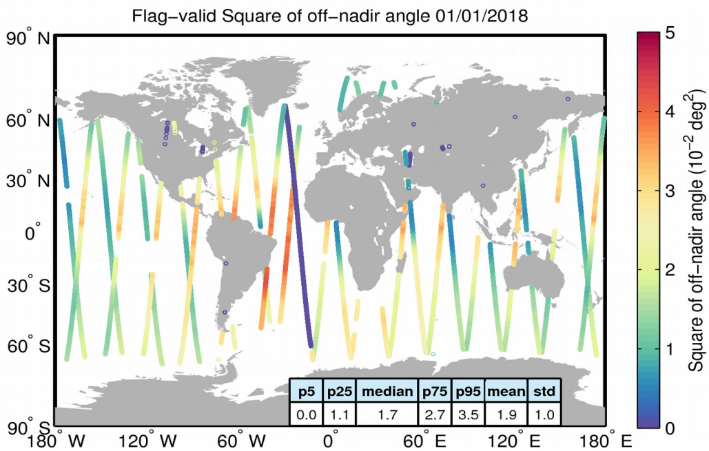
Figure 37. Geographical distribution of flag-valid mispointing data over oceans and lakes for 01/01/2018. The statistical values shown in the table refer to the mispointing in 10^{-2} deg 2 and are calculated over all measurements shown in the figure.
