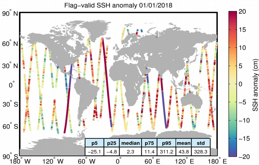
Figure 5. Geographical distribution of flag-valid 1-Hz SSH anomaly data over oceans and lakes for 01/01/2018. The statistical values shown in the table refer to the SSH anomaly in cm and are calculated over all measurements shown in the figure.
