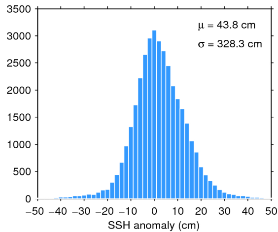
Figure 7. Histogram of flag-valid SSH anomaly over oceans and lakes for 01/01/2018. The mean ( \mu ) and standard deviation ( \sigma ) are also shown. Note that values outside [-50 50] cm are excluded from the histogram for the sake of readability but not from the computation of \mu and \sigma .
