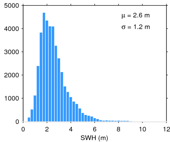
Figure 17. Histogram of flag-valid SWH over oceans and lakes for 01/01/2018. The mean ( \mu ) and standard deviation ( \sigma ) are also shown. Note that values larger than 12 m are excluded from the histogram for the sake of readability but not from the computation of \mu and \sigma .
