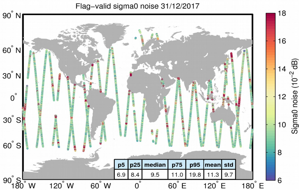
Figure 26. Geographical distribution of flag-valid 20-Hz sigma0 measurement noise over oceans and lakes for 31/12/2017. The statistical values shown in the table refer to the sigma0 noise and are calculated over all measurements shown in the figure.
