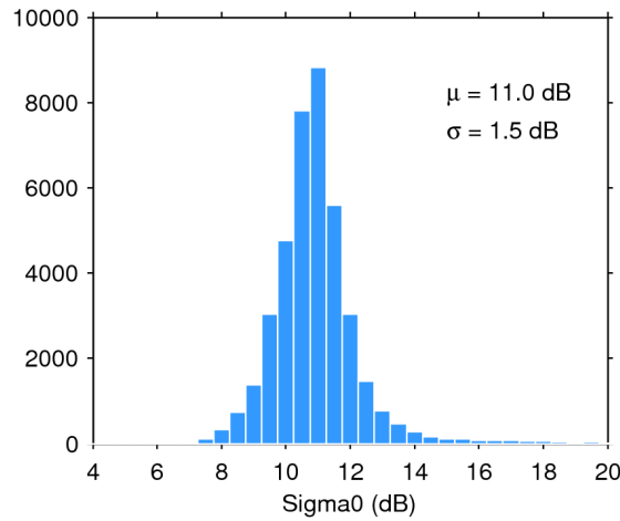
Figure 28. Histogram of science-valid sigma0 over oceans and lakes for 31/12/2017. The mean ( \mu ) and standard deviation ( \sigma ) are also shown. Note that values outside [4 20] dB are excluded from the histogram for the sake of readability but not from the computation of \mu and \sigma .
