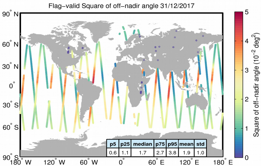
Figure 37. Geographical distribution of flag-valid mispointing data over oceans and lakes for 31/12/2017. The statistical values shown in the table refer to the mispointing in 10^{-2} deg 2 and are calculated over all measurements shown in the figure.
