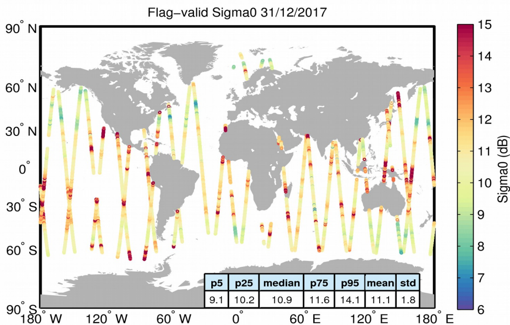
Figure 23. Geographical distribution of flag-valid sigma0 data over oceans and lakes for 31/12/2017. The statistical values shown in the table refer to the sigma0 in dB and are calculated over all measurements shown in the figure.
