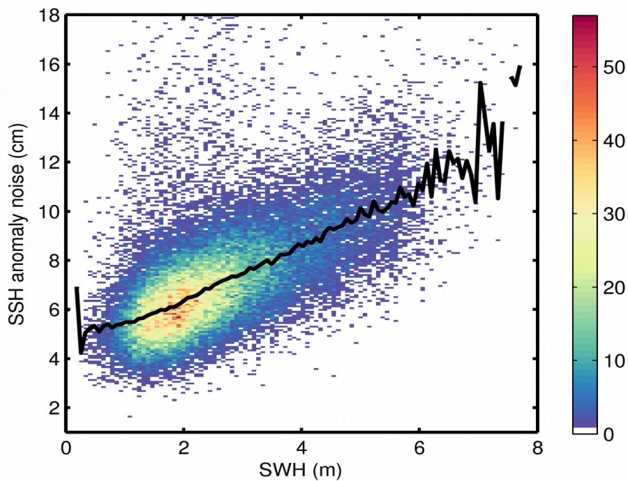
Figure 9. 2D histogram showing flag-valid SSH anomaly noise as a function of SWH for 31/12/2017. The black line denotes the median SSH anomaly noise as a function of SWH.
