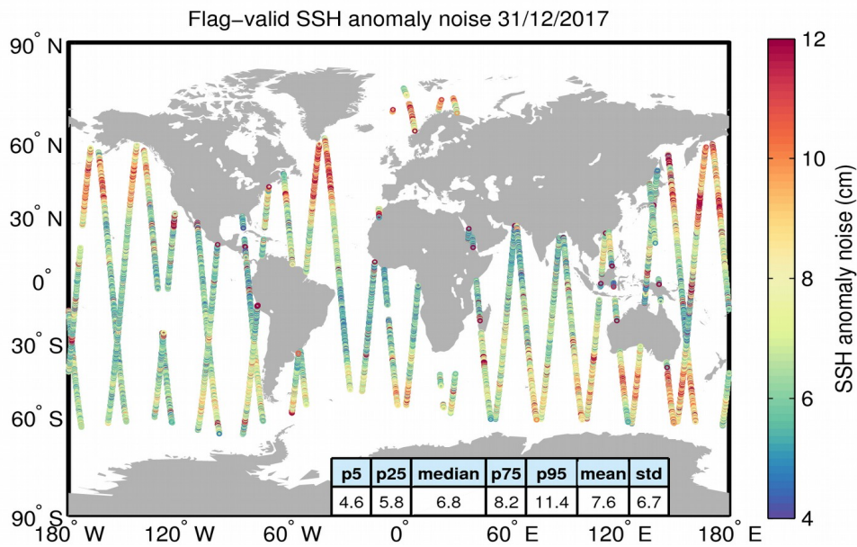
Figure 8. Geographical distribution of flag-valid 20-Hz SSH anomaly measurement noise over oceans and lakes for 31/12/2017. The statistical values shown in the table refer to the SSH anomaly noise and are calculated over all measurements shown in the figure.
