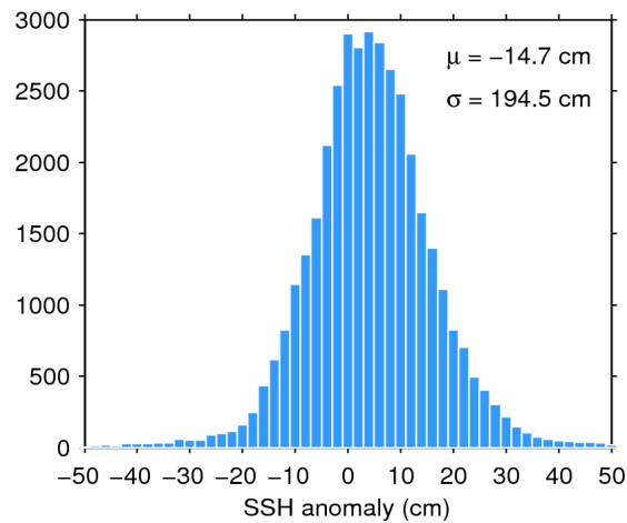
Figure 7. Histogram of flag-valid SSH anomaly over oceans and lakes for 31/12/2017. The mean ( \mu ) and standard deviation ( \sigma ) are also shown. Note that values outside [-50 50] cm are excluded from the histogram for the sake of readability but not from the computation of \mu and \sigma .
