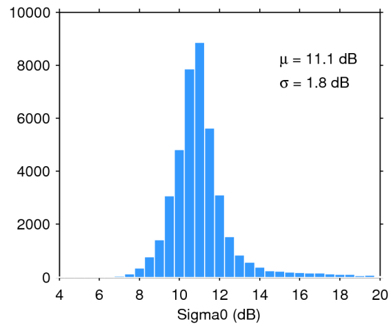
Figure 25. Histogram of flag-valid sigma0 over oceans and lakes for 31/12/2017. The mean ( \mu ) and standard deviation ( \sigma ) are also shown. Note that values outside [4 20] dB are excluded from the histogram for the sake of readability but not from the computation of \mu and \sigma .
