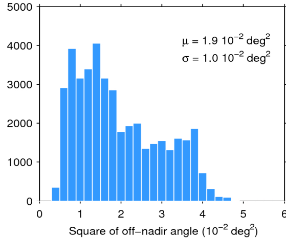
Figure 39. Histogram of flag-valid mispointing over oceans and lakes for 31/12/2017. The mean ( \mu ) and standard deviation ( \sigma ) are also shown. Note that values larger than 6 \cdot 10^{-2} \text{ deg}^2 are excluded from the histogram for the sake of readability but not from the computation of \mu and \sigma .
