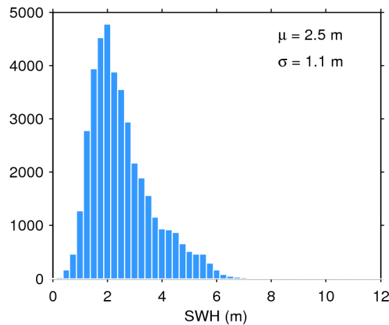
Figure 20. Histogram of science-valid SWH over oceans and lakes for 31/12/2017. The mean ( \mu ) and standard deviation ( \sigma ) are also shown. Note that values larger than 12 m are excluded from the histogram for the sake of readability but not from the computation of \mu and \sigma .
