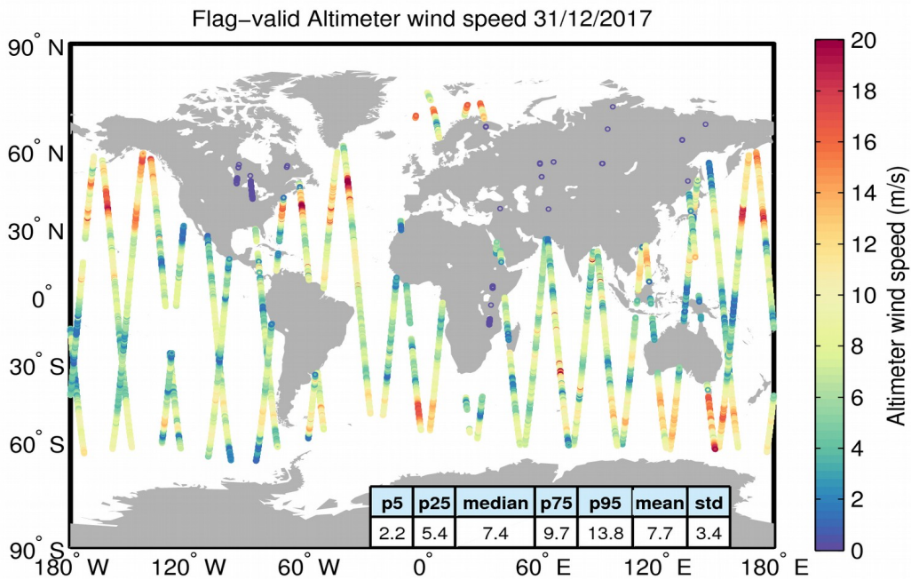
Figure 31. Geographical distribution of flag-valid wind data over oceans and lakes for 31/12/2017. The statistical values shown in the table refer to the wind in m/s and are calculated over all measurements shown in the figure.
