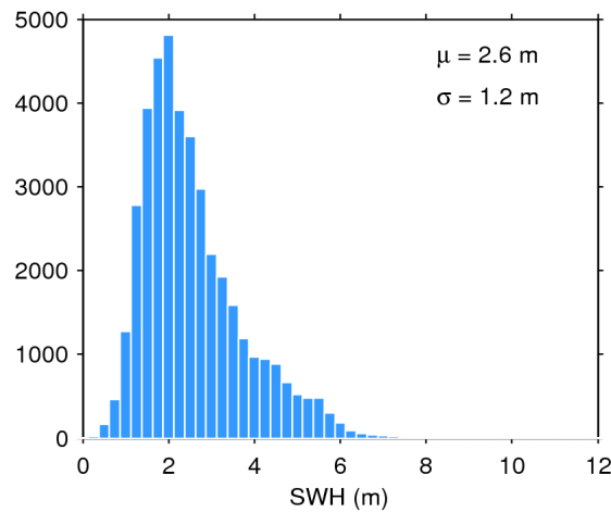
Figure 17. Histogram of flag-valid SWH over oceans and lakes for 31/12/2017. The mean ( \mu ) and standard deviation ( \sigma ) are also shown. Note that values larger than 12 m are excluded from the histogram for the sake of readability but not from the computation of \mu and \sigma .
