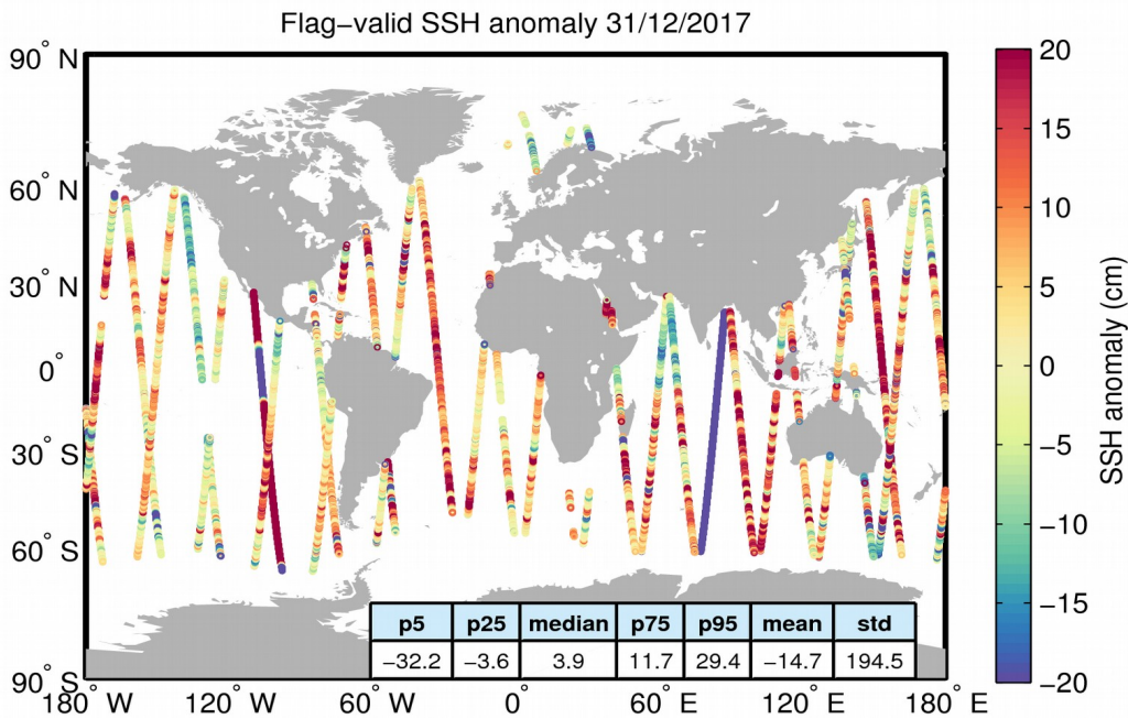
Figure 5. Geographical distribution of flag-valid 1-Hz SSH anomaly data over oceans and lakes for 31/12/2017. The statistical values shown in the table refer to the SSH anomaly in cm and are calculated over all measurements shown in the figure.
