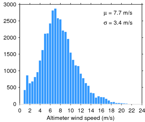
Figure 33. Histogram of flag-valid wind over oceans and lakes for 31/12/2017. The mean ( \mu ) and standard deviation ( \sigma ) are also shown. Note that values larger than 24 m/s are excluded from the histogram for the sake of readability but not from the computation of \mu and \sigma .
