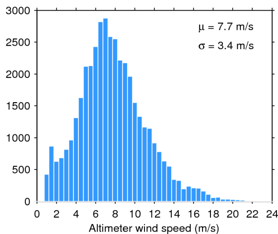
Figure 35. Histogram of science-valid wind over oceans and lakes for 31/12/2017. The mean ( \mu ) and standard deviation ( \sigma ) are also shown. Note that values larger than 24 m/s are excluded from the histogram for the sake of readability but not from the computation of \mu and \sigma .
