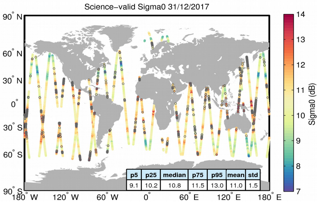
Figure 27. Geographical distribution of science-valid sigma0 data over oceans and lakes for 31/12/2017. The statistical values shown in the table refer to the sigma0 in dB and are calculated over all measurements shown in the figure. Gray circles denote records that have been rejected based on the editing criteria described in Table 4.
