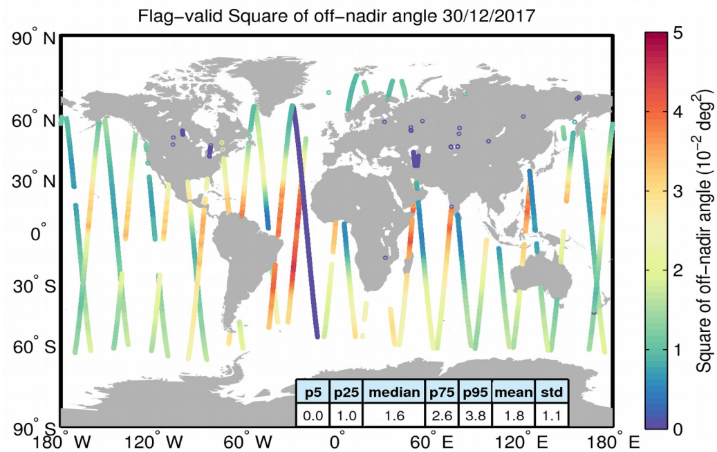
Figure 37. Geographical distribution of flag-valid mispointing data over oceans and lakes for 30/12/2017. The statistical values shown in the table refer to the mispointing in 10^{-2} deg 2 and are calculated over all measurements shown in the figure.
