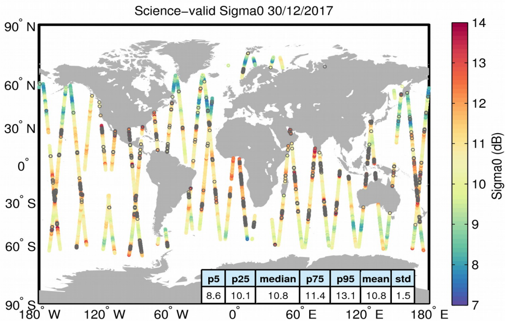
Figure 27. Geographical distribution of science-valid sigma0 data over oceans and lakes for 30/12/2017. The statistical values shown in the table refer to the sigma0 in dB and are calculated over all measurements shown in the figure. Gray circles denote records that have been rejected based on the editing criteria described in Table 4.
