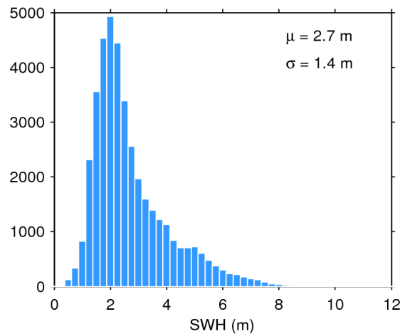
Figure 17. Histogram of flag-valid SWH over oceans and lakes for 30/12/2017. The mean ( \mu ) and standard deviation ( \sigma ) are also shown. Note that values larger than 12 m are excluded from the histogram for the sake of readability but not from the computation of \mu and \sigma .
