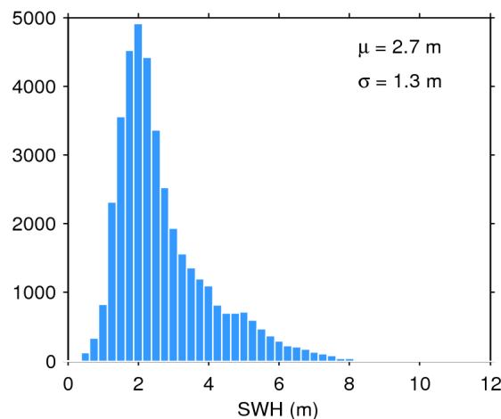
Figure 20. Histogram of science-valid SWH over oceans and lakes for 30/12/2017. The mean ( \mu ) and standard deviation ( \sigma ) are also shown. Note that values larger than 12 m are excluded from the histogram for the sake of readability but not from the computation of \mu and \sigma .
