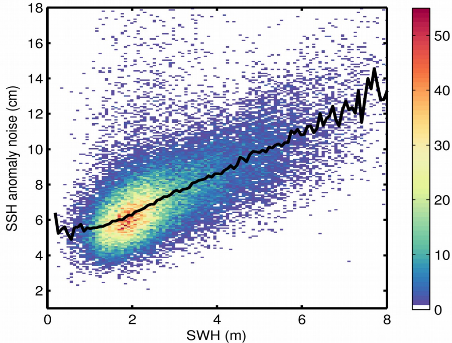
Figure 9. 2D histogram showing flag-valid SSH anomaly noise as a function of SWH for 30/12/2017. The black line denotes the median SSH anomaly noise as a function of SWH.
