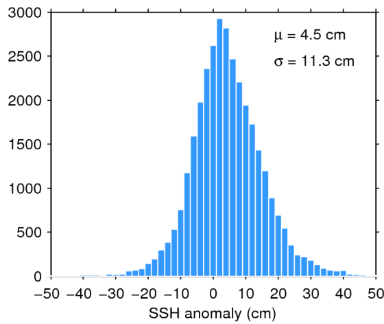
Figure 11. Histogram of science-valid SSH anomaly over oceans and lakes for 30/12/2017. The mean ( \mu ) and standard deviation ( \sigma ) are also shown. Note that values outside [-50 50] cm are excluded from the histogram for the sake of readability but not from the computation of \mu and \sigma .
