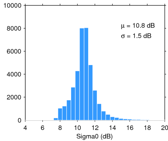
Figure 28. Histogram of science-valid sigma0 over oceans and lakes for 30/12/2017. The mean ( \mu ) and standard deviation ( \sigma ) are also shown. Note that values outside [4 20] dB are excluded from the histogram for the sake of readability but not from the computation of \mu and \sigma .
