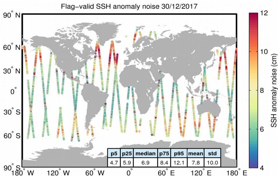
Figure 8. Geographical distribution of flag-valid 20-Hz SSH anomaly measurement noise over oceans and lakes for 30/12/2017. The statistical values shown in the table refer to the SSH anomaly noise and are calculated over all measurements shown in the figure.
