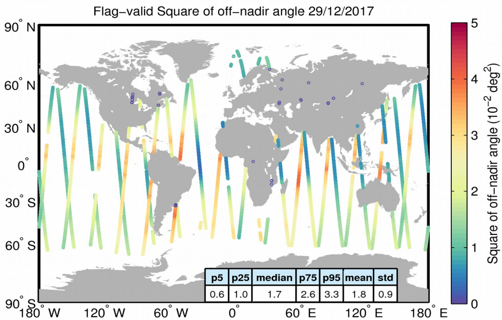
Figure 37. Geographical distribution of flag-valid mispointing data over oceans and lakes for 29/12/2017. The statistical values shown in the table refer to the mispointing in 10^{-2} deg 2 and are calculated over all measurements shown in the figure.
