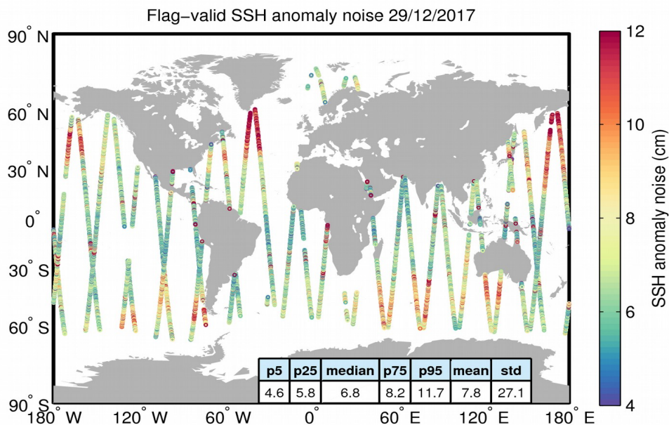
Figure 8. Geographical distribution of flag-valid 20-Hz SSH anomaly measurement noise over oceans and lakes for 29/12/2017. The statistical values shown in the table refer to the SSH anomaly noise and are calculated over all measurements shown in the figure.
