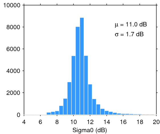
Figure 25. Histogram of flag-valid sigma0 over oceans and lakes for 29/12/2017. The mean ( \mu ) and standard deviation ( \sigma ) are also shown. Note that values outside [4 20] dB are excluded from the histogram for the sake of readability but not from the computation of \mu and \sigma .
