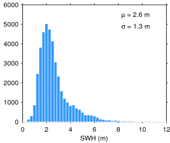
Figure 17. Histogram of flag-valid SWH over oceans and lakes for 29/12/2017. The mean ( \mu ) and standard deviation ( \sigma ) are also shown. Note that values larger than 12 m are excluded from the histogram for the sake of readability but not from the computation of \mu and \sigma .
