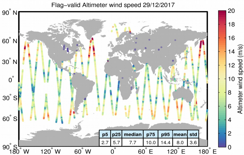
Figure 31. Geographical distribution of flag-valid wind data over oceans and lakes for 29/12/2017. The statistical values shown in the table refer to the wind in m/s and are calculated over all measurements shown in the figure.
