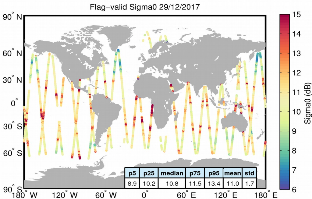
Figure 23. Geographical distribution of flag-valid sigma0 data over oceans and lakes for 29/12/2017. The statistical values shown in the table refer to the sigma0 in dB and are calculated over all measurements shown in the figure.
