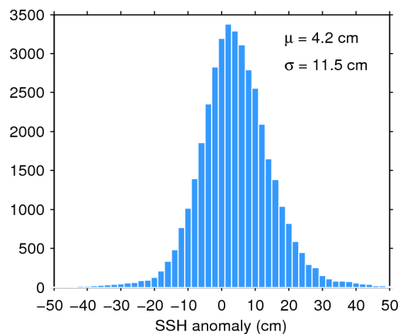
Figure 11. Histogram of science-valid SSH anomaly over oceans and lakes for 29/12/2017. The mean ( \mu ) and standard deviation ( \sigma ) are also shown. Note that values outside [-50 50] cm are excluded from the histogram for the sake of readability but not from the computation of \mu and \sigma .
