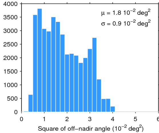
Figure 39. Histogram of flag-valid mispointing over oceans and lakes for 29/12/2017. The mean ( \mu ) and standard deviation ( \sigma ) are also shown. Note that values larger than 6 \cdot 10^{-2} \text{ deg}^2 are excluded from the histogram for the sake of readability but not from the computation of \mu and \sigma .
