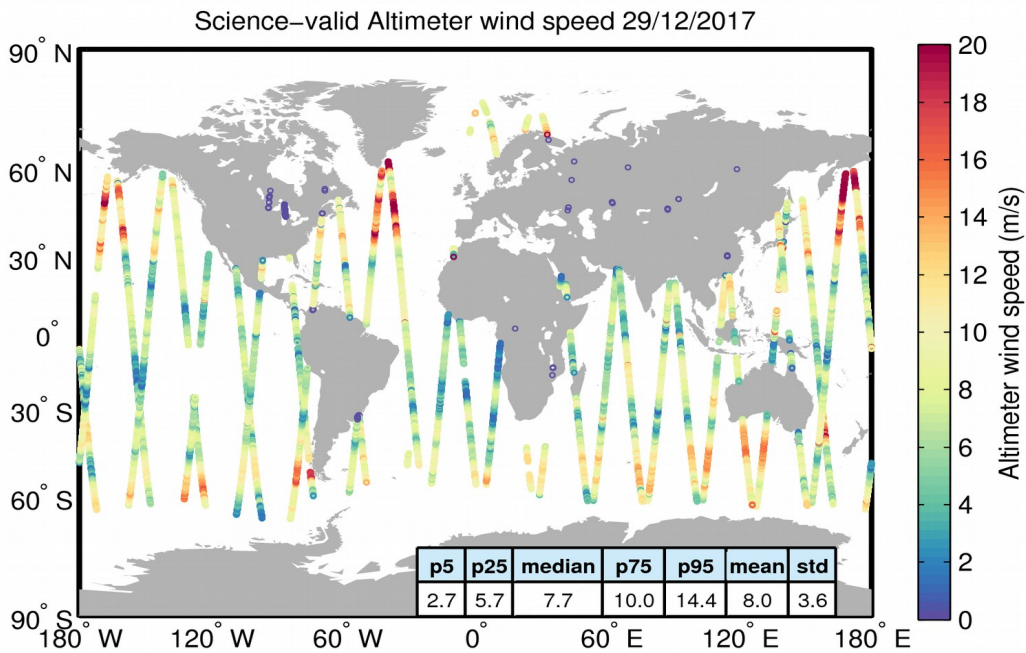
Figure 34. Geographical distribution of science-valid wind data over oceans and lakes for 29/12/2017. The statistical values shown in the table refer to the wind in m/s and are calculated over all measurements shown in the figure. Gray circles denote records that have been rejected based on the editing criteria described in Table 5.
