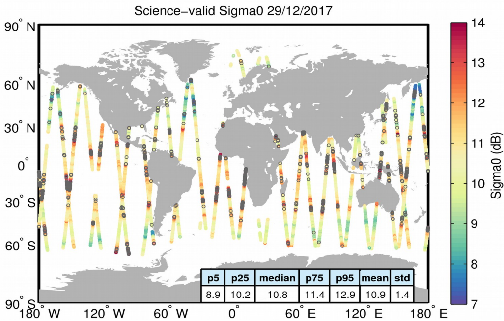
Figure 27. Geographical distribution of science-valid sigma0 data over oceans and lakes for 29/12/2017. The statistical values shown in the table refer to the sigma0 in dB and are calculated over all measurements shown in the figure. Gray circles denote records that have been rejected based on the editing criteria described in Table 4.
