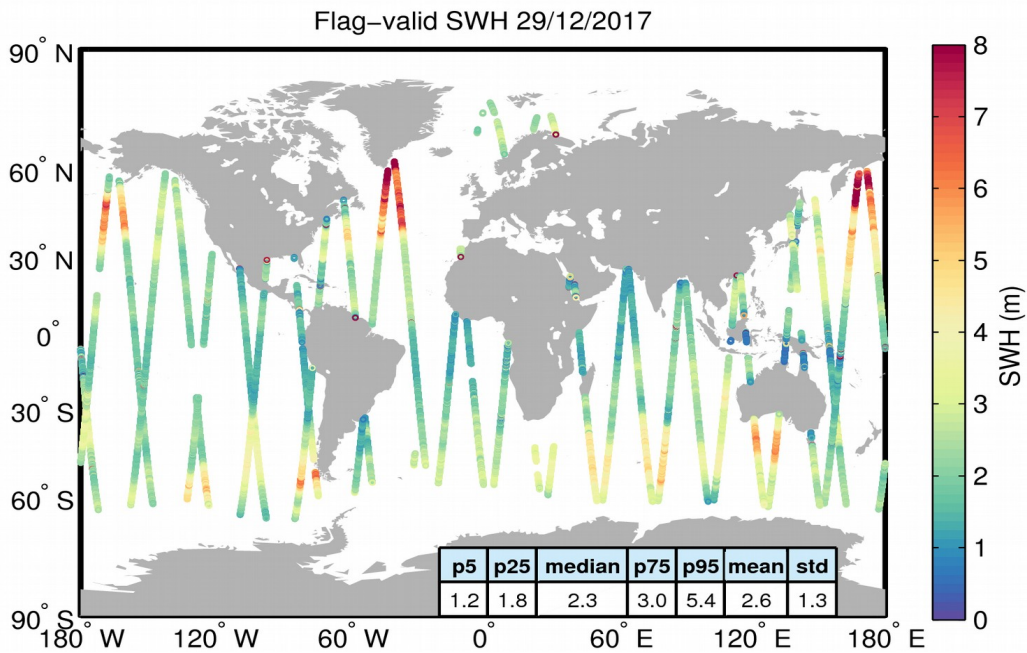
Figure 15. Geographical distribution of flag-valid SWH data over oceans and lakes for 29/12/2017. The statistical values shown in the table refer to the SWH in m and are calculated over all measurements shown in the figure.
