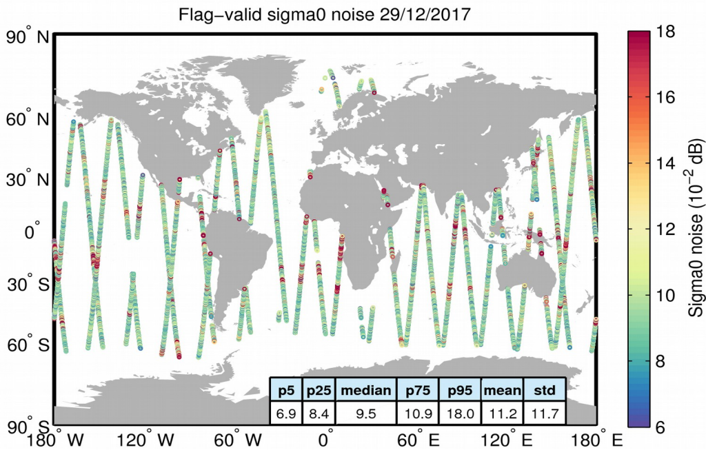
Figure 26. Geographical distribution of flag-valid 20-Hz sigma0 measurement noise over oceans and lakes for 29/12/2017. The statistical values shown in the table refer to the sigma0 noise and are calculated over all measurements shown in the figure.
