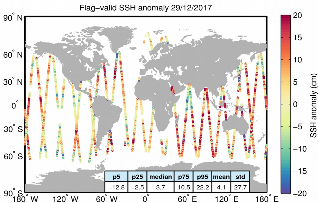
Figure 5. Geographical distribution of flag-valid 1-Hz SSH anomaly data over oceans and lakes for 29/12/2017. The statistical values shown in the table refer to the SSH anomaly in cm and are calculated over all measurements shown in the figure.
