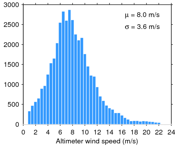
Figure 33. Histogram of flag-valid wind over oceans and lakes for 29/12/2017. The mean ( \mu ) and standard deviation ( \sigma ) are also shown. Note that values larger than 24 m/s are excluded from the histogram for the sake of readability but not from the computation of \mu and \sigma .
