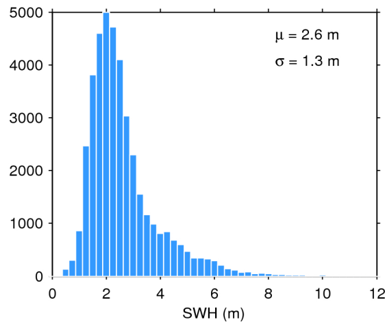
Figure 20. Histogram of science-valid SWH over oceans and lakes for 29/12/2017. The mean ( \mu ) and standard deviation ( \sigma ) are also shown. Note that values larger than 12 m are excluded from the histogram for the sake of readability but not from the computation of \mu and \sigma .
