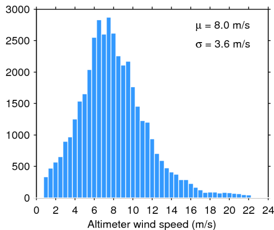
Figure 35. Histogram of science-valid wind over oceans and lakes for 29/12/2017. The mean ( \mu ) and standard deviation ( \sigma ) are also shown. Note that values larger than 24 m/s are excluded from the histogram for the sake of readability but not from the computation of \mu and \sigma .
