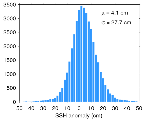
Figure 7. Histogram of flag-valid SSH anomaly over oceans and lakes for 29/12/2017. The mean ( \mu ) and standard deviation ( \sigma ) are also shown. Note that values outside [-50 50] cm are excluded from the histogram for the sake of readability but not from the computation of \mu and \sigma .
