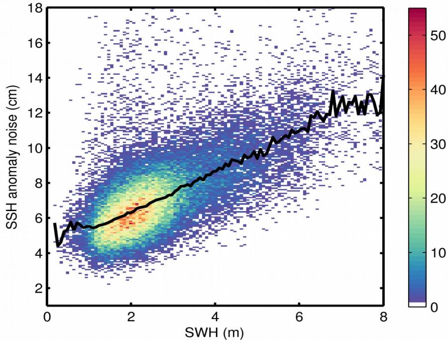
Figure 9. 2D histogram showing flag-valid SSH anomaly noise as a function of SWH for 29/12/2017. The black line denotes the median SSH anomaly noise as a function of SWH.
