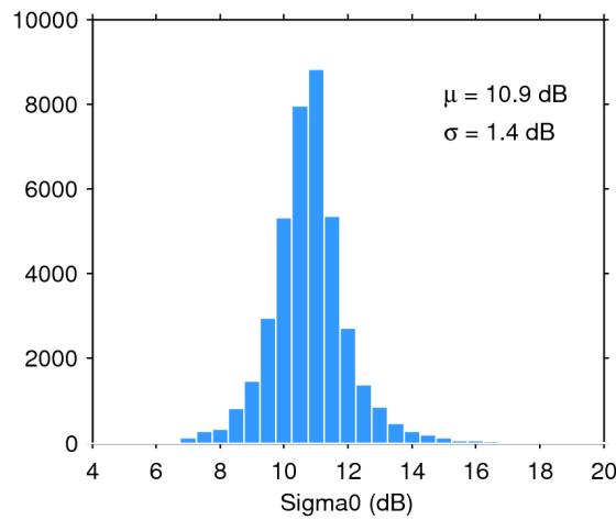
Figure 28. Histogram of science-valid sigma0 over oceans and lakes for 29/12/2017. The mean ( \mu ) and standard deviation ( \sigma ) are also shown. Note that values outside [4 20] dB are excluded from the histogram for the sake of readability but not from the computation of \mu and \sigma .
