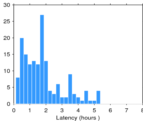
Figure 2. Histogram of the data latency for 29/12/2017. The y-axis denotes the number of files that are made available with a delay of x-hours with respect to the mean time of the records stored in the file.
