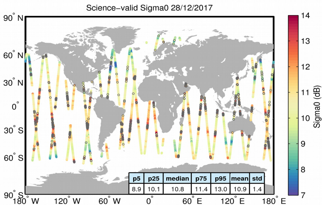
Figure 27. Geographical distribution of science-valid sigma0 data over oceans and lakes for 28/12/2017. The statistical values shown in the table refer to the sigma0 in dB and are calculated over all measurements shown in the figure. Gray circles denote records that have been rejected based on the editing criteria described in Table 4.
