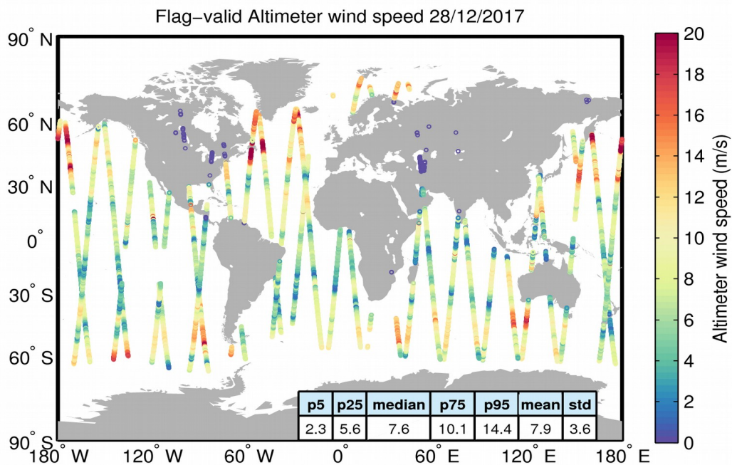
Figure 31. Geographical distribution of flag-valid wind data over oceans and lakes for 28/12/2017. The statistical values shown in the table refer to the wind in m/s and are calculated over all measurements shown in the figure.
