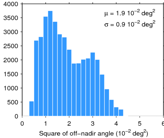
Figure 39. Histogram of flag-valid mispointing over oceans and lakes for 28/12/2017. The mean ( \mu ) and standard deviation ( \sigma ) are also shown. Note that values larger than 6 \cdot 10^{-2} \text{ deg}^2 are excluded from the histogram for the sake of readability but not from the computation of \mu and \sigma .
