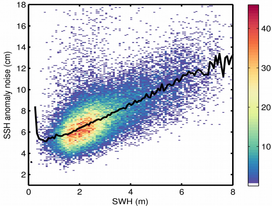
Figure 9. 2D histogram showing flag-valid SSH anomaly noise as a function of SWH for 28/12/2017. The black line denotes the median SSH anomaly noise as a function of SWH.
