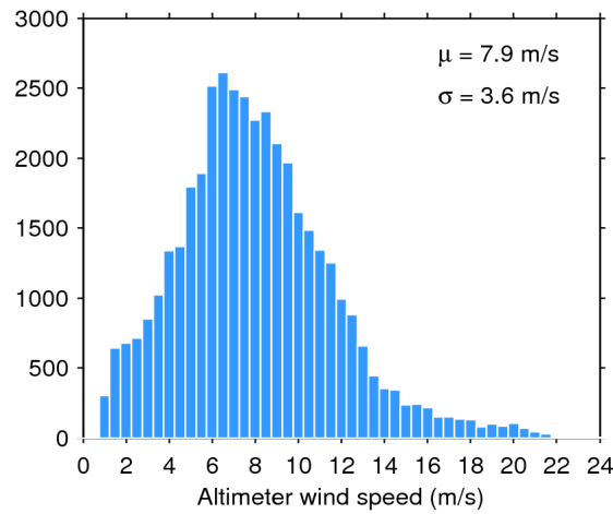
Figure 33. Histogram of flag-valid wind over oceans and lakes for 28/12/2017. The mean ( \mu ) and standard deviation ( \sigma ) are also shown. Note that values larger than 24 m/s are excluded from the histogram for the sake of readability but not from the computation of \mu and \sigma .
