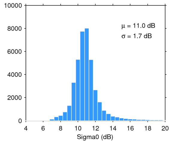
Figure 25. Histogram of flag-valid sigma0 over oceans and lakes for 28/12/2017. The mean ( \mu ) and standard deviation ( \sigma ) are also shown. Note that values outside [4 20] dB are excluded from the histogram for the sake of readability but not from the computation of \mu and \sigma .
