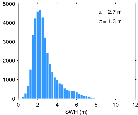
Figure 20. Histogram of science-valid SWH over oceans and lakes for 28/12/2017. The mean ( \mu ) and standard deviation ( \sigma ) are also shown. Note that values larger than 12 m are excluded from the histogram for the sake of readability but not from the computation of \mu and \sigma .
