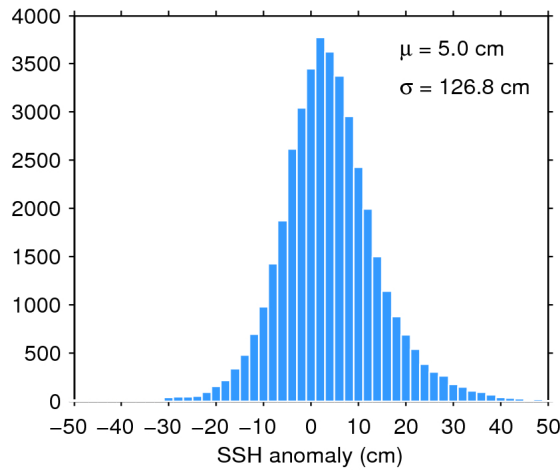
Figure 7. Histogram of flag-valid SSH anomaly over oceans and lakes for 28/12/2017. The mean ( \mu ) and standard deviation ( \sigma ) are also shown. Note that values outside [-50\ 50] cm are excluded from the histogram for the sake of readability but not from the computation of \mu and \sigma .
