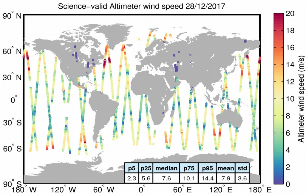
Figure 34. Geographical distribution of science-valid wind data over oceans and lakes for 28/12/2017. The statistical values shown in the table refer to the wind in m/s and are calculated over all measurements shown in the figure. Gray circles denote records that have been rejected based on the editing criteria described in Table 5.
