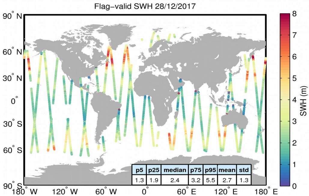
Figure 15. Geographical distribution of flag-valid SWH data over oceans and lakes for 28/12/2017. The statistical values shown in the table refer to the SWH in m and are calculated over all measurements shown in the figure.
