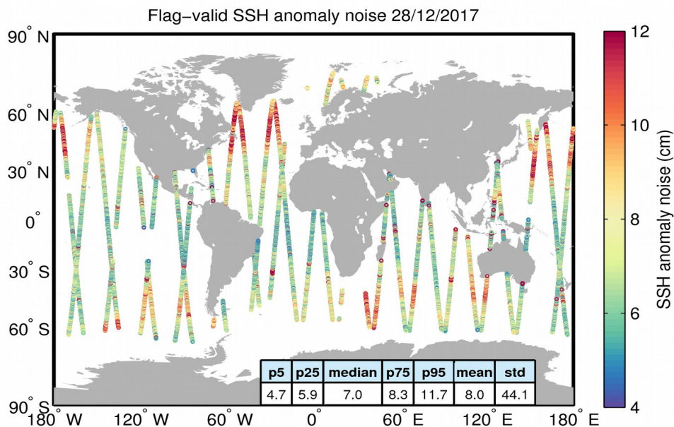
Figure 8. Geographical distribution of flag-valid 20-Hz SSH anomaly measurement noise over oceans and lakes for 28/12/2017. The statistical values shown in the table refer to the SSH anomaly noise and are calculated over all measurements shown in the figure.
