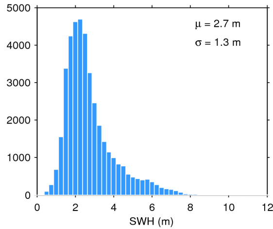
Figure 17. Histogram of flag-valid SWH over oceans and lakes for 28/12/2017. The mean ( \mu ) and standard deviation ( \sigma ) are also shown. Note that values larger than 12 m are excluded from the histogram for the sake of readability but not from the computation of \mu and \sigma .
