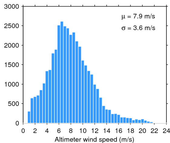
Figure 35. Histogram of science-valid wind over oceans and lakes for 28/12/2017. The mean ( \mu ) and standard deviation ( \sigma ) are also shown. Note that values larger than 24 m/s are excluded from the histogram for the sake of readability but not from the computation of \mu and \sigma .
