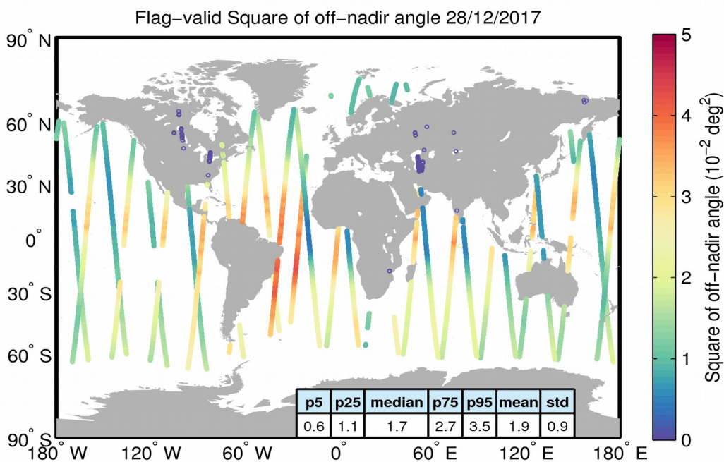
Figure 37. Geographical distribution of flag-valid mispointing data over oceans and lakes for 28/12/2017. The statistical values shown in the table refer to the mispointing in 10^{-2} deg 2 and are calculated over all measurements shown in the figure.
