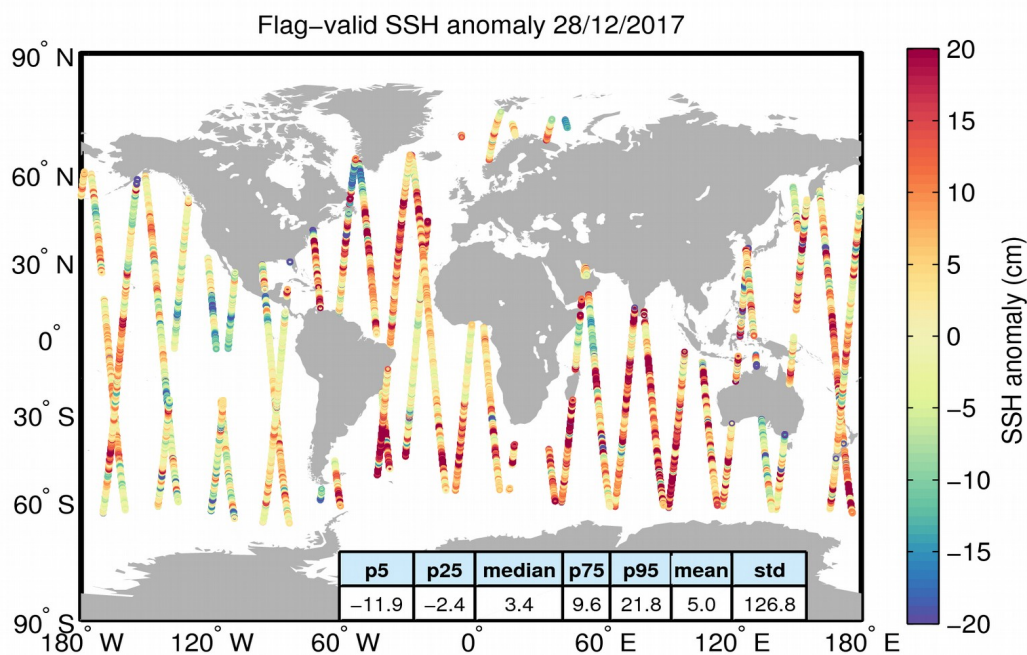
Figure 5. Geographical distribution of flag-valid 1-Hz SSH anomaly data over oceans and lakes for 28/12/2017. The statistical values shown in the table refer to the SSH anomaly in cm and are calculated over all measurements shown in the figure.
