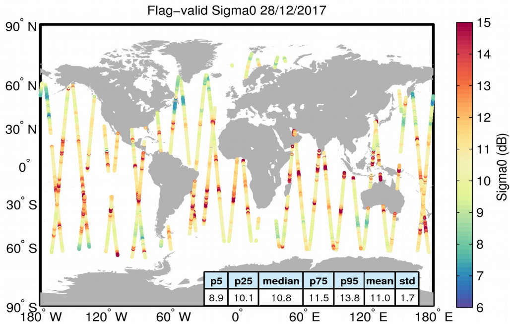
Figure 23. Geographical distribution of flag-valid sigma0 data over oceans and lakes for 28/12/2017. The statistical values shown in the table refer to the sigma0 in dB and are calculated over all measurements shown in the figure.
