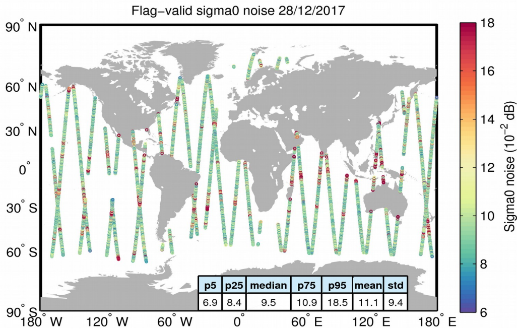
Figure 26. Geographical distribution of flag-valid 20-Hz sigma0 measurement noise over oceans and lakes for 28/12/2017. The statistical values shown in the table refer to the sigma0 noise and are calculated over all measurements shown in the figure.
