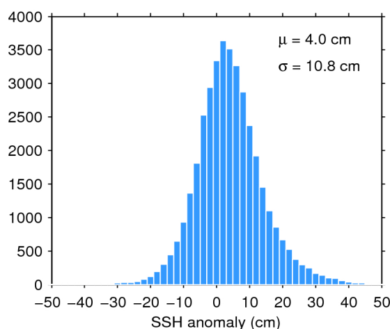
Figure 11. Histogram of science-valid SSH anomaly over oceans and lakes for 28/12/2017. The mean ( \mu ) and standard deviation ( \sigma ) are also shown. Note that values outside [-50 50] cm are excluded from the histogram for the sake of readability but not from the computation of \mu and \sigma .
