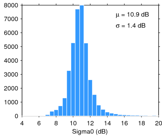
Figure 28. Histogram of science-valid sigma0 over oceans and lakes for 28/12/2017. The mean ( \mu ) and standard deviation ( \sigma ) are also shown. Note that values outside [4 20] dB are excluded from the histogram for the sake of readability but not from the computation of \mu and \sigma .
