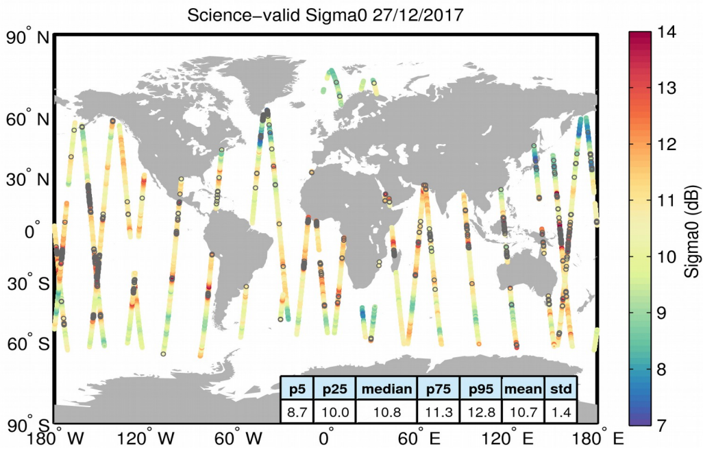
Figure 27. Geographical distribution of science-valid sigma0 data over oceans and lakes for 27/12/2017. The statistical values shown in the table refer to the sigma0 in dB and are calculated over all measurements shown in the figure. Gray circles denote records that have been rejected based on the editing criteria described in Table 4.
