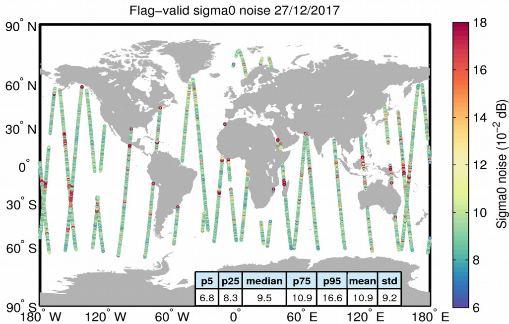
Figure 26. Geographical distribution of flag-valid 20-Hz sigma0 measurement noise over oceans and lakes for 27/12/2017. The statistical values shown in the table refer to the sigma0 noise and are calculated over all measurements shown in the figure.
