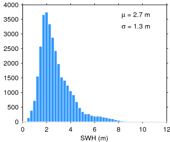
Figure 20. Histogram of science-valid SWH over oceans and lakes for 27/12/2017. The mean ( \mu ) and standard deviation ( \sigma ) are also shown. Note that values larger than 12 m are excluded from the histogram for the sake of readability but not from the computation of \mu and \sigma .
