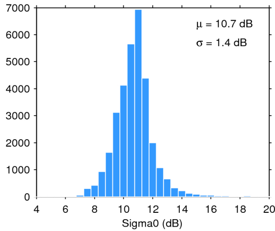
Figure 28. Histogram of science-valid sigma0 over oceans and lakes for 27/12/2017. The mean ( \mu ) and standard deviation ( \sigma ) are also shown. Note that values outside [4 20] dB are excluded from the histogram for the sake of readability but not from the computation of \mu and \sigma .
