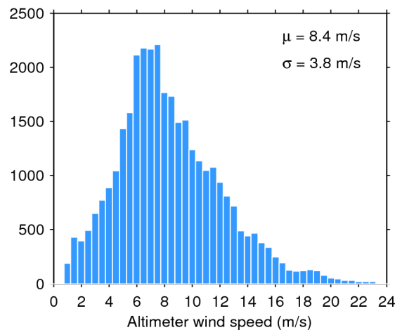
Figure 35. Histogram of science-valid wind over oceans and lakes for 27/12/2017. The mean ( \mu ) and standard deviation ( \sigma ) are also shown. Note that values larger than 24 m/s are excluded from the histogram for the sake of readability but not from the computation of \mu and \sigma .
