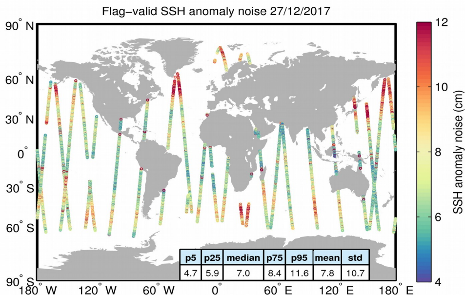
Figure 8. Geographical distribution of flag-valid 20-Hz SSH anomaly measurement noise over oceans and lakes for 27/12/2017. The statistical values shown in the table refer to the SSH anomaly noise and are calculated over all measurements shown in the figure.
