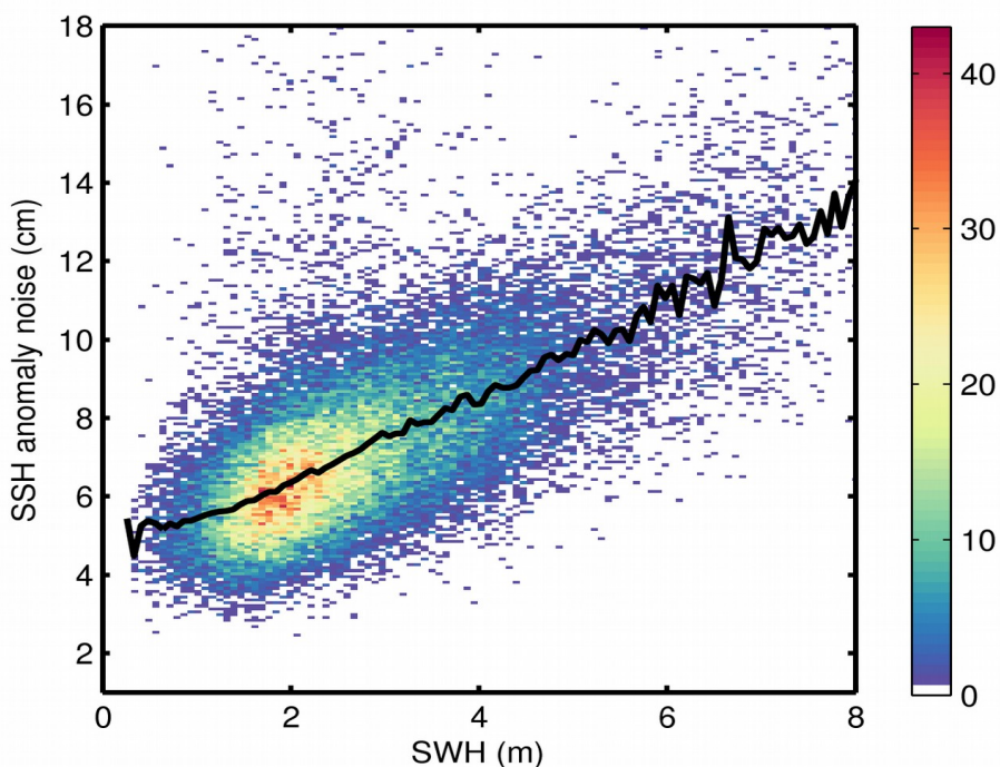
Figure 9. 2D histogram showing flag-valid SSH anomaly noise as a function of SWH for 27/12/2017. The black line denotes the median SSH anomaly noise as a function of SWH.
