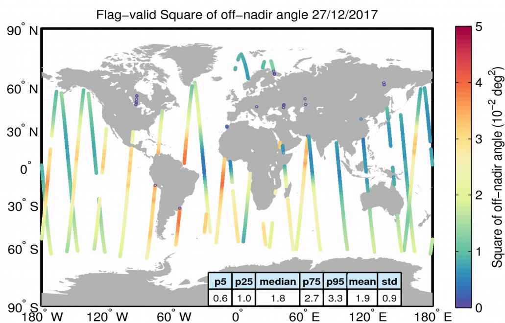
Figure 37. Geographical distribution of flag-valid mispointing data over oceans and lakes for 27/12/2017. The statistical values shown in the table refer to the mispointing in 10^{-2} deg 2 and are calculated over all measurements shown in the figure.
