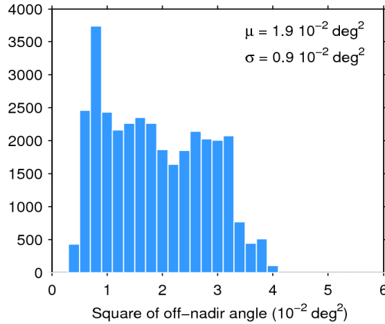
Figure 39. Histogram of flag-valid mispointing over oceans and lakes for 27/12/2017. The mean ( \mu ) and standard deviation ( \sigma ) are also shown. Note that values larger than 6 \cdot 10^{-2} \text{ deg}^2 are excluded from the histogram for the sake of readability but not from the computation of \mu and \sigma .
