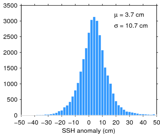
Figure 11. Histogram of science-valid SSH anomaly over oceans and lakes for 27/12/2017. The mean ( \mu ) and standard deviation ( \sigma ) are also shown. Note that values outside [-50 50] cm are excluded from the histogram for the sake of readability but not from the computation of \mu and \sigma .
