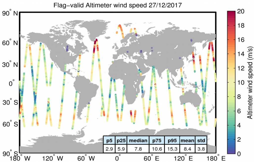
Figure 31. Geographical distribution of flag-valid wind data over oceans and lakes for 27/12/2017. The statistical values shown in the table refer to the wind in m/s and are calculated over all measurements shown in the figure.
