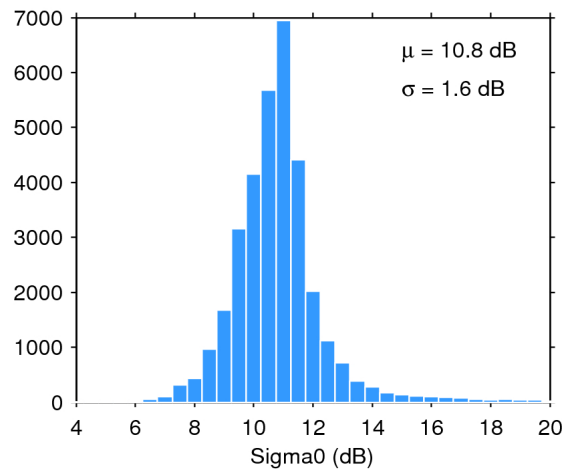
Figure 25. Histogram of flag-valid sigma0 over oceans and lakes for 27/12/2017. The mean ( \mu ) and standard deviation ( \sigma ) are also shown. Note that values outside [4 20] dB are excluded from the histogram for the sake of readability but not from the computation of \mu and \sigma .
