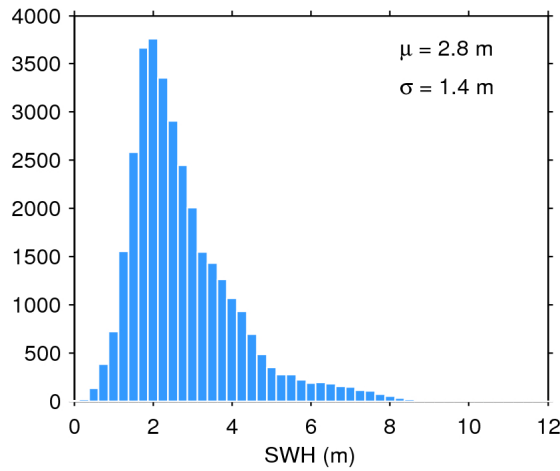
Figure 17. Histogram of flag-valid SWH over oceans and lakes for 27/12/2017. The mean ( \mu ) and standard deviation ( \sigma ) are also shown. Note that values larger than 12 m are excluded from the histogram for the sake of readability but not from the computation of \mu and \sigma .
