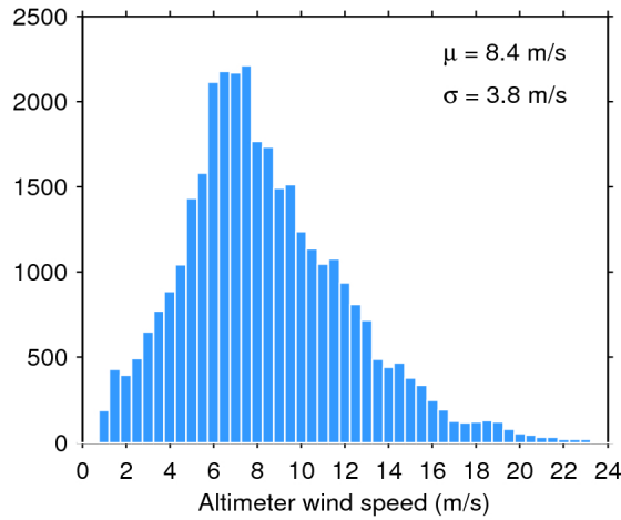
Figure 33. Histogram of flag-valid wind over oceans and lakes for 27/12/2017. The mean ( \mu ) and standard deviation ( \sigma ) are also shown. Note that values larger than 24 m/s are excluded from the histogram for the sake of readability but not from the computation of \mu and \sigma .
