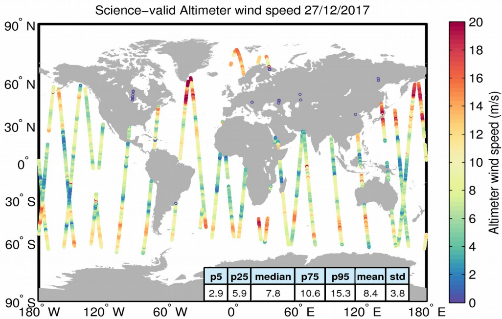
Figure 34. Geographical distribution of science-valid wind data over oceans and lakes for 27/12/2017. The statistical values shown in the table refer to the wind in m/s and are calculated over all measurements shown in the figure. Gray circles denote records that have been rejected based on the editing criteria described in Table 5.
