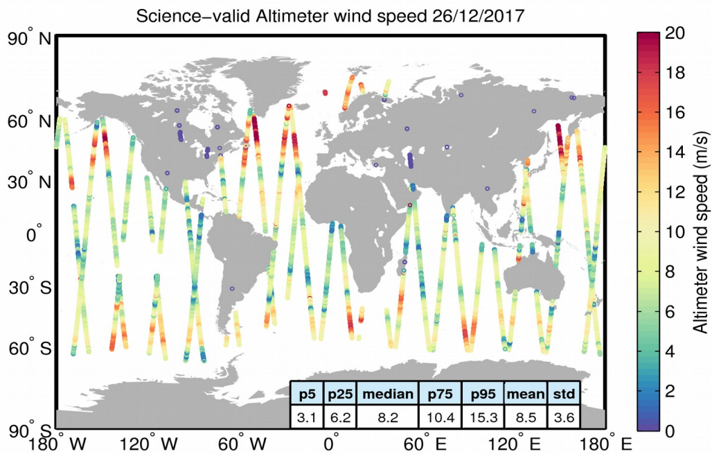
Figure 34. Geographical distribution of science-valid wind data over oceans and lakes for 26/12/2017. The statistical values shown in the table refer to the wind in m/s and are calculated over all measurements shown in the figure. Gray circles denote records that have been rejected based on the editing criteria described in Table 5.
