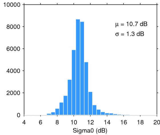
Figure 28. Histogram of science-valid sigma0 over oceans and lakes for 26/12/2017. The mean ( \mu ) and standard deviation ( \sigma ) are also shown. Note that values outside [4 20] dB are excluded from the histogram for the sake of readability but not from the computation of \mu and \sigma .
