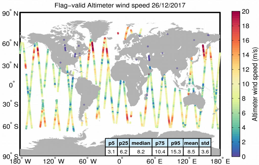
Figure 31. Geographical distribution of flag-valid wind data over oceans and lakes for 26/12/2017. The statistical values shown in the table refer to the wind in m/s and are calculated over all measurements shown in the figure.
