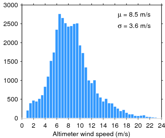
Figure 33. Histogram of flag-valid wind over oceans and lakes for 26/12/2017. The mean ( \mu ) and standard deviation ( \sigma ) are also shown. Note that values larger than 24 m/s are excluded from the histogram for the sake of readability but not from the computation of \mu and \sigma .
