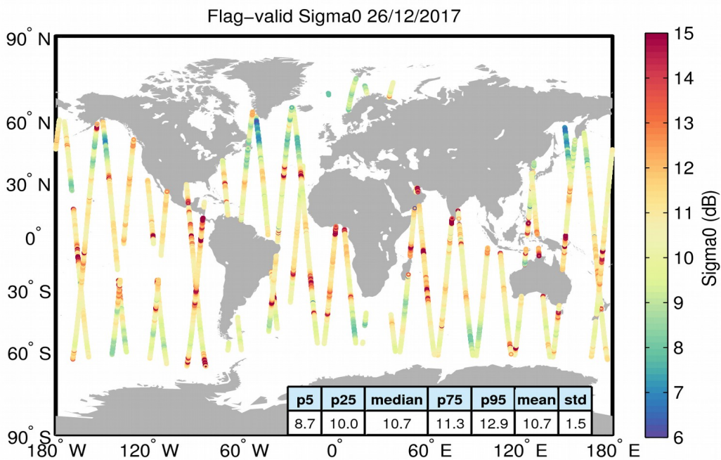
Figure 23. Geographical distribution of flag-valid sigma0 data over oceans and lakes for 26/12/2017. The statistical values shown in the table refer to the sigma0 in dB and are calculated over all measurements shown in the figure.
