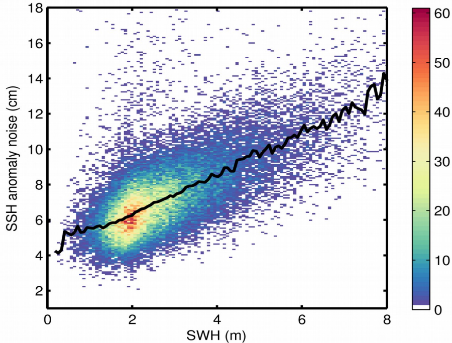
Figure 9. 2D histogram showing flag-valid SSH anomaly noise as a function of SWH for 26/12/2017. The black line denotes the median SSH anomaly noise as a function of SWH.
