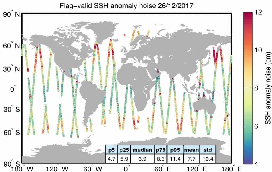
Figure 8. Geographical distribution of flag-valid 20-Hz SSH anomaly measurement noise over oceans and lakes for 26/12/2017. The statistical values shown in the table refer to the SSH anomaly noise and are calculated over all measurements shown in the figure.
