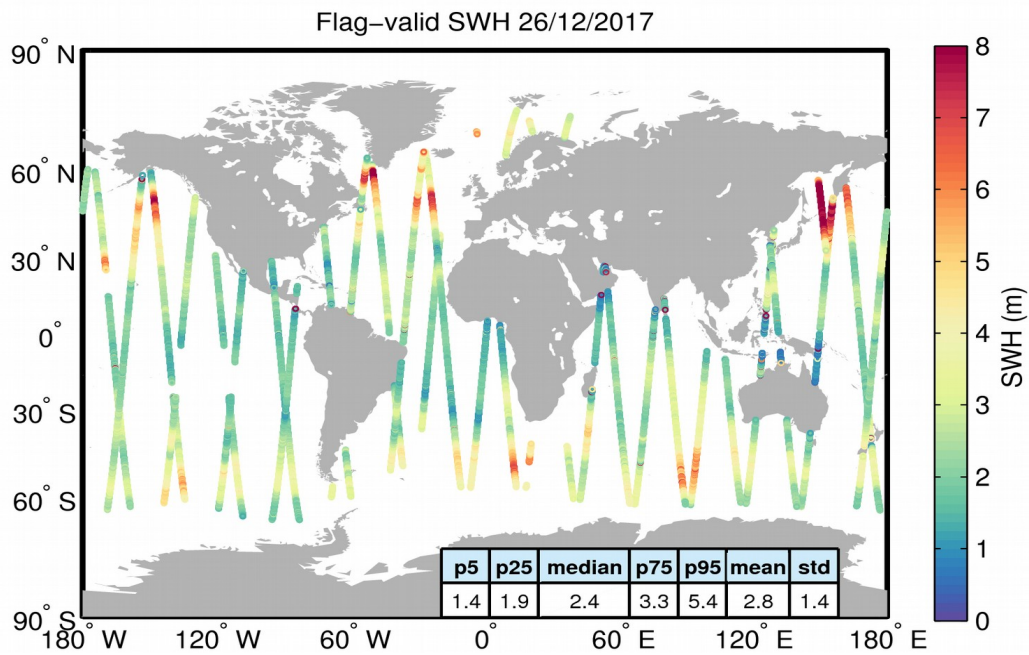
Figure 15. Geographical distribution of flag-valid SWH data over oceans and lakes for 26/12/2017. The statistical values shown in the table refer to the SWH in m and are calculated over all measurements shown in the figure.
