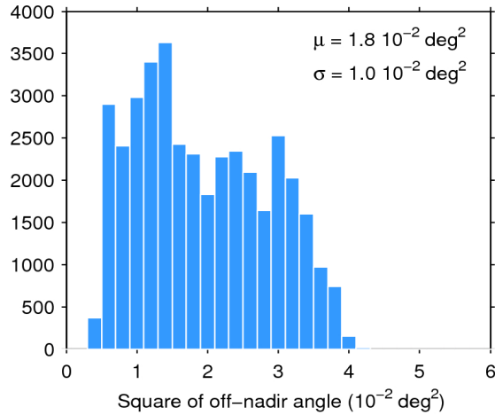
Figure 39. Histogram of flag-valid mispointing over oceans and lakes for 26/12/2017. The mean ( \mu ) and standard deviation ( \sigma ) are also shown. Note that values larger than 6 \cdot 10^{-2} \text{ deg}^2 are excluded from the histogram for the sake of readability but not from the computation of \mu and \sigma .
