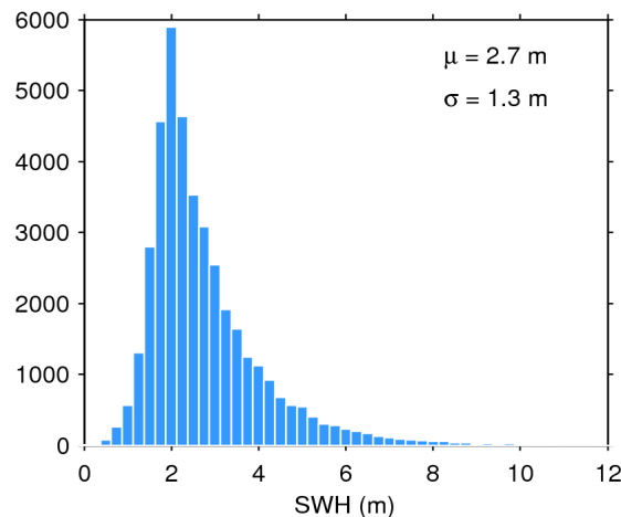
Figure 20. Histogram of science-valid SWH over oceans and lakes for 26/12/2017. The mean ( \mu ) and standard deviation ( \sigma ) are also shown. Note that values larger than 12 m are excluded from the histogram for the sake of readability but not from the computation of \mu and \sigma .
