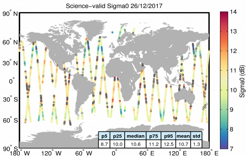
Figure 27. Geographical distribution of science-valid sigma0 data over oceans and lakes for 26/12/2017. The statistical values shown in the table refer to the sigma0 in dB and are calculated over all measurements shown in the figure. Gray circles denote records that have been rejected based on the editing criteria described in Table 4.
