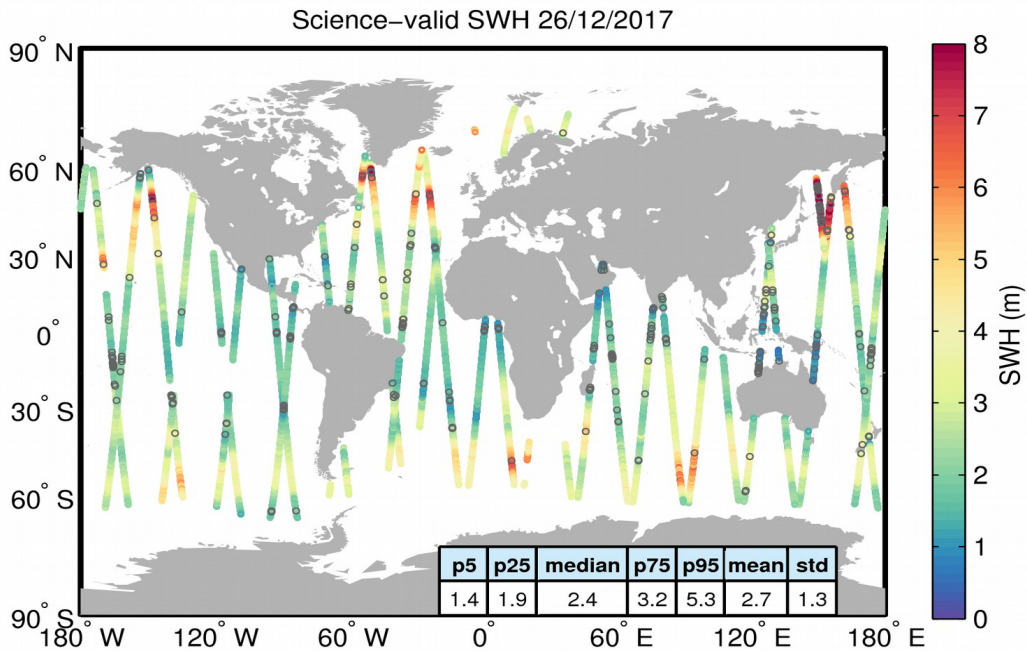
Figure 19. Geographical distribution of science-valid SWH data over oceans and lakes for 26/12/2017. The statistical values shown in the table refer to the SWH in m and are calculated over all measurements shown in the figure. Gray circles denote records that have been rejected based on the editing criteria described in Table 3.
