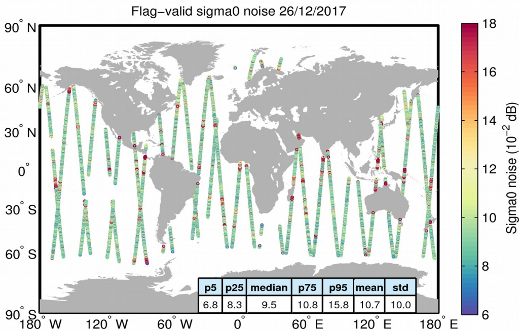
Figure 26. Geographical distribution of flag-valid 20-Hz sigma0 measurement noise over oceans and lakes for 26/12/2017. The statistical values shown in the table refer to the sigma0 noise and are calculated over all measurements shown in the figure.
