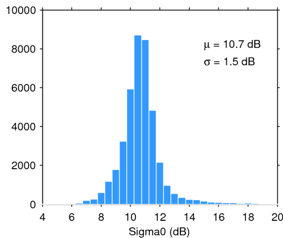
Figure 25. Histogram of flag-valid sigma0 over oceans and lakes for 26/12/2017. The mean ( \mu ) and standard deviation ( \sigma ) are also shown. Note that values outside [4 20] dB are excluded from the histogram for the sake of readability but not from the computation of \mu and \sigma .
