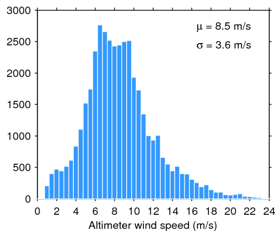
Figure 35. Histogram of science-valid wind over oceans and lakes for 26/12/2017. The mean ( \mu ) and standard deviation ( \sigma ) are also shown. Note that values larger than 24 m/s are excluded from the histogram for the sake of readability but not from the computation of \mu and \sigma .
