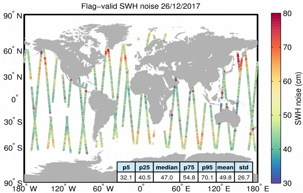
Figure 18. Geographical distribution of flag-valid 20-Hz SWH measurement noise over oceans and lakes for 26/12/2017. The statistical values shown in the table refer to the SWH noise and are calculated over all measurements shown in the figure.
