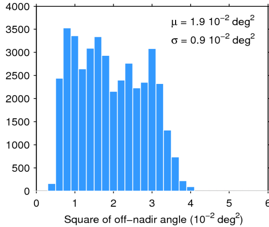
Figure 39. Histogram of flag-valid mispointing over oceans and lakes for 25/12/2017. The mean ( \mu ) and standard deviation ( \sigma ) are also shown. Note that values larger than 6 \cdot 10^{-2} \text{ deg}^2 are excluded from the histogram for the sake of readability but not from the computation of \mu and \sigma .
