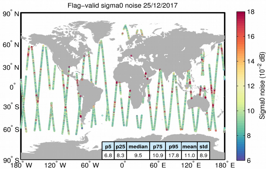
Figure 26. Geographical distribution of flag-valid 20-Hz sigma0 measurement noise over oceans and lakes for 25/12/2017. The statistical values shown in the table refer to the sigma0 noise and are calculated over all measurements shown in the figure.
