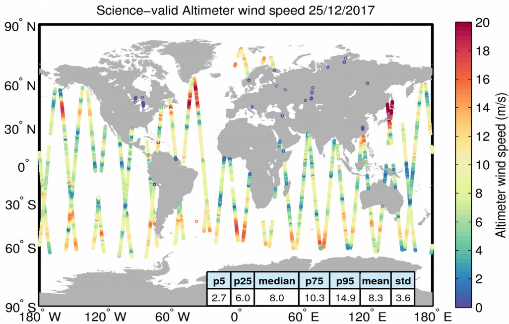
Figure 34. Geographical distribution of science-valid wind data over oceans and lakes for 25/12/2017. The statistical values shown in the table refer to the wind in m/s and are calculated over all measurements shown in the figure. Gray circles denote records that have been rejected based on the editing criteria described in Table 5.
