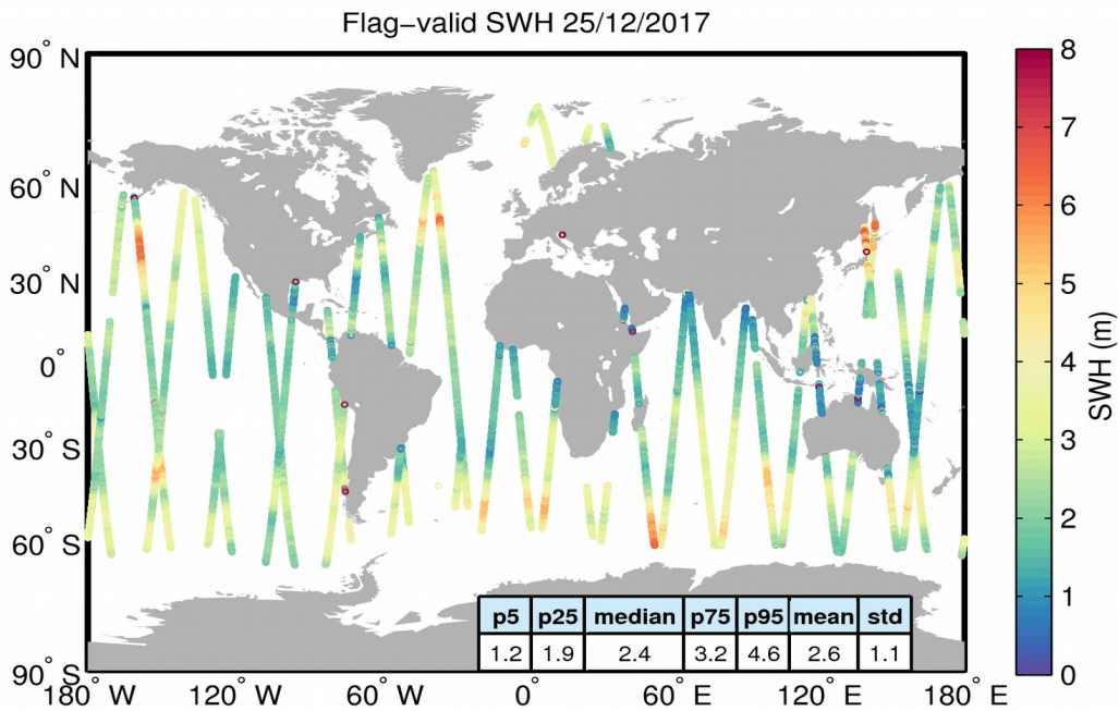
Figure 15. Geographical distribution of flag-valid SWH data over oceans and lakes for 25/12/2017. The statistical values shown in the table refer to the SWH in m and are calculated over all measurements shown in the figure.
