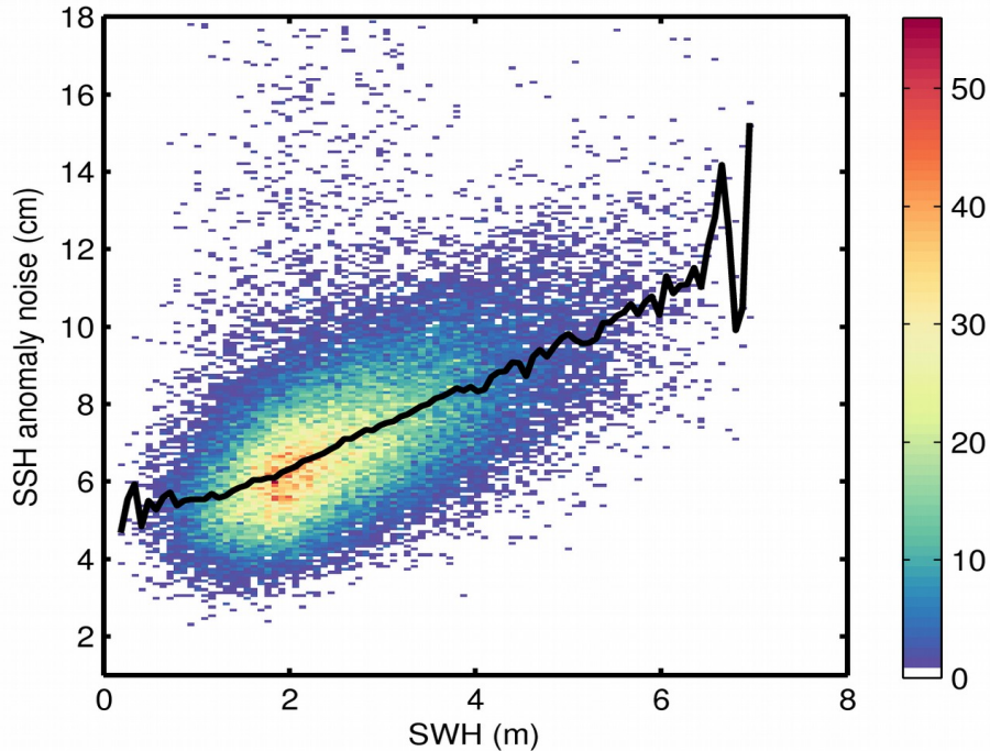
Figure 9. 2D histogram showing flag-valid SSH anomaly noise as a function of SWH for 25/12/2017. The black line denotes the median SSH anomaly noise as a function of SWH.
