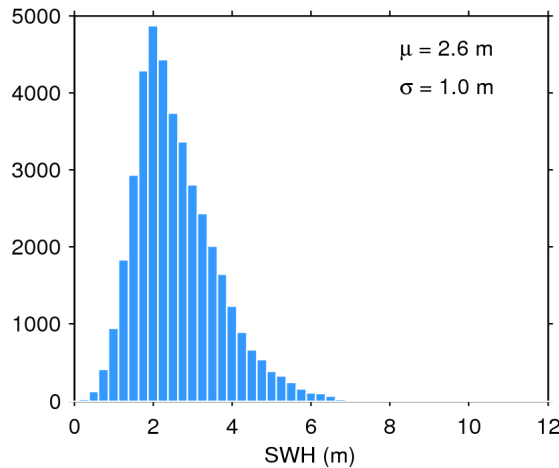
Figure 20. Histogram of science-valid SWH over oceans and lakes for 25/12/2017. The mean ( \mu ) and standard deviation ( \sigma ) are also shown. Note that values larger than 12 m are excluded from the histogram for the sake of readability but not from the computation of \mu and \sigma .
