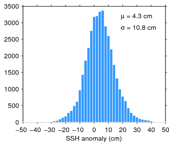
Figure 11. Histogram of science-valid SSH anomaly over oceans and lakes for 25/12/2017. The mean ( \mu ) and standard deviation ( \sigma ) are also shown. Note that values outside [-50 50] cm are excluded from the histogram for the sake of readability but not from the computation of \mu and \sigma .
