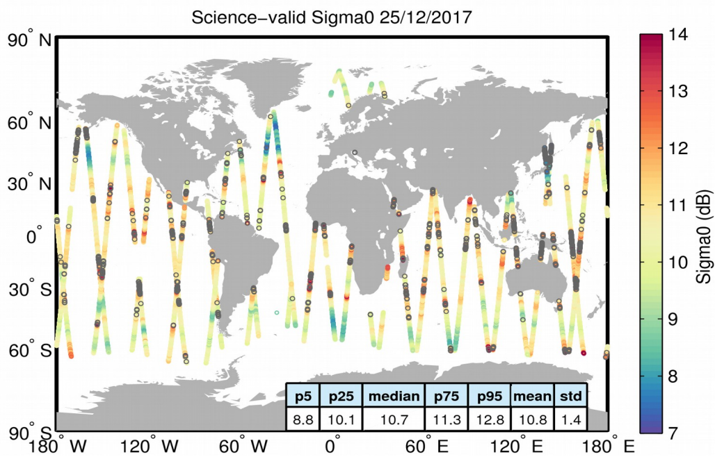
Figure 27. Geographical distribution of science-valid sigma0 data over oceans and lakes for 25/12/2017. The statistical values shown in the table refer to the sigma0 in dB and are calculated over all measurements shown in the figure. Gray circles denote records that have been rejected based on the editing criteria described in Table 4.
