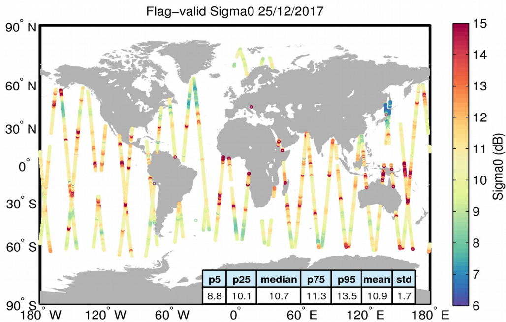
Figure 23. Geographical distribution of flag-valid sigma0 data over oceans and lakes for 25/12/2017. The statistical values shown in the table refer to the sigma0 in dB and are calculated over all measurements shown in the figure.
