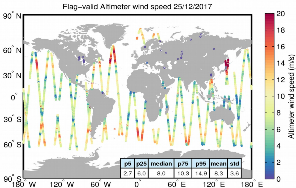
Figure 31. Geographical distribution of flag-valid wind data over oceans and lakes for 25/12/2017. The statistical values shown in the table refer to the wind in m/s and are calculated over all measurements shown in the figure.
