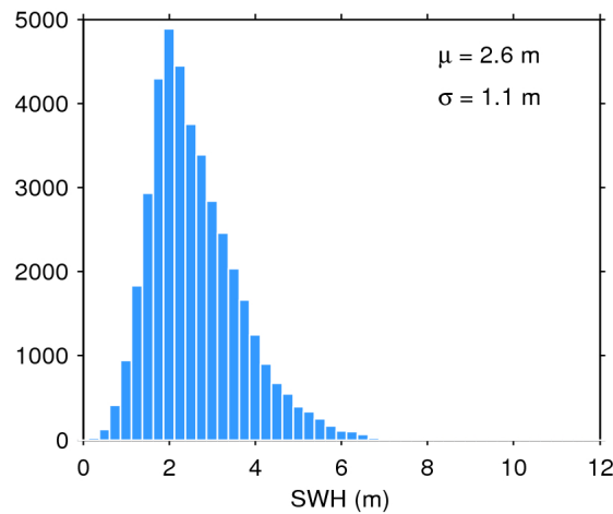
Figure 17. Histogram of flag-valid SWH over oceans and lakes for 25/12/2017. The mean ( \mu ) and standard deviation ( \sigma ) are also shown. Note that values larger than 12 m are excluded from the histogram for the sake of readability but not from the computation of \mu and \sigma .
