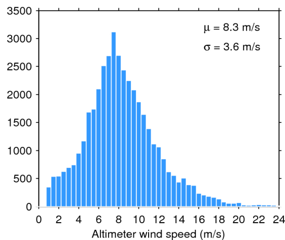
Figure 35. Histogram of science-valid wind over oceans and lakes for 25/12/2017. The mean ( \mu ) and standard deviation ( \sigma ) are also shown. Note that values larger than 24 m/s are excluded from the histogram for the sake of readability but not from the computation of \mu and \sigma .
