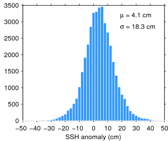
Figure 7. Histogram of flag-valid SSH anomaly over oceans and lakes for 25/12/2017. The mean ( \mu ) and standard deviation ( \sigma ) are also shown. Note that values outside [-50 50] cm are excluded from the histogram for the sake of readability but not from the computation of \mu and \sigma .
