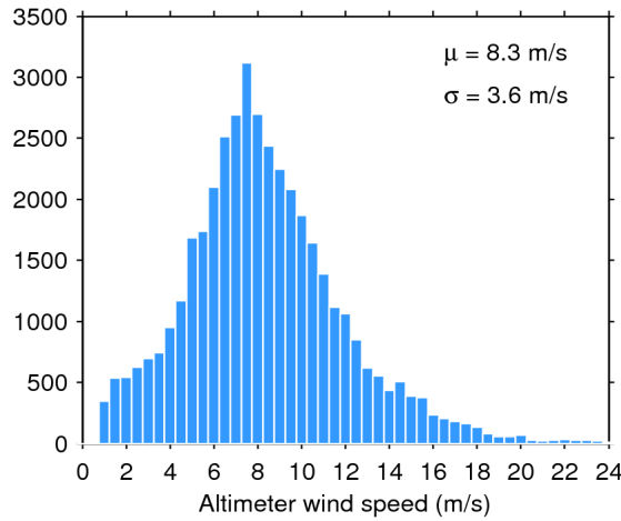
Figure 33. Histogram of flag-valid wind over oceans and lakes for 25/12/2017. The mean ( \mu ) and standard deviation ( \sigma ) are also shown. Note that values larger than 24 m/s are excluded from the histogram for the sake of readability but not from the computation of \mu and \sigma .
