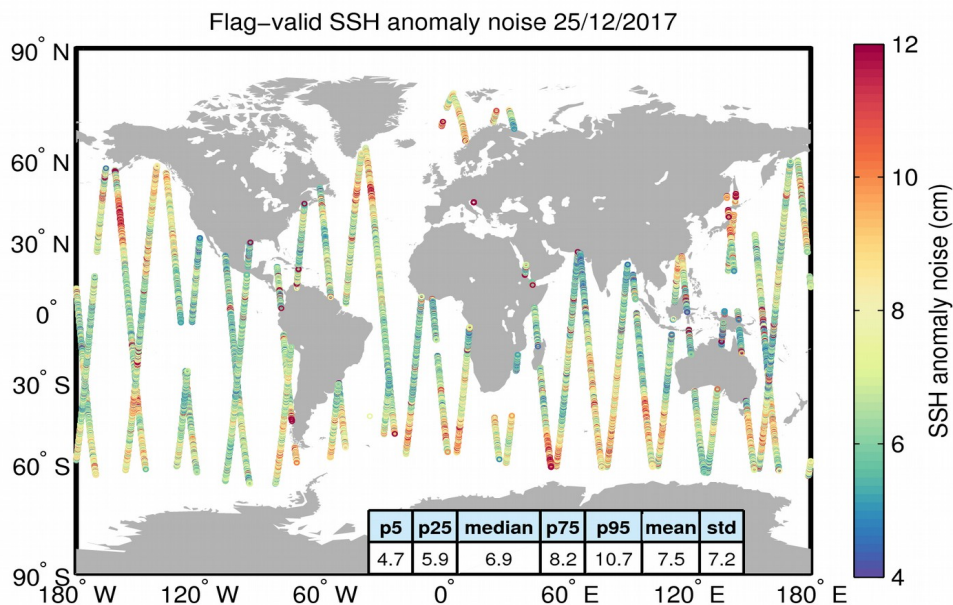
Figure 8. Geographical distribution of flag-valid 20-Hz SSH anomaly measurement noise over oceans and lakes for 25/12/2017. The statistical values shown in the table refer to the SSH anomaly noise and are calculated over all measurements shown in the figure.
