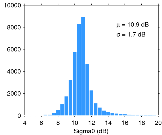
Figure 25. Histogram of flag-valid sigma0 over oceans and lakes for 25/12/2017. The mean ( \mu ) and standard deviation ( \sigma ) are also shown. Note that values outside [4 20] dB are excluded from the histogram for the sake of readability but not from the computation of \mu and \sigma .
