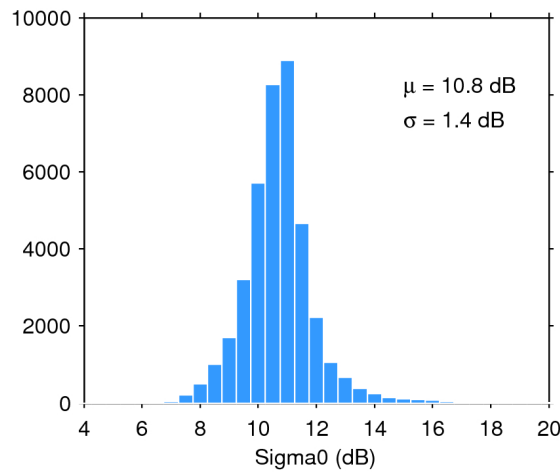
Figure 28. Histogram of science-valid sigma0 over oceans and lakes for 25/12/2017. The mean ( \mu ) and standard deviation ( \sigma ) are also shown. Note that values outside [4 20] dB are excluded from the histogram for the sake of readability but not from the computation of \mu and \sigma .
