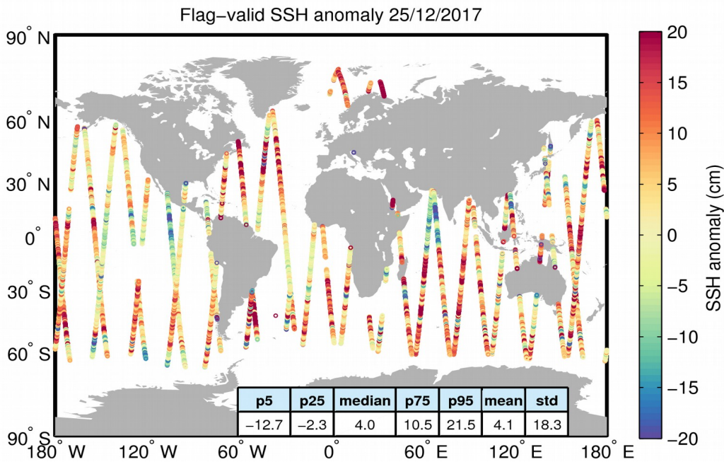
Figure 5. Geographical distribution of flag-valid 1-Hz SSH anomaly data over oceans and lakes for 25/12/2017. The statistical values shown in the table refer to the SSH anomaly in cm and are calculated over all measurements shown in the figure.
