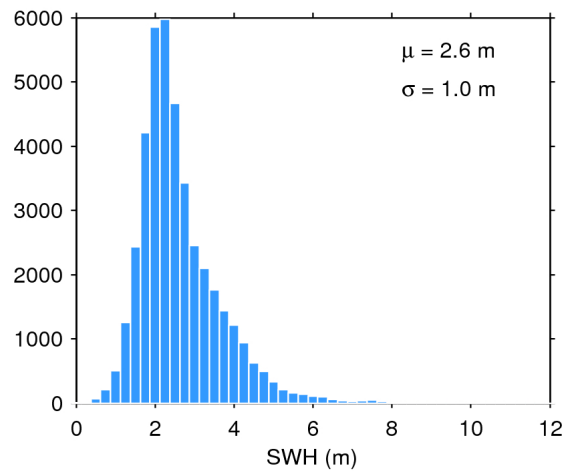
Figure 17. Histogram of flag-valid SWH over oceans and lakes for 24/12/2017. The mean ( \mu ) and standard deviation ( \sigma ) are also shown. Note that values larger than 12 m are excluded from the histogram for the sake of readability but not from the computation of \mu and \sigma .
