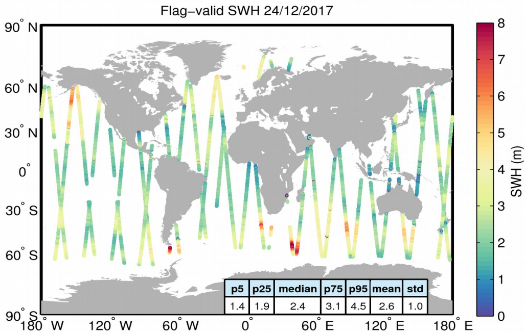
Figure 15. Geographical distribution of flag-valid SWH data over oceans and lakes for 24/12/2017. The statistical values shown in the table refer to the SWH in m and are calculated over all measurements shown in the figure.
