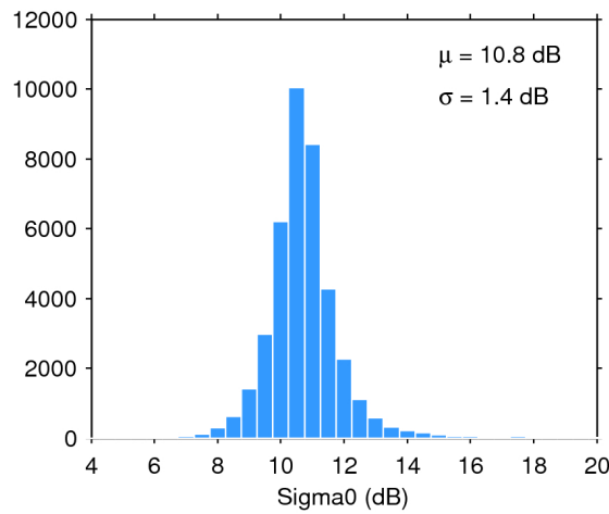
Figure 28. Histogram of science-valid sigma0 over oceans and lakes for 24/12/2017. The mean ( \mu ) and standard deviation ( \sigma ) are also shown. Note that values outside [4 20] dB are excluded from the histogram for the sake of readability but not from the computation of \mu and \sigma .
