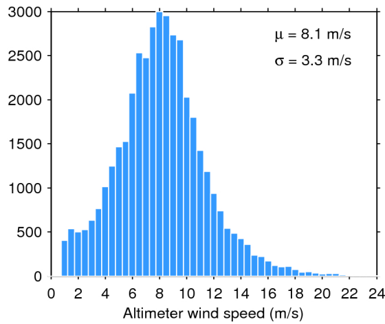
Figure 33. Histogram of flag-valid wind over oceans and lakes for 24/12/2017. The mean ( \mu ) and standard deviation ( \sigma ) are also shown. Note that values larger than 24 m/s are excluded from the histogram for the sake of readability but not from the computation of \mu and \sigma .
