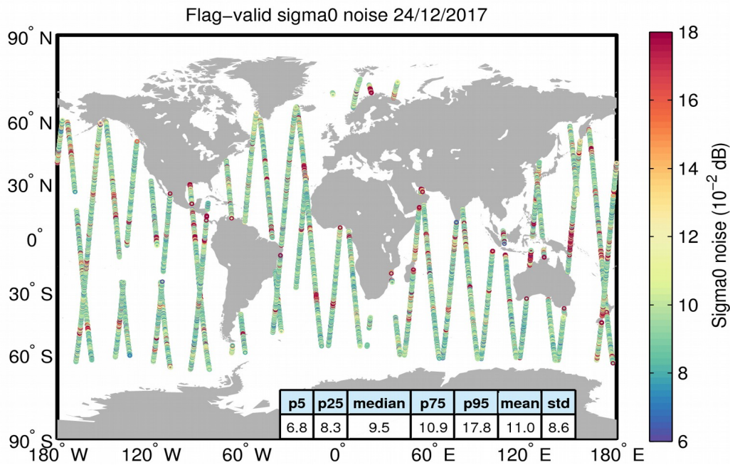
Figure 26. Geographical distribution of flag-valid 20-Hz sigma0 measurement noise over oceans and lakes for 24/12/2017. The statistical values shown in the table refer to the sigma0 noise and are calculated over all measurements shown in the figure.
