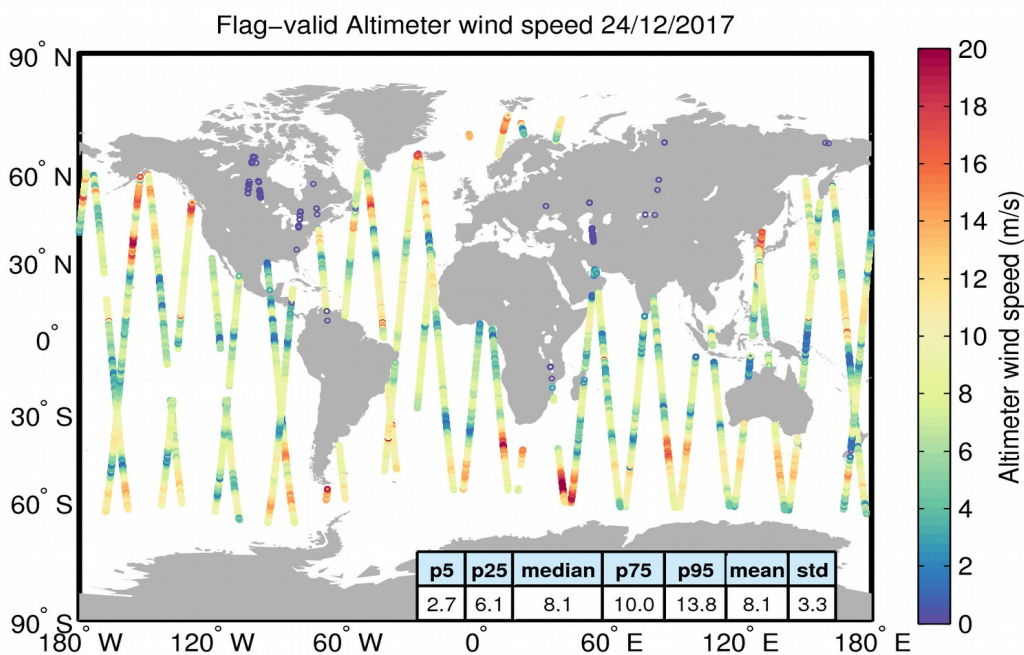
Figure 31. Geographical distribution of flag-valid wind data over oceans and lakes for 24/12/2017. The statistical values shown in the table refer to the wind in m/s and are calculated over all measurements shown in the figure.
