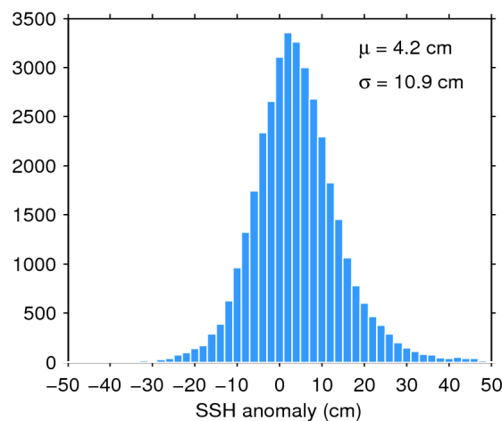
Figure 11. Histogram of science-valid SSH anomaly over oceans and lakes for 24/12/2017. The mean ( \mu ) and standard deviation ( \sigma ) are also shown. Note that values outside [-50 50] cm are excluded from the histogram for the sake of readability but not from the computation of \mu and \sigma .
