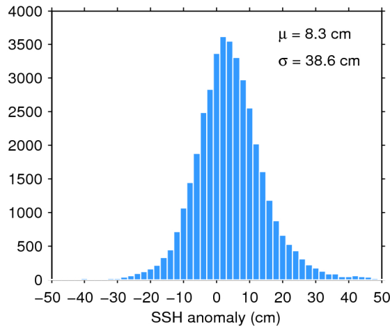
Figure 7. Histogram of flag-valid SSH anomaly over oceans and lakes for 24/12/2017. The mean ( \mu ) and standard deviation ( \sigma ) are also shown. Note that values outside [-50 50] cm are excluded from the histogram for the sake of readability but not from the computation of \mu and \sigma .
