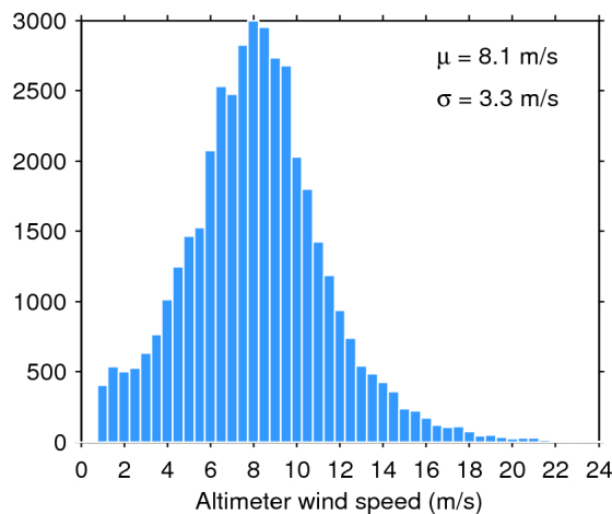
Figure 35. Histogram of science-valid wind over oceans and lakes for 24/12/2017. The mean ( \mu ) and standard deviation ( \sigma ) are also shown. Note that values larger than 24 m/s are excluded from the histogram for the sake of readability but not from the computation of \mu and \sigma .
