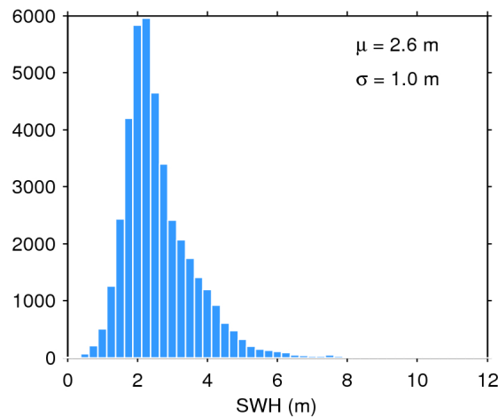
Figure 20. Histogram of science-valid SWH over oceans and lakes for 24/12/2017. The mean ( \mu ) and standard deviation ( \sigma ) are also shown. Note that values larger than 12 m are excluded from the histogram for the sake of readability but not from the computation of \mu and \sigma .
