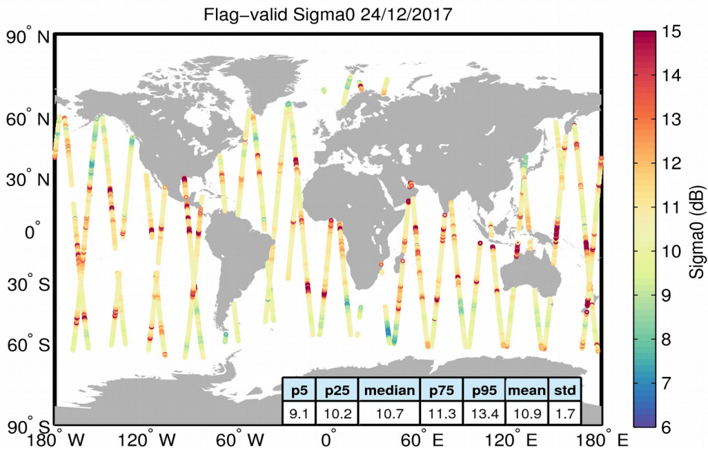
Figure 23. Geographical distribution of flag-valid sigma0 data over oceans and lakes for 24/12/2017. The statistical values shown in the table refer to the sigma0 in dB and are calculated over all measurements shown in the figure.
