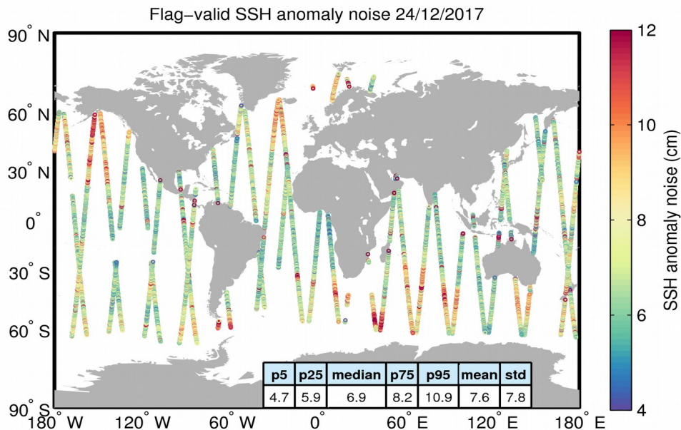
Figure 8. Geographical distribution of flag-valid 20-Hz SSH anomaly measurement noise over oceans and lakes for 24/12/2017. The statistical values shown in the table refer to the SSH anomaly noise and are calculated over all measurements shown in the figure.
