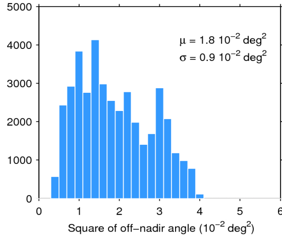
Figure 39. Histogram of flag-valid mispointing over oceans and lakes for 24/12/2017. The mean ( \mu ) and standard deviation ( \sigma ) are also shown. Note that values larger than 6 \cdot 10^{-2} \text{ deg}^2 are excluded from the histogram for the sake of readability but not from the computation of \mu and \sigma .
