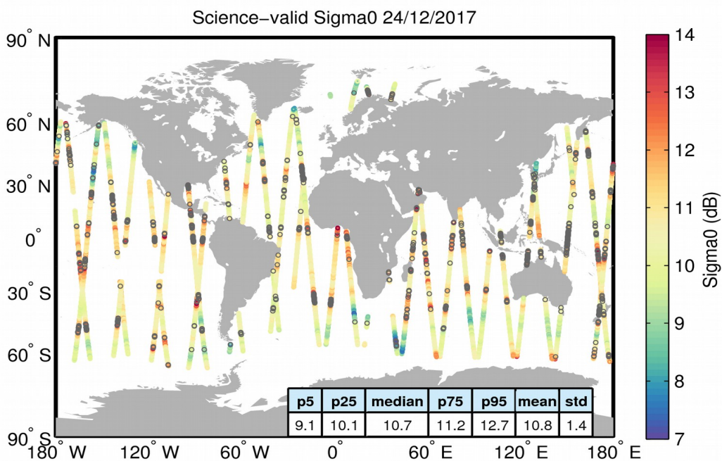
Figure 27. Geographical distribution of science-valid sigma0 data over oceans and lakes for 24/12/2017. The statistical values shown in the table refer to the sigma0 in dB and are calculated over all measurements shown in the figure. Gray circles denote records that have been rejected based on the editing criteria described in Table 4.
