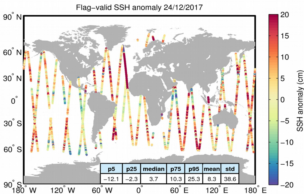
Figure 5. Geographical distribution of flag-valid 1-Hz SSH anomaly data over oceans and lakes for 24/12/2017. The statistical values shown in the table refer to the SSH anomaly in cm and are calculated over all measurements shown in the figure.
