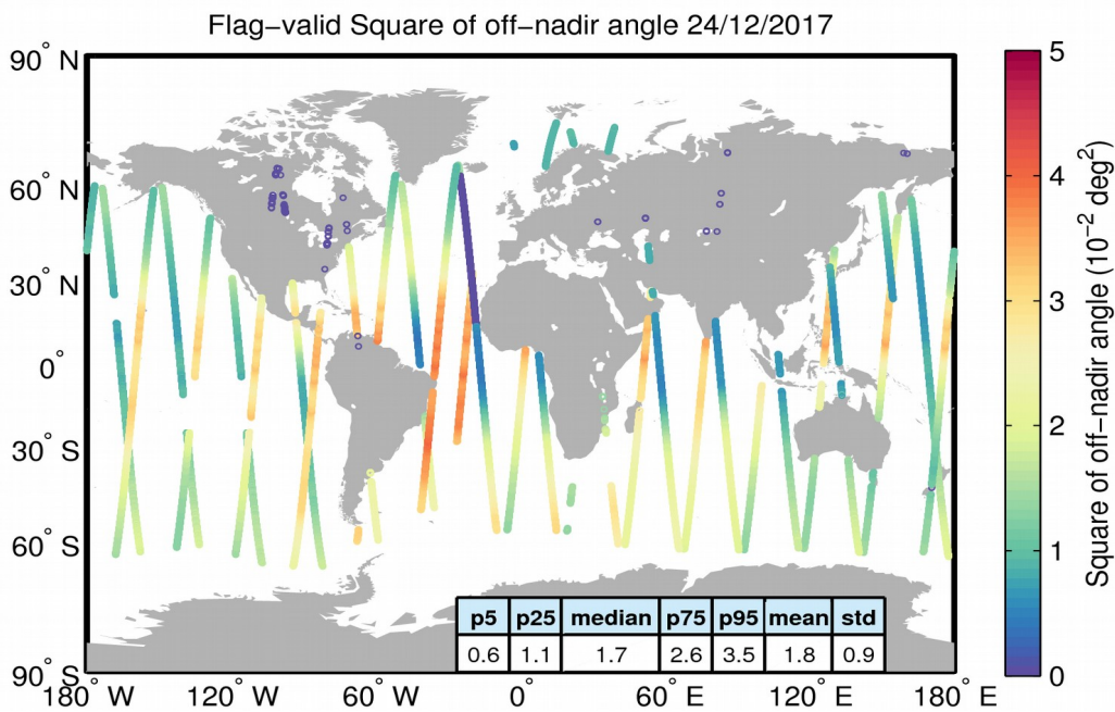
Figure 37. Geographical distribution of flag-valid mispointing data over oceans and lakes for 24/12/2017. The statistical values shown in the table refer to the mispointing in 10^{-2} deg 2 and are calculated over all measurements shown in the figure.
