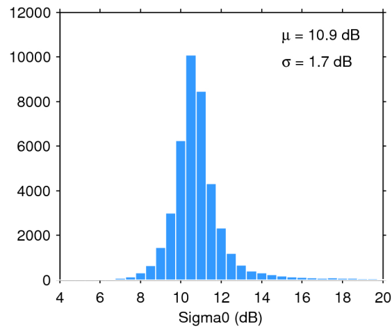
Figure 25. Histogram of flag-valid sigma0 over oceans and lakes for 24/12/2017. The mean ( \mu ) and standard deviation ( \sigma ) are also shown. Note that values outside [4 20] dB are excluded from the histogram for the sake of readability but not from the computation of \mu and \sigma .
