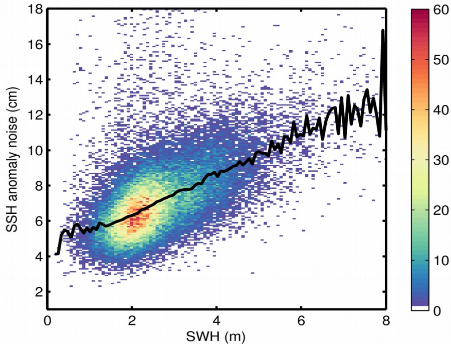
Figure 9. 2D histogram showing flag-valid SSH anomaly noise as a function of SWH for 24/12/2017. The black line denotes the median SSH anomaly noise as a function of SWH.
