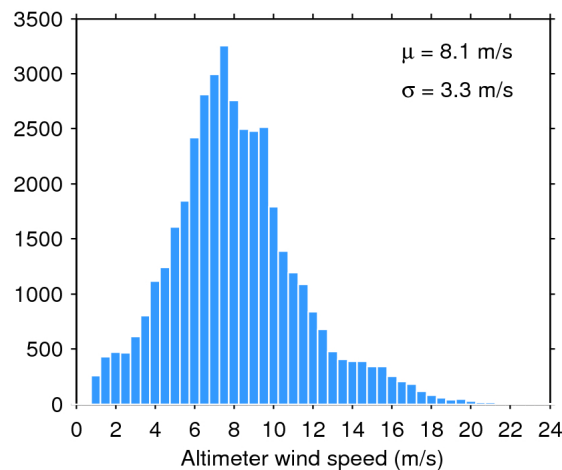
Figure 35. Histogram of science-valid wind over oceans and lakes for 23/12/2017. The mean ( \mu ) and standard deviation ( \sigma ) are also shown. Note that values larger than 24 m/s are excluded from the histogram for the sake of readability but not from the computation of \mu and \sigma .
