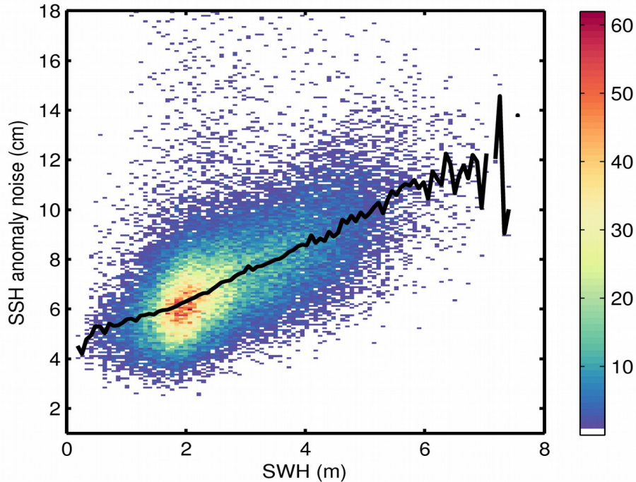
Figure 9. 2D histogram showing flag-valid SSH anomaly noise as a function of SWH for 23/12/2017. The black line denotes the median SSH anomaly noise as a function of SWH.
