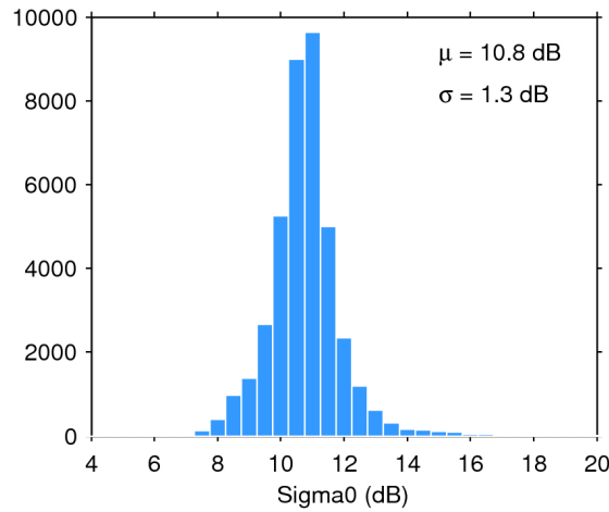
Figure 28. Histogram of science-valid sigma0 over oceans and lakes for 23/12/2017. The mean ( \mu ) and standard deviation ( \sigma ) are also shown. Note that values outside [4 20] dB are excluded from the histogram for the sake of readability but not from the computation of \mu and \sigma .
