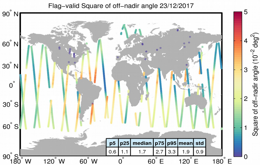
Figure 37. Geographical distribution of flag-valid mispointing data over oceans and lakes for 23/12/2017. The statistical values shown in the table refer to the mispointing in 10^{-2} \text{ deg}^2 and are calculated over all measurements shown in the figure.
