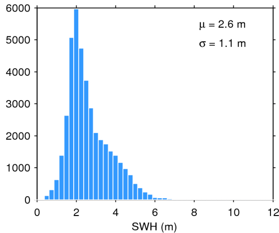
Figure 20. Histogram of science-valid SWH over oceans and lakes for 23/12/2017. The mean ( \mu ) and standard deviation ( \sigma ) are also shown. Note that values larger than 12 m are excluded from the histogram for the sake of readability but not from the computation of \mu and \sigma .
