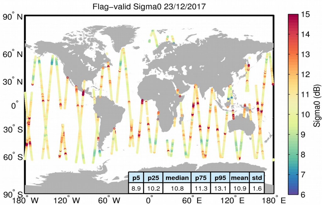
Figure 23. Geographical distribution of flag-valid sigma0 data over oceans and lakes for 23/12/2017. The statistical values shown in the table refer to the sigma0 in dB and are calculated over all measurements shown in the figure.
