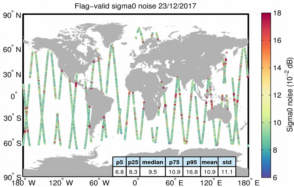
Figure 26. Geographical distribution of flag-valid 20-Hz sigma0 measurement noise over oceans and lakes for 23/12/2017. The statistical values shown in the table refer to the sigma0 noise and are calculated over all measurements shown in the figure.
