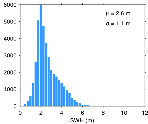
Figure 17. Histogram of flag-valid SWH over oceans and lakes for 23/12/2017. The mean ( \mu ) and standard deviation ( \sigma ) are also shown. Note that values larger than 12 m are excluded from the histogram for the sake of readability but not from the computation of \mu and \sigma .
