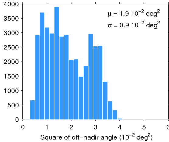
Figure 39. Histogram of flag-valid mispointing over oceans and lakes for 23/12/2017. The mean ( \mu ) and standard deviation ( \sigma ) are also shown. Note that values larger than 6 \cdot 10^{-2} \text{ deg}^2 are excluded from the histogram for the sake of readability but not from the computation of \mu and \sigma .
