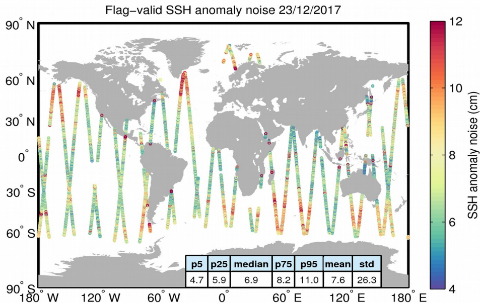
Figure 8. Geographical distribution of flag-valid 20-Hz SSH anomaly measurement noise over oceans and lakes for 23/12/2017. The statistical values shown in the table refer to the SSH anomaly noise and are calculated over all measurements shown in the figure.
