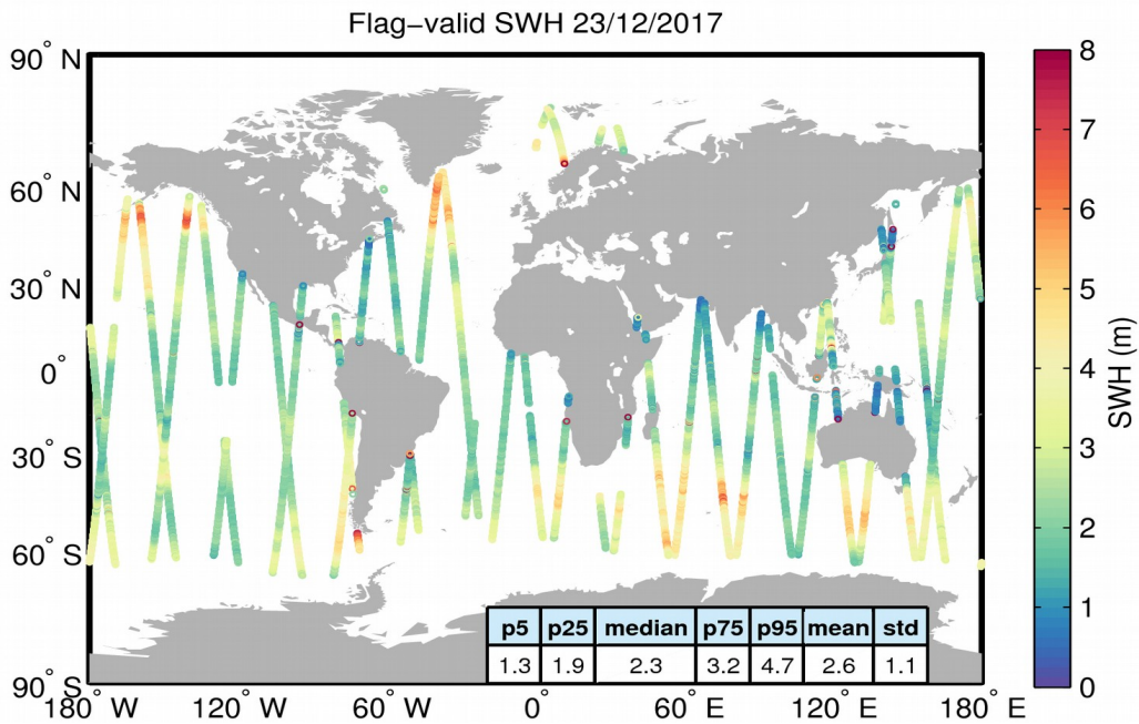
Figure 15. Geographical distribution of flag-valid SWH data over oceans and lakes for 23/12/2017. The statistical values shown in the table refer to the SWH in m and are calculated over all measurements shown in the figure.
