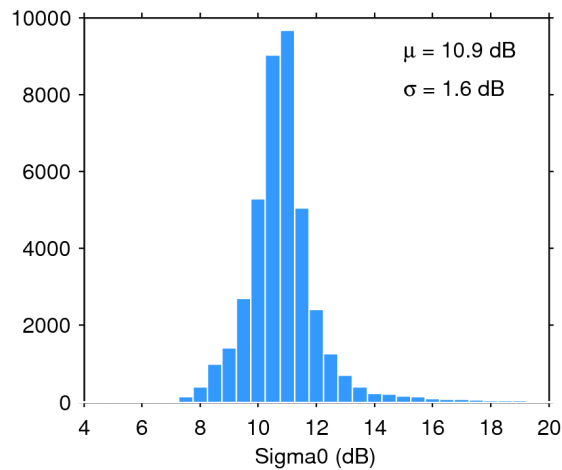
Figure 25. Histogram of flag-valid sigma0 over oceans and lakes for 23/12/2017. The mean ( \mu ) and standard deviation ( \sigma ) are also shown. Note that values outside [4 20] dB are excluded from the histogram for the sake of readability but not from the computation of \mu and \sigma .
