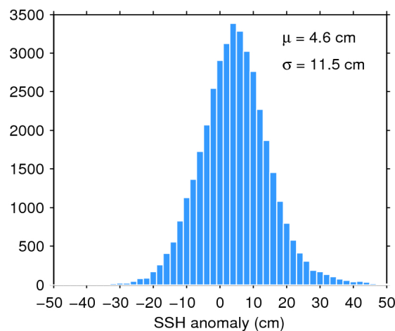
Figure 11. Histogram of science-valid SSH anomaly over oceans and lakes for 23/12/2017. The mean ( \mu ) and standard deviation ( \sigma ) are also shown. Note that values outside [-50 50] cm are excluded from the histogram for the sake of readability but not from the computation of \mu and \sigma .
