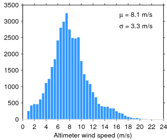
Figure 33. Histogram of flag-valid wind over oceans and lakes for 23/12/2017. The mean ( \mu ) and standard deviation ( \sigma ) are also shown. Note that values larger than 24 m/s are excluded from the histogram for the sake of readability but not from the computation of \mu and \sigma .
