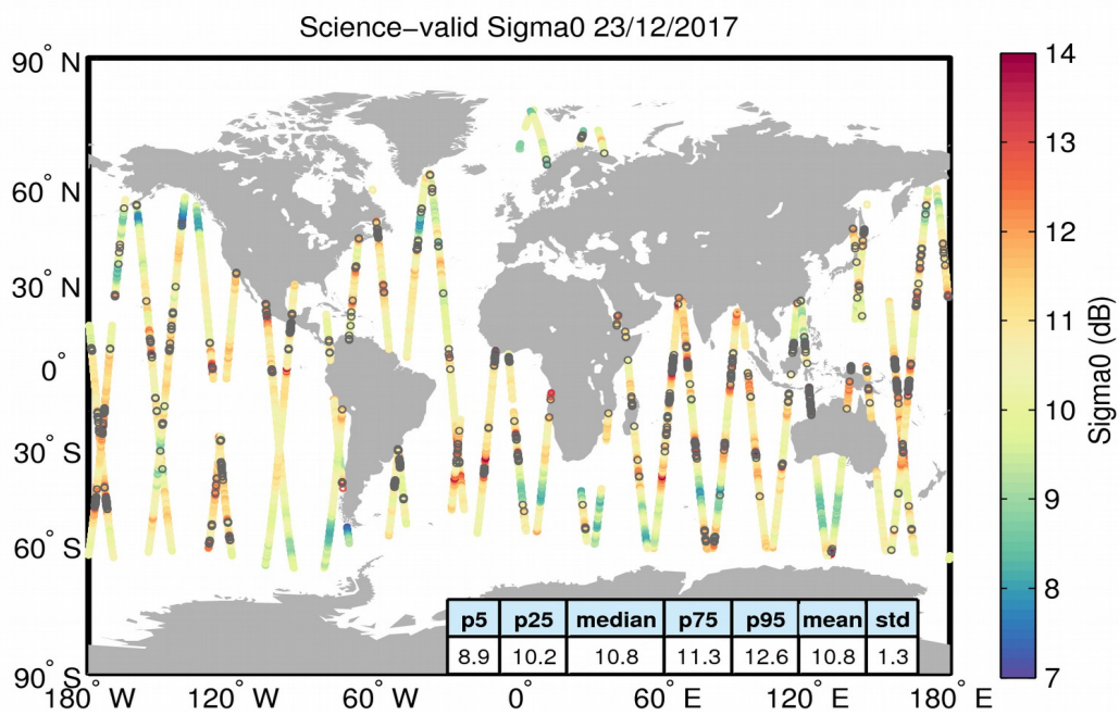
Figure 27. Geographical distribution of science-valid sigma0 data over oceans and lakes for 23/12/2017. The statistical values shown in the table refer to the sigma0 in dB and are calculated over all measurements shown in the figure. Gray circles denote records that have been rejected based on the editing criteria described in Table 4.
