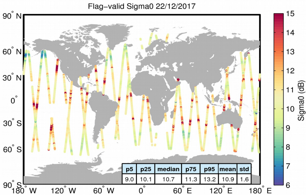
Figure 23. Geographical distribution of flag-valid sigma0 data over oceans and lakes for 22/12/2017. The statistical values shown in the table refer to the sigma0 in dB and are calculated over all measurements shown in the figure.
