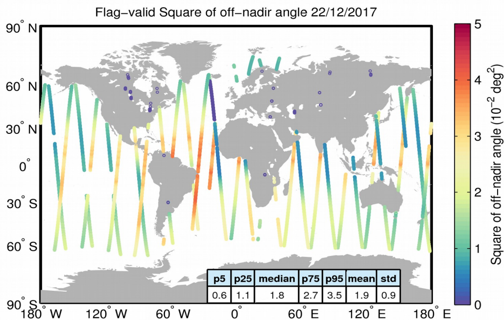
Figure 37. Geographical distribution of flag-valid mispointing data over oceans and lakes for 22/12/2017. The statistical values shown in the table refer to the mispointing in 10^{-2} deg 2 and are calculated over all measurements shown in the figure.
