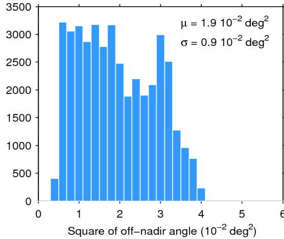
Figure 39. Histogram of flag-valid mispointing over oceans and lakes for 22/12/2017. The mean ( \mu ) and standard deviation ( \sigma ) are also shown. Note that values larger than 6 \cdot 10^{-2} \text{ deg}^2 are excluded from the histogram for the sake of readability but not from the computation of \mu and \sigma .
