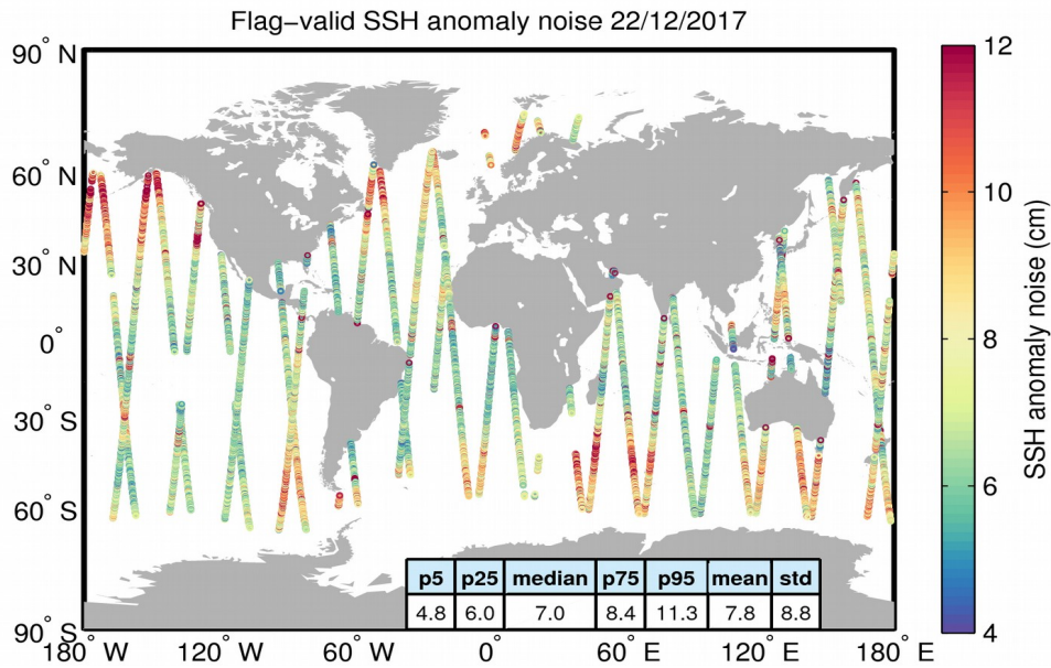
Figure 8. Geographical distribution of flag-valid 20-Hz SSH anomaly measurement noise over oceans and lakes for 22/12/2017. The statistical values shown in the table refer to the SSH anomaly noise and are calculated over all measurements shown in the figure.
