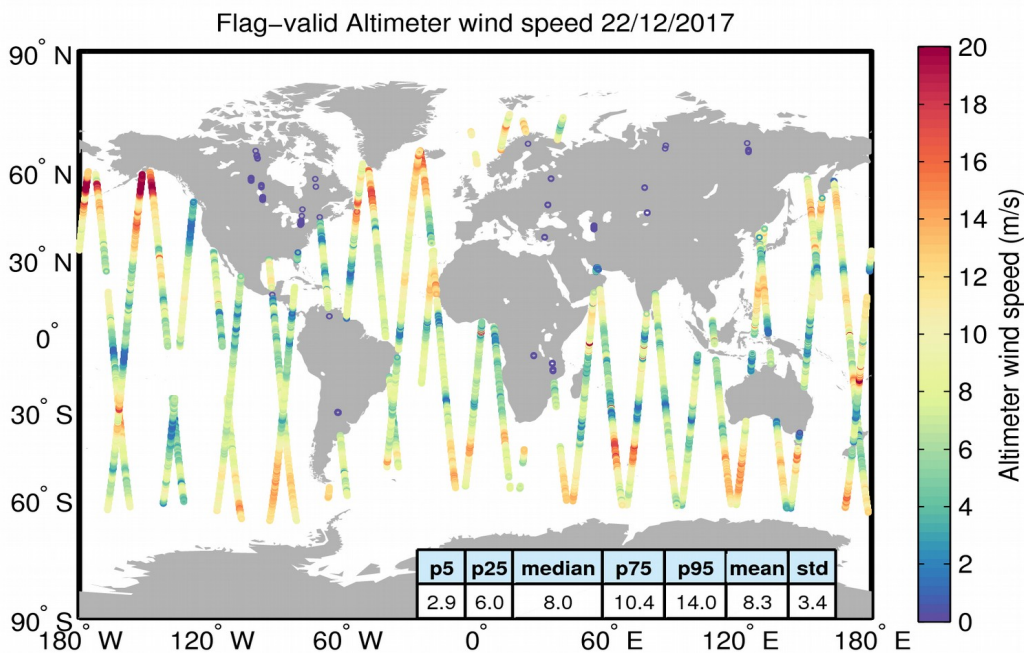
Figure 31. Geographical distribution of flag-valid wind data over oceans and lakes for 22/12/2017. The statistical values shown in the table refer to the wind in m/s and are calculated over all measurements shown in the figure.
