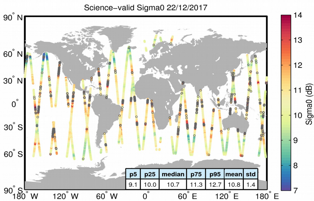
Figure 27. Geographical distribution of science-valid sigma0 data over oceans and lakes for 22/12/2017. The statistical values shown in the table refer to the sigma0 in dB and are calculated over all measurements shown in the figure. Gray circles denote records that have been rejected based on the editing criteria described in Table 4.
