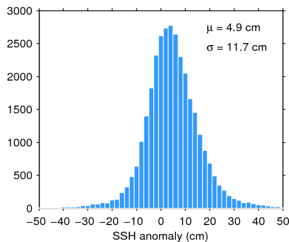
Figure 11. Histogram of science-valid SSH anomaly over oceans and lakes for 22/12/2017. The mean ( \mu ) and standard deviation ( \sigma ) are also shown. Note that values outside [-50 50] cm are excluded from the histogram for the sake of readability but not from the computation of \mu and \sigma .
