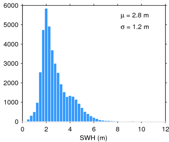
Figure 17. Histogram of flag-valid SWH over oceans and lakes for 22/12/2017. The mean ( \mu ) and standard deviation ( \sigma ) are also shown. Note that values larger than 12 m are excluded from the histogram for the sake of readability but not from the computation of \mu and \sigma .
