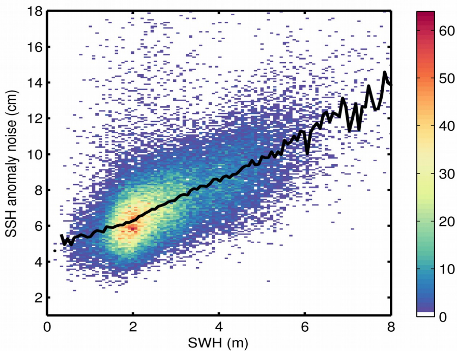
Figure 9. 2D histogram showing flag-valid SSH anomaly noise as a function of SWH for 22/12/2017. The black line denotes the median SSH anomaly noise as a function of SWH.
