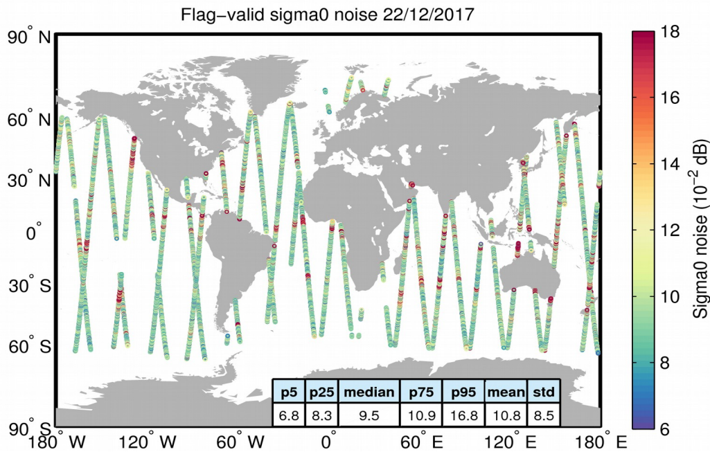
Figure 26. Geographical distribution of flag-valid 20-Hz sigma0 measurement noise over oceans and lakes for 22/12/2017. The statistical values shown in the table refer to the sigma0 noise and are calculated over all measurements shown in the figure.
