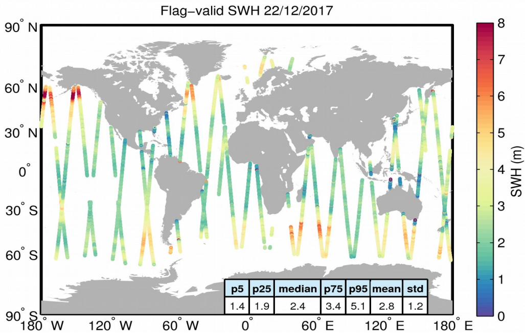
Figure 15. Geographical distribution of flag-valid SWH data over oceans and lakes for 22/12/2017. The statistical values shown in the table refer to the SWH in m and are calculated over all measurements shown in the figure.
