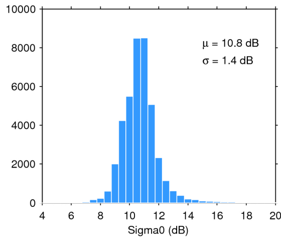
Figure 28. Histogram of science-valid sigma0 over oceans and lakes for 22/12/2017. The mean ( \mu ) and standard deviation ( \sigma ) are also shown. Note that values outside [4 20] dB are excluded from the histogram for the sake of readability but not from the computation of \mu and \sigma .
