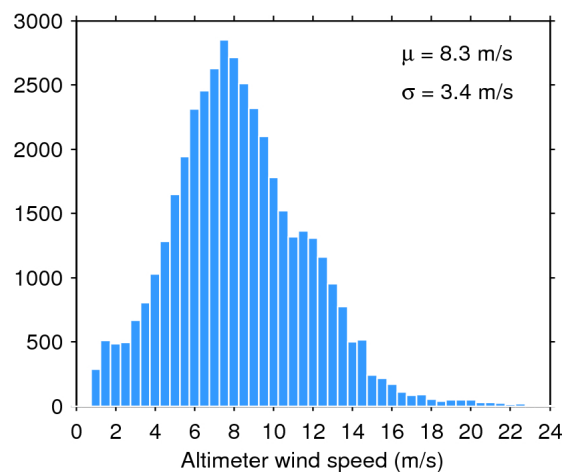
Figure 35. Histogram of science-valid wind over oceans and lakes for 22/12/2017. The mean ( \mu ) and standard deviation ( \sigma ) are also shown. Note that values larger than 24 m/s are excluded from the histogram for the sake of readability but not from the computation of \mu and \sigma .
