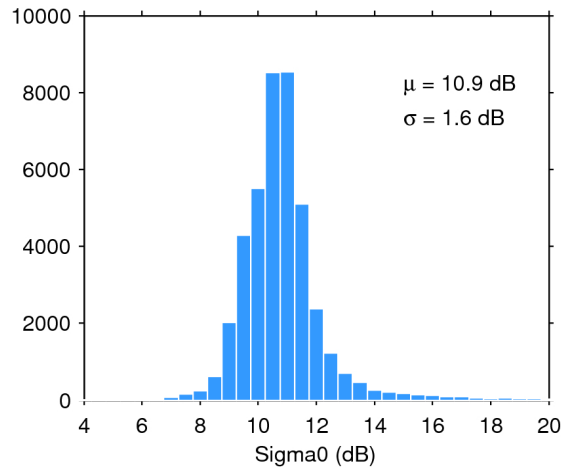
Figure 25. Histogram of flag-valid sigma0 over oceans and lakes for 22/12/2017. The mean ( \mu ) and standard deviation ( \sigma ) are also shown. Note that values outside [4 20] dB are excluded from the histogram for the sake of readability but not from the computation of \mu and \sigma .
