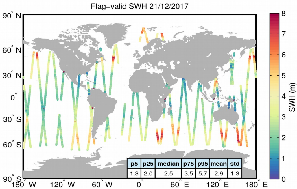
Figure 15. Geographical distribution of flag-valid SWH data over oceans and lakes for 21/12/2017. The statistical values shown in the table refer to the SWH in m and are calculated over all measurements shown in the figure.
