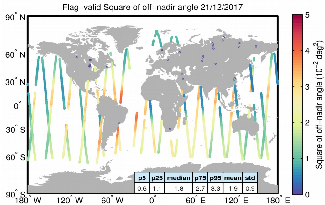
Figure 37. Geographical distribution of flag-valid mispointing data over oceans and lakes for 21/12/2017. The statistical values shown in the table refer to the mispointing in 10^{-2} \text{ deg}^2 and are calculated over all measurements shown in the figure.
