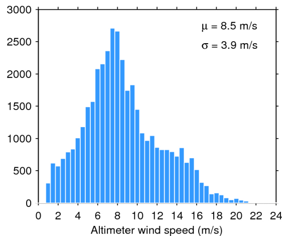
Figure 35. Histogram of science-valid wind over oceans and lakes for 21/12/2017. The mean ( \mu ) and standard deviation ( \sigma ) are also shown. Note that values larger than 24 m/s are excluded from the histogram for the sake of readability but not from the computation of \mu and \sigma .
