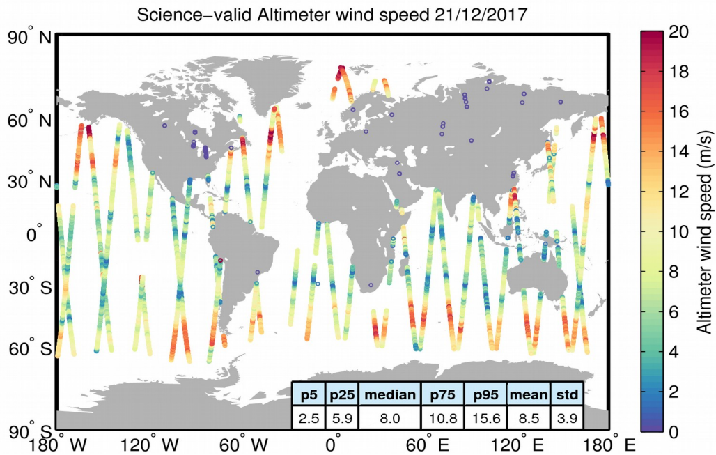
Figure 34. Geographical distribution of science-valid wind data over oceans and lakes for 21/12/2017. The statistical values shown in the table refer to the wind in m/s and are calculated over all measurements shown in the figure. Gray circles denote records that have been rejected based on the editing criteria described in Table 5.
