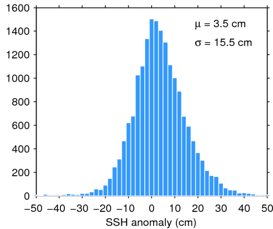
Figure 7. Histogram of flag-valid SSH anomaly over oceans and lakes for 21/12/2017. The mean ( \mu ) and standard deviation ( \sigma ) are also shown. Note that values outside [-50 50] cm are excluded from the histogram for the sake of readability but not from the computation of \mu and \sigma .
