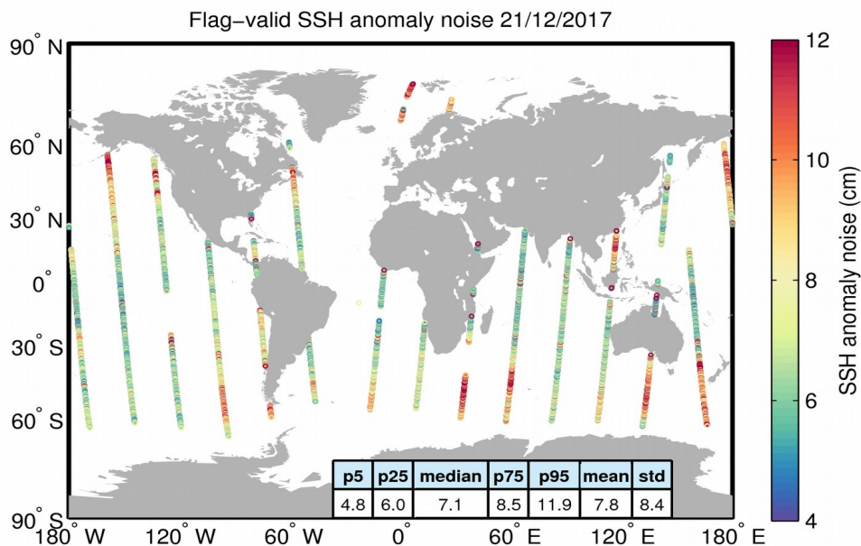
Figure 8. Geographical distribution of flag-valid 20-Hz SSH anomaly measurement noise over oceans and lakes for 21/12/2017. The statistical values shown in the table refer to the SSH anomaly noise and are calculated over all measurements shown in the figure.
