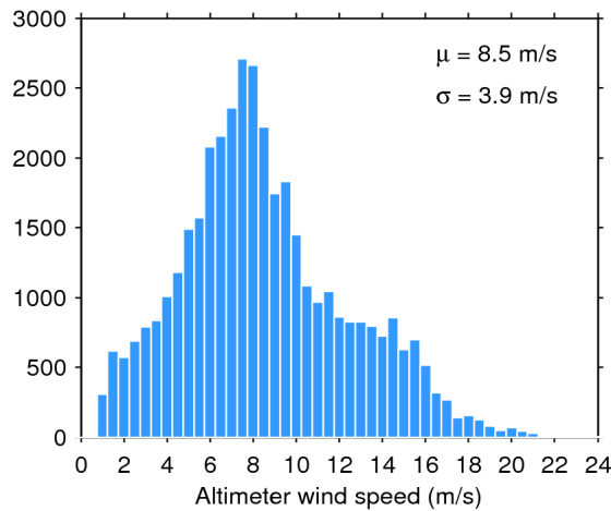
Figure 33. Histogram of flag-valid wind over oceans and lakes for 21/12/2017. The mean ( \mu ) and standard deviation ( \sigma ) are also shown. Note that values larger than 24 m/s are excluded from the histogram for the sake of readability but not from the computation of \mu and \sigma .
