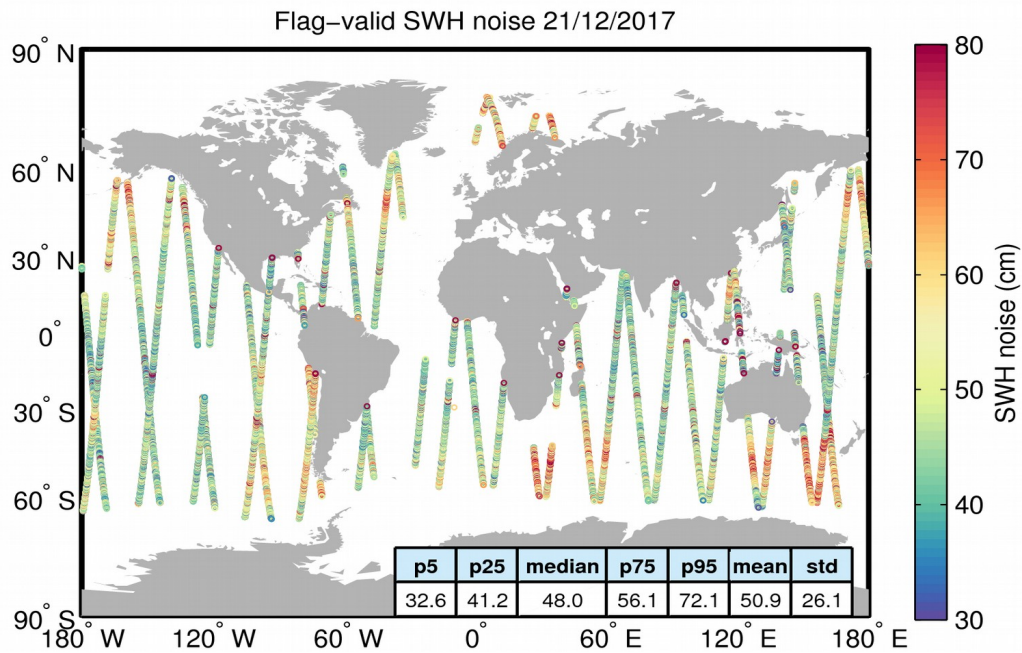
Figure 18. Geographical distribution of flag-valid 20-Hz SWH measurement noise over oceans and lakes for 21/12/2017. The statistical values shown in the table refer to the SWH noise and are calculated over all measurements shown in the figure.
