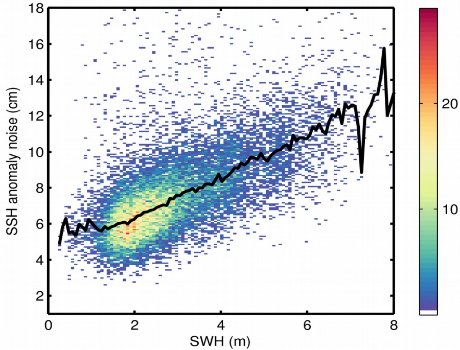
Figure 9. 2D histogram showing flag-valid SSH anomaly noise as a function of SWH for 21/12/2017. The black line denotes the median SSH anomaly noise as a function of SWH.
