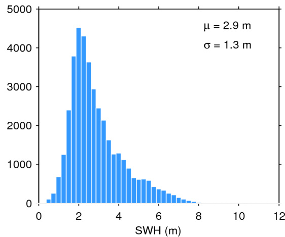
Figure 17. Histogram of flag-valid SWH over oceans and lakes for 21/12/2017. The mean ( \mu ) and standard deviation ( \sigma ) are also shown. Note that values larger than 12 m are excluded from the histogram for the sake of readability but not from the computation of \mu and \sigma .
