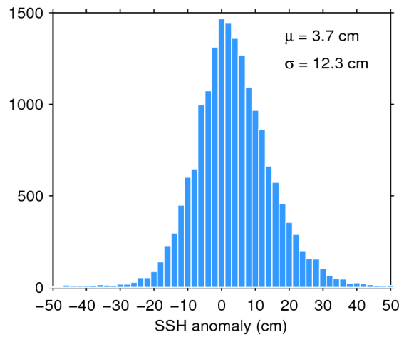
Figure 11. Histogram of science-valid SSH anomaly over oceans and lakes for 21/12/2017. The mean ( \mu ) and standard deviation ( \sigma ) are also shown. Note that values outside [-50 50] cm are excluded from the histogram for the sake of readability but not from the computation of \mu and \sigma .
