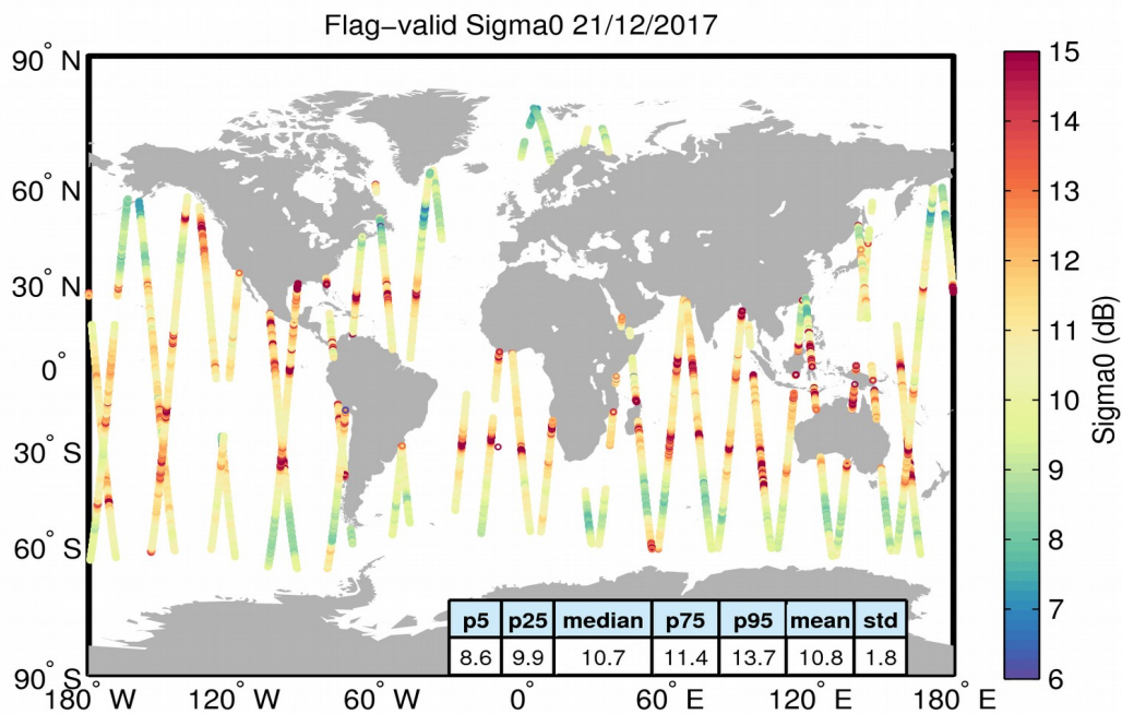
Figure 23. Geographical distribution of flag-valid sigma0 data over oceans and lakes for 21/12/2017. The statistical values shown in the table refer to the sigma0 in dB and are calculated over all measurements shown in the figure.
