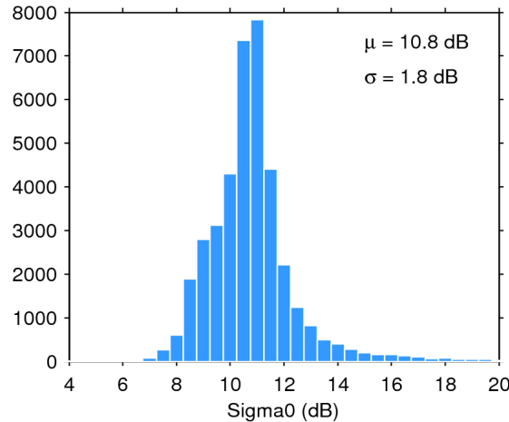
Figure 25. Histogram of flag-valid sigma0 over oceans and lakes for 21/12/2017. The mean ( \mu ) and standard deviation ( \sigma ) are also shown. Note that values outside [4 20] dB are excluded from the histogram for the sake of readability but not from the computation of \mu and \sigma .
