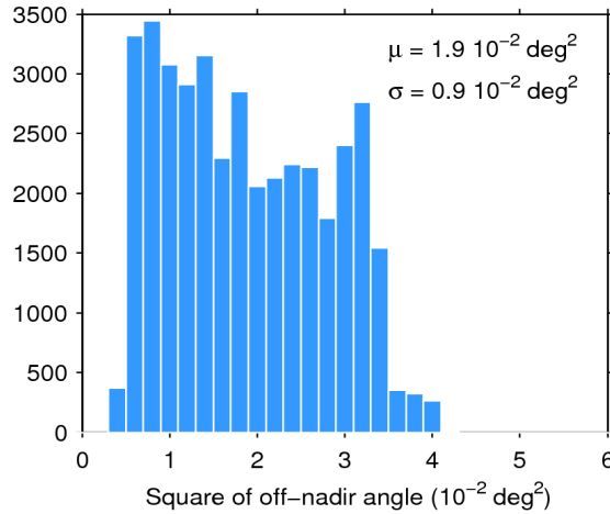
Figure 39. Histogram of flag-valid mispointing over oceans and lakes for 21/12/2017. The mean ( \mu ) and standard deviation ( \sigma ) are also shown. Note that values larger than 6 \cdot 10^{-2} \text{ deg}^2 are excluded from the histogram for the sake of readability but not from the computation of \mu and \sigma .
