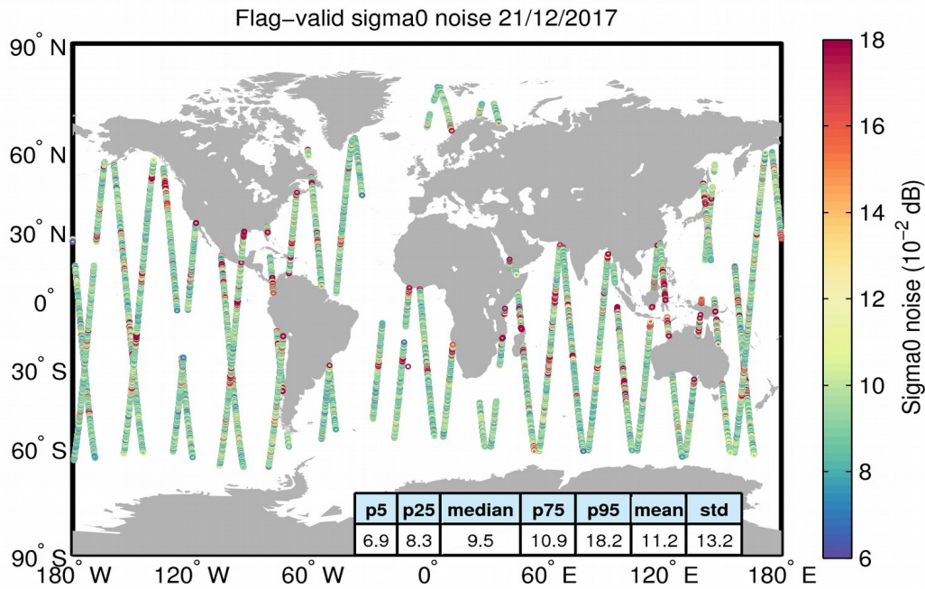
Figure 26. Geographical distribution of flag-valid 20-Hz sigma0 measurement noise over oceans and lakes for 21/12/2017. The statistical values shown in the table refer to the sigma0 noise and are calculated over all measurements shown in the figure.
