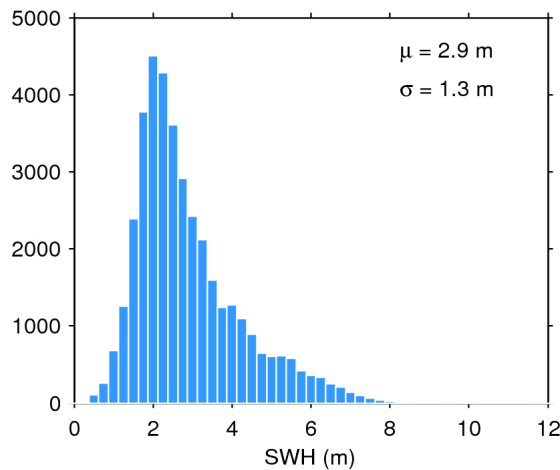
Figure 20. Histogram of science-valid SWH over oceans and lakes for 21/12/2017. The mean ( \mu ) and standard deviation ( \sigma ) are also shown. Note that values larger than 12 m are excluded from the histogram for the sake of readability but not from the computation of \mu and \sigma .
