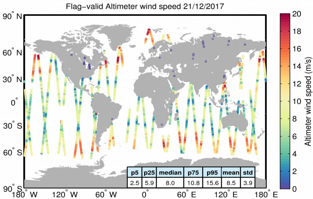
Figure 31. Geographical distribution of flag-valid wind data over oceans and lakes for 21/12/2017. The statistical values shown in the table refer to the wind in m/s and are calculated over all measurements shown in the figure.
