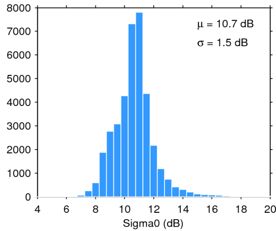
Figure 28. Histogram of science-valid sigma0 over oceans and lakes for 21/12/2017. The mean ( \mu ) and standard deviation ( \sigma ) are also shown. Note that values outside [4 20] dB are excluded from the histogram for the sake of readability but not from the computation of \mu and \sigma .
