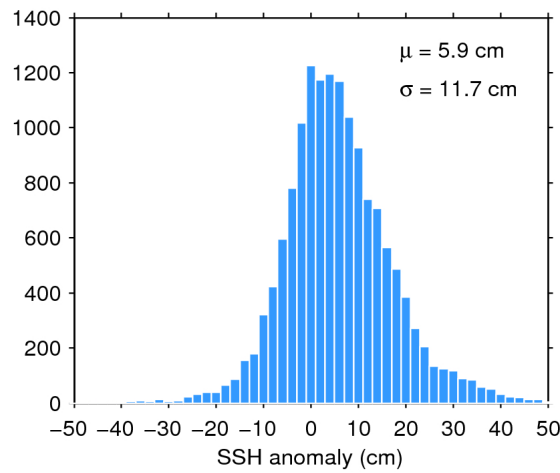
Figure 11. Histogram of science-valid SSH anomaly over oceans and lakes for 20/12/2017. The mean ( \mu ) and standard deviation ( \sigma ) are also shown. Note that values outside [-50 50] cm are excluded from the histogram for the sake of readability but not from the computation of \mu and \sigma .
