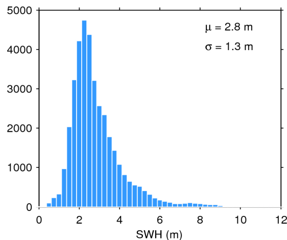
Figure 20. Histogram of science-valid SWH over oceans and lakes for 20/12/2017. The mean ( \mu ) and standard deviation ( \sigma ) are also shown. Note that values larger than 12 m are excluded from the histogram for the sake of readability but not from the computation of \mu and \sigma .
