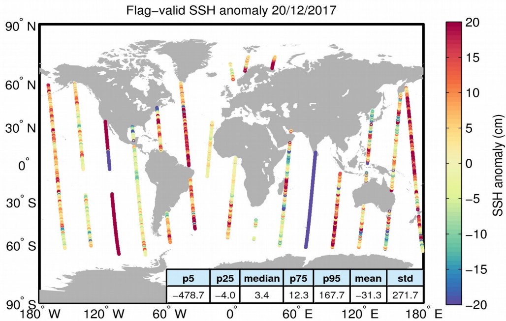
Figure 5. Geographical distribution of flag-valid 1-Hz SSH anomaly data over oceans and lakes for 20/12/2017. The statistical values shown in the table refer to the SSH anomaly in cm and are calculated over all measurements shown in the figure.
