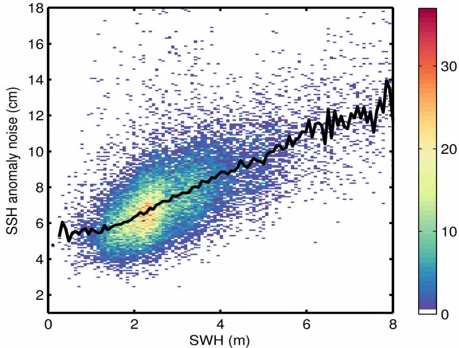
Figure 9. 2D histogram showing flag-valid SSH anomaly noise as a function of SWH for 20/12/2017. The black line denotes the median SSH anomaly noise as a function of SWH.
