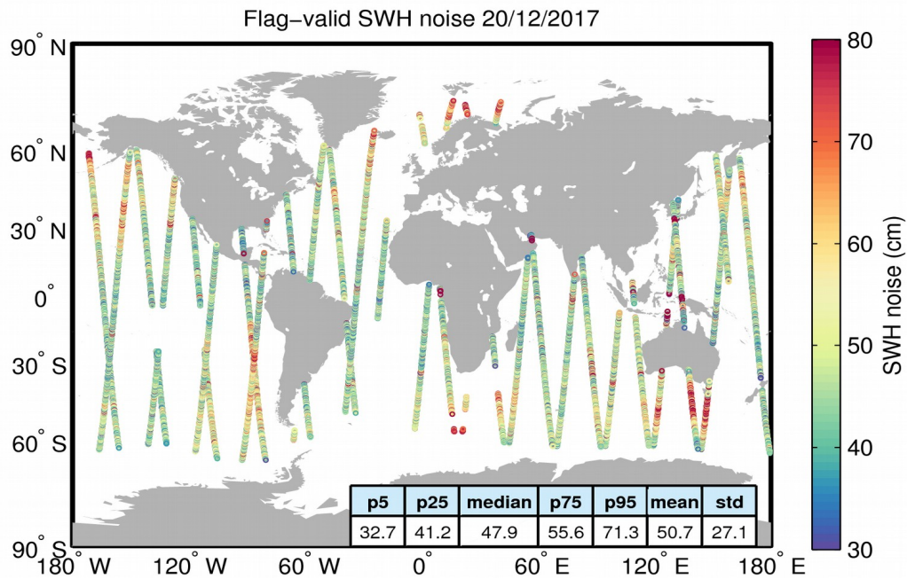
Figure 18. Geographical distribution of flag-valid 20-Hz SWH measurement noise over oceans and lakes for 20/12/2017. The statistical values shown in the table refer to the SWH noise and are calculated over all measurements shown in the figure.
