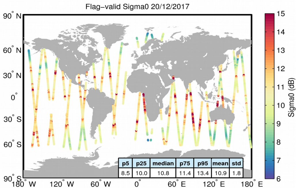
Figure 23. Geographical distribution of flag-valid sigma0 data over oceans and lakes for 20/12/2017. The statistical values shown in the table refer to the sigma0 in dB and are calculated over all measurements shown in the figure.
