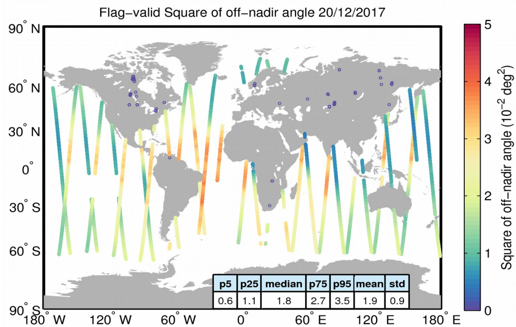
Figure 37. Geographical distribution of flag-valid mispointing data over oceans and lakes for 20/12/2017. The statistical values shown in the table refer to the mispointing in 10^{-2} deg 2 and are calculated over all measurements shown in the figure.
