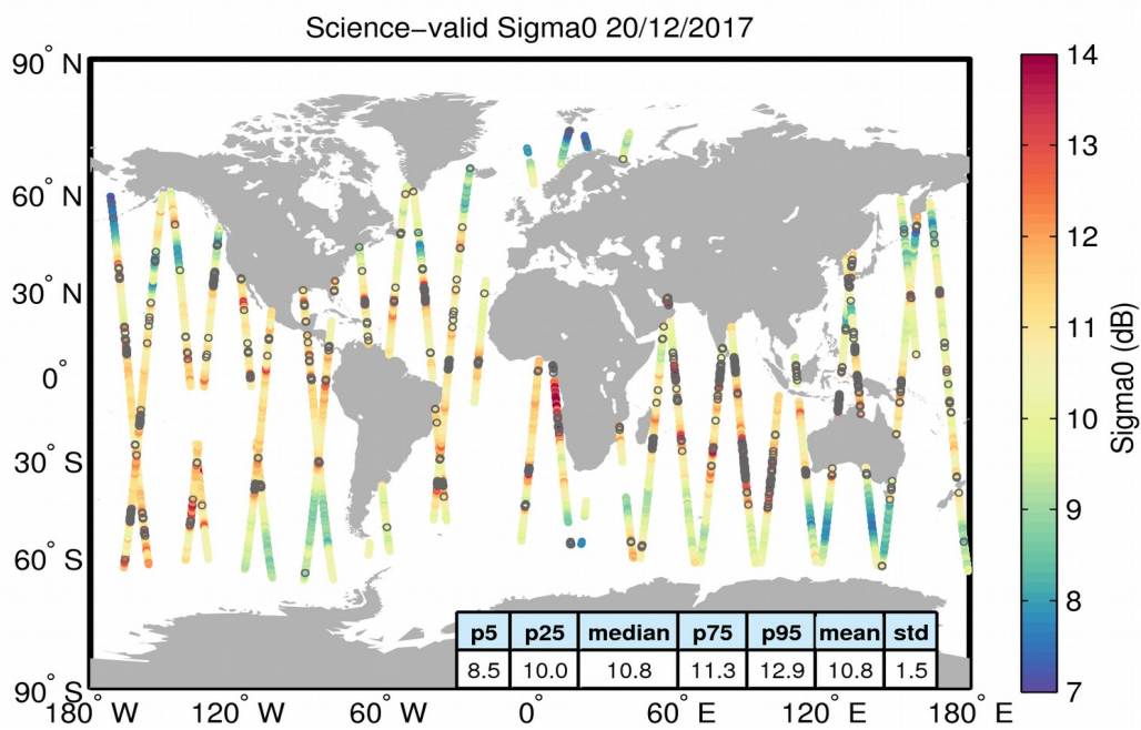
Figure 27. Geographical distribution of science-valid sigma0 data over oceans and lakes for 20/12/2017. The statistical values shown in the table refer to the sigma0 in dB and are calculated over all measurements shown in the figure. Gray circles denote records that have been rejected based on the editing criteria described in Table 4.
