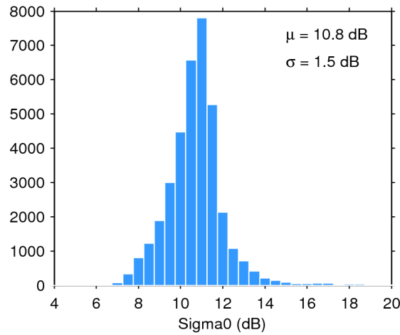
Figure 28. Histogram of science-valid sigma0 over oceans and lakes for 20/12/2017. The mean ( \mu ) and standard deviation ( \sigma ) are also shown. Note that values outside [4 20] dB are excluded from the histogram for the sake of readability but not from the computation of \mu and \sigma .
