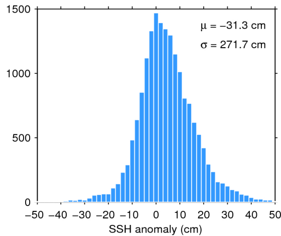
Figure 7. Histogram of flag-valid SSH anomaly over oceans and lakes for 20/12/2017. The mean ( \mu ) and standard deviation ( \sigma ) are also shown. Note that values outside [-50 50] cm are excluded from the histogram for the sake of readability but not from the computation of \mu and \sigma .
