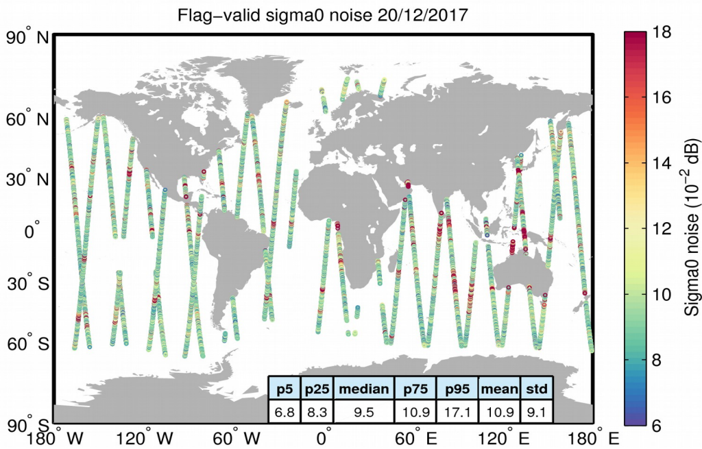
Figure 26. Geographical distribution of flag-valid 20-Hz sigma0 measurement noise over oceans and lakes for 20/12/2017. The statistical values shown in the table refer to the sigma0 noise and are calculated over all measurements shown in the figure.
