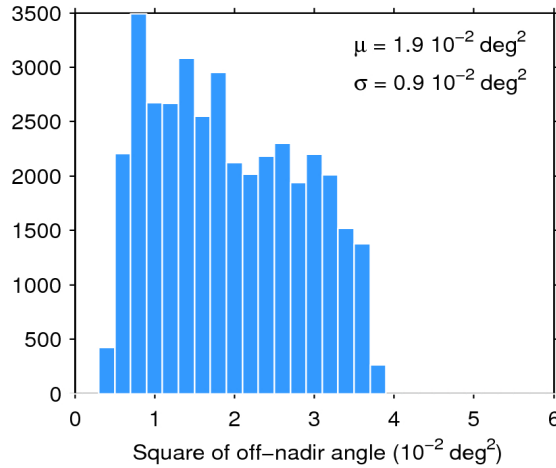
Figure 39. Histogram of flag-valid mispointing over oceans and lakes for 20/12/2017. The mean ( \mu ) and standard deviation ( \sigma ) are also shown. Note that values larger than 6 \cdot 10^{-2} \text{ deg}^2 are excluded from the histogram for the sake of readability but not from the computation of \mu and \sigma .
