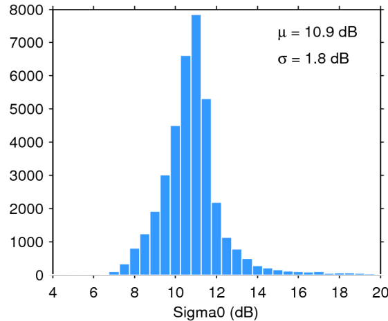
Figure 25. Histogram of flag-valid sigma0 over oceans and lakes for 20/12/2017. The mean ( \mu ) and standard deviation ( \sigma ) are also shown. Note that values outside [4 20] dB are excluded from the histogram for the sake of readability but not from the computation of \mu and \sigma .
