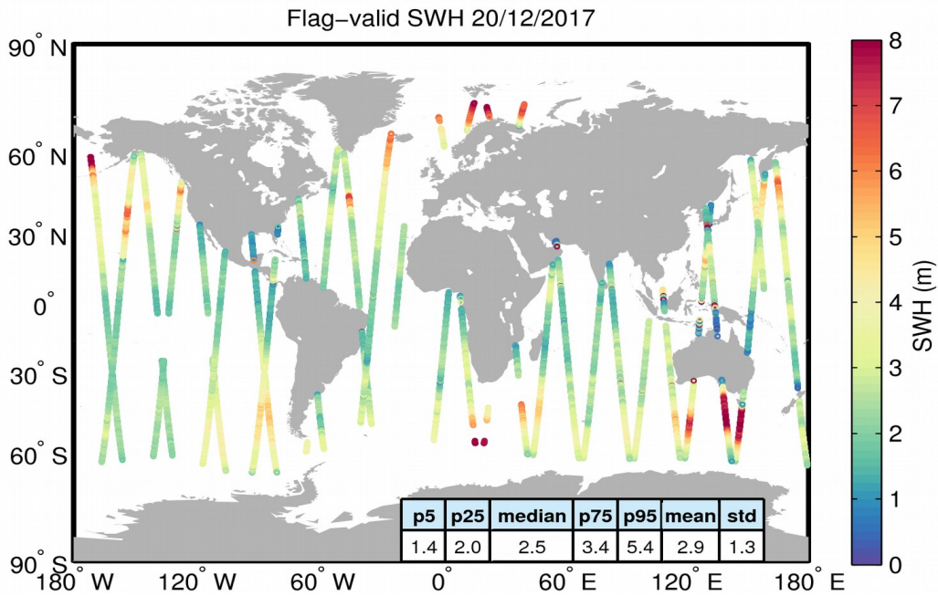
Figure 15. Geographical distribution of flag-valid SWH data over oceans and lakes for 20/12/2017. The statistical values shown in the table refer to the SWH in m and are calculated over all measurements shown in the figure.
