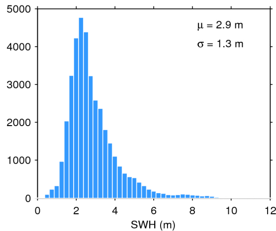
Figure 17. Histogram of flag-valid SWH over oceans and lakes for 20/12/2017. The mean ( \mu ) and standard deviation ( \sigma ) are also shown. Note that values larger than 12 m are excluded from the histogram for the sake of readability but not from the computation of \mu and \sigma .
