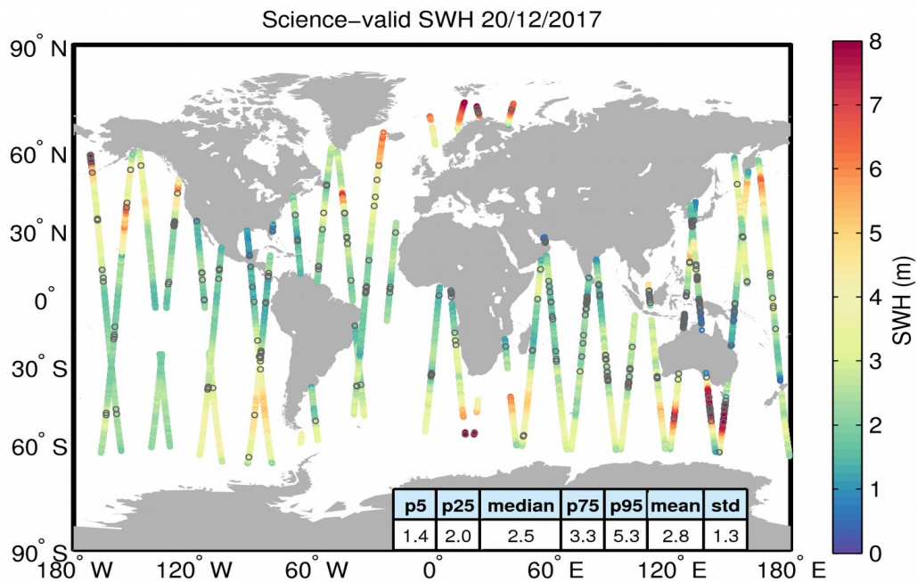
Figure 19. Geographical distribution of science-valid SWH data over oceans and lakes for 20/12/2017. The statistical values shown in the table refer to the SWH in m and are calculated over all measurements shown in the figure. Gray circles denote records that have been rejected based on the editing criteria described in Table 3.
