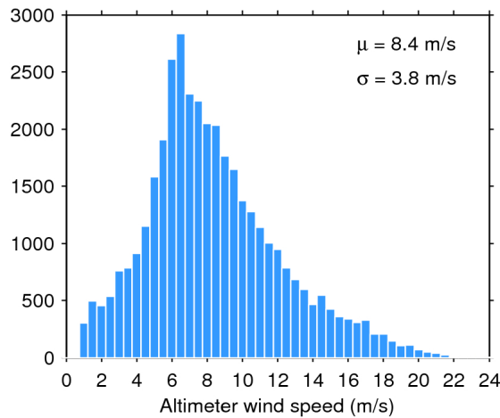
Figure 33. Histogram of flag-valid wind over oceans and lakes for 20/12/2017. The mean ( \mu ) and standard deviation ( \sigma ) are also shown. Note that values larger than 24 m/s are excluded from the histogram for the sake of readability but not from the computation of \mu and \sigma .
