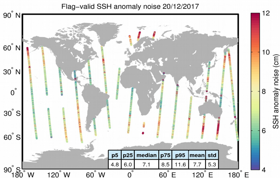
Figure 8. Geographical distribution of flag-valid 20-Hz SSH anomaly measurement noise over oceans and lakes for 20/12/2017. The statistical values shown in the table refer to the SSH anomaly noise and are calculated over all measurements shown in the figure.
