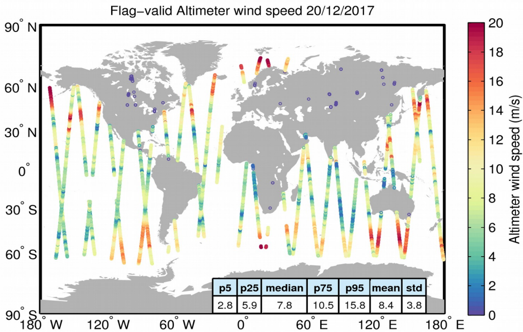
Figure 31. Geographical distribution of flag-valid wind data over oceans and lakes for 20/12/2017. The statistical values shown in the table refer to the wind in m/s and are calculated over all measurements shown in the figure.
