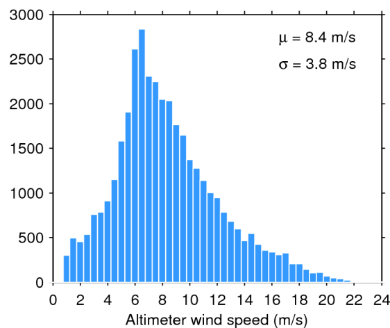
Figure 35. Histogram of science-valid wind over oceans and lakes for 20/12/2017. The mean ( \mu ) and standard deviation ( \sigma ) are also shown. Note that values larger than 24 m/s are excluded from the histogram for the sake of readability but not from the computation of \mu and \sigma .
