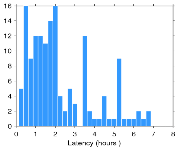
Figure 2. Histogram of the data latency for 20/12/2017. The y-axis denotes the number of files that are made available with a delay of x-hours with respect to the mean time of the records stored in the file.
