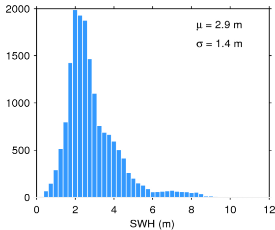
Figure 20. Histogram of science-valid SWH over oceans and lakes for 18/12/2017. The mean ( \mu ) and standard deviation ( \sigma ) are also shown. Note that values larger than 12 m are excluded from the histogram for the sake of readability but not from the computation of \mu and \sigma .
