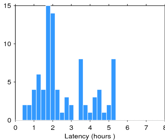
Figure 2. Histogram of the data latency for 18/12/2017. The y-axis denotes the number of files that are made available with a delay of x-hours with respect to the mean time of the records stored in the file.
