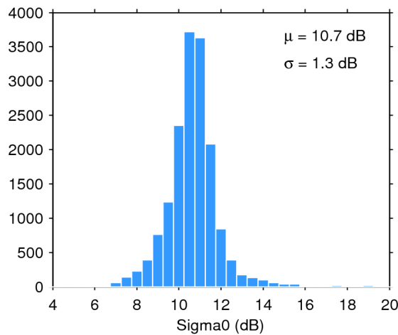
Figure 28. Histogram of science-valid sigma0 over oceans and lakes for 18/12/2017. The mean ( \mu ) and standard deviation ( \sigma ) are also shown. Note that values outside [4 20] dB are excluded from the histogram for the sake of readability but not from the computation of \mu and \sigma .
