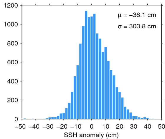
Figure 7. Histogram of flag-valid SSH anomaly over oceans and lakes for 18/12/2017. The mean ( \mu ) and standard deviation ( \sigma ) are also shown. Note that values outside [-50 50] cm are excluded from the histogram for the sake of readability but not from the computation of \mu and \sigma .
