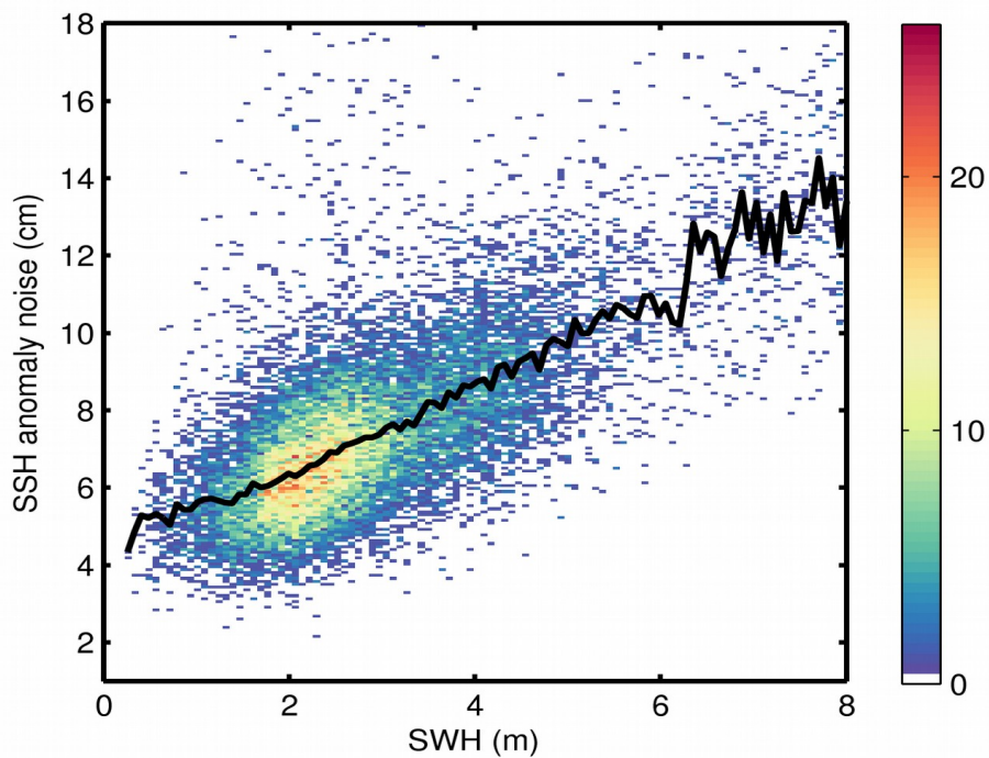
Figure 9. 2D histogram showing flag-valid SSH anomaly noise as a function of SWH for 18/12/2017. The black line denotes the median SSH anomaly noise as a function of SWH.
