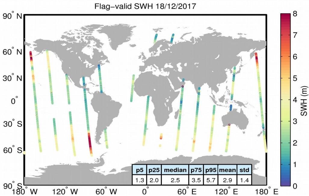
Figure 15. Geographical distribution of flag-valid SWH data over oceans and lakes for 18/12/2017. The statistical values shown in the table refer to the SWH in m and are calculated over all measurements shown in the figure.
