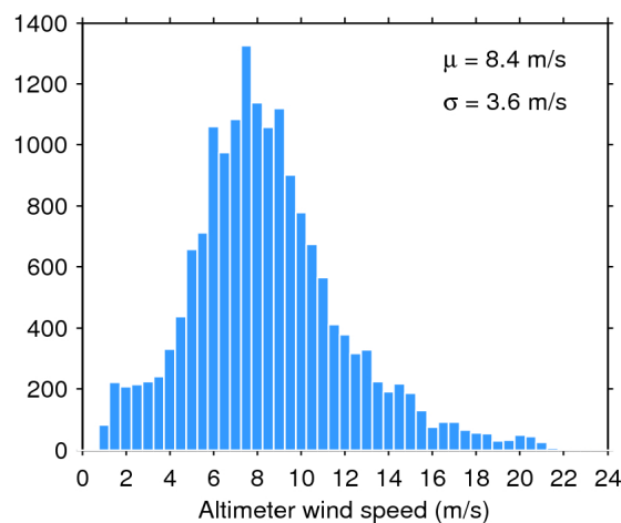
Figure 35. Histogram of science-valid wind over oceans and lakes for 18/12/2017. The mean ( \mu ) and standard deviation ( \sigma ) are also shown. Note that values larger than 24 m/s are excluded from the histogram for the sake of readability but not from the computation of \mu and \sigma .
