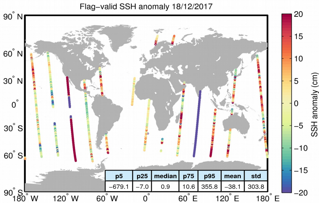
Figure 5. Geographical distribution of flag-valid 1-Hz SSH anomaly data over oceans and lakes for 18/12/2017. The statistical values shown in the table refer to the SSH anomaly in cm and are calculated over all measurements shown in the figure.
