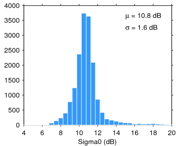
Figure 25. Histogram of flag-valid sigma0 over oceans and lakes for 18/12/2017. The mean ( \mu ) and standard deviation ( \sigma ) are also shown. Note that values outside [4 20] dB are excluded from the histogram for the sake of readability but not from the computation of \mu and \sigma .
