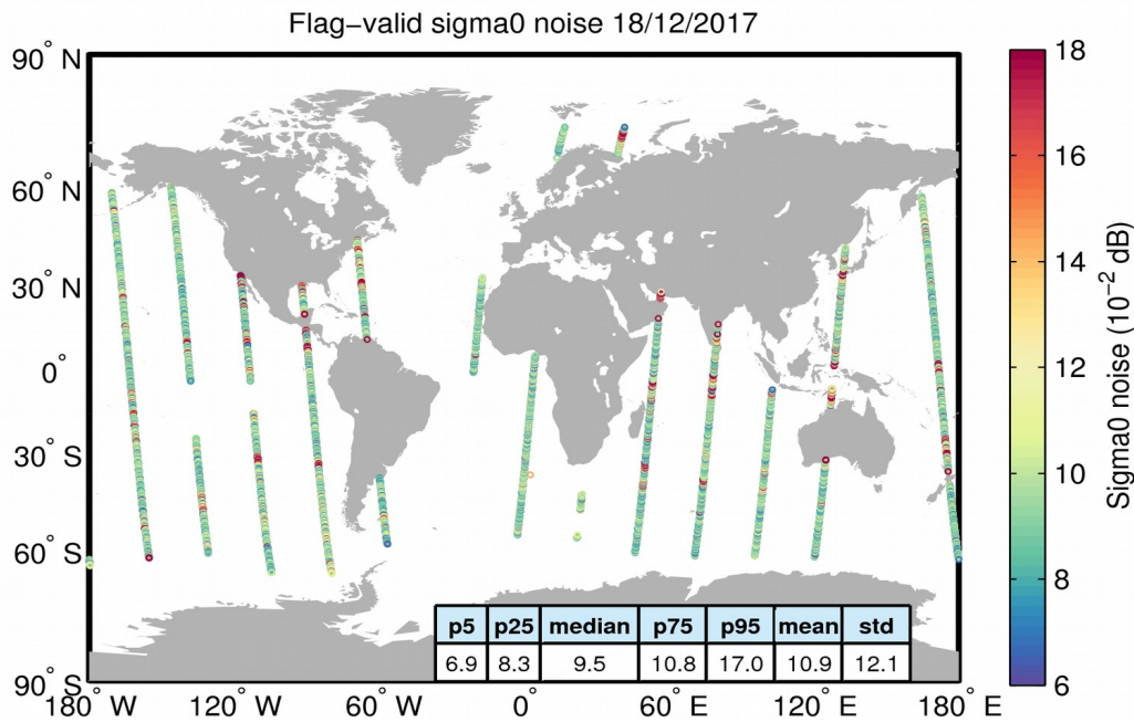
Figure 26. Geographical distribution of flag-valid 20-Hz sigma0 measurement noise over oceans and lakes for 18/12/2017. The statistical values shown in the table refer to the sigma0 noise and are calculated over all measurements shown in the figure.
