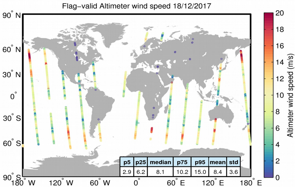
Figure 31. Geographical distribution of flag-valid wind data over oceans and lakes for 18/12/2017. The statistical values shown in the table refer to the wind in m/s and are calculated over all measurements shown in the figure.
