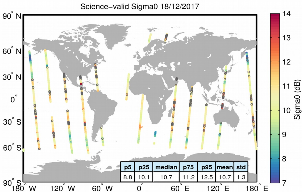
Figure 27. Geographical distribution of science-valid sigma0 data over oceans and lakes for 18/12/2017. The statistical values shown in the table refer to the sigma0 in dB and are calculated over all measurements shown in the figure. Gray circles denote records that have been rejected based on the editing criteria described in Table 4.
