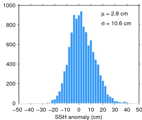
Figure 11. Histogram of science-valid SSH anomaly over oceans and lakes for 18/12/2017. The mean ( \mu ) and standard deviation ( \sigma ) are also shown. Note that values outside [-50 50] cm are excluded from the histogram for the sake of readability but not from the computation of \mu and \sigma .
