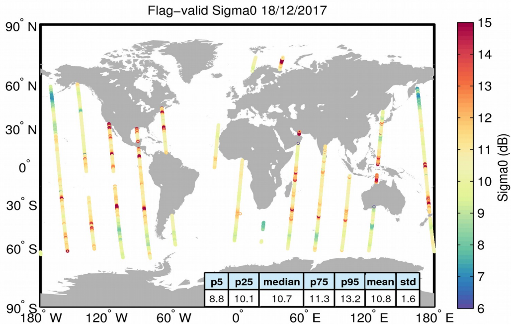
Figure 23. Geographical distribution of flag-valid sigma0 data over oceans and lakes for 18/12/2017. The statistical values shown in the table refer to the sigma0 in dB and are calculated over all measurements shown in the figure.
