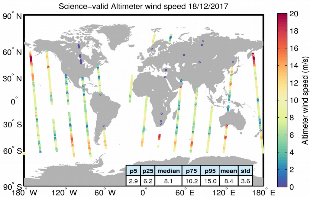
Figure 34. Geographical distribution of science-valid wind data over oceans and lakes for 18/12/2017. The statistical values shown in the table refer to the wind in m/s and are calculated over all measurements shown in the figure. Gray circles denote records that have been rejected based on the editing criteria described in Table 5.
