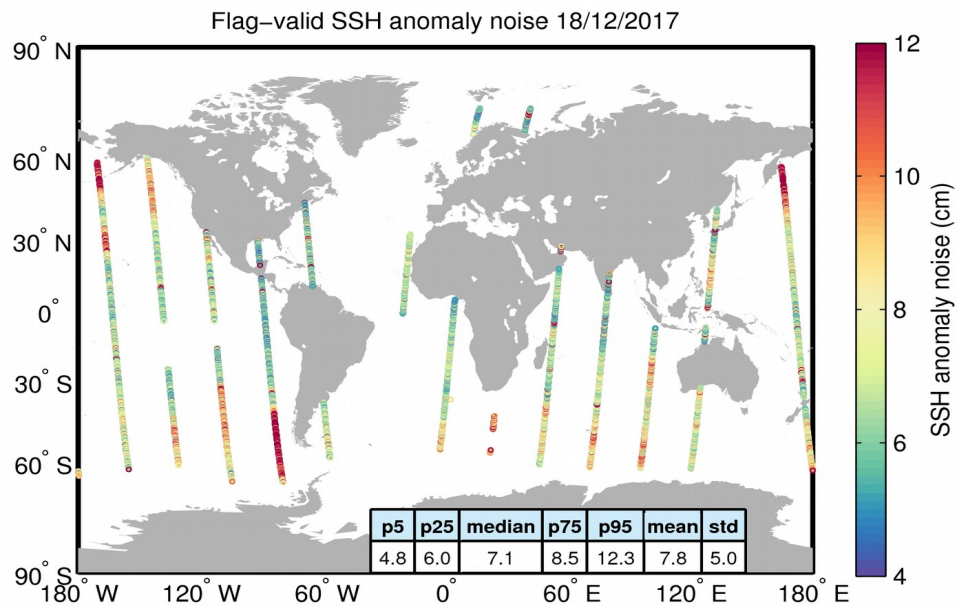
Figure 8. Geographical distribution of flag-valid 20-Hz SSH anomaly measurement noise over oceans and lakes for 18/12/2017. The statistical values shown in the table refer to the SSH anomaly noise and are calculated over all measurements shown in the figure.
