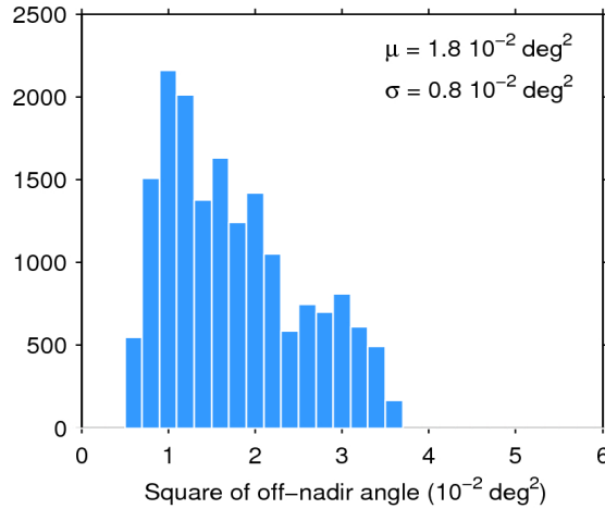
Figure 39. Histogram of flag-valid mispointing over oceans and lakes for 18/12/2017. The mean ( \mu ) and standard deviation ( \sigma ) are also shown. Note that values larger than 6 \cdot 10^{-2} \text{ deg}^2 are excluded from the histogram for the sake of readability but not from the computation of \mu and \sigma .
