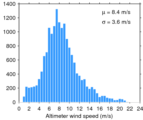
Figure 33. Histogram of flag-valid wind over oceans and lakes for 18/12/2017. The mean ( \mu ) and standard deviation ( \sigma ) are also shown. Note that values larger than 24 m/s are excluded from the histogram for the sake of readability but not from the computation of \mu and \sigma .
