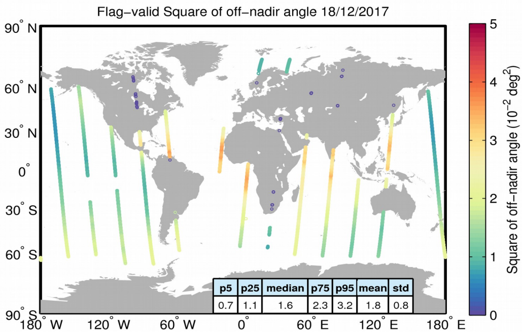
Figure 37. Geographical distribution of flag-valid mispointing data over oceans and lakes for 18/12/2017. The statistical values shown in the table refer to the mispointing in 10^{-2} deg 2 and are calculated over all measurements shown in the figure.
