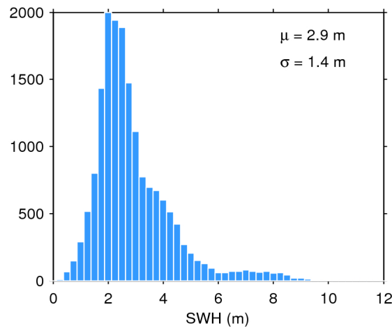
Figure 17. Histogram of flag-valid SWH over oceans and lakes for 18/12/2017. The mean ( \mu ) and standard deviation ( \sigma ) are also shown. Note that values larger than 12 m are excluded from the histogram for the sake of readability but not from the computation of \mu and \sigma .
