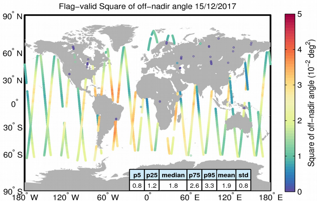
Figure 37. Geographical distribution of flag-valid mispointing data over oceans and lakes for 15/12/2017. The statistical values shown in the table refer to the mispointing in 10^{-2} deg 2 and are calculated over all measurements shown in the figure.
