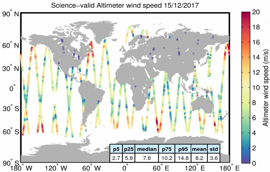
Figure 34. Geographical distribution of science-valid wind data over oceans and lakes for 15/12/2017. The statistical values shown in the table refer to the wind in m/s and are calculated over all measurements shown in the figure. Gray circles denote records that have been rejected based on the editing criteria described in Table 5.
