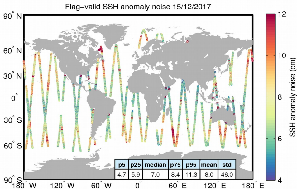
Figure 8. Geographical distribution of flag-valid 20-Hz SSH anomaly measurement noise over oceans and lakes for 15/12/2017. The statistical values shown in the table refer to the SSH anomaly noise and are calculated over all measurements shown in the figure.
