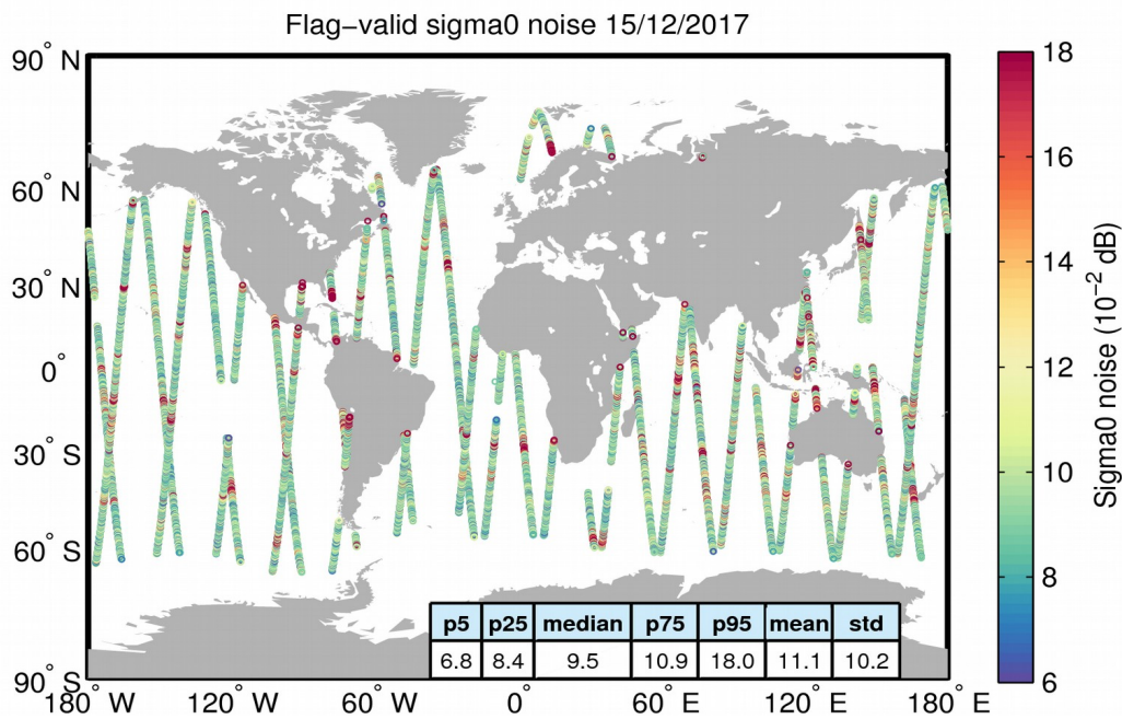
Figure 26. Geographical distribution of flag-valid 20-Hz sigma0 measurement noise over oceans and lakes for 15/12/2017. The statistical values shown in the table refer to the sigma0 noise and are calculated over all measurements shown in the figure.
