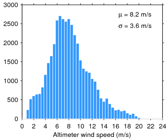
Figure 33. Histogram of flag-valid wind over oceans and lakes for 15/12/2017. The mean ( \mu ) and standard deviation ( \sigma ) are also shown. Note that values larger than 24 m/s are excluded from the histogram for the sake of readability but not from the computation of \mu and \sigma .
