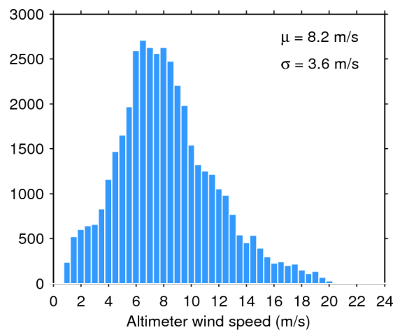
Figure 35. Histogram of science-valid wind over oceans and lakes for 15/12/2017. The mean ( \mu ) and standard deviation ( \sigma ) are also shown. Note that values larger than 24 m/s are excluded from the histogram for the sake of readability but not from the computation of \mu and \sigma .
