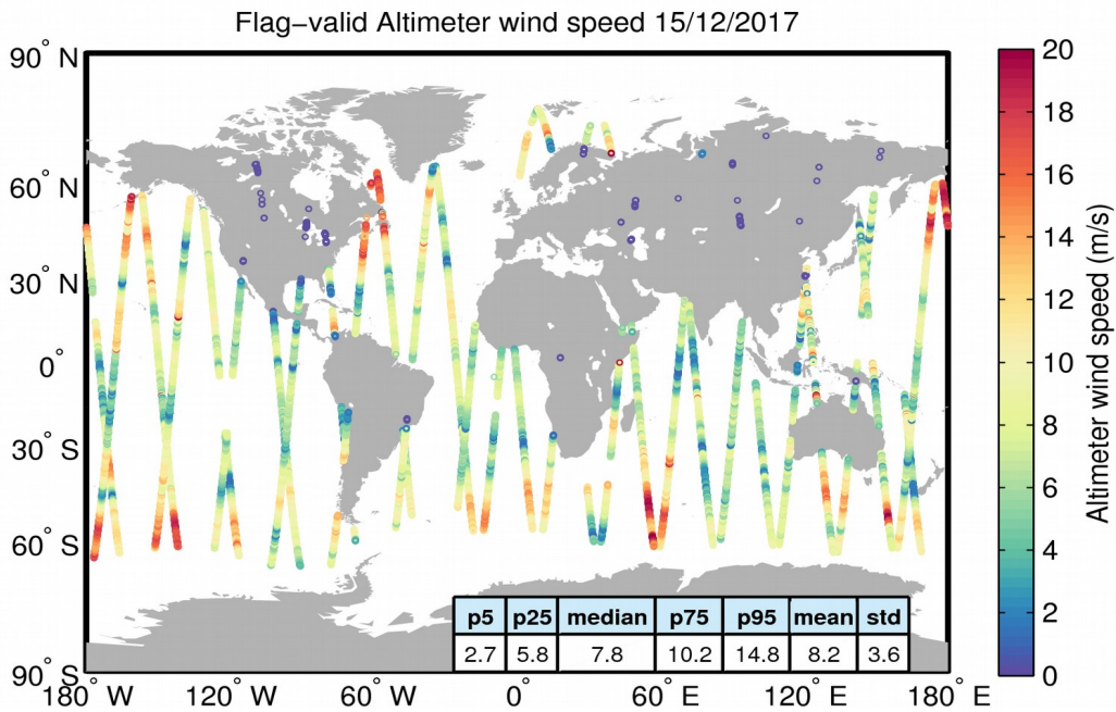
Figure 31. Geographical distribution of flag-valid wind data over oceans and lakes for 15/12/2017. The statistical values shown in the table refer to the wind in m/s and are calculated over all measurements shown in the figure.
