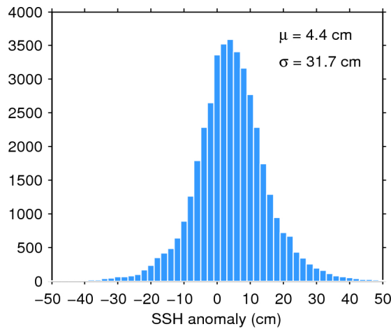
Figure 7. Histogram of flag-valid SSH anomaly over oceans and lakes for 15/12/2017. The mean ( \mu ) and standard deviation ( \sigma ) are also shown. Note that values outside [-50 50] cm are excluded from the histogram for the sake of readability but not from the computation of \mu and \sigma .
