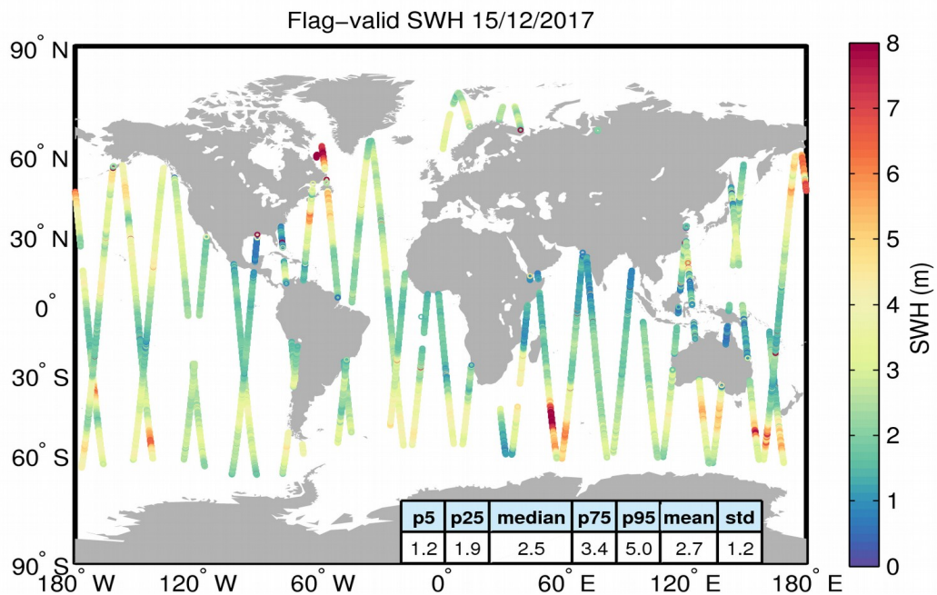
Figure 15. Geographical distribution of flag-valid SWH data over oceans and lakes for 15/12/2017. The statistical values shown in the table refer to the SWH in m and are calculated over all measurements shown in the figure.
