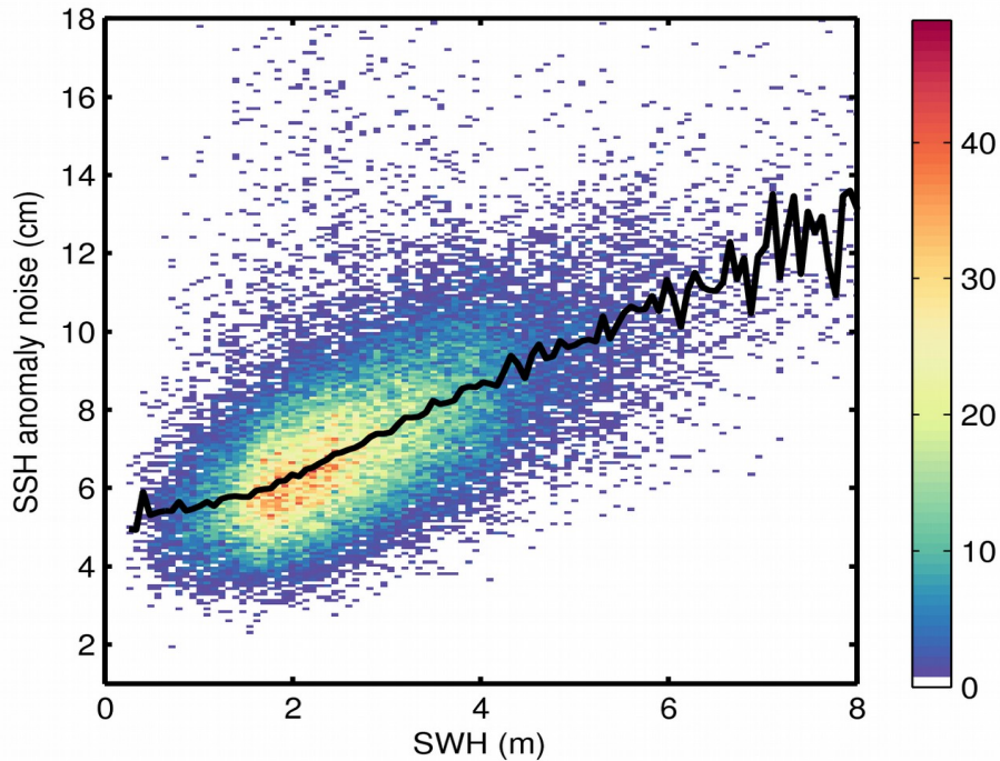
Figure 9. 2D histogram showing flag-valid SSH anomaly noise as a function of SWH for 15/12/2017. The black line denotes the median SSH anomaly noise as a function of SWH.
