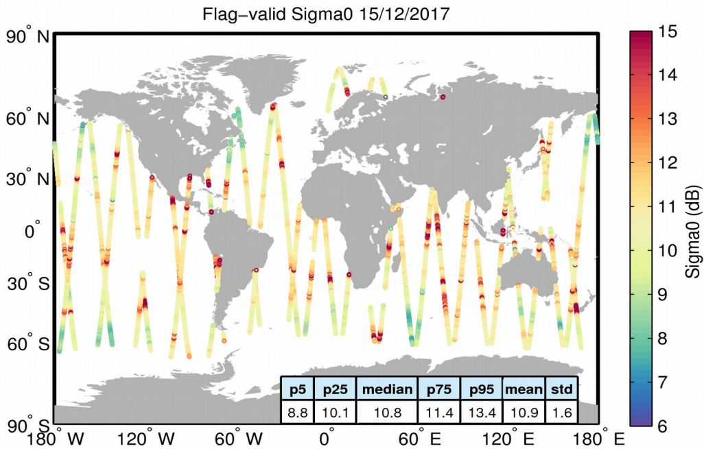
Figure 23. Geographical distribution of flag-valid sigma0 data over oceans and lakes for 15/12/2017. The statistical values shown in the table refer to the sigma0 in dB and are calculated over all measurements shown in the figure.
