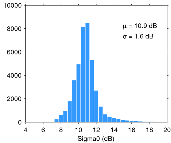
Figure 25. Histogram of flag-valid sigma0 over oceans and lakes for 15/12/2017. The mean ( \mu ) and standard deviation ( \sigma ) are also shown. Note that values outside [4 20] dB are excluded from the histogram for the sake of readability but not from the computation of \mu and \sigma .
