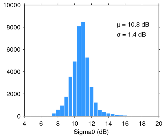
Figure 28. Histogram of science-valid sigma0 over oceans and lakes for 15/12/2017. The mean ( \mu ) and standard deviation ( \sigma ) are also shown. Note that values outside [4 20] dB are excluded from the histogram for the sake of readability but not from the computation of \mu and \sigma .
