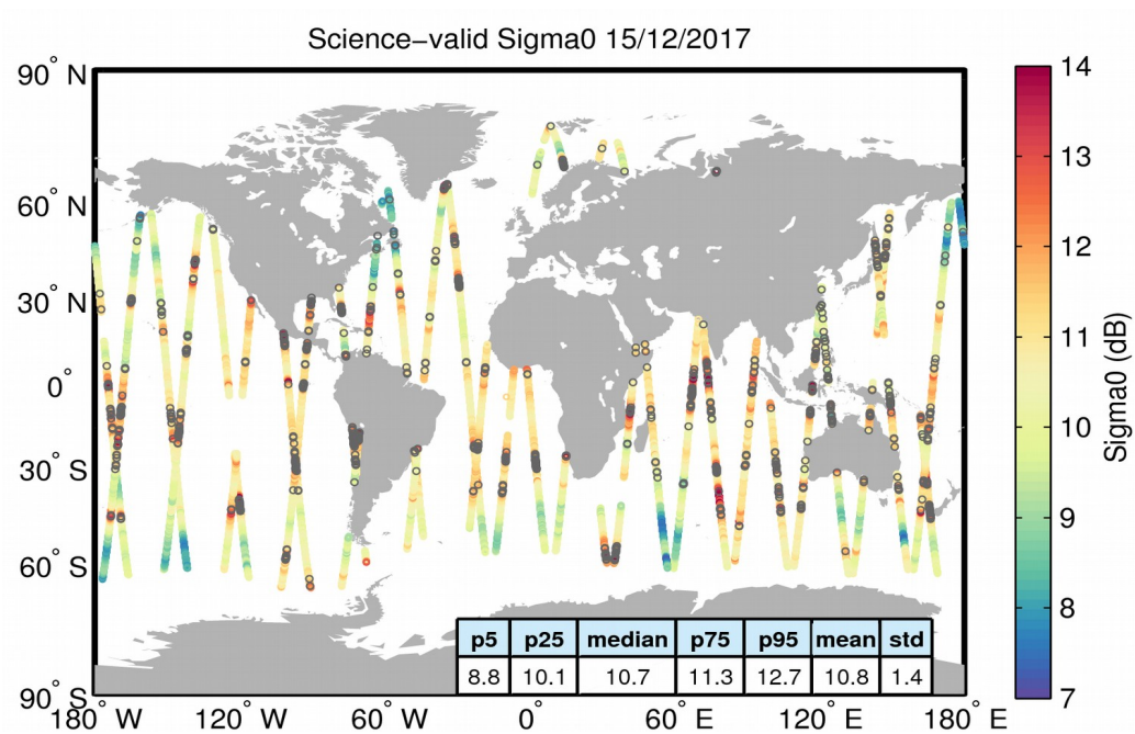
Figure 27. Geographical distribution of science-valid sigma0 data over oceans and lakes for 15/12/2017. The statistical values shown in the table refer to the sigma0 in dB and are calculated over all measurements shown in the figure. Gray circles denote records that have been rejected based on the editing criteria described in Table 4.
