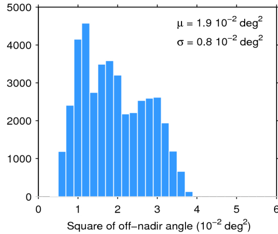
Figure 39. Histogram of flag-valid mispointing over oceans and lakes for 15/12/2017. The mean ( \mu ) and standard deviation ( \sigma ) are also shown. Note that values larger than 6 \cdot 10^{-2} \text{ deg}^2 are excluded from the histogram for the sake of readability but not from the computation of \mu and \sigma .
