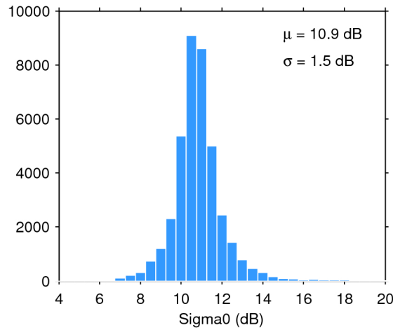
Figure 28. Histogram of science-valid sigma0 over oceans and lakes for 13/12/2017. The mean ( \mu ) and standard deviation ( \sigma ) are also shown. Note that values outside [4 20] dB are excluded from the histogram for the sake of readability but not from the computation of \mu and \sigma .
