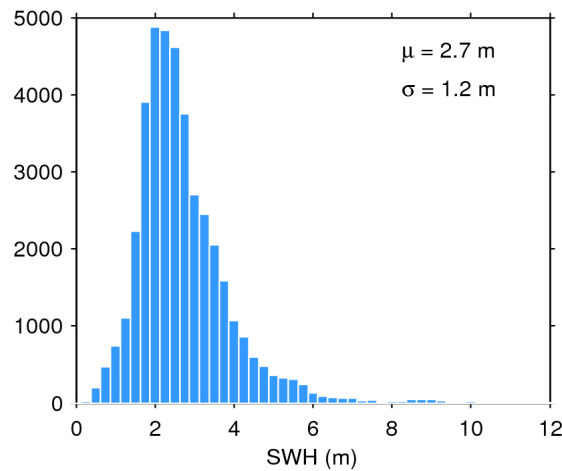
Figure 17. Histogram of flag-valid SWH over oceans and lakes for 13/12/2017. The mean ( \mu ) and standard deviation ( \sigma ) are also shown. Note that values larger than 12 m are excluded from the histogram for the sake of readability but not from the computation of \mu and \sigma .
