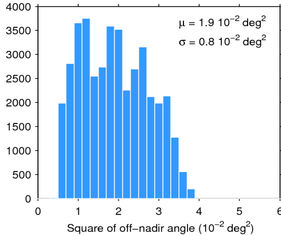
Figure 39. Histogram of flag-valid mispointing over oceans and lakes for 13/12/2017. The mean ( \mu ) and standard deviation ( \sigma ) are also shown. Note that values larger than 6 \cdot 10^{-2} \text{ deg}^2 are excluded from the histogram for the sake of readability but not from the computation of \mu and \sigma .
