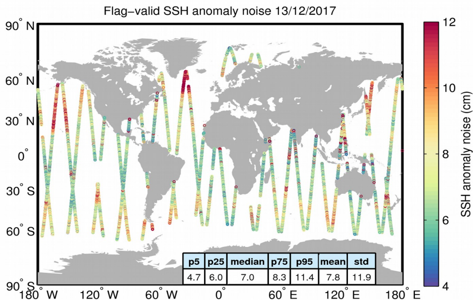
Figure 8. Geographical distribution of flag-valid 20-Hz SSH anomaly measurement noise over oceans and lakes for 13/12/2017. The statistical values shown in the table refer to the SSH anomaly noise and are calculated over all measurements shown in the figure.
