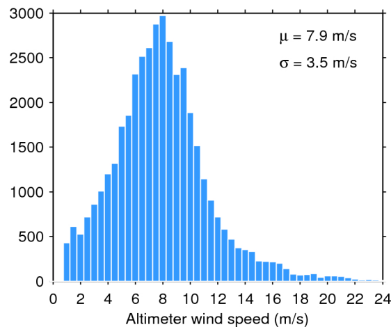
Figure 35. Histogram of science-valid wind over oceans and lakes for 13/12/2017. The mean ( \mu ) and standard deviation ( \sigma ) are also shown. Note that values larger than 24 m/s are excluded from the histogram for the sake of readability but not from the computation of \mu and \sigma .
