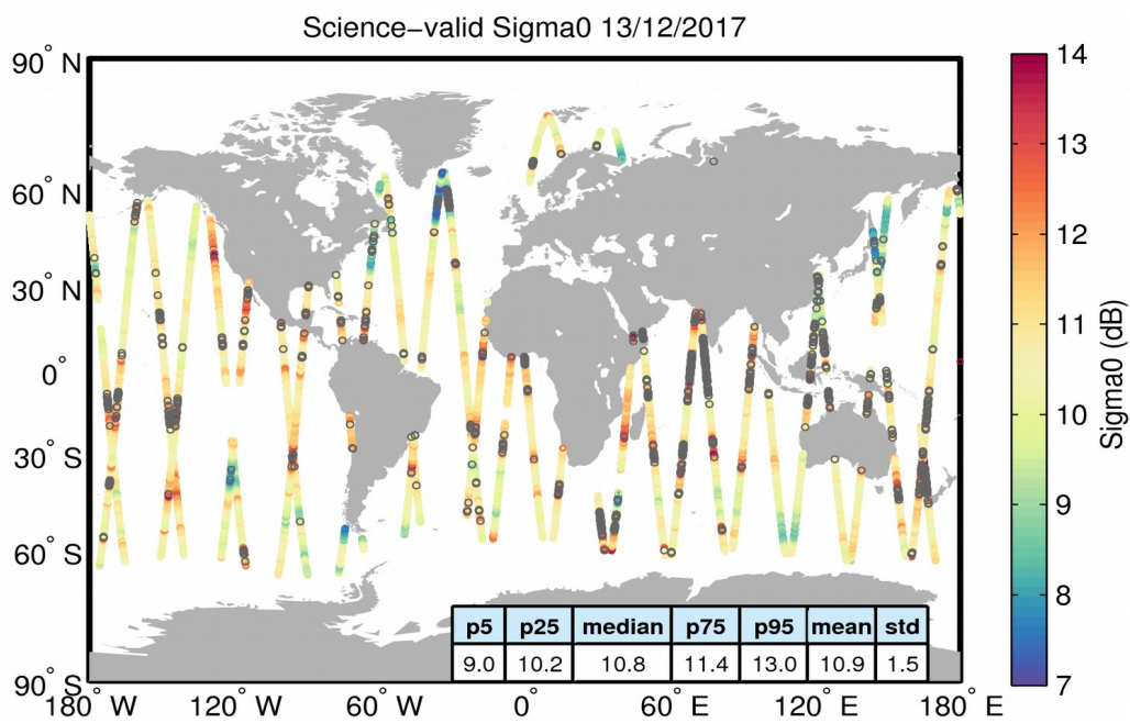
Figure 27. Geographical distribution of science-valid sigma0 data over oceans and lakes for 13/12/2017. The statistical values shown in the table refer to the sigma0 in dB and are calculated over all measurements shown in the figure. Gray circles denote records that have been rejected based on the editing criteria described in Table 4.
