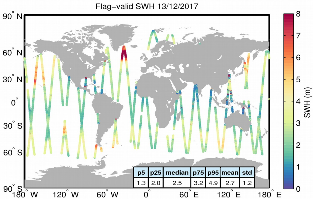
Figure 15. Geographical distribution of flag-valid SWH data over oceans and lakes for 13/12/2017. The statistical values shown in the table refer to the SWH in m and are calculated over all measurements shown in the figure.
