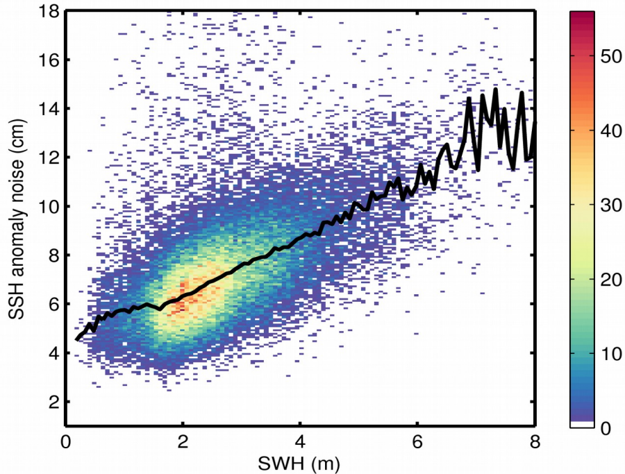
Figure 9. 2D histogram showing flag-valid SSH anomaly noise as a function of SWH for 13/12/2017. The black line denotes the median SSH anomaly noise as a function of SWH.
