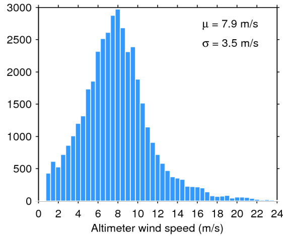
Figure 33. Histogram of flag-valid wind over oceans and lakes for 13/12/2017. The mean ( \mu ) and standard deviation ( \sigma ) are also shown. Note that values larger than 24 m/s are excluded from the histogram for the sake of readability but not from the computation of \mu and \sigma .
