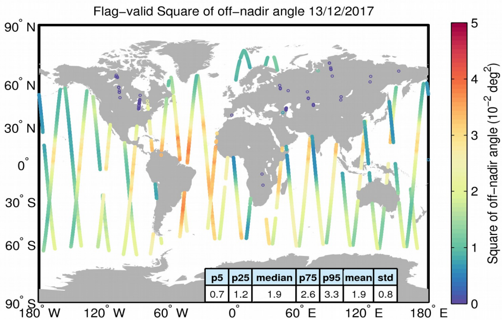
Figure 37. Geographical distribution of flag-valid mispointing data over oceans and lakes for 13/12/2017. The statistical values shown in the table refer to the mispointing in 10^{-2} deg 2 and are calculated over all measurements shown in the figure.
