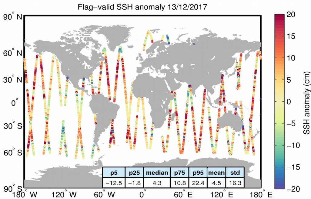
Figure 5. Geographical distribution of flag-valid 1-Hz SSH anomaly data over oceans and lakes for 13/12/2017. The statistical values shown in the table refer to the SSH anomaly in cm and are calculated over all measurements shown in the figure.
