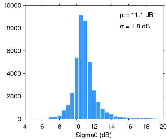
Figure 25. Histogram of flag-valid sigma0 over oceans and lakes for 13/12/2017. The mean ( \mu ) and standard deviation ( \sigma ) are also shown. Note that values outside [4 20] dB are excluded from the histogram for the sake of readability but not from the computation of \mu and \sigma .
