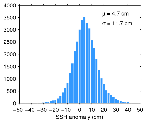
Figure 11. Histogram of science-valid SSH anomaly over oceans and lakes for 13/12/2017. The mean ( \mu ) and standard deviation ( \sigma ) are also shown. Note that values outside [-50 50] cm are excluded from the histogram for the sake of readability but not from the computation of \mu and \sigma .
