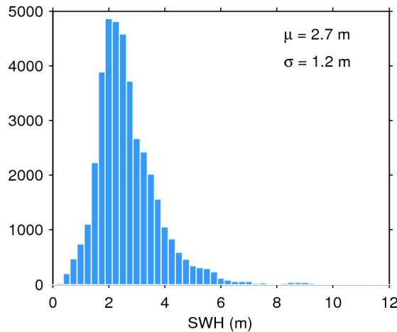
Figure 20. Histogram of science-valid SWH over oceans and lakes for 13/12/2017. The mean ( \mu ) and standard deviation ( \sigma ) are also shown. Note that values larger than 12 m are excluded from the histogram for the sake of readability but not from the computation of \mu and \sigma .
