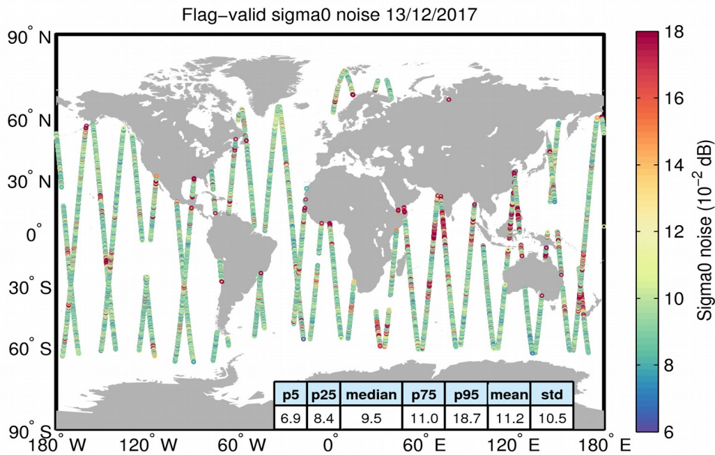
Figure 26. Geographical distribution of flag-valid 20-Hz sigma0 measurement noise over oceans and lakes for 13/12/2017. The statistical values shown in the table refer to the sigma0 noise and are calculated over all measurements shown in the figure.
