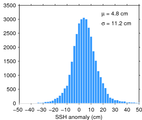
Figure 11. Histogram of science-valid SSH anomaly over oceans and lakes for 12/12/2017. The mean ( \mu ) and standard deviation ( \sigma ) are also shown. Note that values outside [-50 50] cm are excluded from the histogram for the sake of readability but not from the computation of \mu and \sigma .
