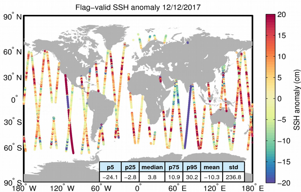
Figure 5. Geographical distribution of flag-valid 1-Hz SSH anomaly data over oceans and lakes for 12/12/2017. The statistical values shown in the table refer to the SSH anomaly in cm and are calculated over all measurements shown in the figure.
