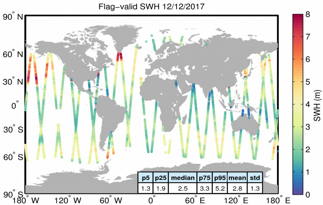
Figure 15. Geographical distribution of flag-valid SWH data over oceans and lakes for 12/12/2017. The statistical values shown in the table refer to the SWH in m and are calculated over all measurements shown in the figure.
