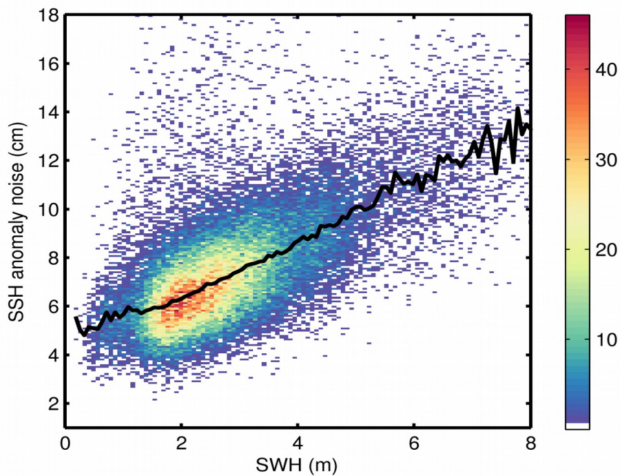
Figure 9. 2D histogram showing flag-valid SSH anomaly noise as a function of SWH for 12/12/2017. The black line denotes the median SSH anomaly noise as a function of SWH.
