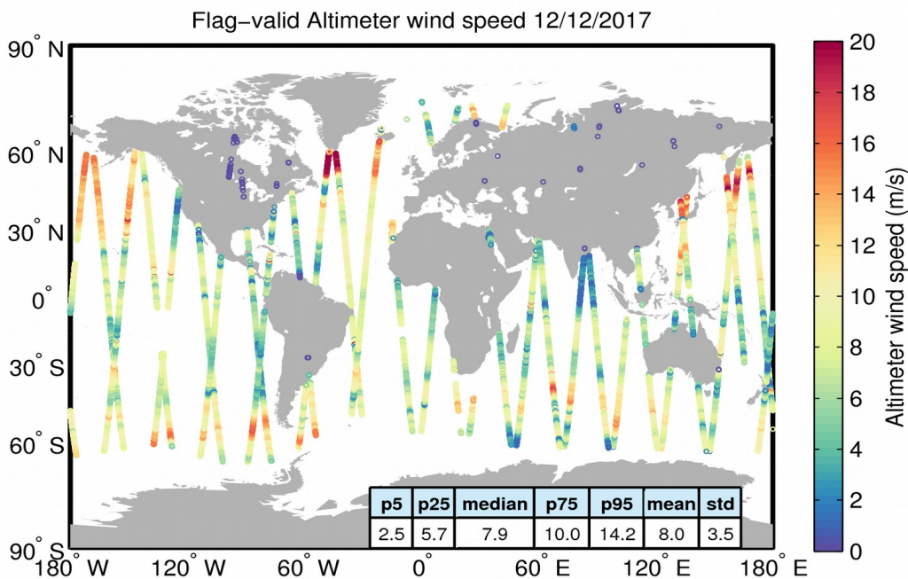
Figure 31. Geographical distribution of flag-valid wind data over oceans and lakes for 12/12/2017. The statistical values shown in the table refer to the wind in m/s and are calculated over all measurements shown in the figure.
