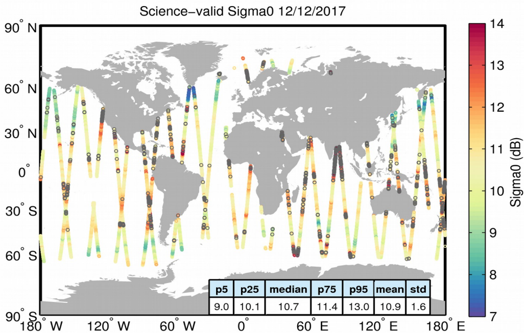
Figure 27. Geographical distribution of science-valid sigma0 data over oceans and lakes for 12/12/2017. The statistical values shown in the table refer to the sigma0 in dB and are calculated over all measurements shown in the figure. Gray circles denote records that have been rejected based on the editing criteria described in Table 4.
