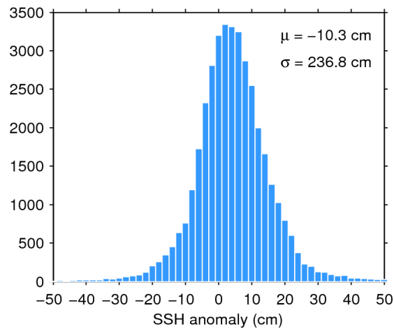
Figure 7. Histogram of flag-valid SSH anomaly over oceans and lakes for 12/12/2017. The mean ( \mu ) and standard deviation ( \sigma ) are also shown. Note that values outside [-50 50] cm are excluded from the histogram for the sake of readability but not from the computation of \mu and \sigma .
