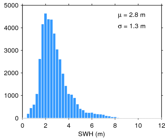
Figure 17. Histogram of flag-valid SWH over oceans and lakes for 12/12/2017. The mean ( \mu ) and standard deviation ( \sigma ) are also shown. Note that values larger than 12 m are excluded from the histogram for the sake of readability but not from the computation of \mu and \sigma .
