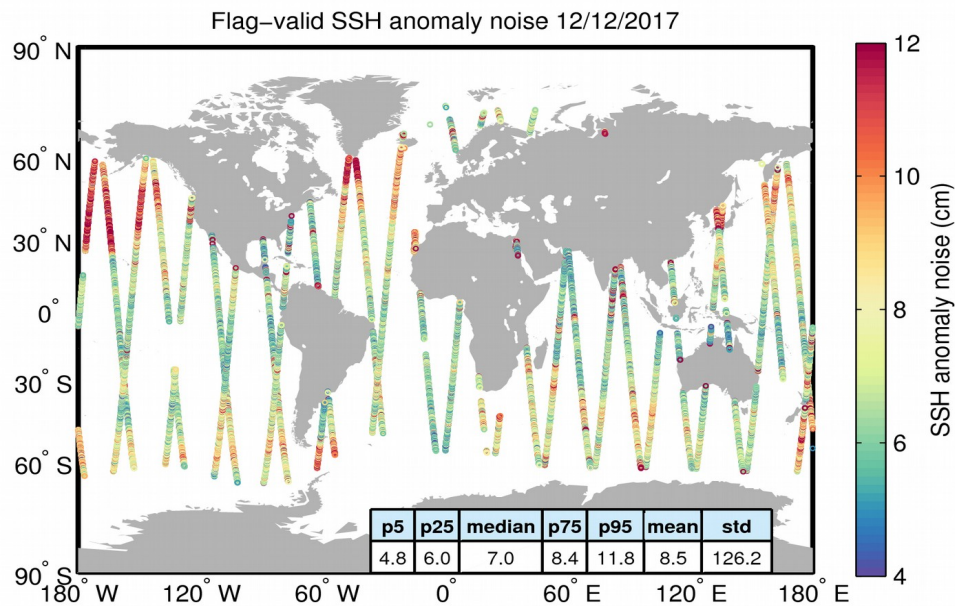
Figure 8. Geographical distribution of flag-valid 20-Hz SSH anomaly measurement noise over oceans and lakes for 12/12/2017. The statistical values shown in the table refer to the SSH anomaly noise and are calculated over all measurements shown in the figure.
