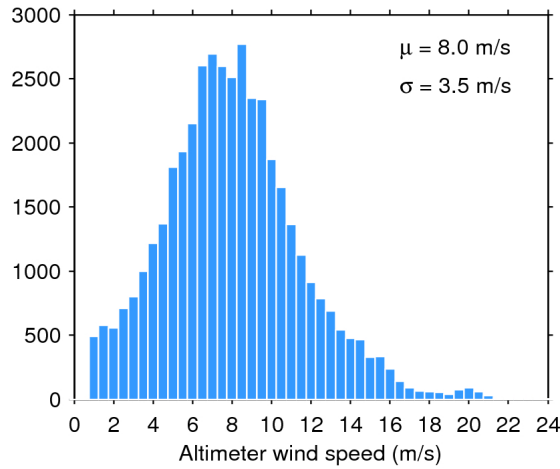
Figure 33. Histogram of flag-valid wind over oceans and lakes for 12/12/2017. The mean ( \mu ) and standard deviation ( \sigma ) are also shown. Note that values larger than 24 m/s are excluded from the histogram for the sake of readability but not from the computation of \mu and \sigma .
