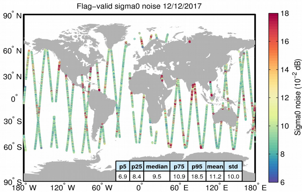
Figure 26. Geographical distribution of flag-valid 20-Hz sigma0 measurement noise over oceans and lakes for 12/12/2017. The statistical values shown in the table refer to the sigma0 noise and are calculated over all measurements shown in the figure.
