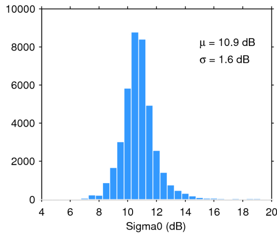
Figure 28. Histogram of science-valid sigma0 over oceans and lakes for 12/12/2017. The mean ( \mu ) and standard deviation ( \sigma ) are also shown. Note that values outside [4 20] dB are excluded from the histogram for the sake of readability but not from the computation of \mu and \sigma .
