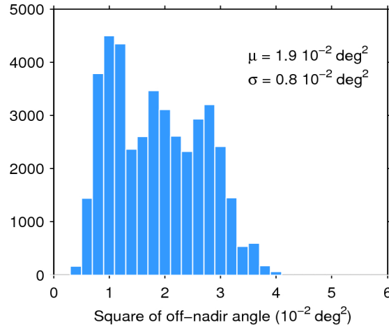
Figure 39. Histogram of flag-valid mispointing over oceans and lakes for 12/12/2017. The mean ( \mu ) and standard deviation ( \sigma ) are also shown. Note that values larger than 6 \cdot 10^{-2} \text{ deg}^2 are excluded from the histogram for the sake of readability but not from the computation of \mu and \sigma .
