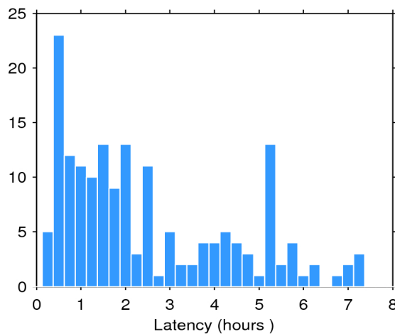
Figure 2. Histogram of the data latency for 12/12/2017. The y-axis denotes the number of files that are made available with a delay of x-hours with respect to the mean time of the records stored in the file.
