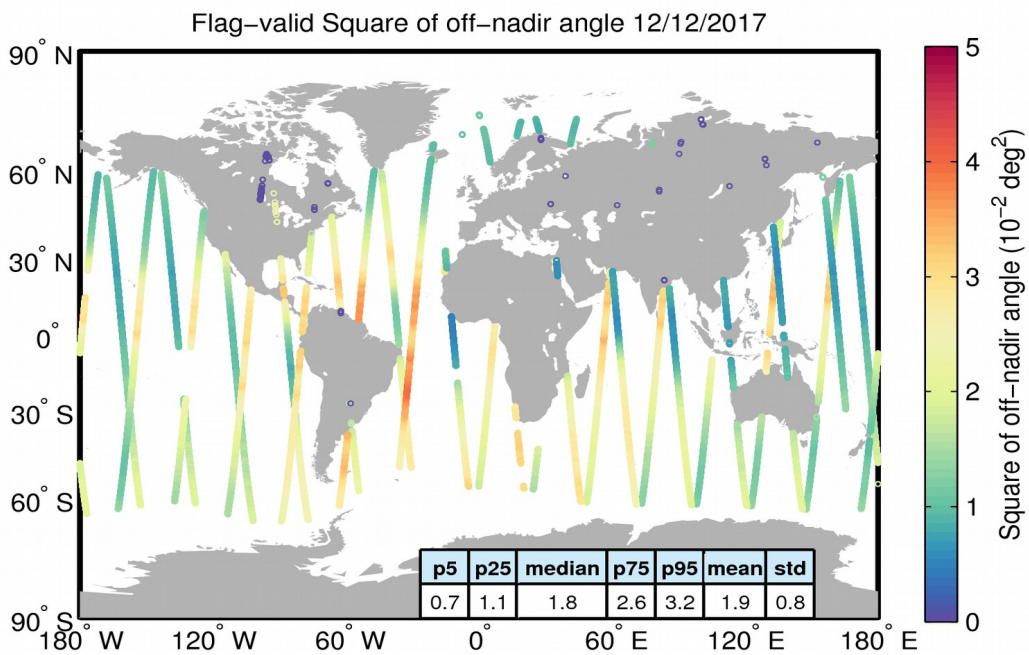
Figure 37. Geographical distribution of flag-valid mispointing data over oceans and lakes for 12/12/2017. The statistical values shown in the table refer to the mispointing in 10^{-2} deg 2 and are calculated over all measurements shown in the figure.
