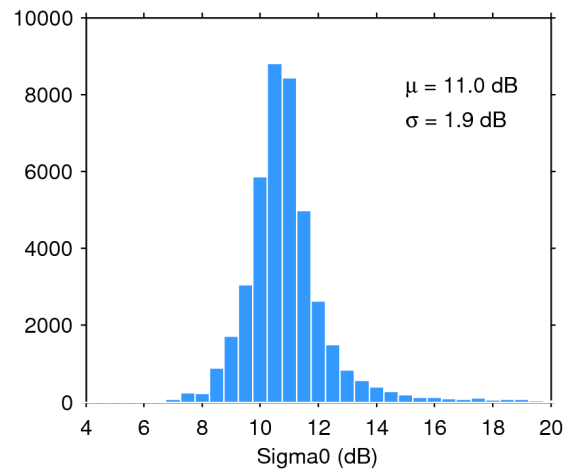
Figure 25. Histogram of flag-valid sigma0 over oceans and lakes for 12/12/2017. The mean ( \mu ) and standard deviation ( \sigma ) are also shown. Note that values outside [4 20] dB are excluded from the histogram for the sake of readability but not from the computation of \mu and \sigma .
