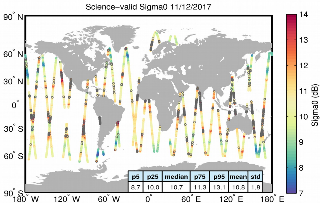
Figure 27. Geographical distribution of science-valid sigma0 data over oceans and lakes for 11/12/2017. The statistical values shown in the table refer to the sigma0 in dB and are calculated over all measurements shown in the figure. Gray circles denote records that have been rejected based on the editing criteria described in Table 4.
