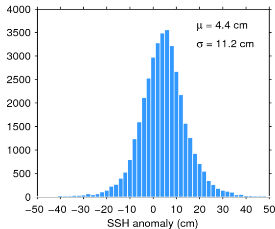
Figure 11. Histogram of science-valid SSH anomaly over oceans and lakes for 11/12/2017. The mean ( \mu ) and standard deviation ( \sigma ) are also shown. Note that values outside [-50 50] cm are excluded from the histogram for the sake of readability but not from the computation of \mu and \sigma .
