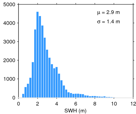
Figure 17. Histogram of flag-valid SWH over oceans and lakes for 11/12/2017. The mean ( \mu ) and standard deviation ( \sigma ) are also shown. Note that values larger than 12 m are excluded from the histogram for the sake of readability but not from the computation of \mu and \sigma .
