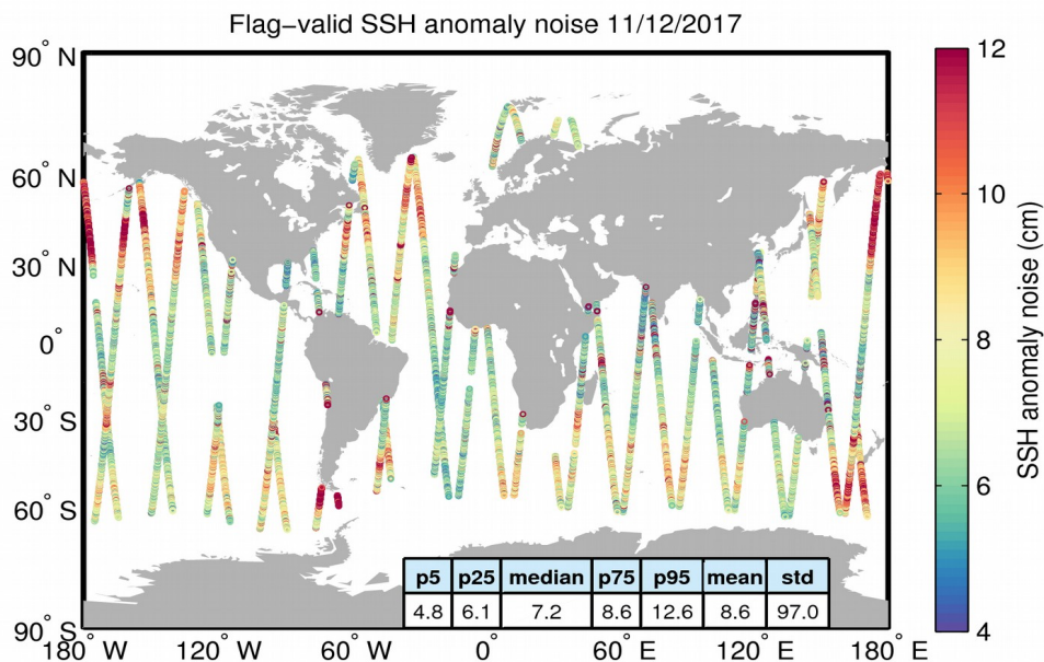
Figure 8. Geographical distribution of flag-valid 20-Hz SSH anomaly measurement noise over oceans and lakes for 11/12/2017. The statistical values shown in the table refer to the SSH anomaly noise and are calculated over all measurements shown in the figure.
