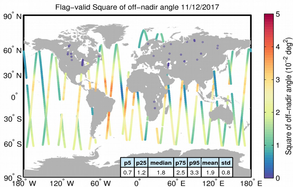
Figure 37. Geographical distribution of flag-valid mispointing data over oceans and lakes for 11/12/2017. The statistical values shown in the table refer to the mispointing in 10^{-2} deg 2 and are calculated over all measurements shown in the figure.
