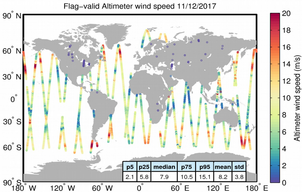
Figure 31. Geographical distribution of flag-valid wind data over oceans and lakes for 11/12/2017. The statistical values shown in the table refer to the wind in m/s and are calculated over all measurements shown in the figure.
