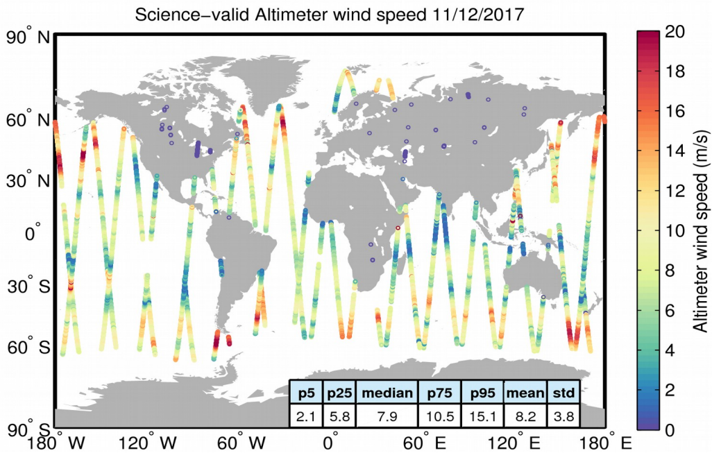
Figure 34. Geographical distribution of science-valid wind data over oceans and lakes for 11/12/2017. The statistical values shown in the table refer to the wind in m/s and are calculated over all measurements shown in the figure. Gray circles denote records that have been rejected based on the editing criteria described in Table 5.
