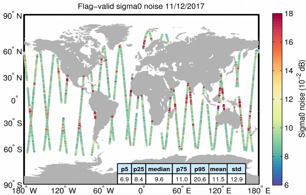
Figure 26. Geographical distribution of flag-valid 20-Hz sigma0 measurement noise over oceans and lakes for 11/12/2017. The statistical values shown in the table refer to the sigma0 noise and are calculated over all measurements shown in the figure.
