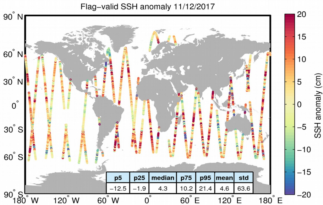
Figure 5. Geographical distribution of flag-valid 1-Hz SSH anomaly data over oceans and lakes for 11/12/2017. The statistical values shown in the table refer to the SSH anomaly in cm and are calculated over all measurements shown in the figure.
