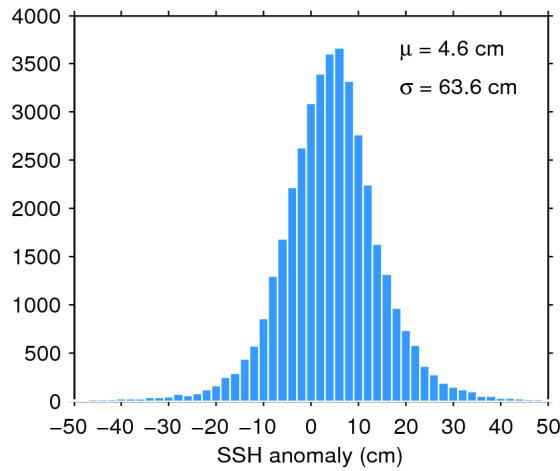
Figure 7. Histogram of flag-valid SSH anomaly over oceans and lakes for 11/12/2017. The mean ( \mu ) and standard deviation ( \sigma ) are also shown. Note that values outside [-50 50] cm are excluded from the histogram for the sake of readability but not from the computation of \mu and \sigma .
