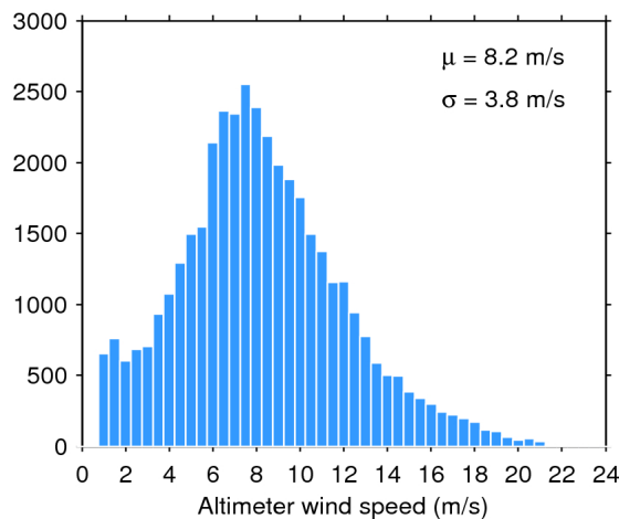
Figure 35. Histogram of science-valid wind over oceans and lakes for 11/12/2017. The mean ( \mu ) and standard deviation ( \sigma ) are also shown. Note that values larger than 24 m/s are excluded from the histogram for the sake of readability but not from the computation of \mu and \sigma .
