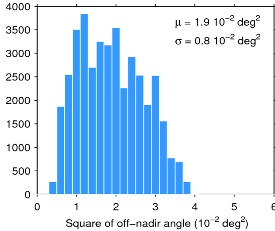
Figure 39. Histogram of flag-valid mispointing over oceans and lakes for 11/12/2017. The mean ( \mu ) and standard deviation ( \sigma ) are also shown. Note that values larger than 6 \cdot 10^{-2} \text{ deg}^2 are excluded from the histogram for the sake of readability but not from the computation of \mu and \sigma .
