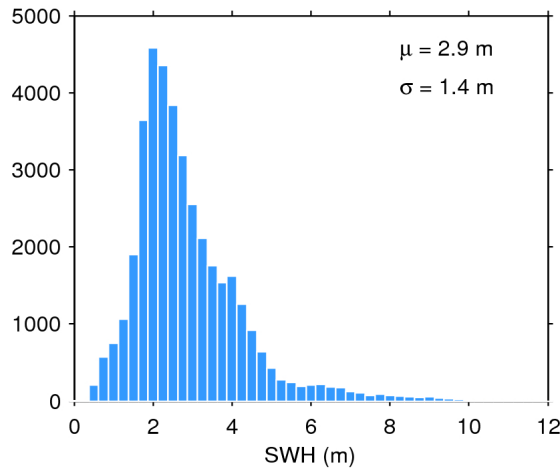
Figure 20. Histogram of science-valid SWH over oceans and lakes for 11/12/2017. The mean ( \mu ) and standard deviation ( \sigma ) are also shown. Note that values larger than 12 m are excluded from the histogram for the sake of readability but not from the computation of \mu and \sigma .
