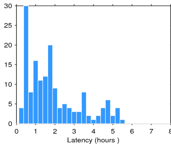
Figure 2. Histogram of the data latency for 11/12/2017. The y-axis denotes the number of files that are made available with a delay of x-hours with respect to the mean time of the records stored in the file.
