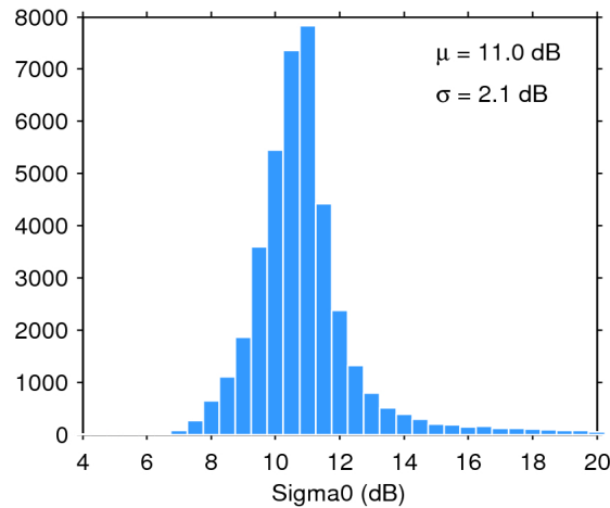
Figure 25. Histogram of flag-valid sigma0 over oceans and lakes for 11/12/2017. The mean ( \mu ) and standard deviation ( \sigma ) are also shown. Note that values outside [4 20] dB are excluded from the histogram for the sake of readability but not from the computation of \mu and \sigma .
