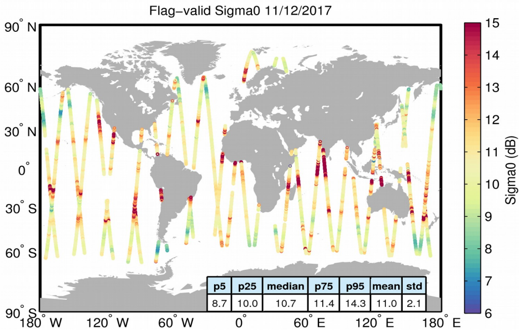
Figure 23. Geographical distribution of flag-valid sigma0 data over oceans and lakes for 11/12/2017. The statistical values shown in the table refer to the sigma0 in dB and are calculated over all measurements shown in the figure.
