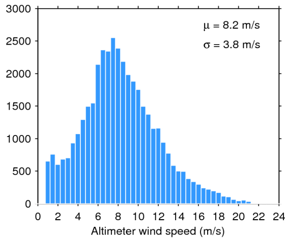
Figure 33. Histogram of flag-valid wind over oceans and lakes for 11/12/2017. The mean ( \mu ) and standard deviation ( \sigma ) are also shown. Note that values larger than 24 m/s are excluded from the histogram for the sake of readability but not from the computation of \mu and \sigma .
