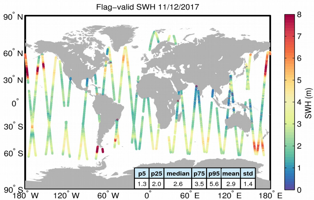
Figure 15. Geographical distribution of flag-valid SWH data over oceans and lakes for 11/12/2017. The statistical values shown in the table refer to the SWH in m and are calculated over all measurements shown in the figure.
