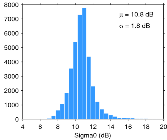
Figure 28. Histogram of science-valid sigma0 over oceans and lakes for 11/12/2017. The mean ( \mu ) and standard deviation ( \sigma ) are also shown. Note that values outside [4 20] dB are excluded from the histogram for the sake of readability but not from the computation of \mu and \sigma .
