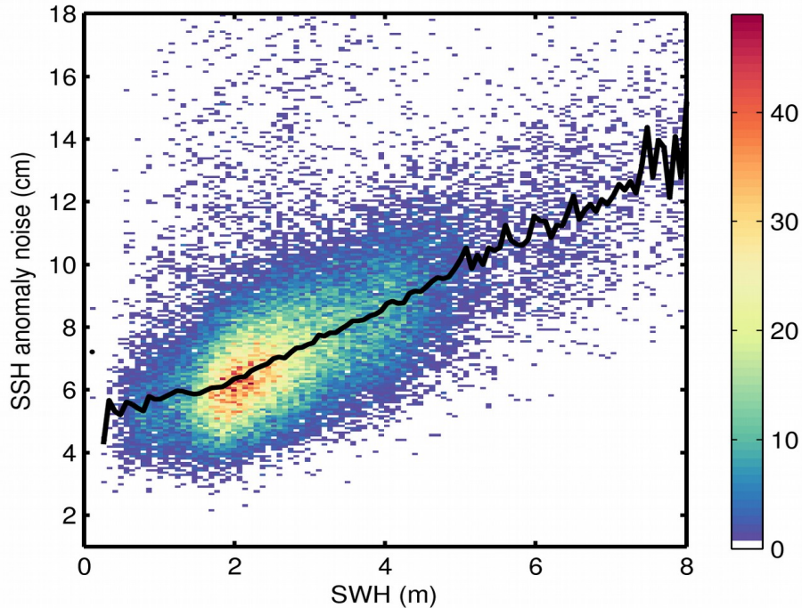
Figure 9. 2D histogram showing flag-valid SSH anomaly noise as a function of SWH for 11/12/2017. The black line denotes the median SSH anomaly noise as a function of SWH.
