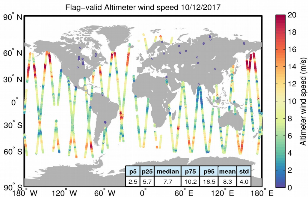
Figure 31. Geographical distribution of flag-valid wind data over oceans and lakes for 10/12/2017. The statistical values shown in the table refer to the wind in m/s and are calculated over all measurements shown in the figure.
