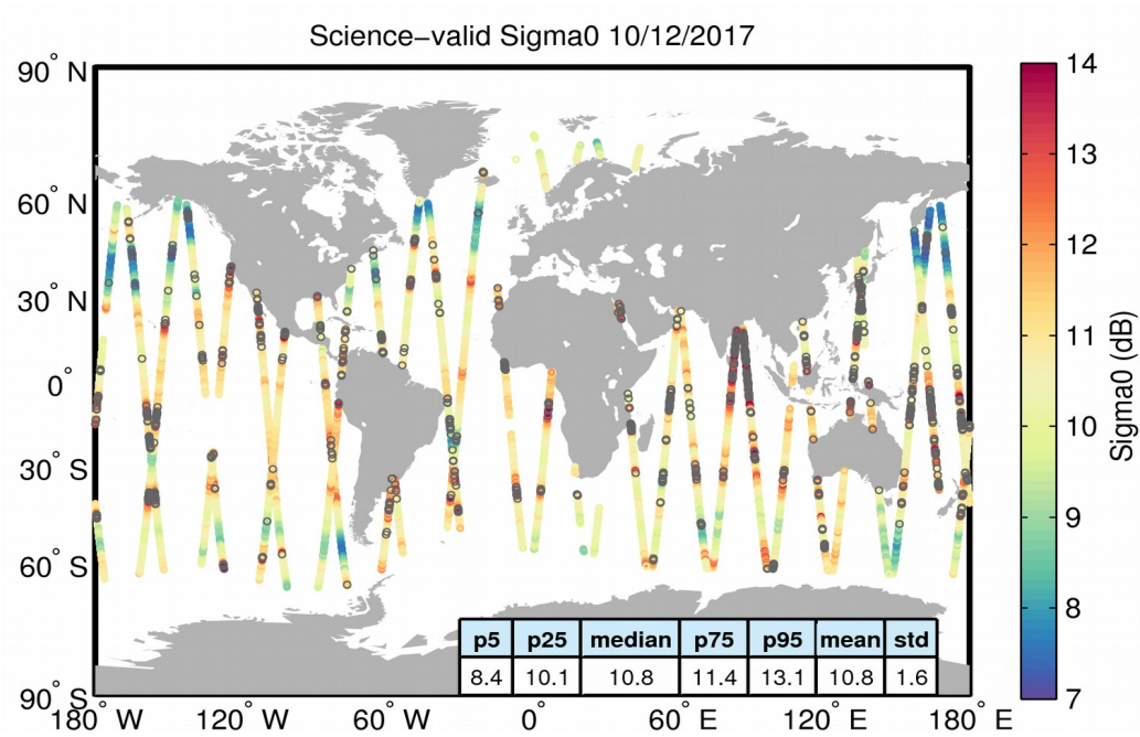
Figure 27. Geographical distribution of science-valid sigma0 data over oceans and lakes for 10/12/2017. The statistical values shown in the table refer to the sigma0 in dB and are calculated over all measurements shown in the figure. Gray circles denote records that have been rejected based on the editing criteria described in Table 4.
