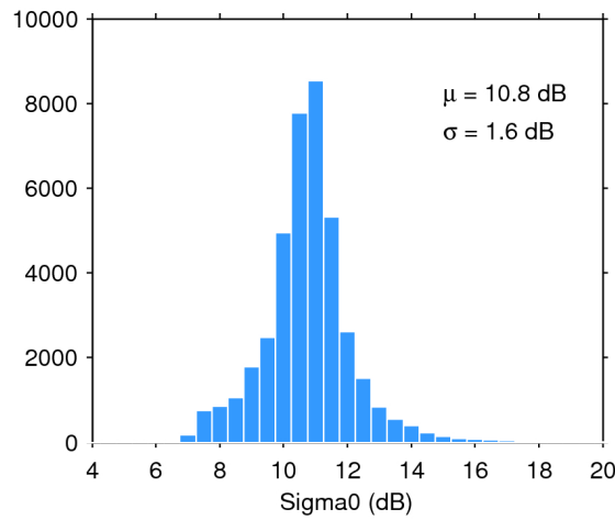
Figure 28. Histogram of science-valid sigma0 over oceans and lakes for 10/12/2017. The mean ( \mu ) and standard deviation ( \sigma ) are also shown. Note that values outside [4 20] dB are excluded from the histogram for the sake of readability but not from the computation of \mu and \sigma .
