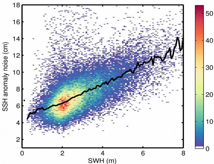
Figure 9. 2D histogram showing flag-valid SSH anomaly noise as a function of SWH for 10/12/2017. The black line denotes the median SSH anomaly noise as a function of SWH.
