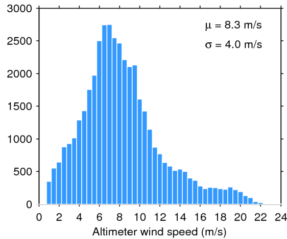
Figure 33. Histogram of flag-valid wind over oceans and lakes for 10/12/2017. The mean ( \mu ) and standard deviation ( \sigma ) are also shown. Note that values larger than 24 m/s are excluded from the histogram for the sake of readability but not from the computation of \mu and \sigma .
