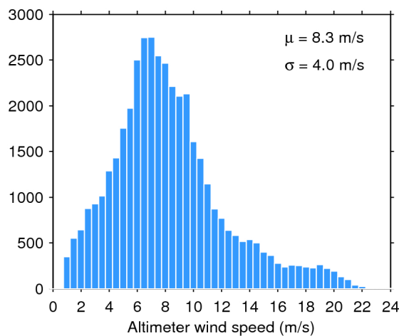
Figure 35. Histogram of science-valid wind over oceans and lakes for 10/12/2017. The mean ( \mu ) and standard deviation ( \sigma ) are also shown. Note that values larger than 24 m/s are excluded from the histogram for the sake of readability but not from the computation of \mu and \sigma .
