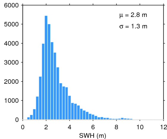
Figure 20. Histogram of science-valid SWH over oceans and lakes for 10/12/2017. The mean ( \mu ) and standard deviation ( \sigma ) are also shown. Note that values larger than 12 m are excluded from the histogram for the sake of readability but not from the computation of \mu and \sigma .
