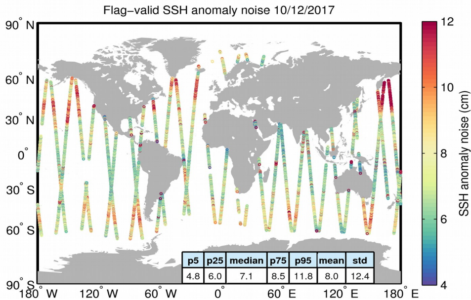
Figure 8. Geographical distribution of flag-valid 20-Hz SSH anomaly measurement noise over oceans and lakes for 10/12/2017. The statistical values shown in the table refer to the SSH anomaly noise and are calculated over all measurements shown in the figure.
