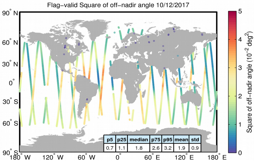
Figure 37. Geographical distribution of flag-valid mispointing data over oceans and lakes for 10/12/2017. The statistical values shown in the table refer to the mispointing in 10^{-2} deg 2 and are calculated over all measurements shown in the figure.
