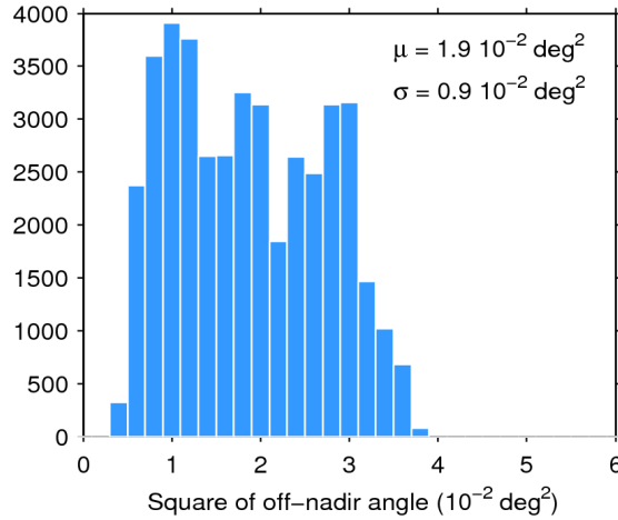
Figure 39. Histogram of flag-valid mispointing over oceans and lakes for 10/12/2017. The mean ( \mu ) and standard deviation ( \sigma ) are also shown. Note that values larger than 6 \cdot 10^{-2} \text{ deg}^2 are excluded from the histogram for the sake of readability but not from the computation of \mu and \sigma .
