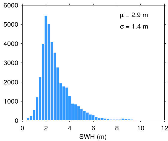
Figure 17. Histogram of flag-valid SWH over oceans and lakes for 10/12/2017. The mean ( \mu ) and standard deviation ( \sigma ) are also shown. Note that values larger than 12 m are excluded from the histogram for the sake of readability but not from the computation of \mu and \sigma .
