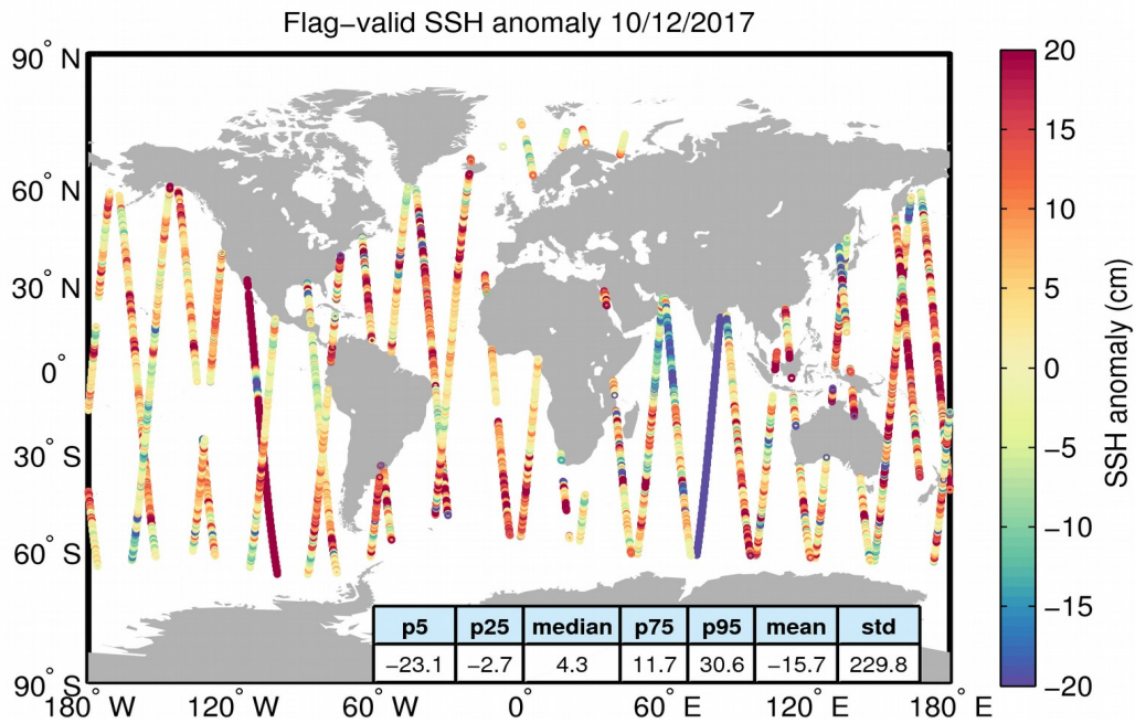
Figure 5. Geographical distribution of flag-valid 1-Hz SSH anomaly data over oceans and lakes for 10/12/2017. The statistical values shown in the table refer to the SSH anomaly in cm and are calculated over all measurements shown in the figure.
