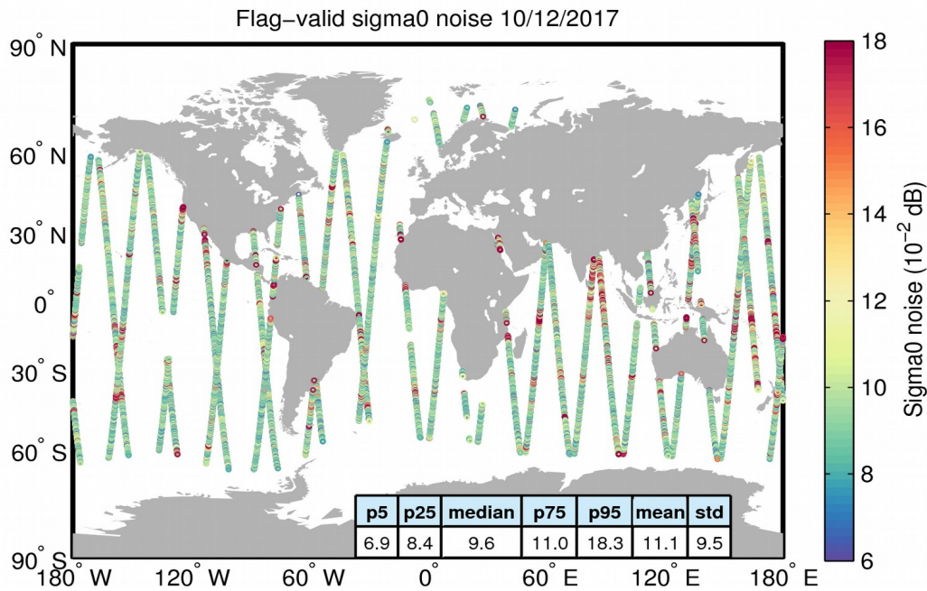
Figure 26. Geographical distribution of flag-valid 20-Hz sigma0 measurement noise over oceans and lakes for 10/12/2017. The statistical values shown in the table refer to the sigma0 noise and are calculated over all measurements shown in the figure.
