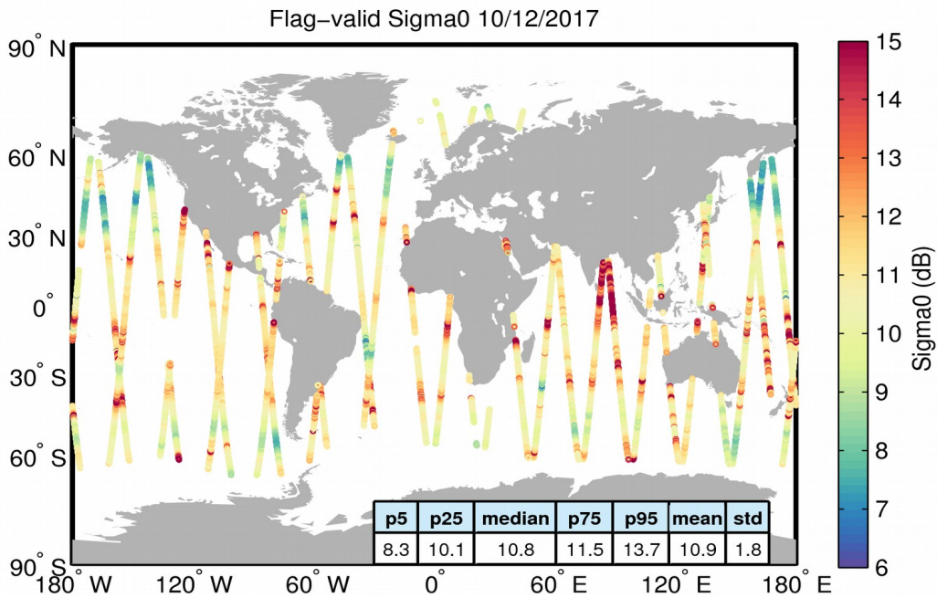
Figure 23. Geographical distribution of flag-valid sigma0 data over oceans and lakes for 10/12/2017. The statistical values shown in the table refer to the sigma0 in dB and are calculated over all measurements shown in the figure.
