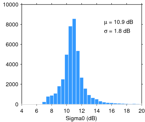
Figure 25. Histogram of flag-valid sigma0 over oceans and lakes for 10/12/2017. The mean ( \mu ) and standard deviation ( \sigma ) are also shown. Note that values outside [4 20] dB are excluded from the histogram for the sake of readability but not from the computation of \mu and \sigma .
