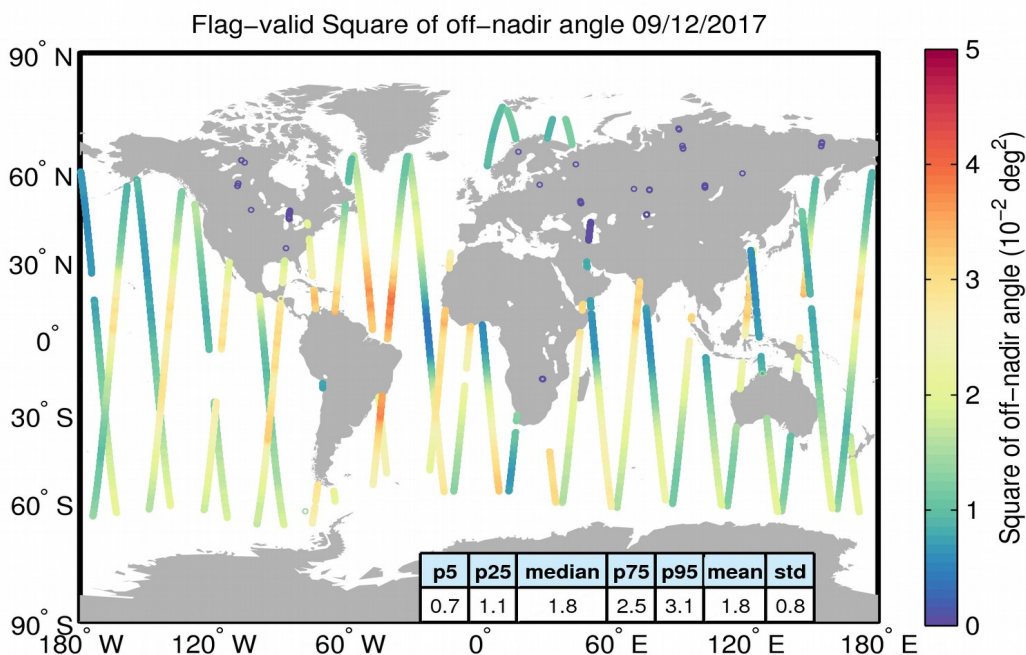
Figure 37. Geographical distribution of flag-valid mispointing data over oceans and lakes for 09/12/2017. The statistical values shown in the table refer to the mispointing in 10^{-2} deg 2 and are calculated over all measurements shown in the figure.
