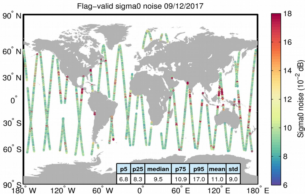
Figure 26. Geographical distribution of flag-valid 20-Hz sigma0 measurement noise over oceans and lakes for 09/12/2017. The statistical values shown in the table refer to the sigma0 noise and are calculated over all measurements shown in the figure.
