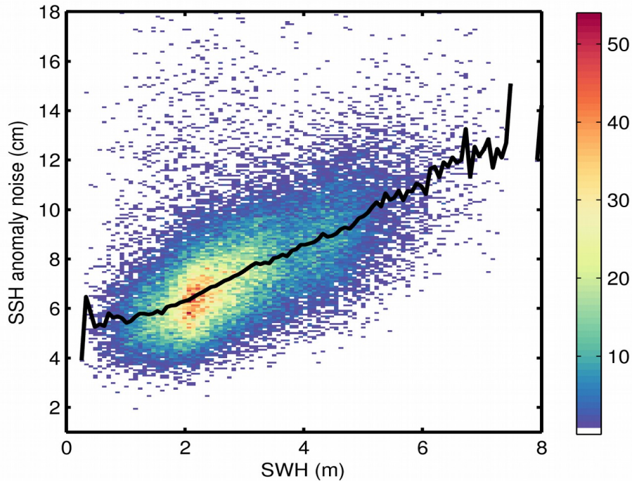
Figure 9. 2D histogram showing flag-valid SSH anomaly noise as a function of SWH for 09/12/2017. The black line denotes the median SSH anomaly noise as a function of SWH.
