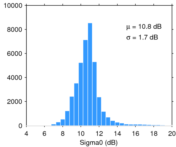
Figure 25. Histogram of flag-valid sigma0 over oceans and lakes for 09/12/2017. The mean ( \mu ) and standard deviation ( \sigma ) are also shown. Note that values outside [4 20] dB are excluded from the histogram for the sake of readability but not from the computation of \mu and \sigma .
