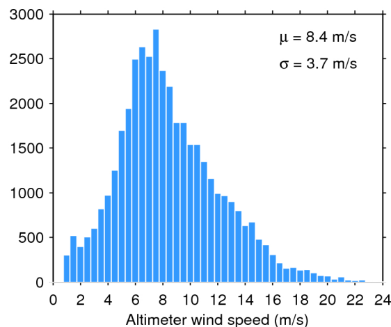
Figure 35. Histogram of science-valid wind over oceans and lakes for 09/12/2017. The mean ( \mu ) and standard deviation ( \sigma ) are also shown. Note that values larger than 24 m/s are excluded from the histogram for the sake of readability but not from the computation of \mu and \sigma .
