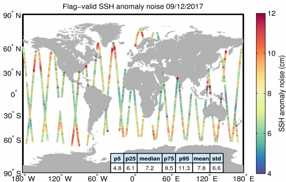
Figure 8. Geographical distribution of flag-valid 20-Hz SSH anomaly measurement noise over oceans and lakes for 09/12/2017. The statistical values shown in the table refer to the SSH anomaly noise and are calculated over all measurements shown in the figure.
