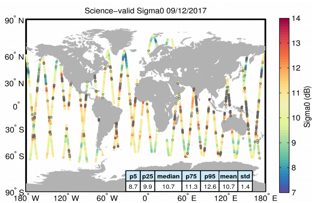
Figure 27. Geographical distribution of science-valid sigma0 data over oceans and lakes for 09/12/2017. The statistical values shown in the table refer to the sigma0 in dB and are calculated over all measurements shown in the figure. Gray circles denote records that have been rejected based on the editing criteria described in Table 4.
