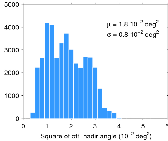
Figure 39. Histogram of flag-valid mispointing over oceans and lakes for 09/12/2017. The mean ( \mu ) and standard deviation ( \sigma ) are also shown. Note that values larger than 6 \cdot 10^{-2} \text{ deg}^2 are excluded from the histogram for the sake of readability but not from the computation of \mu and \sigma .
