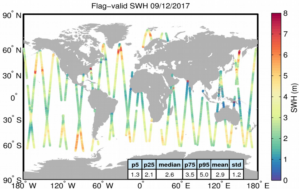
Figure 15. Geographical distribution of flag-valid SWH data over oceans and lakes for 09/12/2017. The statistical values shown in the table refer to the SWH in m and are calculated over all measurements shown in the figure.
