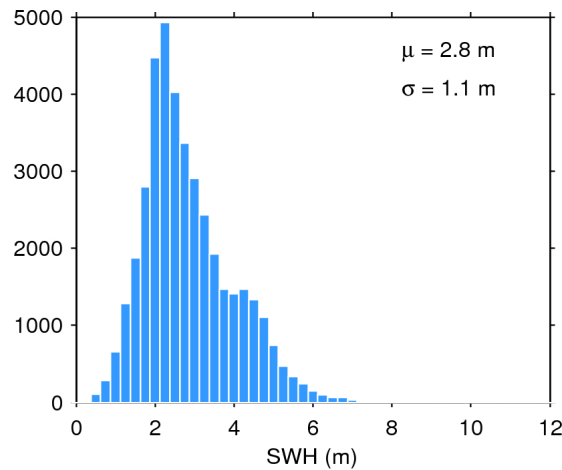
Figure 20. Histogram of science-valid SWH over oceans and lakes for 09/12/2017. The mean ( \mu ) and standard deviation ( \sigma ) are also shown. Note that values larger than 12 m are excluded from the histogram for the sake of readability but not from the computation of \mu and \sigma .
