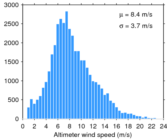
Figure 33. Histogram of flag-valid wind over oceans and lakes for 09/12/2017. The mean ( \mu ) and standard deviation ( \sigma ) are also shown. Note that values larger than 24 m/s are excluded from the histogram for the sake of readability but not from the computation of \mu and \sigma .
