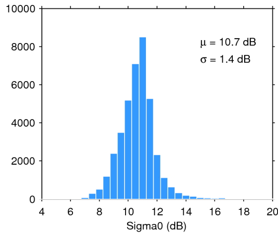
Figure 28. Histogram of science-valid sigma0 over oceans and lakes for 09/12/2017. The mean ( \mu ) and standard deviation ( \sigma ) are also shown. Note that values outside [4 20] dB are excluded from the histogram for the sake of readability but not from the computation of \mu and \sigma .
