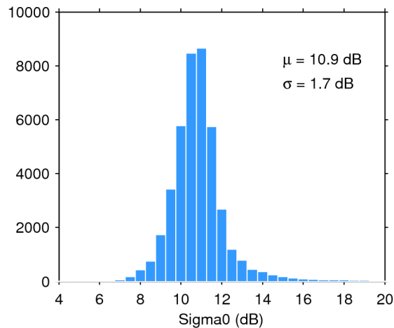
Figure 25. Histogram of flag-valid sigma0 over oceans and lakes for 08/12/2017. The mean ( \mu ) and standard deviation ( \sigma ) are also shown. Note that values outside [4 20] dB are excluded from the histogram for the sake of readability but not from the computation of \mu and \sigma .
