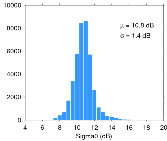
Figure 28. Histogram of science-valid sigma0 over oceans and lakes for 08/12/2017. The mean ( \mu ) and standard deviation ( \sigma ) are also shown. Note that values outside [4 20] dB are excluded from the histogram for the sake of readability but not from the computation of \mu and \sigma .
