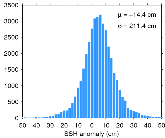
Figure 7. Histogram of flag-valid SSH anomaly over oceans and lakes for 08/12/2017. The mean ( \mu ) and standard deviation ( \sigma ) are also shown. Note that values outside [-50 50] cm are excluded from the histogram for the sake of readability but not from the computation of \mu and \sigma .
