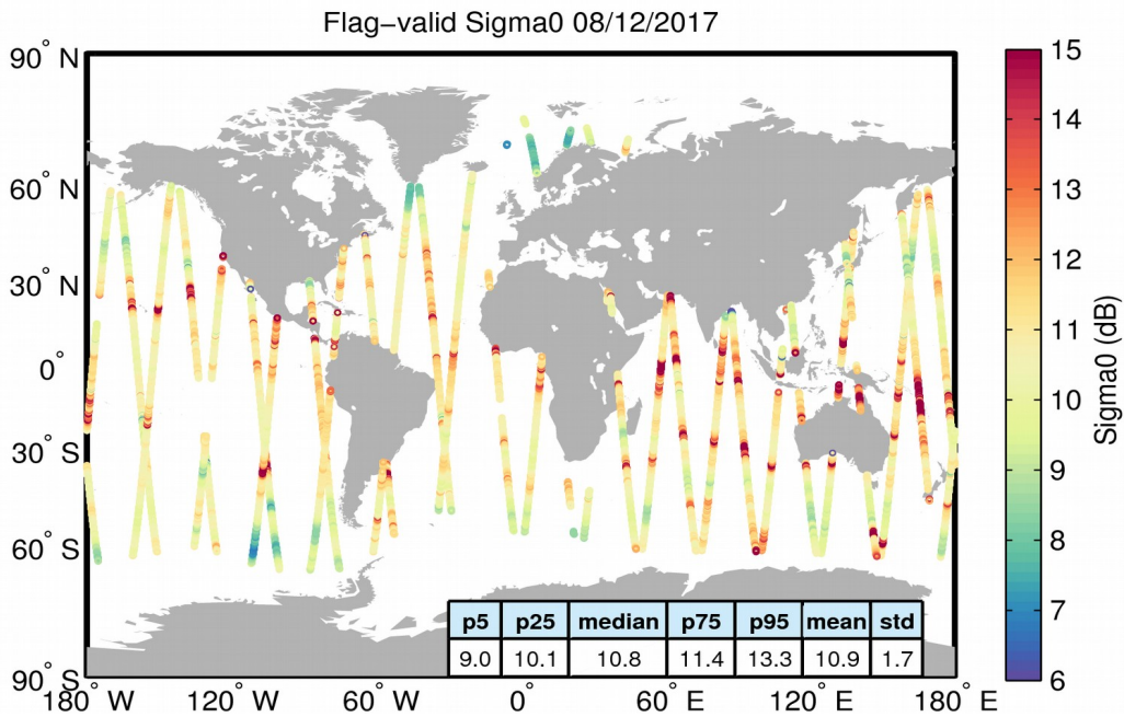
Figure 23. Geographical distribution of flag-valid sigma0 data over oceans and lakes for 08/12/2017. The statistical values shown in the table refer to the sigma0 in dB and are calculated over all measurements shown in the figure.
