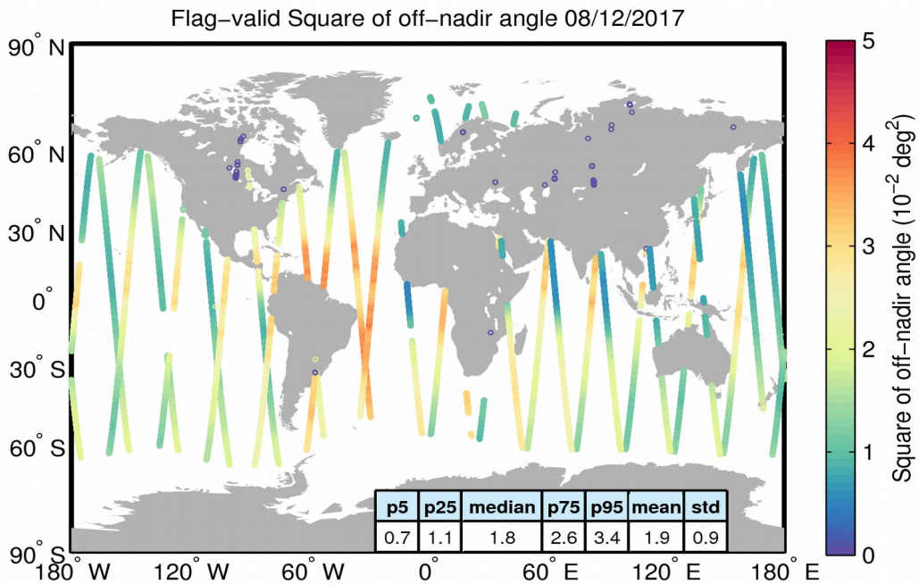
Figure 37. Geographical distribution of flag-valid mispointing data over oceans and lakes for 08/12/2017. The statistical values shown in the table refer to the mispointing in 10^{-2} deg 2 and are calculated over all measurements shown in the figure.
