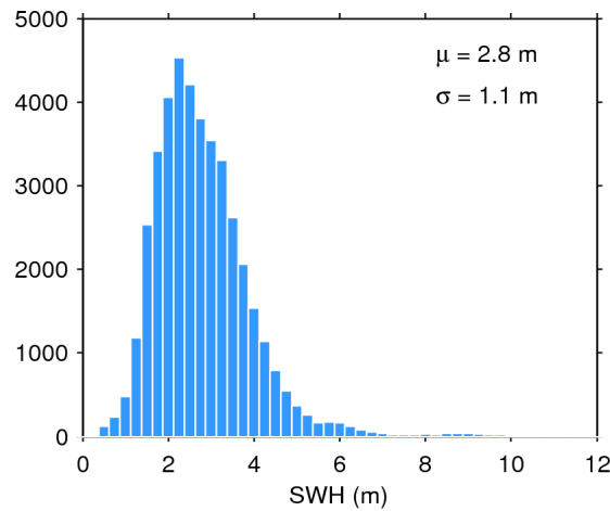
Figure 17. Histogram of flag-valid SWH over oceans and lakes for 08/12/2017. The mean ( \mu ) and standard deviation ( \sigma ) are also shown. Note that values larger than 12 m are excluded from the histogram for the sake of readability but not from the computation of \mu and \sigma .
