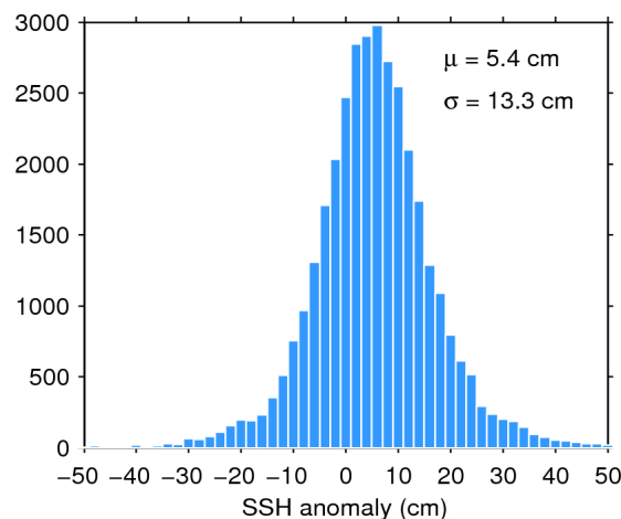
Figure 11. Histogram of science-valid SSH anomaly over oceans and lakes for 08/12/2017. The mean ( \mu ) and standard deviation ( \sigma ) are also shown. Note that values outside [-50 50] cm are excluded from the histogram for the sake of readability but not from the computation of \mu and \sigma .
