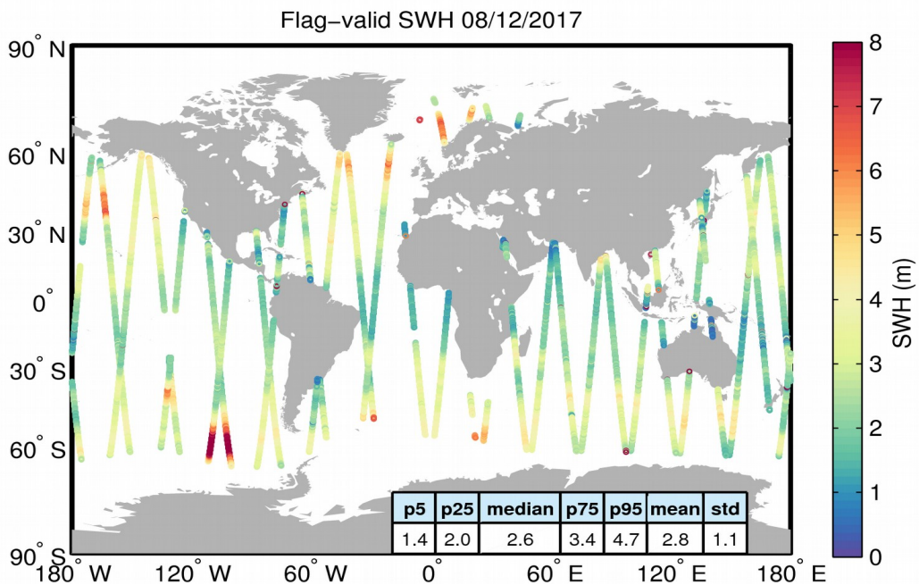
Figure 15. Geographical distribution of flag-valid SWH data over oceans and lakes for 08/12/2017. The statistical values shown in the table refer to the SWH in m and are calculated over all measurements shown in the figure.
