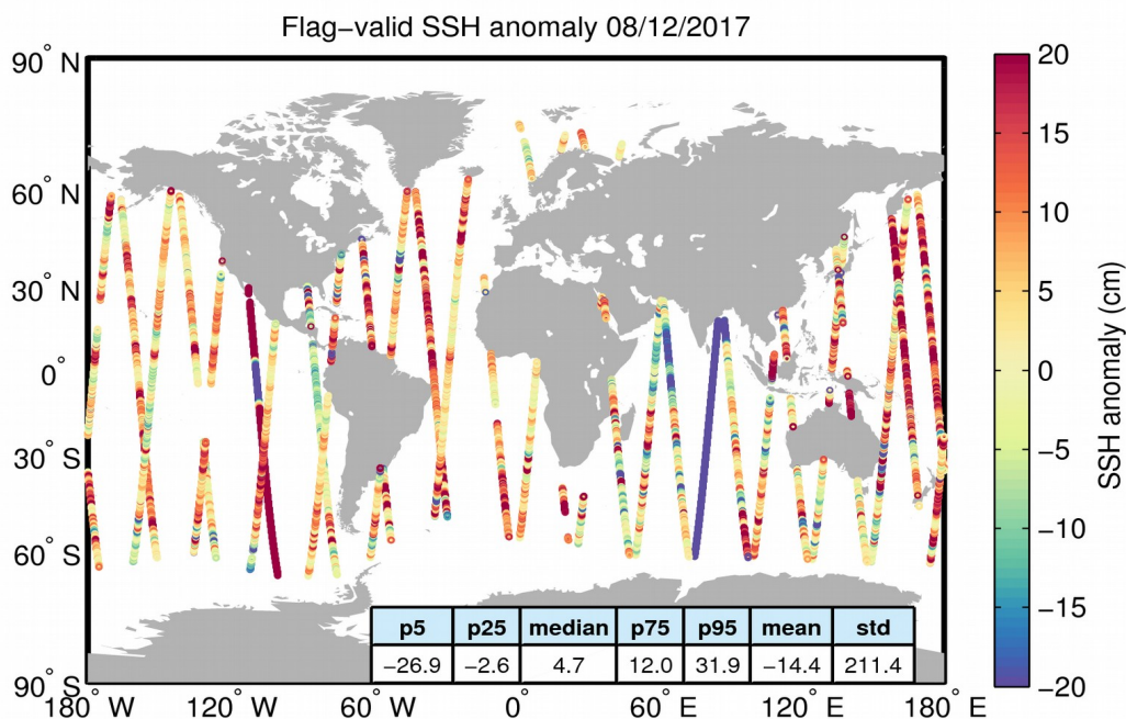
Figure 5. Geographical distribution of flag-valid 1-Hz SSH anomaly data over oceans and lakes for 08/12/2017. The statistical values shown in the table refer to the SSH anomaly in cm and are calculated over all measurements shown in the figure.
