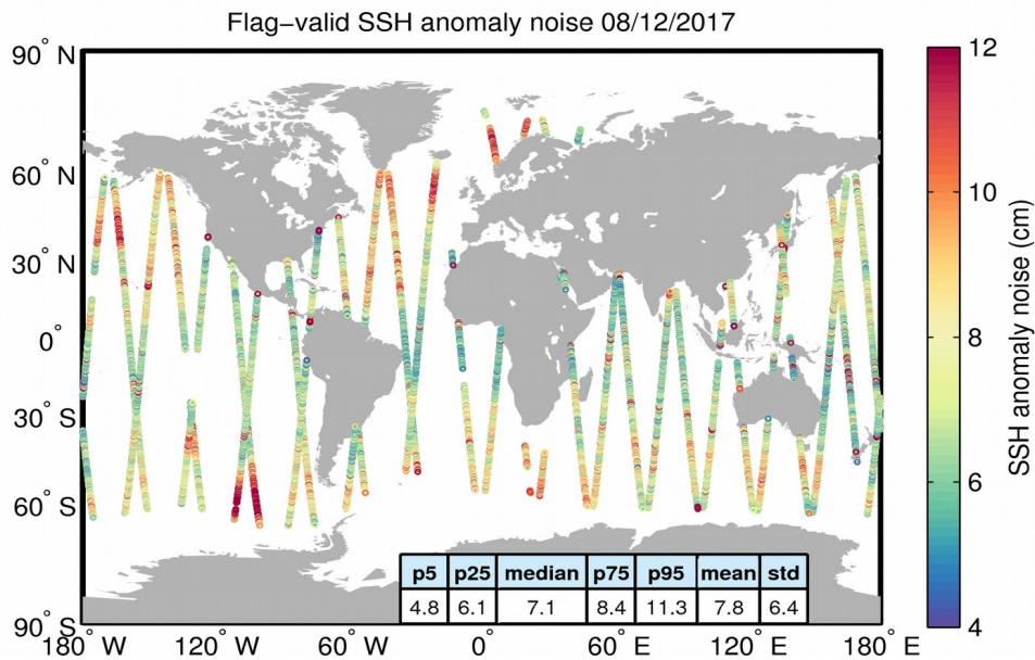
Figure 8. Geographical distribution of flag-valid 20-Hz SSH anomaly measurement noise over oceans and lakes for 08/12/2017. The statistical values shown in the table refer to the SSH anomaly noise and are calculated over all measurements shown in the figure.
