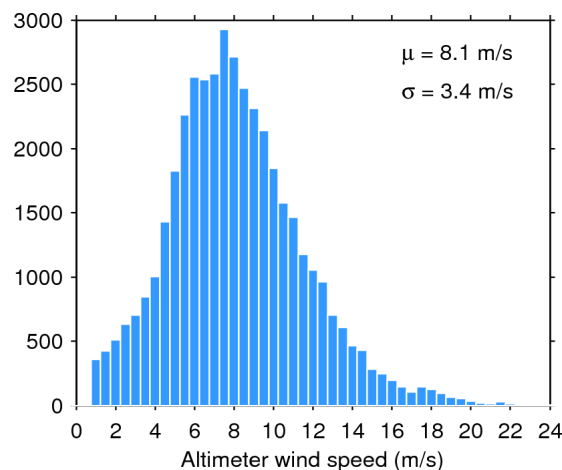
Figure 35. Histogram of science-valid wind over oceans and lakes for 08/12/2017. The mean ( \mu ) and standard deviation ( \sigma ) are also shown. Note that values larger than 24 m/s are excluded from the histogram for the sake of readability but not from the computation of \mu and \sigma .
