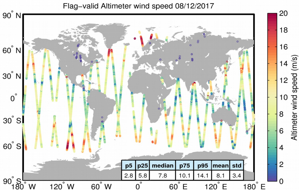
Figure 31. Geographical distribution of flag-valid wind data over oceans and lakes for 08/12/2017. The statistical values shown in the table refer to the wind in m/s and are calculated over all measurements shown in the figure.
