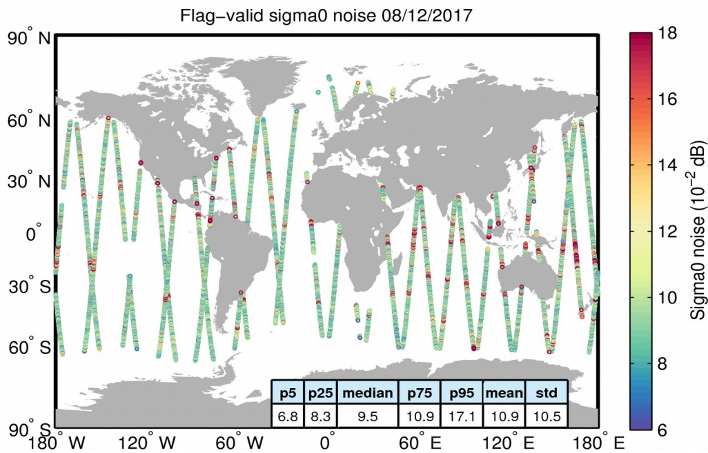
Figure 26. Geographical distribution of flag-valid 20-Hz sigma0 measurement noise over oceans and lakes for 08/12/2017. The statistical values shown in the table refer to the sigma0 noise and are calculated over all measurements shown in the figure.
