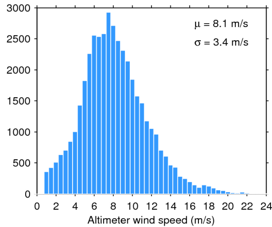
Figure 33. Histogram of flag-valid wind over oceans and lakes for 08/12/2017. The mean ( \mu ) and standard deviation ( \sigma ) are also shown. Note that values larger than 24 m/s are excluded from the histogram for the sake of readability but not from the computation of \mu and \sigma .
