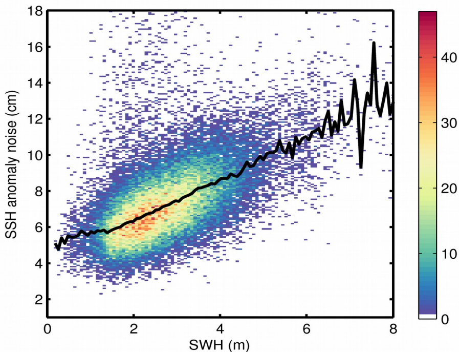
Figure 9. 2D histogram showing flag-valid SSH anomaly noise as a function of SWH for 08/12/2017. The black line denotes the median SSH anomaly noise as a function of SWH.
