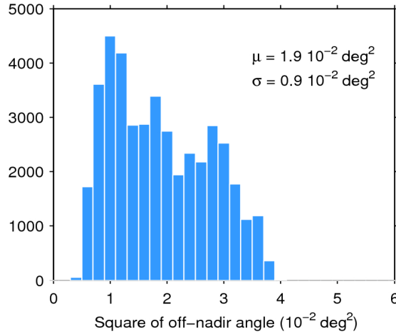
Figure 39. Histogram of flag-valid mispointing over oceans and lakes for 08/12/2017. The mean ( \mu ) and standard deviation ( \sigma ) are also shown. Note that values larger than 6 \cdot 10^{-2} \text{ deg}^2 are excluded from the histogram for the sake of readability but not from the computation of \mu and \sigma .
