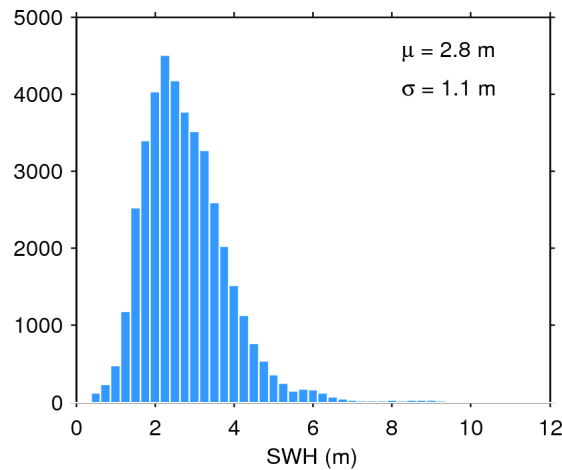
Figure 20. Histogram of science-valid SWH over oceans and lakes for 08/12/2017. The mean ( \mu ) and standard deviation ( \sigma ) are also shown. Note that values larger than 12 m are excluded from the histogram for the sake of readability but not from the computation of \mu and \sigma .
