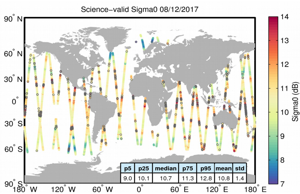
Figure 27. Geographical distribution of science-valid sigma0 data over oceans and lakes for 08/12/2017. The statistical values shown in the table refer to the sigma0 in dB and are calculated over all measurements shown in the figure. Gray circles denote records that have been rejected based on the editing criteria described in Table 4.
