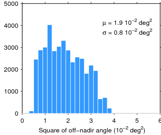
Figure 39. Histogram of flag-valid mispointing over oceans and lakes for 07/12/2017. The mean ( \mu ) and standard deviation ( \sigma ) are also shown. Note that values larger than 6 \cdot 10^{-2} \text{ deg}^2 are excluded from the histogram for the sake of readability but not from the computation of \mu and \sigma .
