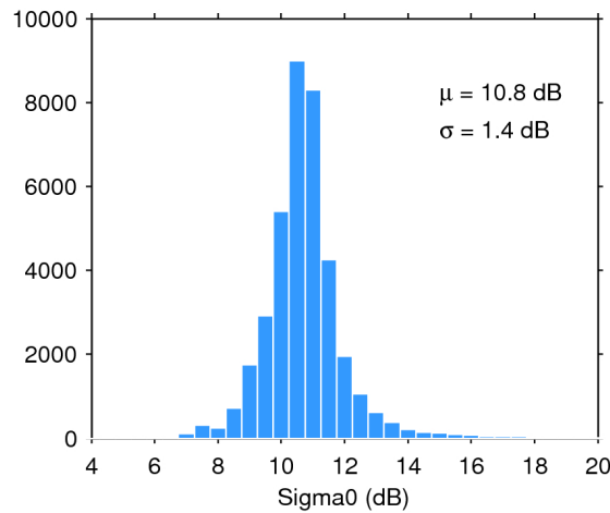
Figure 28. Histogram of science-valid sigma0 over oceans and lakes for 07/12/2017. The mean ( \mu ) and standard deviation ( \sigma ) are also shown. Note that values outside [4 20] dB are excluded from the histogram for the sake of readability but not from the computation of \mu and \sigma .
