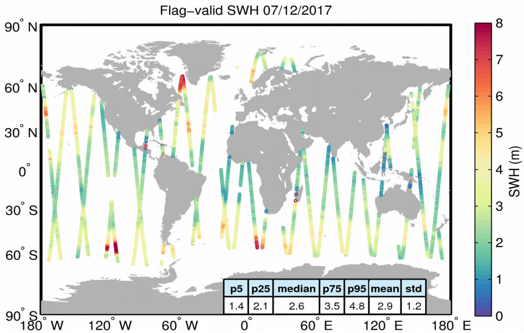
Figure 15. Geographical distribution of flag-valid SWH data over oceans and lakes for 07/12/2017. The statistical values shown in the table refer to the SWH in m and are calculated over all measurements shown in the figure.
