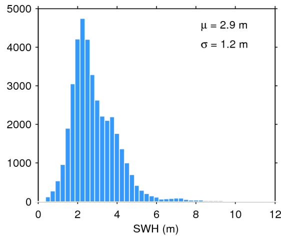
Figure 17. Histogram of flag-valid SWH over oceans and lakes for 07/12/2017. The mean ( \mu ) and standard deviation ( \sigma ) are also shown. Note that values larger than 12 m are excluded from the histogram for the sake of readability but not from the computation of \mu and \sigma .
