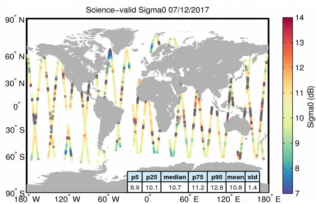
Figure 27. Geographical distribution of science-valid sigma0 data over oceans and lakes for 07/12/2017. The statistical values shown in the table refer to the sigma0 in dB and are calculated over all measurements shown in the figure. Gray circles denote records that have been rejected based on the editing criteria described in Table 4.
