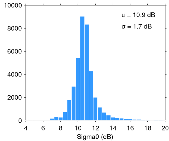
Figure 25. Histogram of flag-valid sigma0 over oceans and lakes for 07/12/2017. The mean ( \mu ) and standard deviation ( \sigma ) are also shown. Note that values outside [4 20] dB are excluded from the histogram for the sake of readability but not from the computation of \mu and \sigma .
