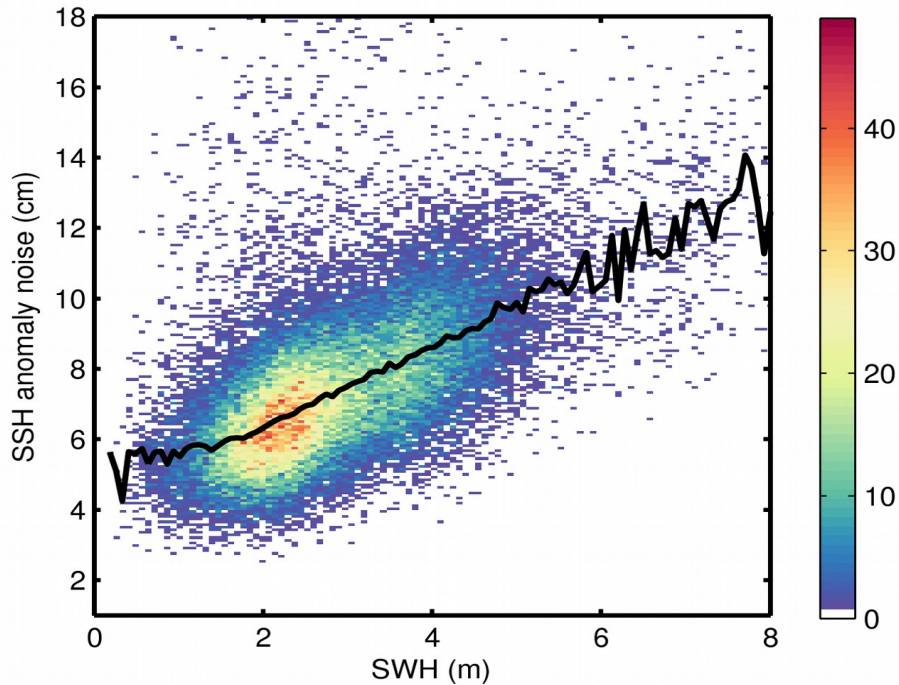
Figure 9. 2D histogram showing flag-valid SSH anomaly noise as a function of SWH for 07/12/2017. The black line denotes the median SSH anomaly noise as a function of SWH.
