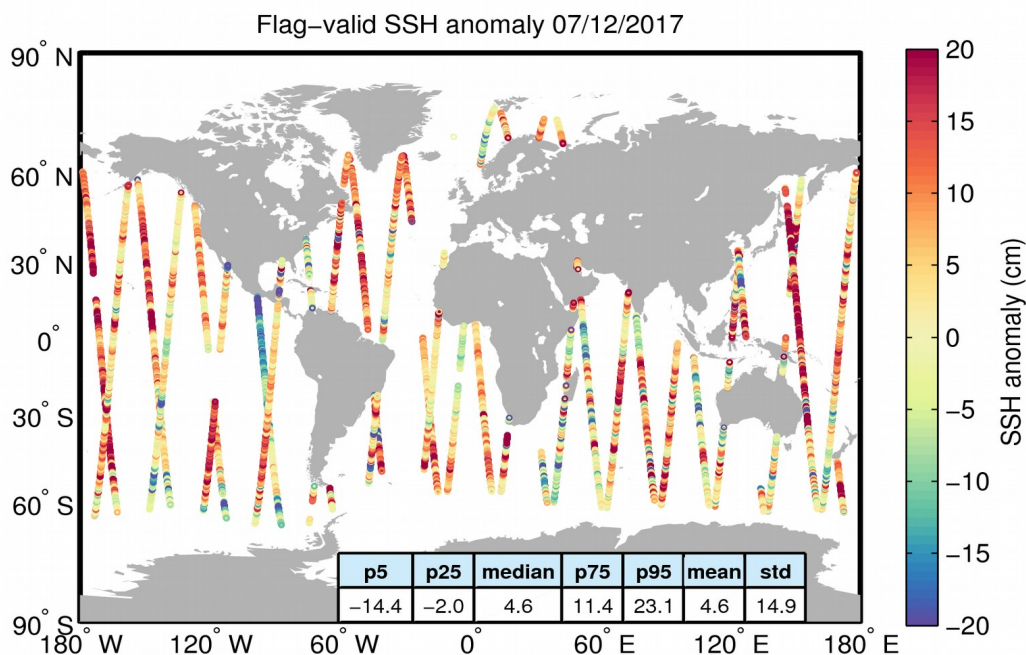
Figure 5. Geographical distribution of flag-valid 1-Hz SSH anomaly data over oceans and lakes for 07/12/2017. The statistical values shown in the table refer to the SSH anomaly in cm and are calculated over all measurements shown in the figure.
