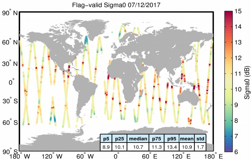
Figure 23. Geographical distribution of flag-valid sigma0 data over oceans and lakes for 07/12/2017. The statistical values shown in the table refer to the sigma0 in dB and are calculated over all measurements shown in the figure.
