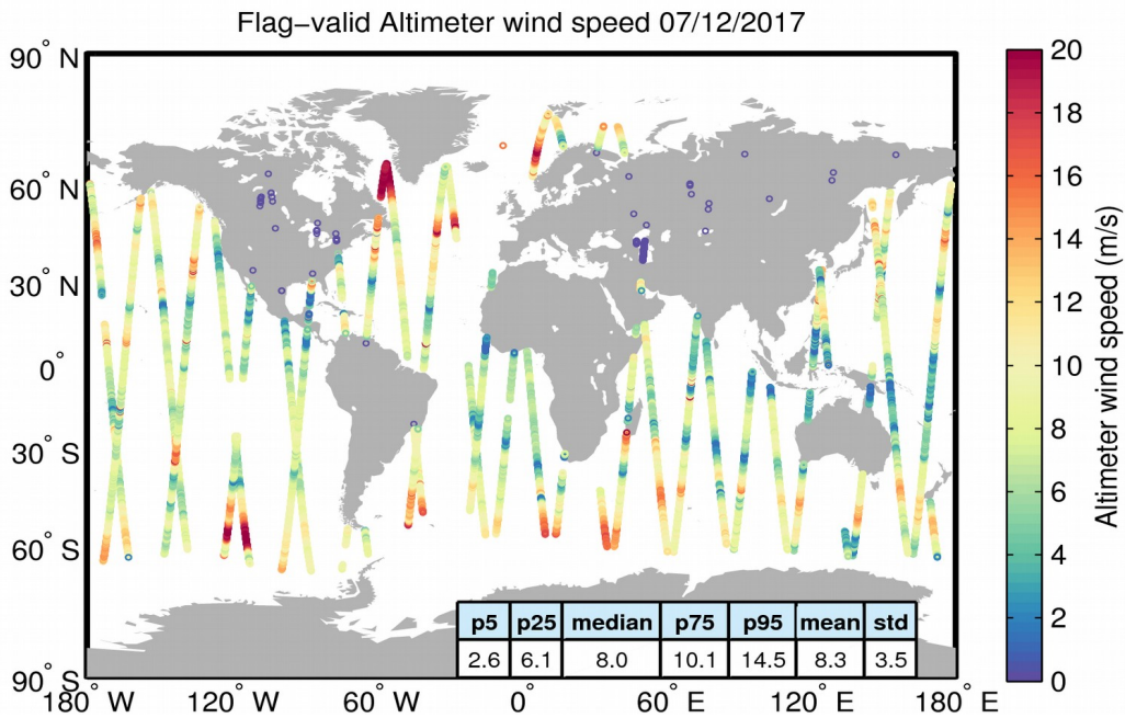
Figure 31. Geographical distribution of flag-valid wind data over oceans and lakes for 07/12/2017. The statistical values shown in the table refer to the wind in m/s and are calculated over all measurements shown in the figure.
