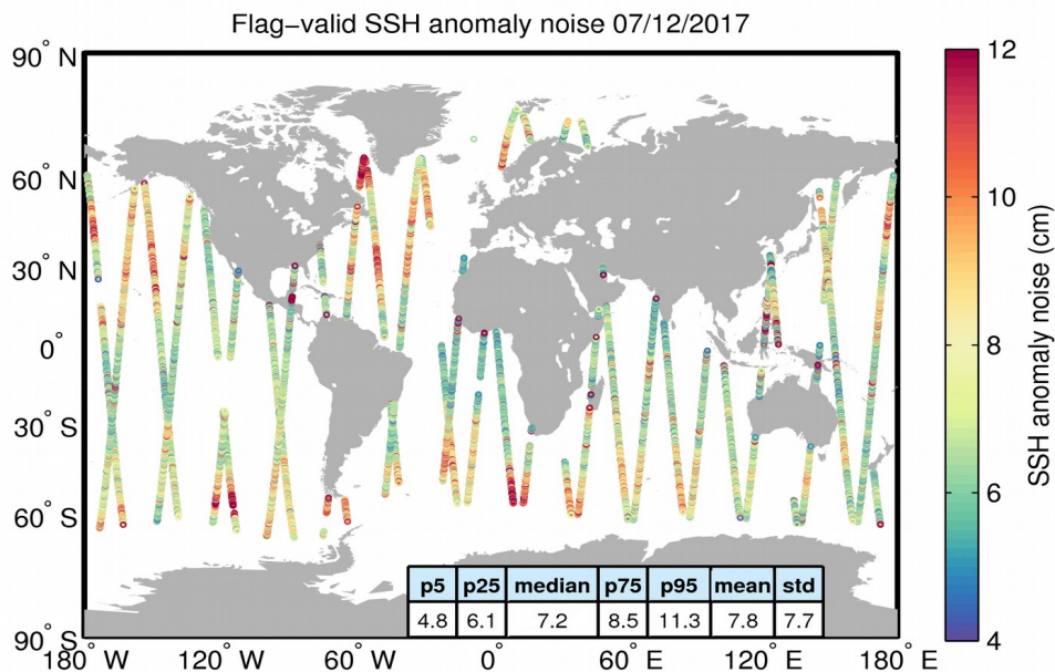
Figure 8. Geographical distribution of flag-valid 20-Hz SSH anomaly measurement noise over oceans and lakes for 07/12/2017. The statistical values shown in the table refer to the SSH anomaly noise and are calculated over all measurements shown in the figure.
