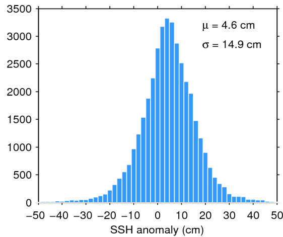
Figure 7. Histogram of flag-valid SSH anomaly over oceans and lakes for 07/12/2017. The mean ( \mu ) and standard deviation ( \sigma ) are also shown. Note that values outside [-50\ 50] cm are excluded from the histogram for the sake of readability but not from the computation of \mu and \sigma .
