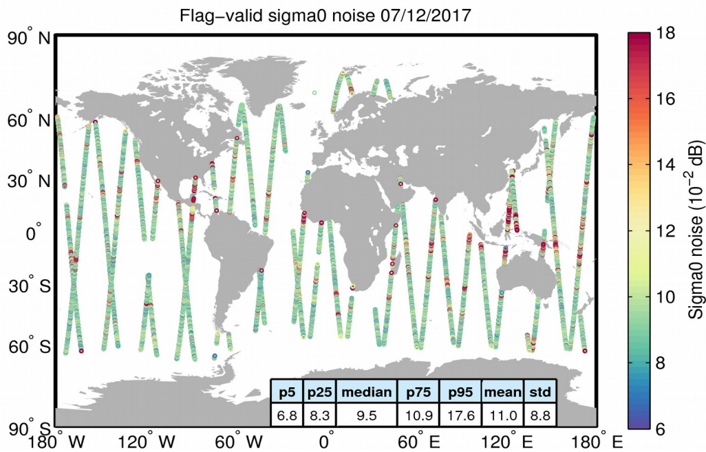
Figure 26. Geographical distribution of flag-valid 20-Hz sigma0 measurement noise over oceans and lakes for 07/12/2017. The statistical values shown in the table refer to the sigma0 noise and are calculated over all measurements shown in the figure.
