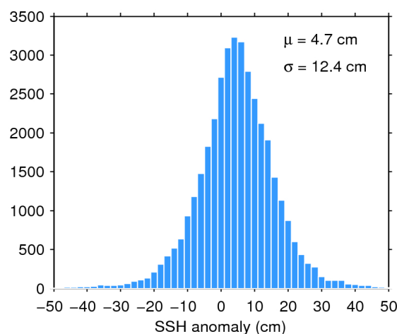
Figure 11. Histogram of science-valid SSH anomaly over oceans and lakes for 07/12/2017. The mean ( \mu ) and standard deviation ( \sigma ) are also shown. Note that values outside [-50 50] cm are excluded from the histogram for the sake of readability but not from the computation of \mu and \sigma .
