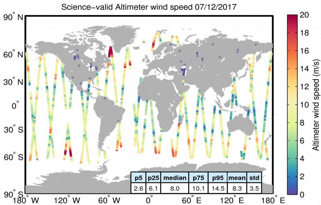
Figure 34. Geographical distribution of science-valid wind data over oceans and lakes for 07/12/2017. The statistical values shown in the table refer to the wind in m/s and are calculated over all measurements shown in the figure. Gray circles denote records that have been rejected based on the editing criteria described in Table 5.
