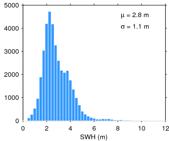
Figure 20. Histogram of science-valid SWH over oceans and lakes for 07/12/2017. The mean ( \mu ) and standard deviation ( \sigma ) are also shown. Note that values larger than 12 m are excluded from the histogram for the sake of readability but not from the computation of \mu and \sigma .
