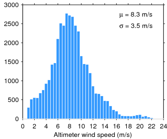
Figure 33. Histogram of flag-valid wind over oceans and lakes for 07/12/2017. The mean ( \mu ) and standard deviation ( \sigma ) are also shown. Note that values larger than 24 m/s are excluded from the histogram for the sake of readability but not from the computation of \mu and \sigma .
