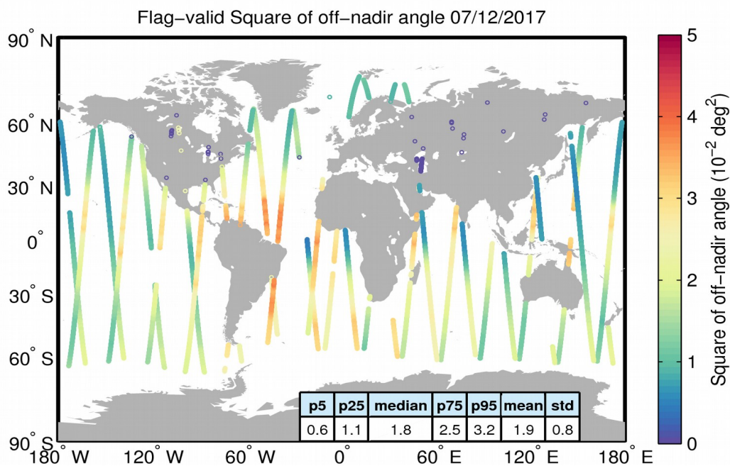
Figure 37. Geographical distribution of flag-valid mispointing data over oceans and lakes for 07/12/2017. The statistical values shown in the table refer to the mispointing in 10^{-2} deg 2 and are calculated over all measurements shown in the figure.
