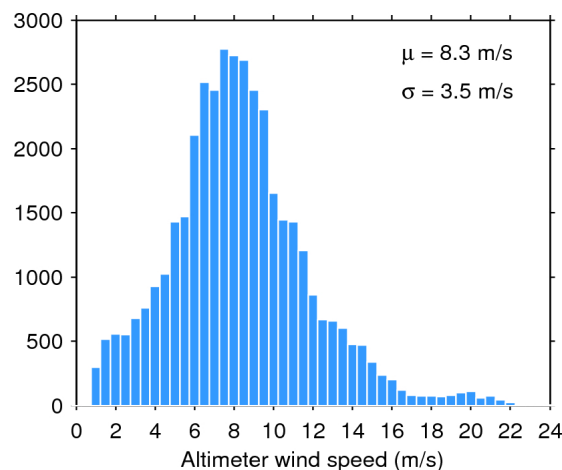
Figure 35. Histogram of science-valid wind over oceans and lakes for 07/12/2017. The mean ( \mu ) and standard deviation ( \sigma ) are also shown. Note that values larger than 24 m/s are excluded from the histogram for the sake of readability but not from the computation of \mu and \sigma .
