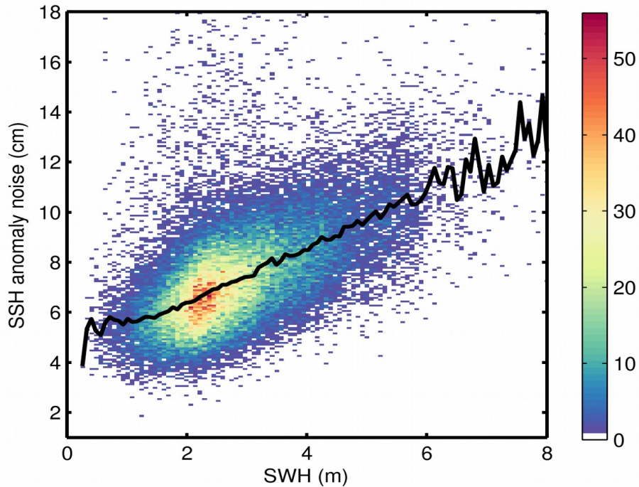
Figure 9. 2D histogram showing flag-valid SSH anomaly noise as a function of SWH for 06/12/2017. The black line denotes the median SSH anomaly noise as a function of SWH.
