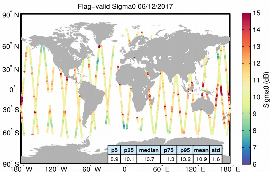
Figure 23. Geographical distribution of flag-valid sigma0 data over oceans and lakes for 06/12/2017. The statistical values shown in the table refer to the sigma0 in dB and are calculated over all measurements shown in the figure.
