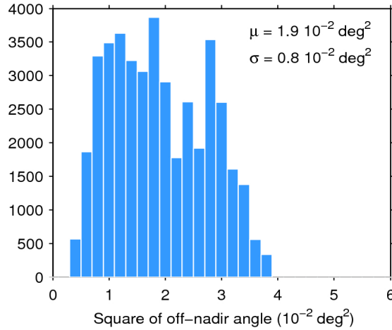
Figure 39. Histogram of flag-valid mispointing over oceans and lakes for 06/12/2017. The mean ( \mu ) and standard deviation ( \sigma ) are also shown. Note that values larger than 6 \cdot 10^{-2} \text{ deg}^2 are excluded from the histogram for the sake of readability but not from the computation of \mu and \sigma .
