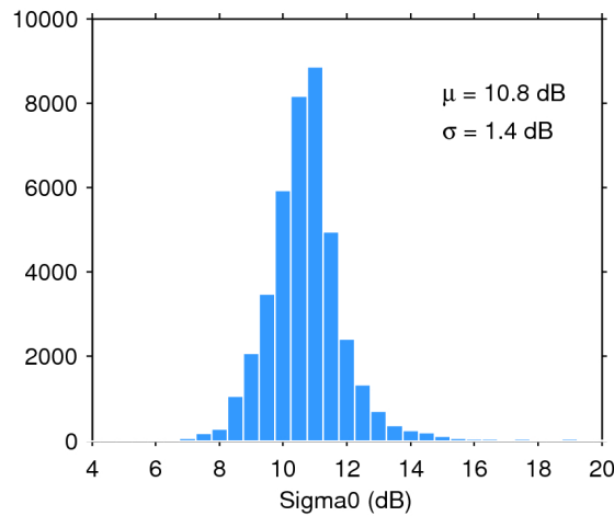
Figure 28. Histogram of science-valid sigma0 over oceans and lakes for 06/12/2017. The mean ( \mu ) and standard deviation ( \sigma ) are also shown. Note that values outside [4 20] dB are excluded from the histogram for the sake of readability but not from the computation of \mu and \sigma .
