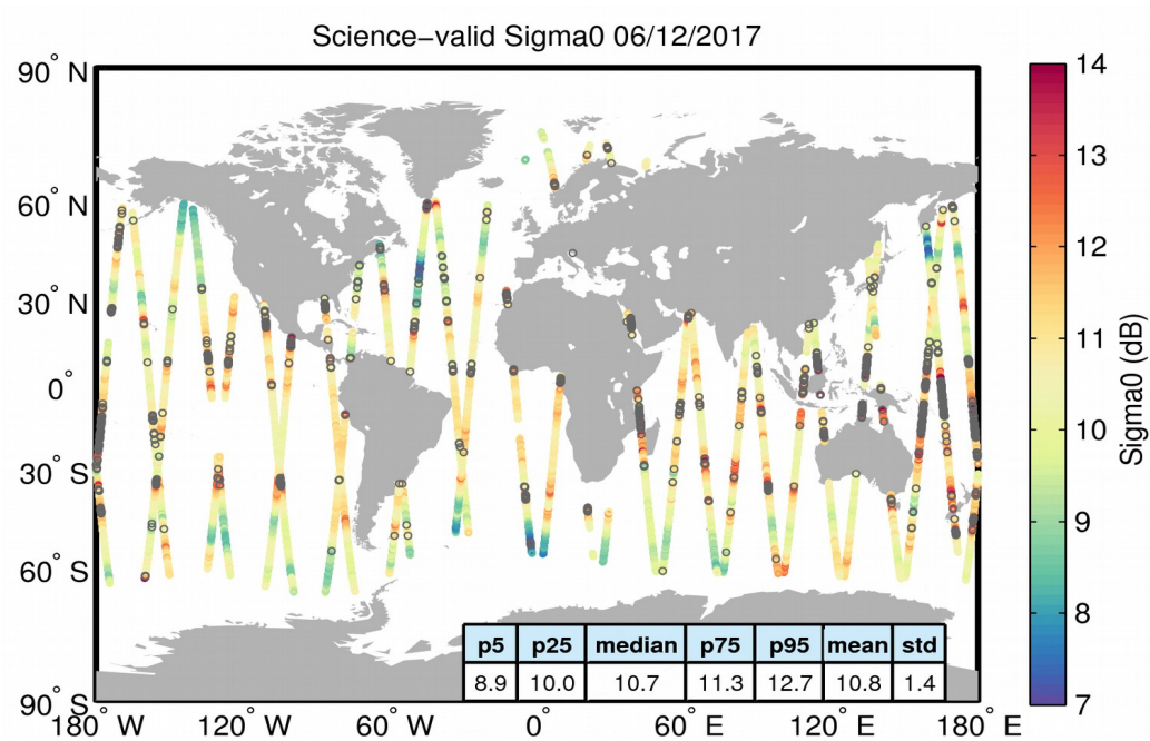
Figure 27. Geographical distribution of science-valid sigma0 data over oceans and lakes for 06/12/2017. The statistical values shown in the table refer to the sigma0 in dB and are calculated over all measurements shown in the figure. Gray circles denote records that have been rejected based on the editing criteria described in Table 4.
