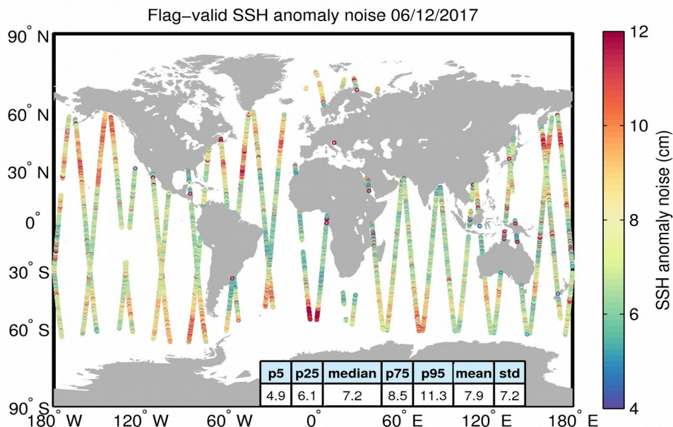
Figure 8. Geographical distribution of flag-valid 20-Hz SSH anomaly measurement noise over oceans and lakes for 06/12/2017. The statistical values shown in the table refer to the SSH anomaly noise and are calculated over all measurements shown in the figure.
