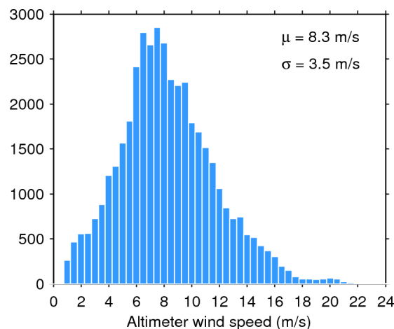
Figure 35. Histogram of science-valid wind over oceans and lakes for 06/12/2017. The mean ( \mu ) and standard deviation ( \sigma ) are also shown. Note that values larger than 24 m/s are excluded from the histogram for the sake of readability but not from the computation of \mu and \sigma .
