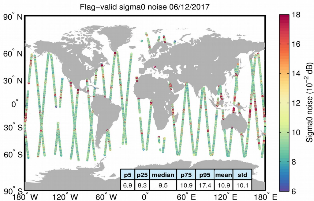
Figure 26. Geographical distribution of flag-valid 20-Hz sigma0 measurement noise over oceans and lakes for 06/12/2017. The statistical values shown in the table refer to the sigma0 noise and are calculated over all measurements shown in the figure.
