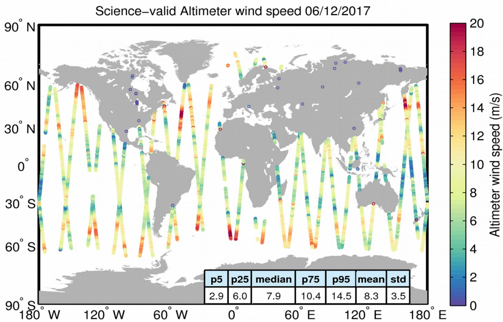
Figure 34. Geographical distribution of science-valid wind data over oceans and lakes for 06/12/2017. The statistical values shown in the table refer to the wind in m/s and are calculated over all measurements shown in the figure. Gray circles denote records that have been rejected based on the editing criteria described in Table 5.
