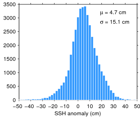
Figure 7. Histogram of flag-valid SSH anomaly over oceans and lakes for 06/12/2017. The mean ( \mu ) and standard deviation ( \sigma ) are also shown. Note that values outside [-50 50] cm are excluded from the histogram for the sake of readability but not from the computation of \mu and \sigma .
