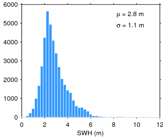
Figure 20. Histogram of science-valid SWH over oceans and lakes for 06/12/2017. The mean ( \mu ) and standard deviation ( \sigma ) are also shown. Note that values larger than 12 m are excluded from the histogram for the sake of readability but not from the computation of \mu and \sigma .
