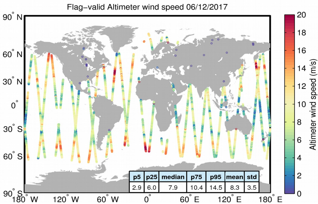
Figure 31. Geographical distribution of flag-valid wind data over oceans and lakes for 06/12/2017. The statistical values shown in the table refer to the wind in m/s and are calculated over all measurements shown in the figure.
