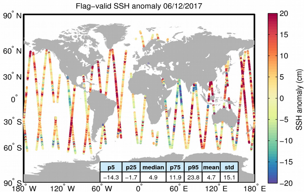
Figure 5. Geographical distribution of flag-valid 1-Hz SSH anomaly data over oceans and lakes for 06/12/2017. The statistical values shown in the table refer to the SSH anomaly in cm and are calculated over all measurements shown in the figure.
