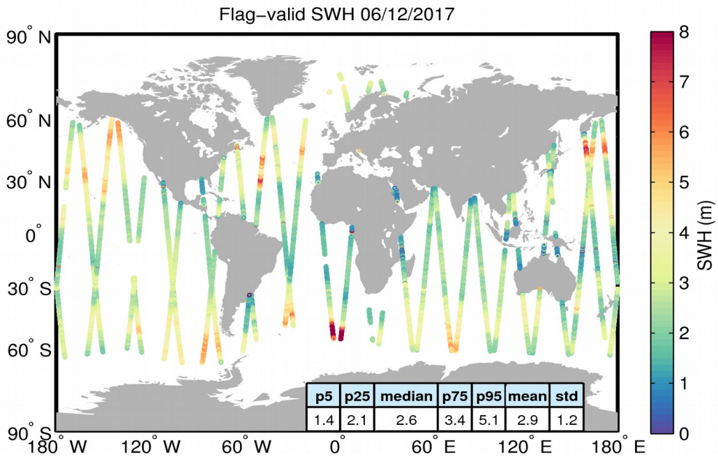
Figure 15. Geographical distribution of flag-valid SWH data over oceans and lakes for 06/12/2017. The statistical values shown in the table refer to the SWH in m and are calculated over all measurements shown in the figure.
