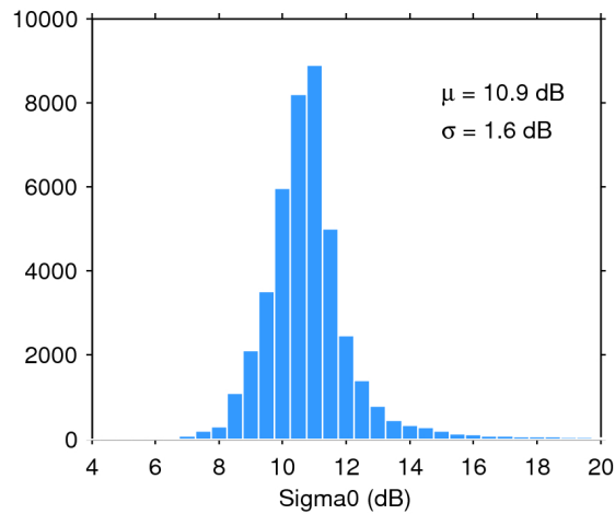
Figure 25. Histogram of flag-valid sigma0 over oceans and lakes for 06/12/2017. The mean ( \mu ) and standard deviation ( \sigma ) are also shown. Note that values outside [4 20] dB are excluded from the histogram for the sake of readability but not from the computation of \mu and \sigma .
