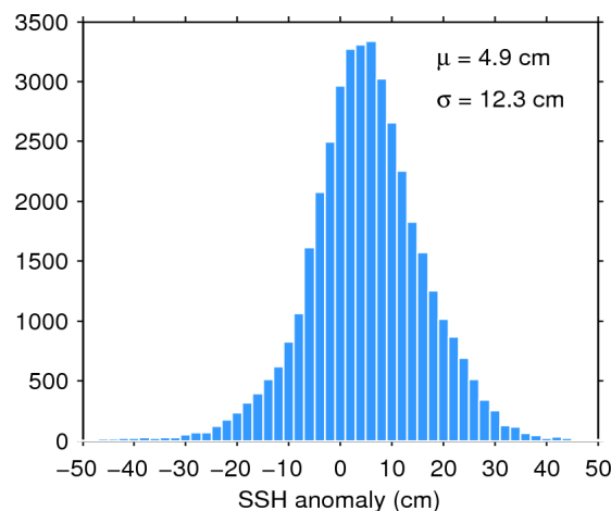
Figure 11. Histogram of science-valid SSH anomaly over oceans and lakes for 06/12/2017. The mean ( \mu ) and standard deviation ( \sigma ) are also shown. Note that values outside [-50 50] cm are excluded from the histogram for the sake of readability but not from the computation of \mu and \sigma .
