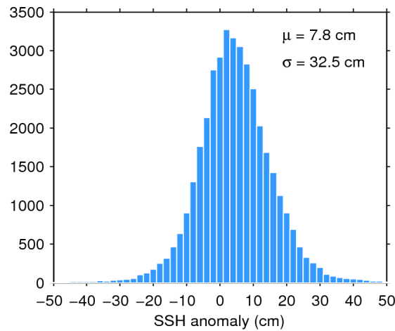
Figure 7. Histogram of flag-valid SSH anomaly over oceans and lakes for 05/12/2017. The mean ( \mu ) and standard deviation ( \sigma ) are also shown. Note that values outside [-50\ 50] cm are excluded from the histogram for the sake of readability but not from the computation of \mu and \sigma .
