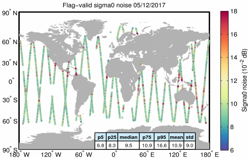
Figure 26. Geographical distribution of flag-valid 20-Hz sigma0 measurement noise over oceans and lakes for 05/12/2017. The statistical values shown in the table refer to the sigma0 noise and are calculated over all measurements shown in the figure.
