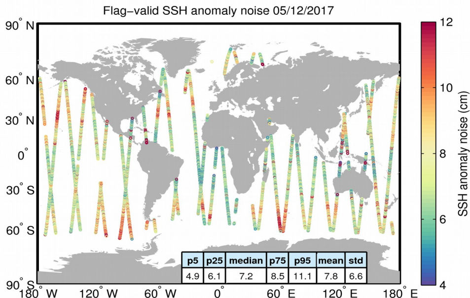
Figure 8. Geographical distribution of flag-valid 20-Hz SSH anomaly measurement noise over oceans and lakes for 05/12/2017. The statistical values shown in the table refer to the SSH anomaly noise and are calculated over all measurements shown in the figure.
