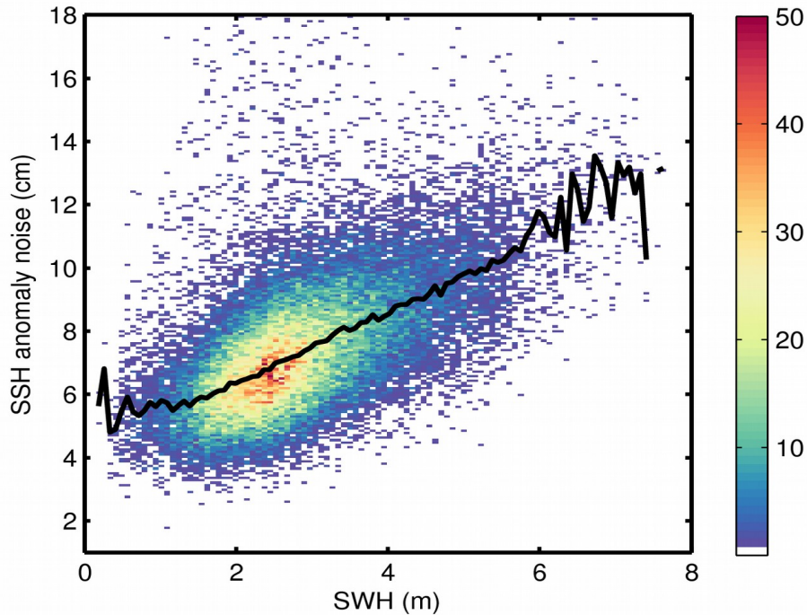
Figure 9. 2D histogram showing flag-valid SSH anomaly noise as a function of SWH for 05/12/2017. The black line denotes the median SSH anomaly noise as a function of SWH.
