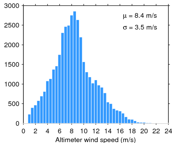
Figure 35. Histogram of science-valid wind over oceans and lakes for 05/12/2017. The mean ( \mu ) and standard deviation ( \sigma ) are also shown. Note that values larger than 24 m/s are excluded from the histogram for the sake of readability but not from the computation of \mu and \sigma .
