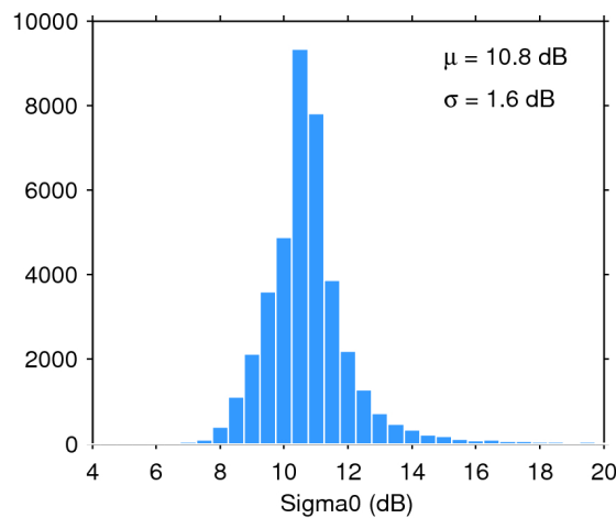
Figure 25. Histogram of flag-valid sigma0 over oceans and lakes for 05/12/2017. The mean ( \mu ) and standard deviation ( \sigma ) are also shown. Note that values outside [4 20] dB are excluded from the histogram for the sake of readability but not from the computation of \mu and \sigma .
