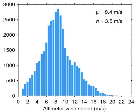
Figure 33. Histogram of flag-valid wind over oceans and lakes for 05/12/2017. The mean ( \mu ) and standard deviation ( \sigma ) are also shown. Note that values larger than 24 m/s are excluded from the histogram for the sake of readability but not from the computation of \mu and \sigma .
