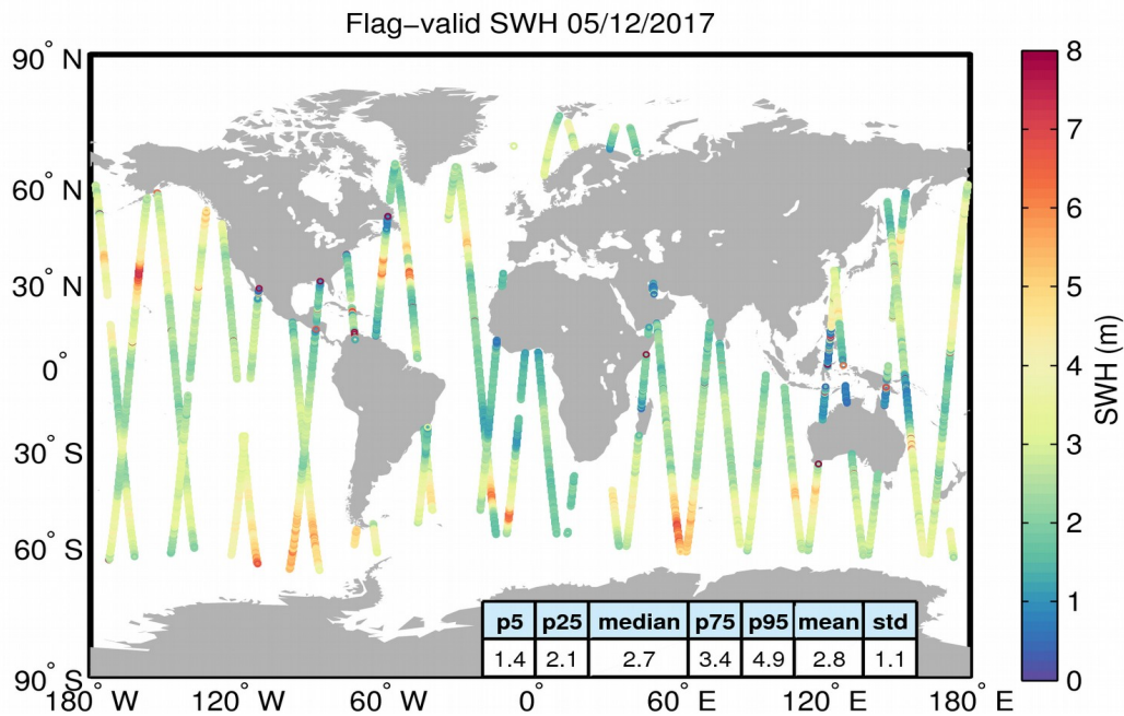
Figure 15. Geographical distribution of flag-valid SWH data over oceans and lakes for 05/12/2017. The statistical values shown in the table refer to the SWH in m and are calculated over all measurements shown in the figure.
