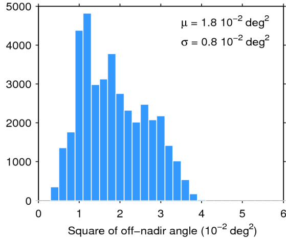
Figure 39. Histogram of flag-valid mispointing over oceans and lakes for 05/12/2017. The mean ( \mu ) and standard deviation ( \sigma ) are also shown. Note that values larger than 6 \cdot 10^{-2} \text{ deg}^2 are excluded from the histogram for the sake of readability but not from the computation of \mu and \sigma .
