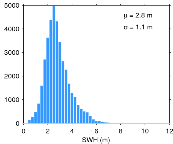
Figure 17. Histogram of flag-valid SWH over oceans and lakes for 05/12/2017. The mean ( \mu ) and standard deviation ( \sigma ) are also shown. Note that values larger than 12 m are excluded from the histogram for the sake of readability but not from the computation of \mu and \sigma .
