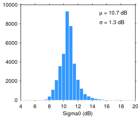
Figure 28. Histogram of science-valid sigma0 over oceans and lakes for 05/12/2017. The mean ( \mu ) and standard deviation ( \sigma ) are also shown. Note that values outside [4 20] dB are excluded from the histogram for the sake of readability but not from the computation of \mu and \sigma .
