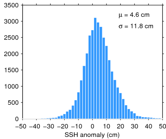
Figure 11. Histogram of science-valid SSH anomaly over oceans and lakes for 05/12/2017. The mean ( \mu ) and standard deviation ( \sigma ) are also shown. Note that values outside [-50 50] cm are excluded from the histogram for the sake of readability but not from the computation of \mu and \sigma .
