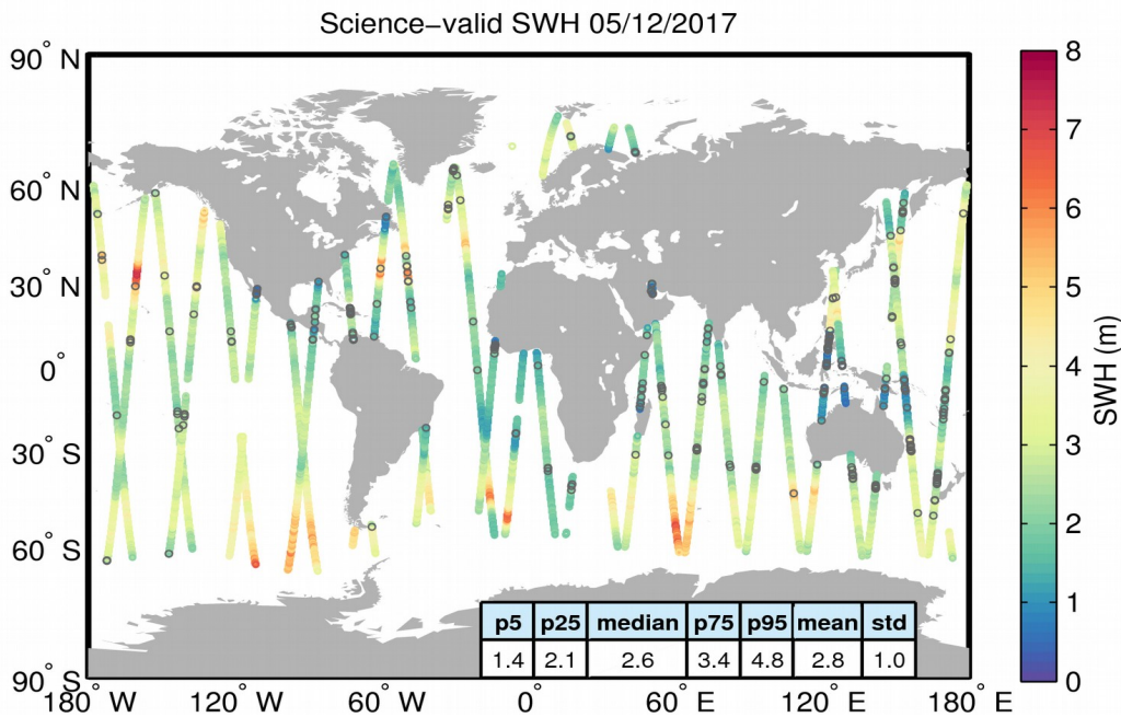
Figure 19. Geographical distribution of science-valid SWH data over oceans and lakes for 05/12/2017. The statistical values shown in the table refer to the SWH in m and are calculated over all measurements shown in the figure. Gray circles denote records that have been rejected based on the editing criteria described in Table 3.
