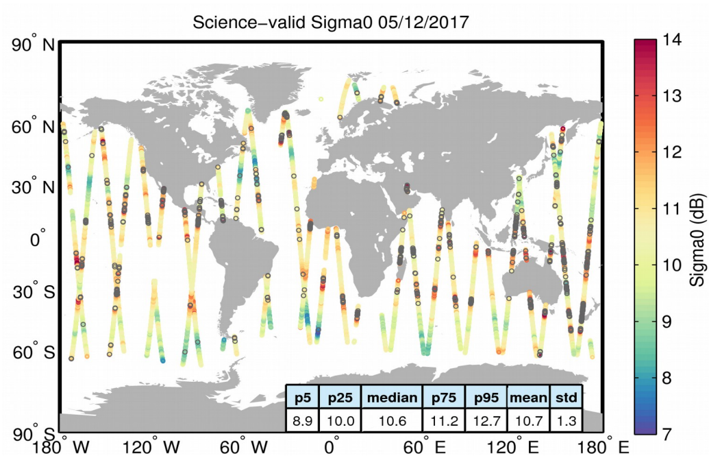
Figure 27. Geographical distribution of science-valid sigma0 data over oceans and lakes for 05/12/2017. The statistical values shown in the table refer to the sigma0 in dB and are calculated over all measurements shown in the figure. Gray circles denote records that have been rejected based on the editing criteria described in Table 4.
