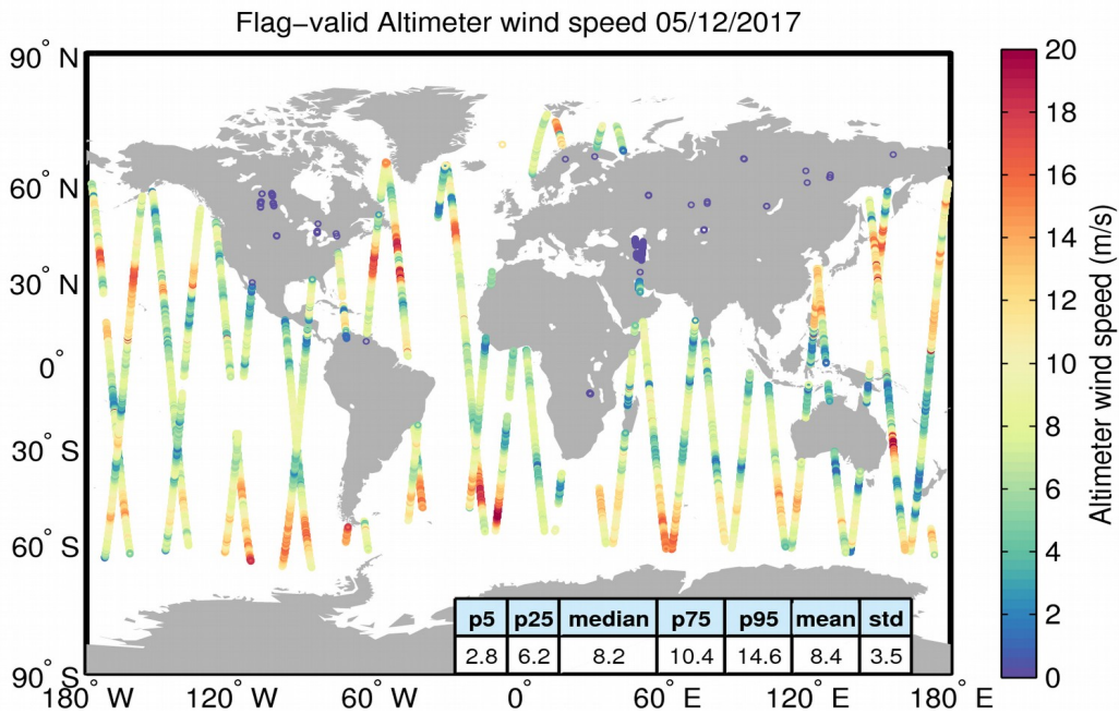
Figure 31. Geographical distribution of flag-valid wind data over oceans and lakes for 05/12/2017. The statistical values shown in the table refer to the wind in m/s and are calculated over all measurements shown in the figure.
