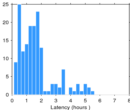
Figure 2. Histogram of the data latency for 05/12/2017. The y-axis denotes the number of files that are made available with a delay of x-hours with respect to the mean time of the records stored in the file.
