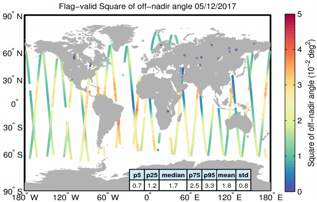
Figure 37. Geographical distribution of flag-valid mispointing data over oceans and lakes for 05/12/2017. The statistical values shown in the table refer to the mispointing in 10^{-2} deg 2 and are calculated over all measurements shown in the figure.
