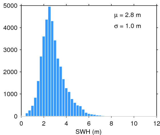
Figure 20. Histogram of science-valid SWH over oceans and lakes for 05/12/2017. The mean ( \mu ) and standard deviation ( \sigma ) are also shown. Note that values larger than 12 m are excluded from the histogram for the sake of readability but not from the computation of \mu and \sigma .
