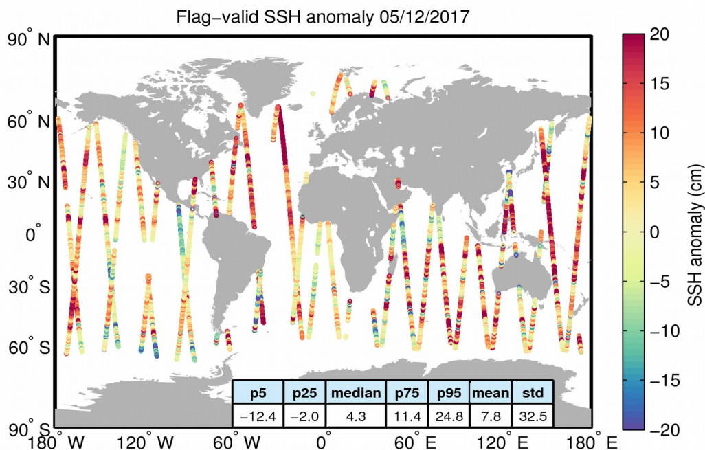
Figure 5. Geographical distribution of flag-valid 1-Hz SSH anomaly data over oceans and lakes for 05/12/2017. The statistical values shown in the table refer to the SSH anomaly in cm and are calculated over all measurements shown in the figure.
