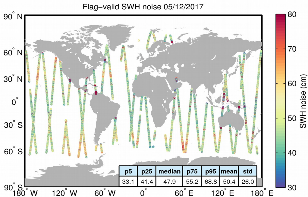
Figure 18. Geographical distribution of flag-valid 20-Hz SWH measurement noise over oceans and lakes for 05/12/2017. The statistical values shown in the table refer to the SWH noise and are calculated over all measurements shown in the figure.
