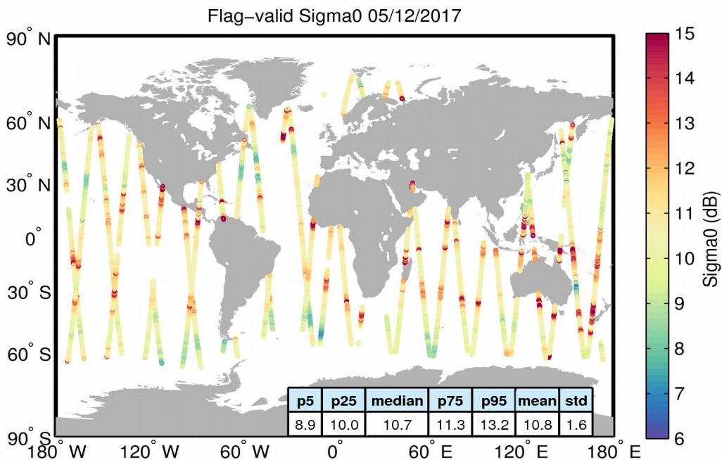
Figure 23. Geographical distribution of flag-valid sigma0 data over oceans and lakes for 05/12/2017. The statistical values shown in the table refer to the sigma0 in dB and are calculated over all measurements shown in the figure.
